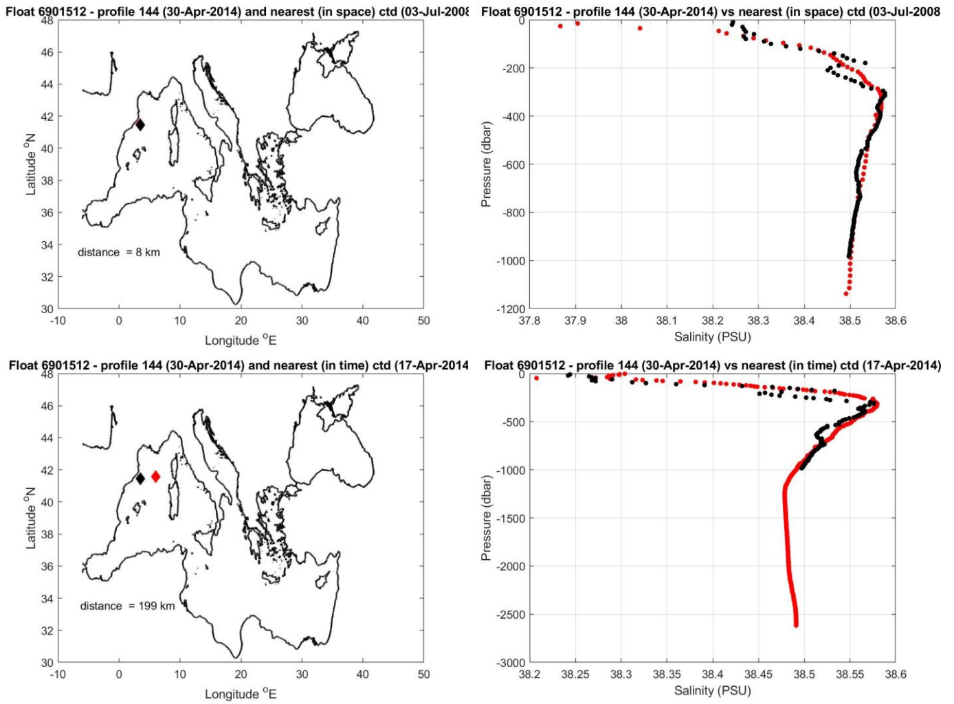
Figure 11: Float 6901512. The salinity float profile number 144 (black dots) are compared to the nearest in space (top) and in time (bottom) reference profile (red dots). The locations of the two profiles and their distance is given in the left panel.
