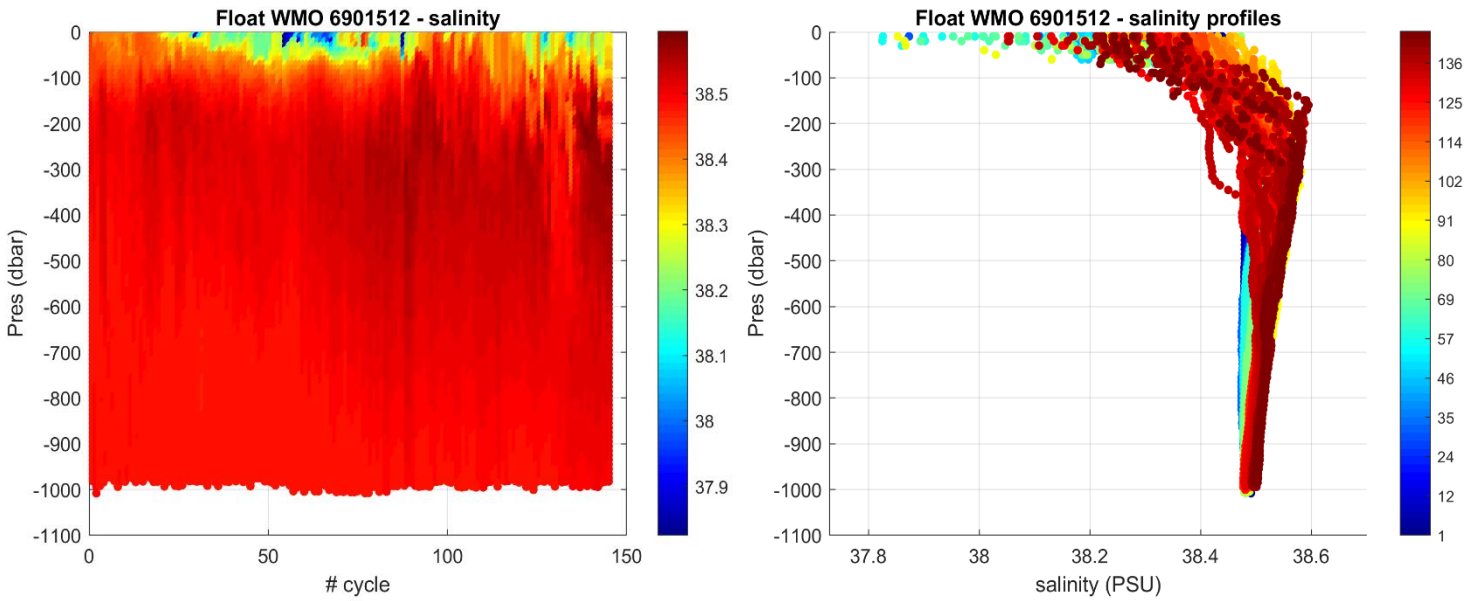
Figure 3: Float 6901512. Time series of Argo float potential salinity (PSS-78) on the left, and salinity profiles color-coded per cycle number on the right.
