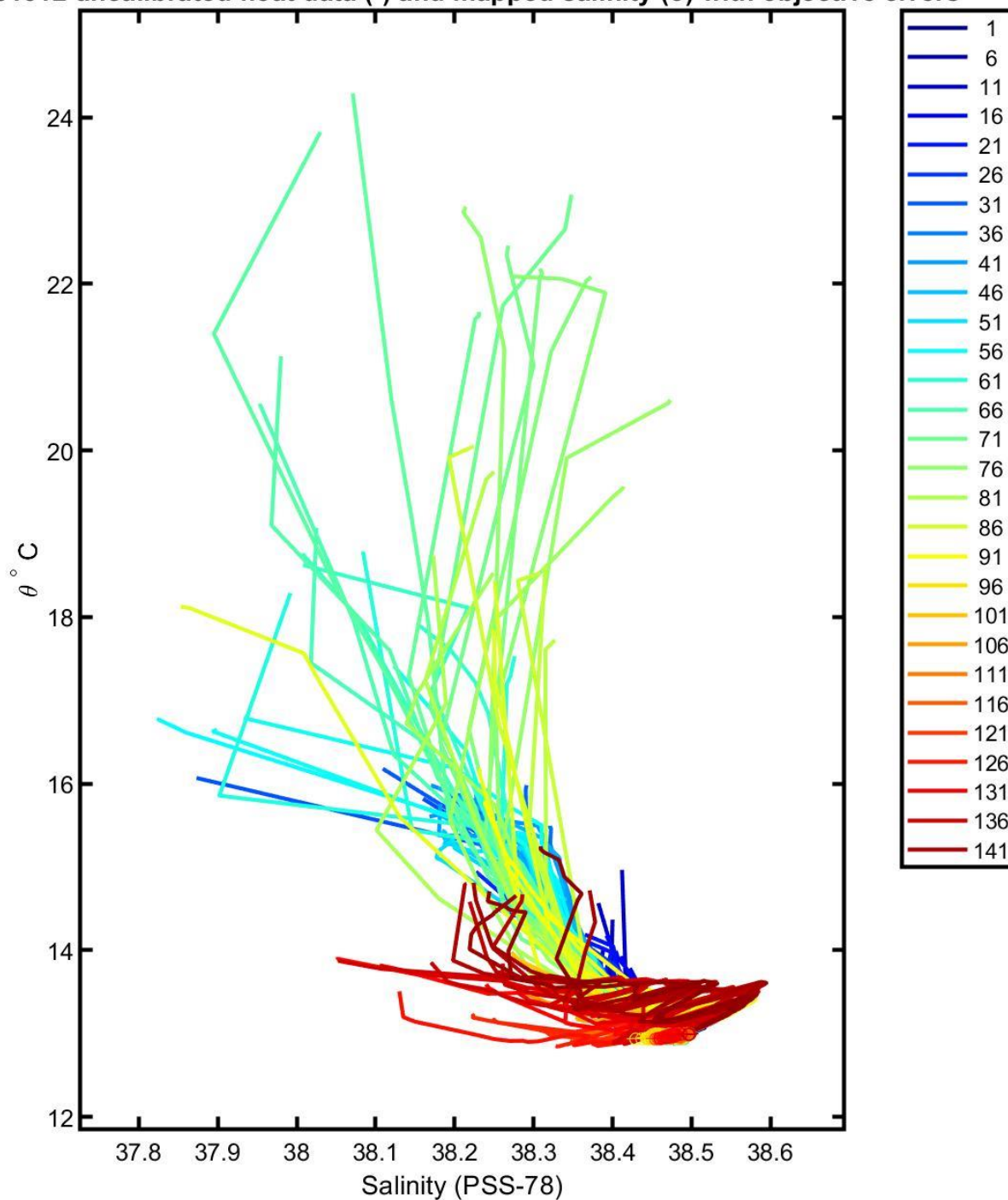
6901512 uncalibrated float data (-) and mapped salinity (o) with objective errors
