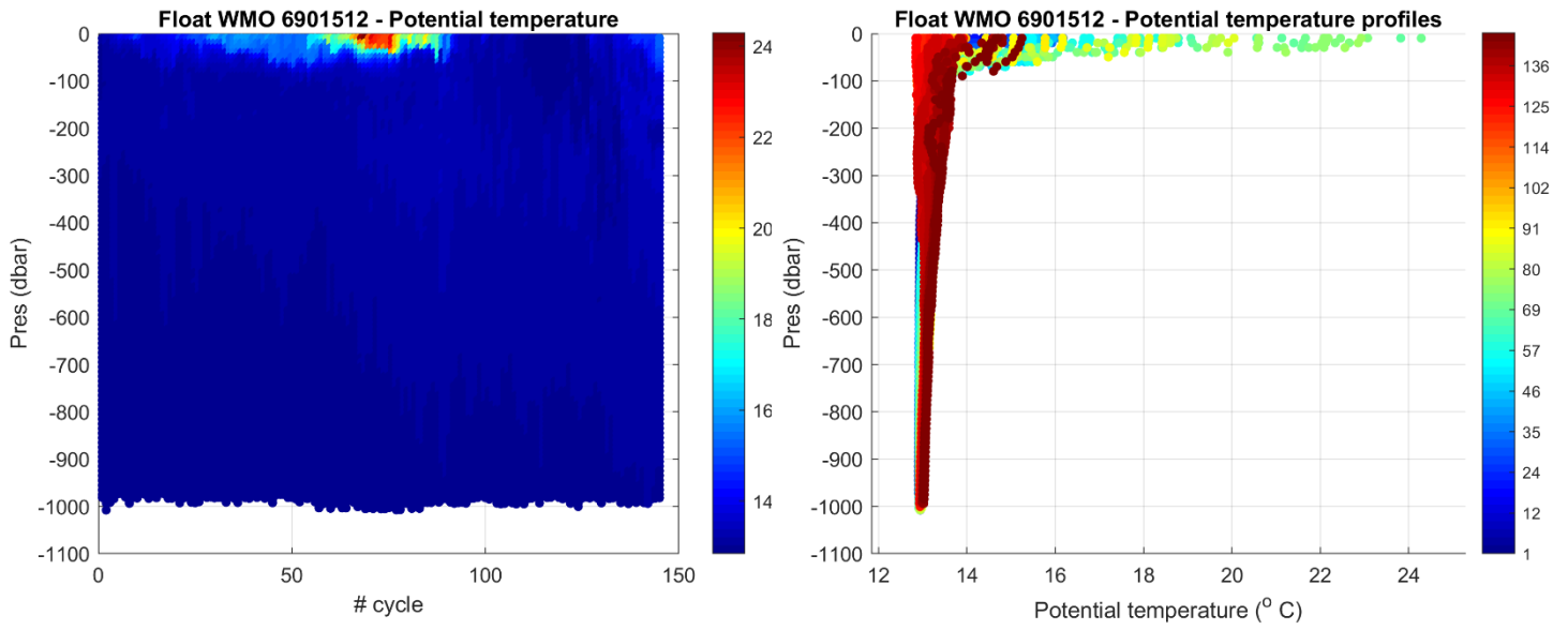
Figure 2: Float 6901512. Time series of Argo float potential temperature ( ^{\circ}\text{C} ) on the left, and potential temperature profiles color-coded per cycle number on the right.
