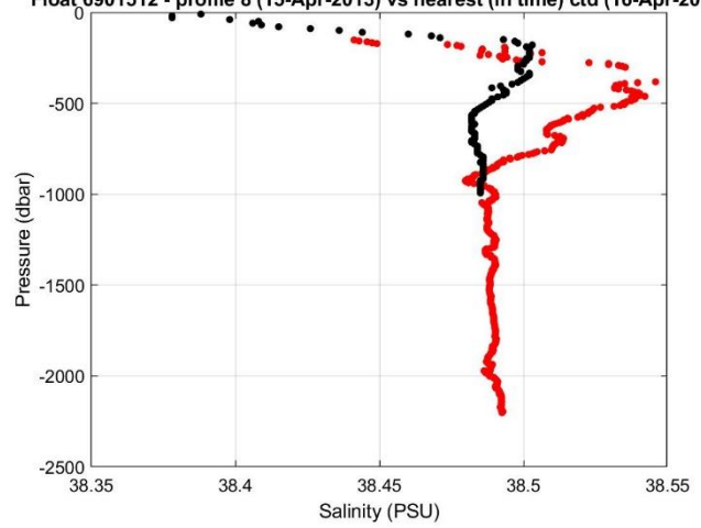
Figure 9: Float 6901512. The salinity float profile number 8 (black dots) are compared to the nearest in space (top) and in time (bottom) reference profile (red dots). The locations of the two profiles and their distance is given in the left panel.
