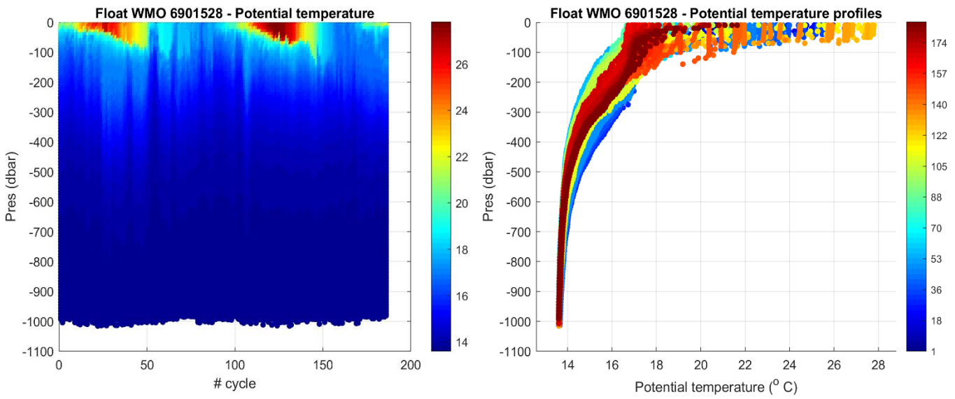
Figure 2: Float 6901528. Time series of Argo float potential temperature ( ^{\circ}\text{C} ) on the left, and potential temperature profiles color-coded per cycle number on the right.
