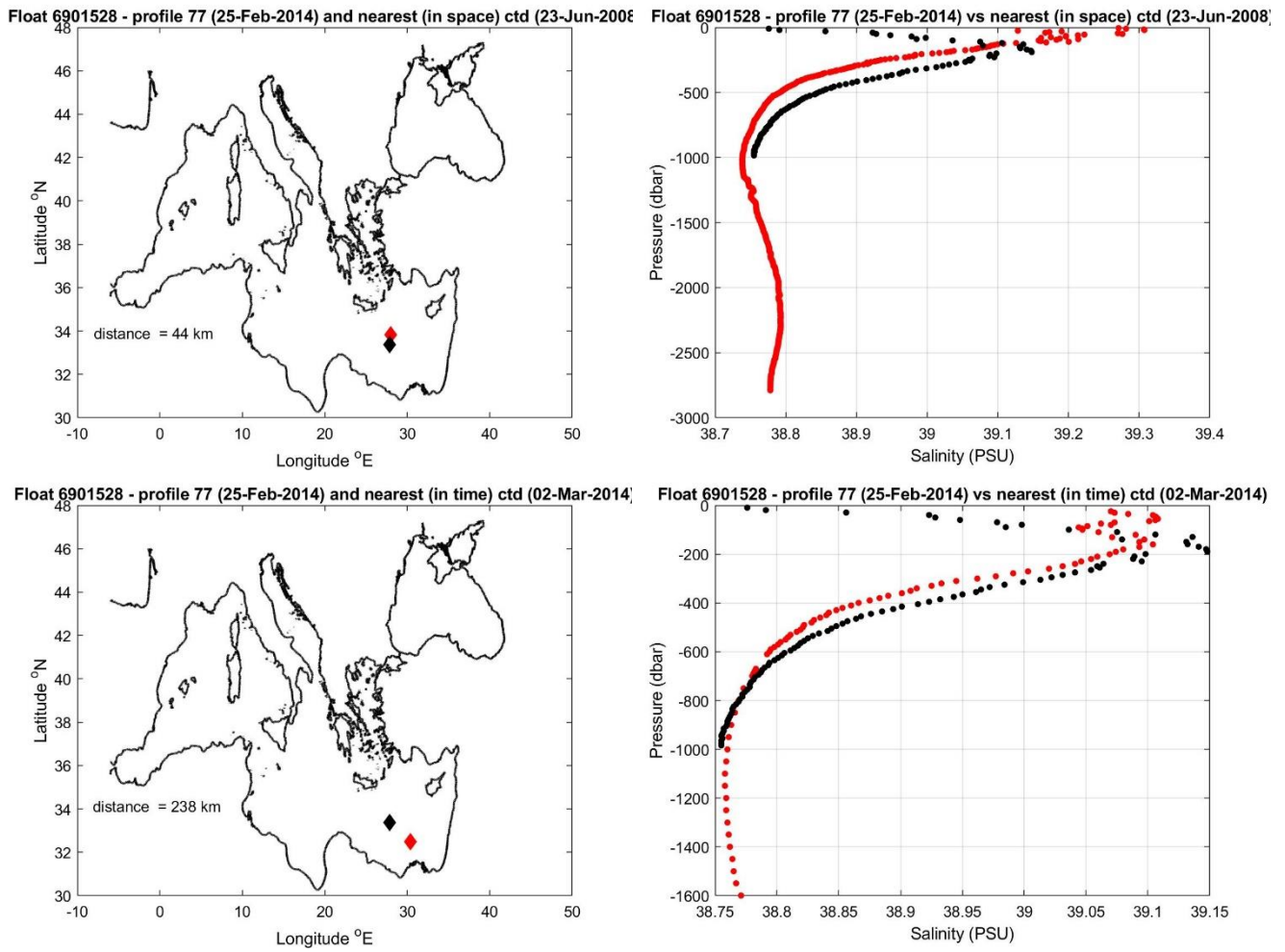
Figure 10: Float 6901528. The salinity float profile number 77 (black dots) are compared to the nearest in space (top) and in time (bottom) reference profile (red dots). The locations of the two profiles and their distance is given in the left panel.
