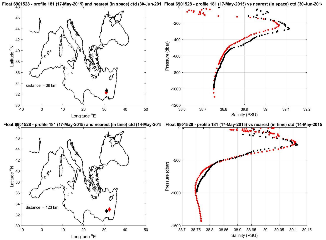
Figure 11: Float 6901528. The salinity float profile number 181 (black dots) are compared to the nearest in space (top) and in time (bottom) reference profile (red dots). The locations of the two profiles and their distance is given in the left panel.
