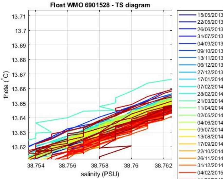
Figure 4: Float 6901528. \theta -S diagram color-coded per cycle number.
