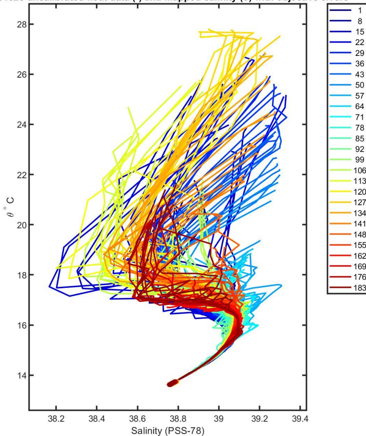
6901528 uncalibrated float data (-) and mapped salinity (o) with objective errors
