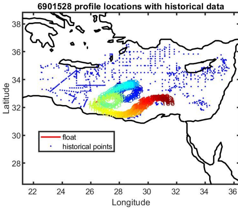
Figure 13: Float 6901528. Location of the float profiles (red line with colored numbers) and the reference data selected for mapping (blue dots).
