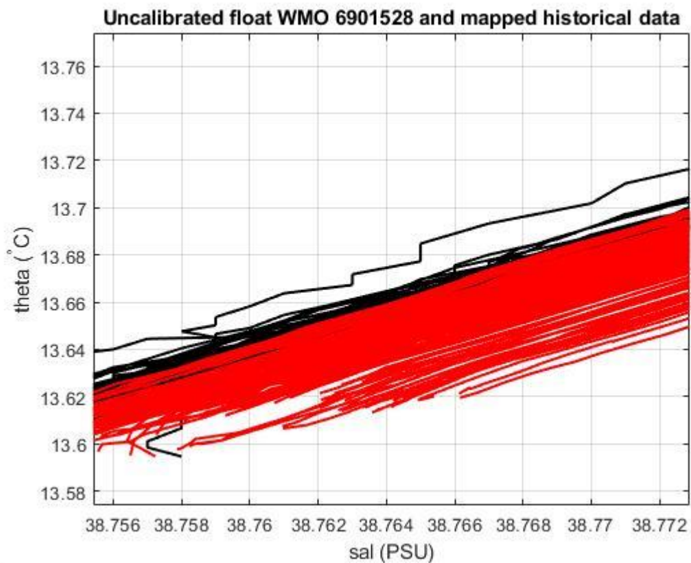
Figure 19: Float 6901528. Uncalibrated float salinity profile (black lines) and mapped historical data (red lines) in the most uniform part of the \theta -S curve.
