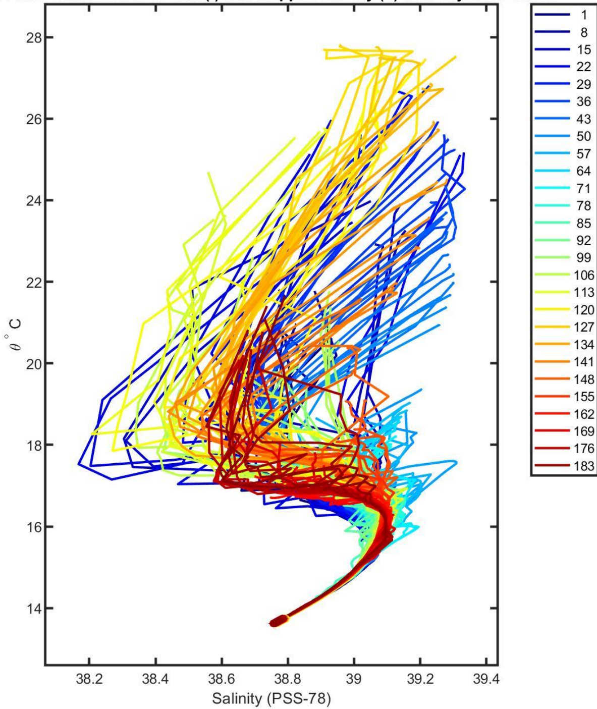
6901528 calibrated float data (-) and mapped salinity (o) with objective errors
