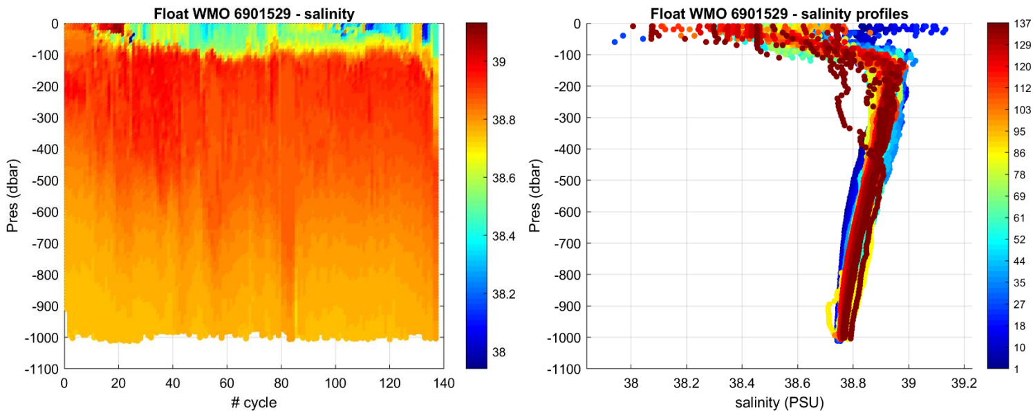
Figure 3: Float 6901529. Time series of Argo float potential salinity (PSS-78) on the left, and salinity profiles color-coded per cycle number on the right.
