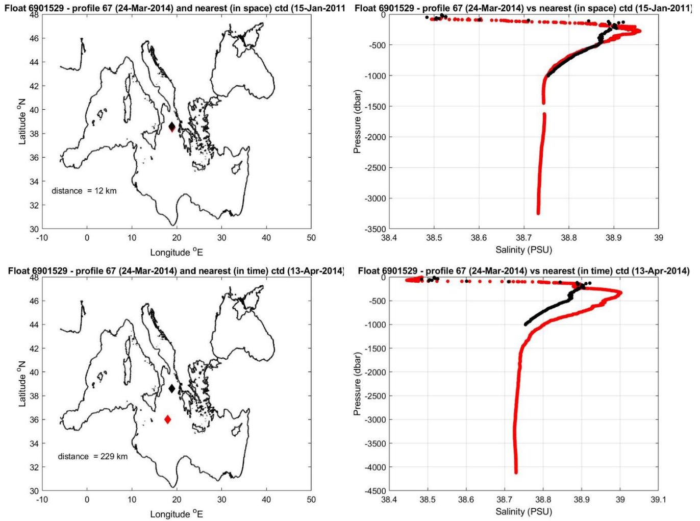
Figure 10: Float 6901529. The salinity float profile number 67 (black dots) are compared to the nearest in space (top) and in time (bottom) reference profile (red dots). The locations of the two profiles and their distance is given in the left panel.
