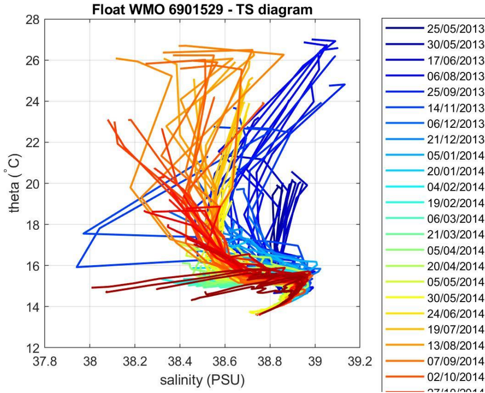
Figure 4: Float 6901529. \theta -S diagram color-coded per cycle number.
