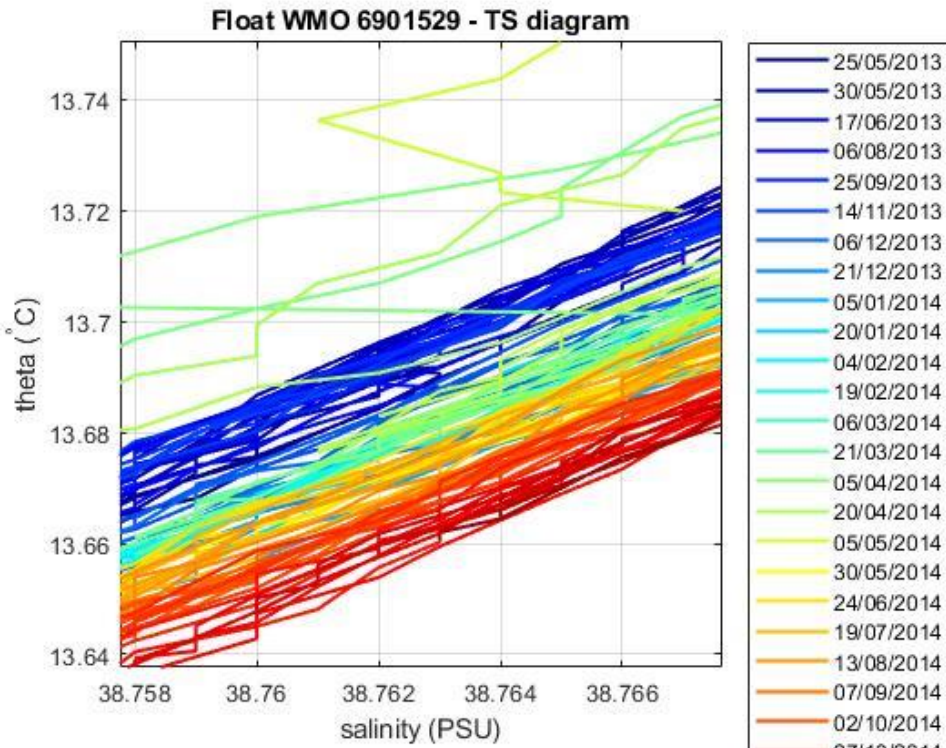
Figure 5: Float 6901529. Area of the \theta -S diagram (color-coded per cycle number) where the \theta -S relationship is more uniform.
