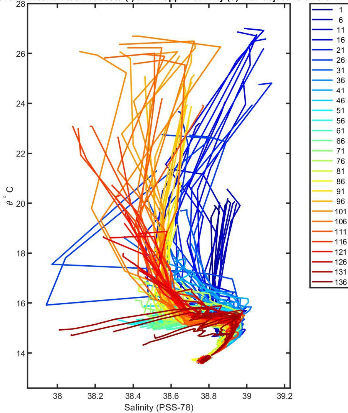
6901529 uncalibrated float data (-) and mapped salinity (o) with objective errors
