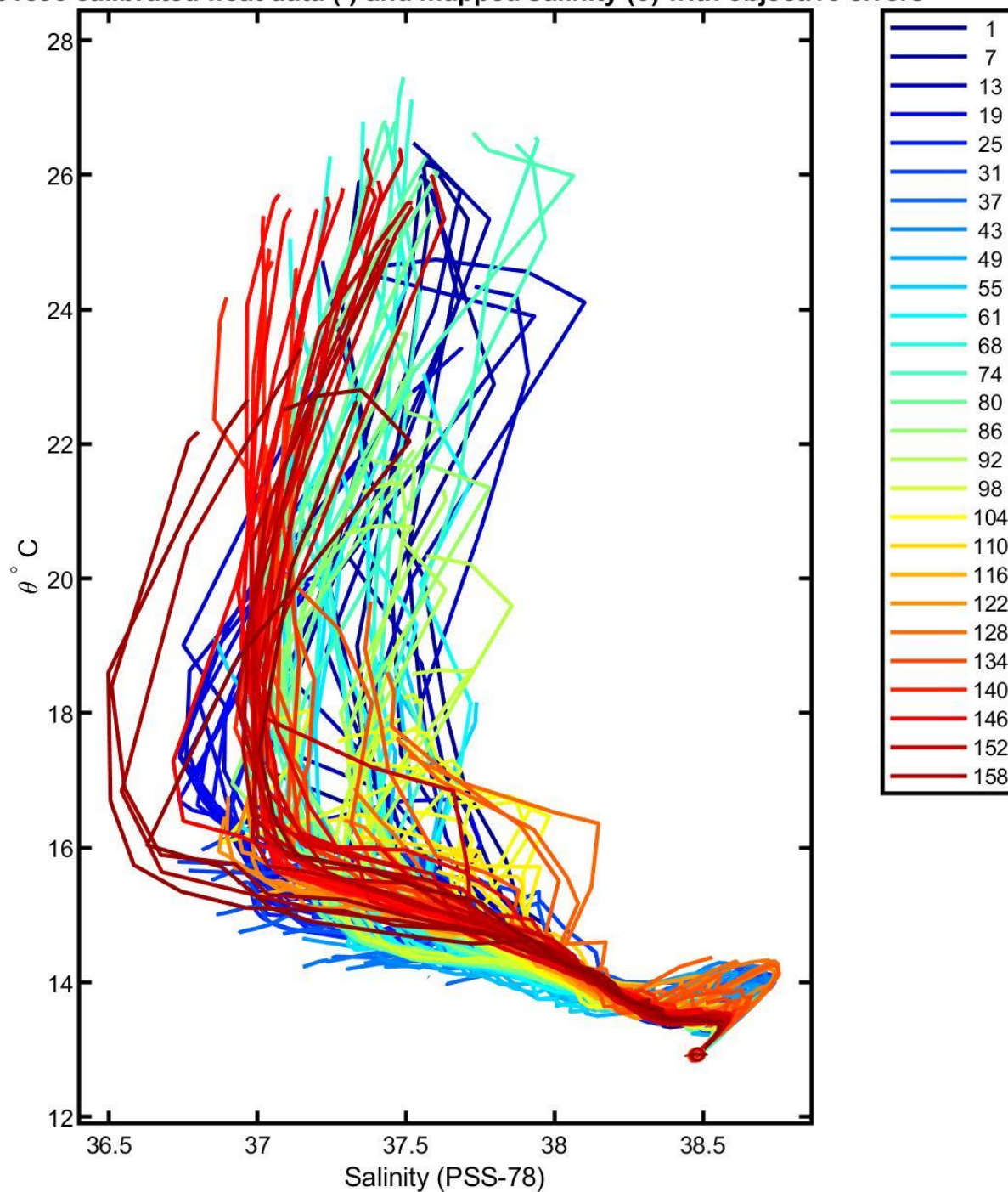
6901596 calibrated float data (-) and mapped salinity (o) with objective errors
