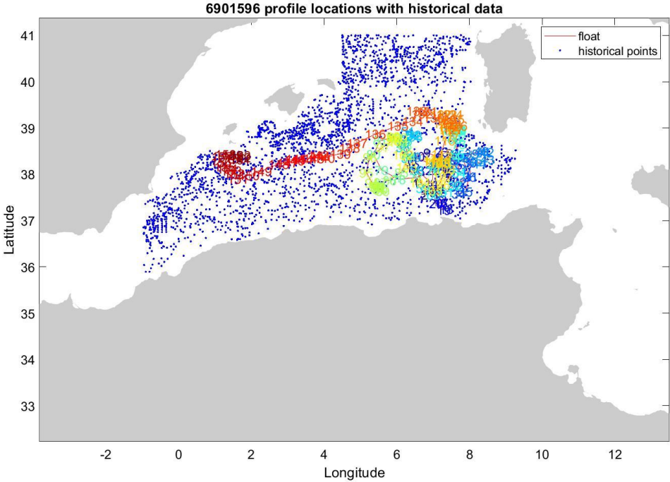
Figure 1: Location of the float profiles (red line with colored numbers) and the reference data selected for mapping (blue dots).
