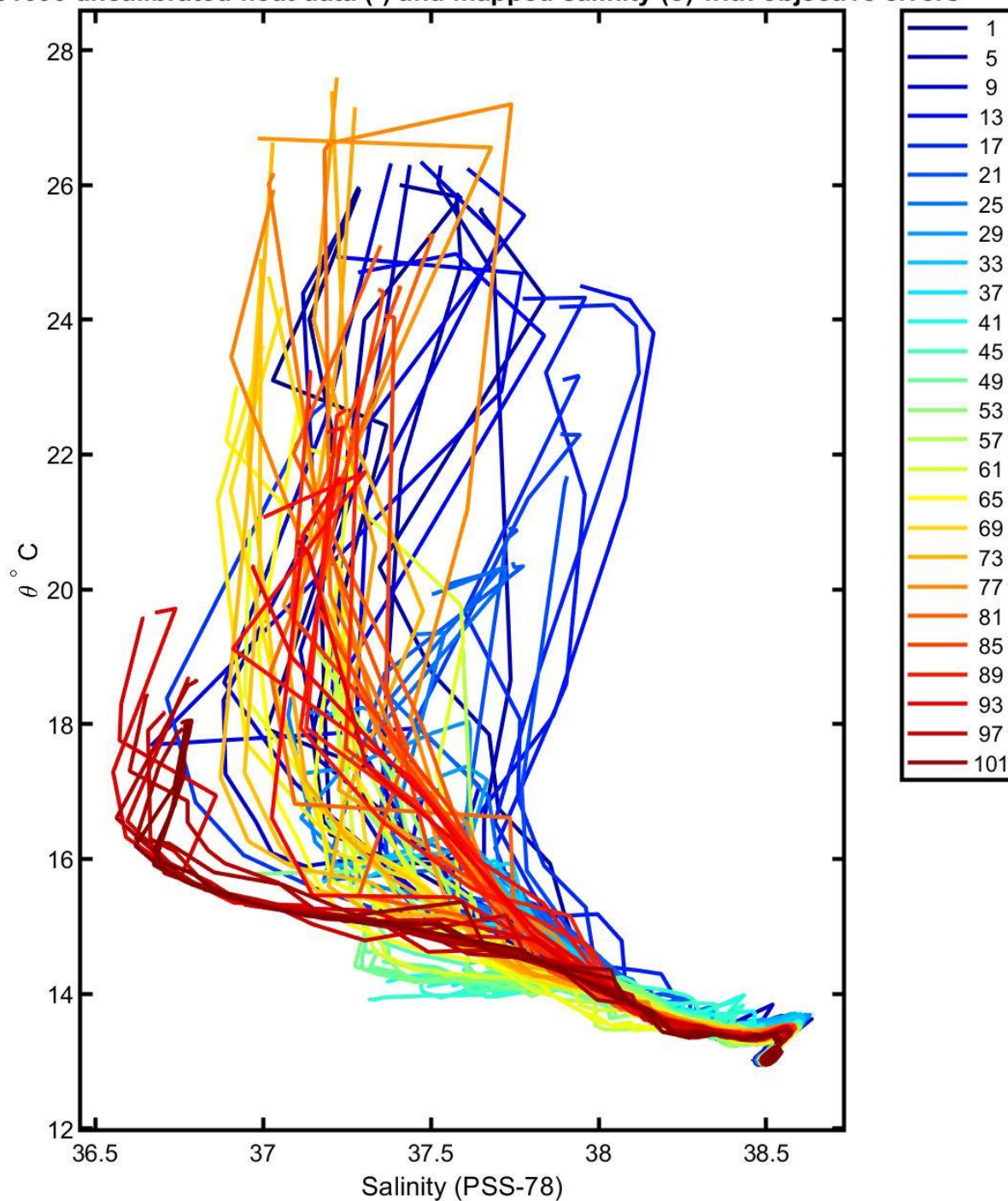
6901600 uncalibrated float data (-) and mapped salinity (o) with objective errors
