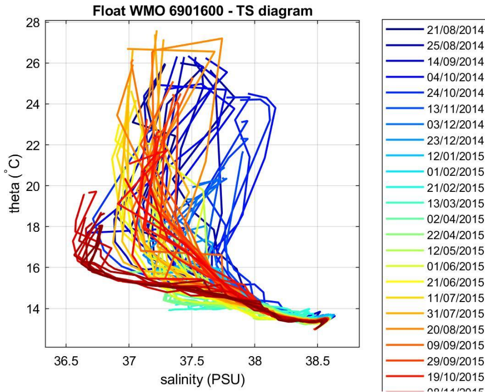
Figure 4: Float 6901600. \theta -S diagram color-coded per cycle number.
