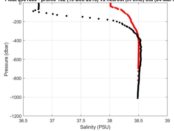
Float 6901600 - profile 102 (19-Dec-2015) vs nearest (in time) ctd (04-Mar-2014)
