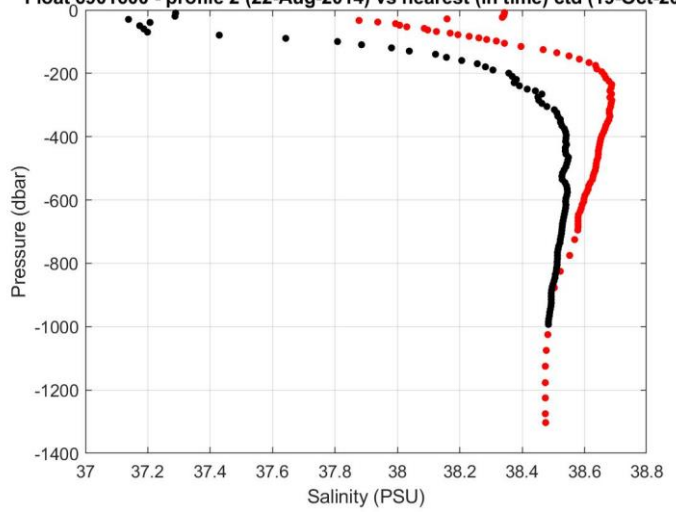
Figure 9: Float 6901600. The salinity float profile number 2 (black dots) are compared to the nearest in space (top) and in time (bottom) reference profile (red dots). The locations of the two profiles and their distance is given in the left panel.
