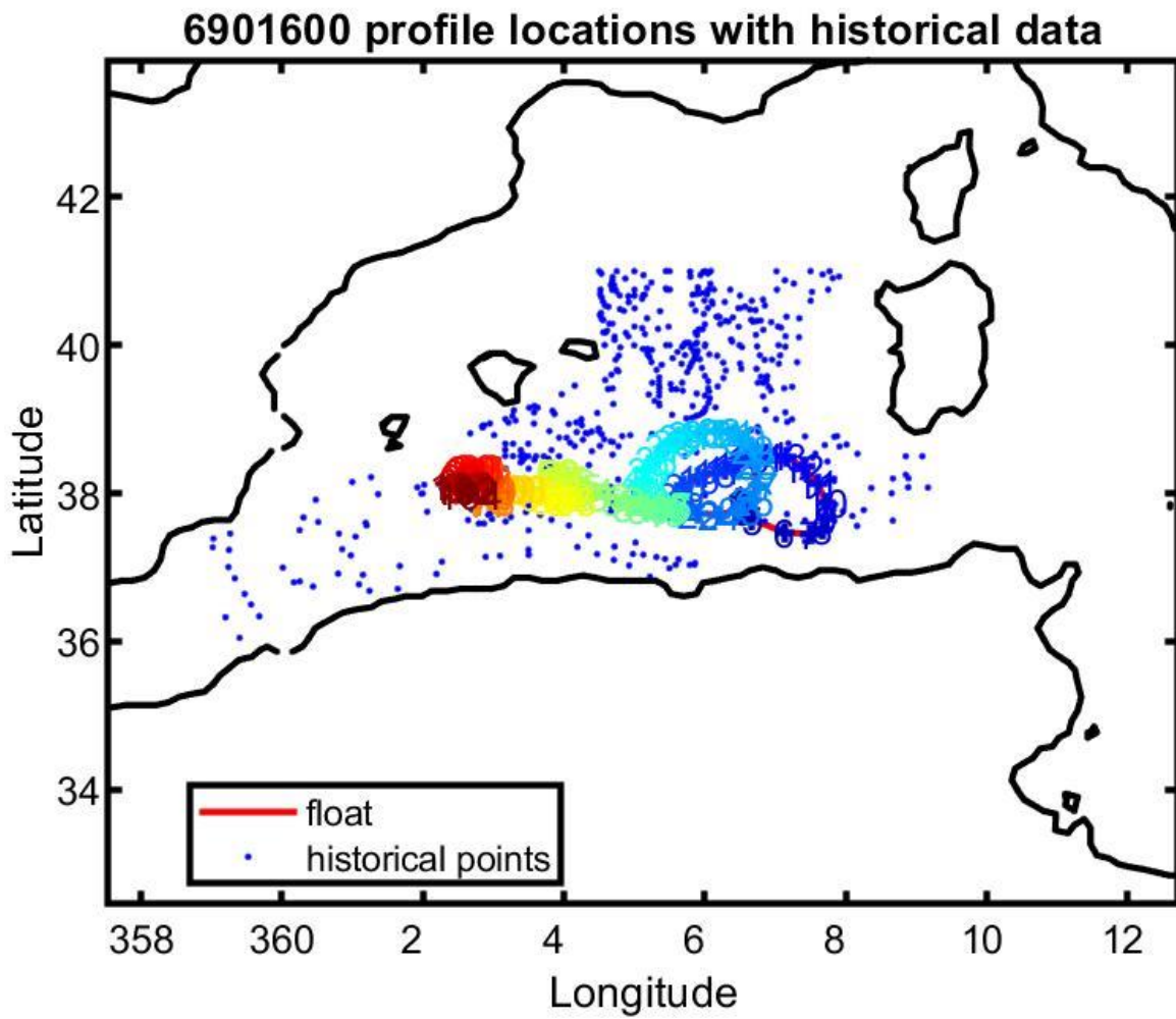
Figure 13: Float 6901600. Location of the float profiles (red line with colored numbers) and the reference data selected for mapping (blue dots).
