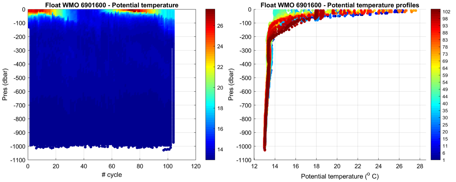
Figure 2: Float 6901600. Time series of Argo float potential temperature ( ^{\circ}\text{C} ) on the left, and potential temperature profiles color-coded per cycle number on the right.
