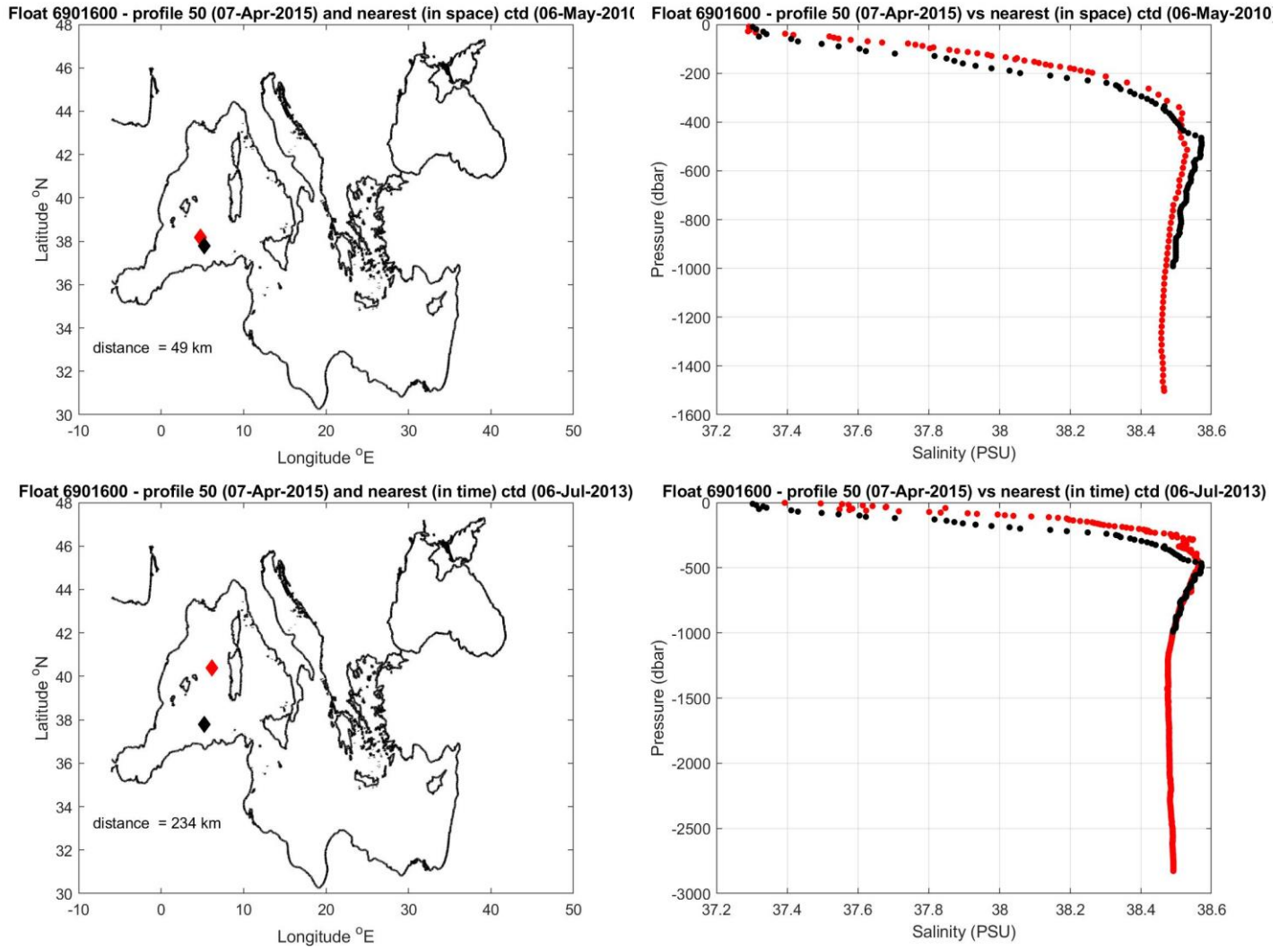
Figure 10: Float 6901600. The salinity float profile number 50 (black dots) are compared to the nearest in space (top) and in time (bottom) reference profile (red dots). The locations of the two profiles and their distance is given in the left panel.
