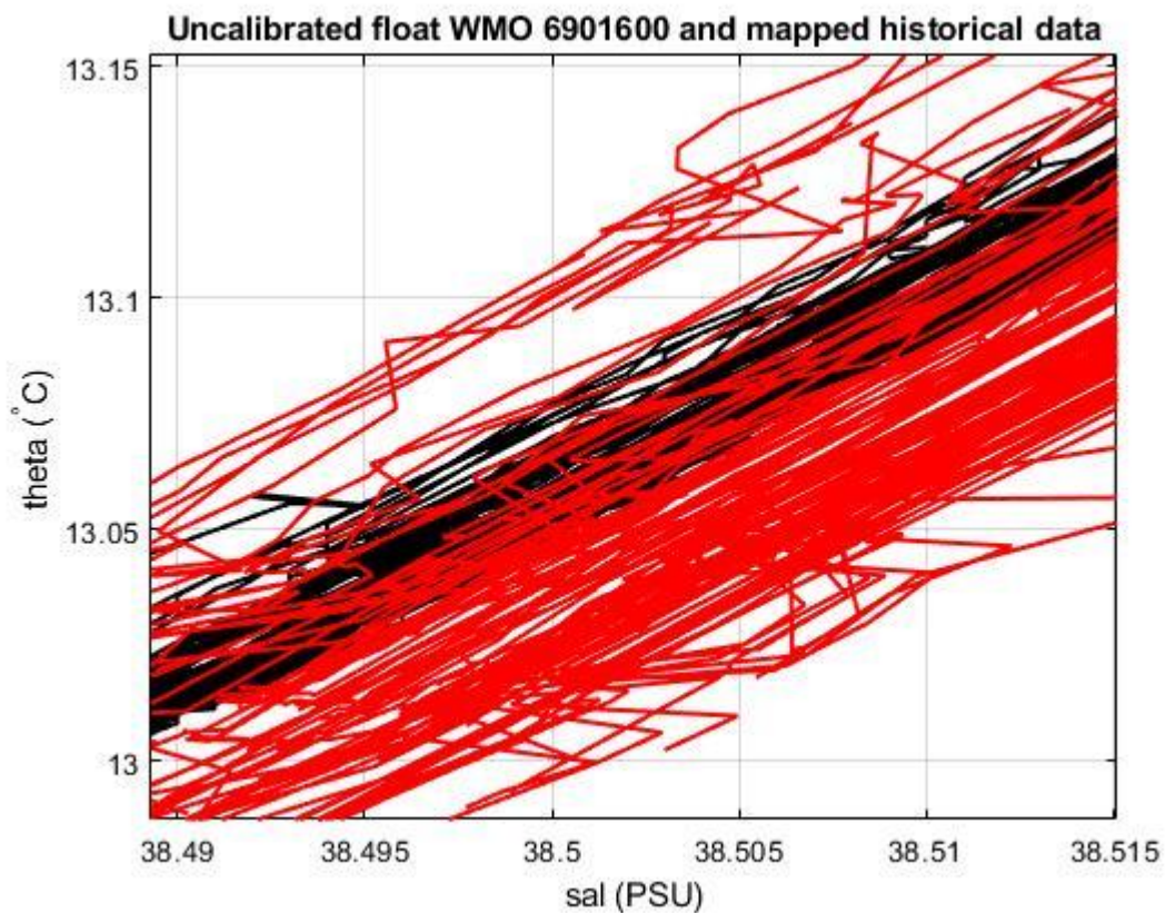
Figure 19: Float 6901600. Uncalibrated float salinity profile (black lines) and mapped historical data (red lines) in the most uniform part of the \theta -S curve.
