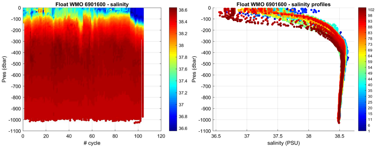
Figure 3: Float 6901600. Time series of Argo float potential salinity (PSS-78) on the left, and salinity profiles color-coded per cycle number on the right.
