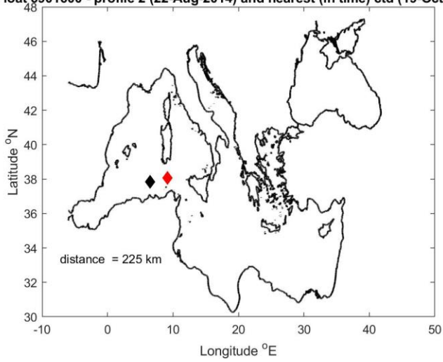
Figure 9: Float 6901600. The salinity float profile number 2 (black dots) are compared to the nearest in space (top) and in time (bottom) reference profile (red dots). The locations of the two profiles and their distance is given in the left panel.
