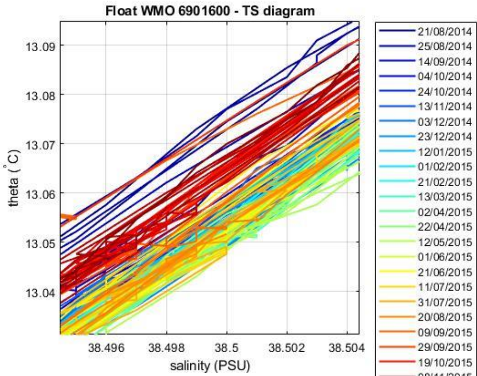
Figure 5: Float 6901600. Area of the \theta -S diagram (color-coded per cycle number) where the \theta -S relationship is more uniform.
