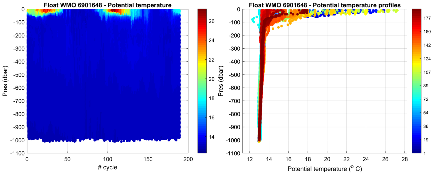
Figure 2: Float 6901648. Time series of Argo float potential temperature ( ^{\circ}\text{C} ) on the left, and potential temperature profiles color-coded per cycle number on the right.
