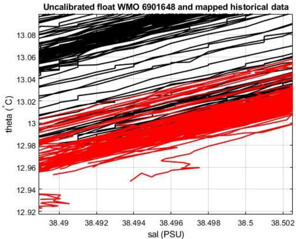
Figure 19: Float 6901648. Uncalibrated float salinity profile (black lines) and mapped historical data (red lines) in the most uniform part of the \theta -S curve.
