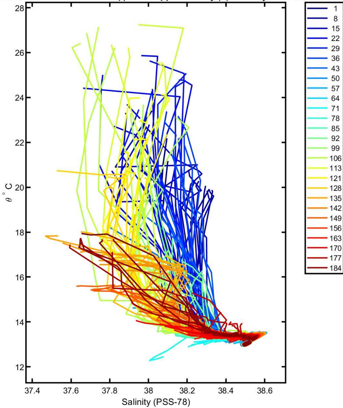
6901648 calibrated float data (-) and mapped salinity (o) with objective errors
