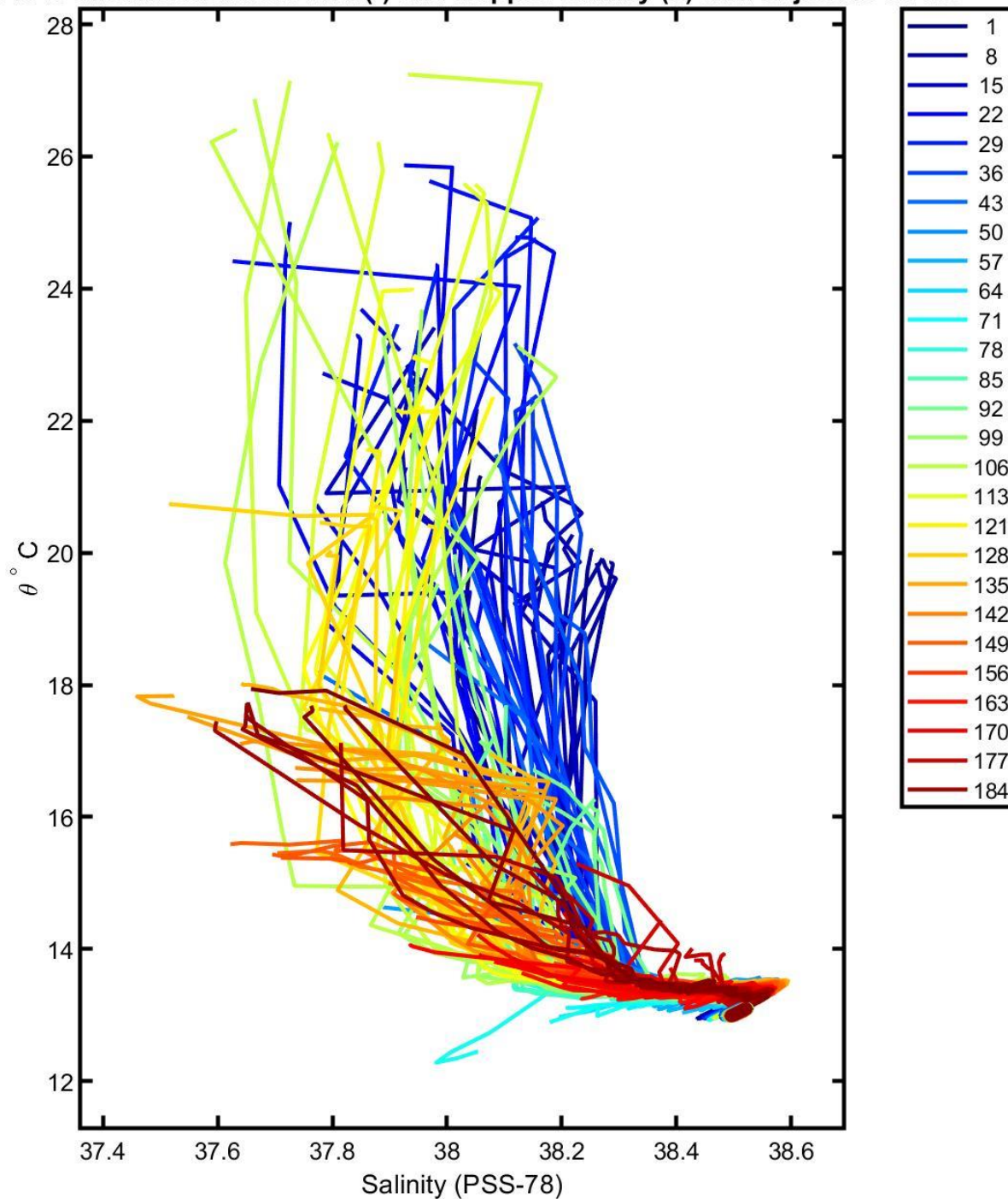
6901648 uncalibrated float data (-) and mapped salinity (o) with objective errors
