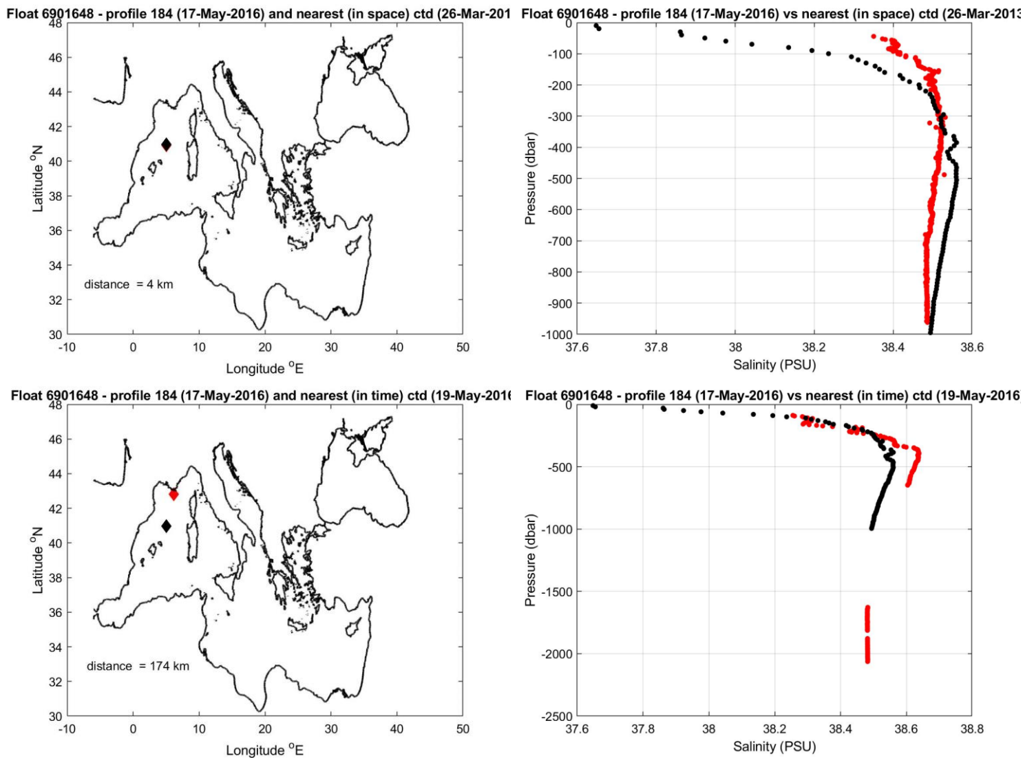
Figure 11: Float 6901648. The salinity float profile number 184 (black dots) are compared to the nearest in space (top) and in time (bottom) reference profile (red dots). The locations of the two profiles and their distance is given in the left panel.
