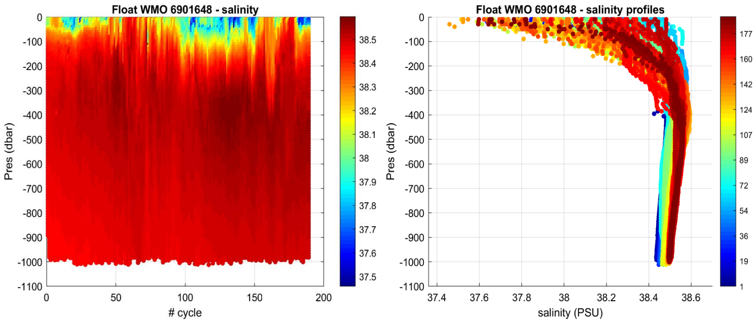
Figure 3: Float 6901648. Time series of Argo float potential salinity (PSS-78) on the left, and salinity profiles color-coded per cycle number on the right.
