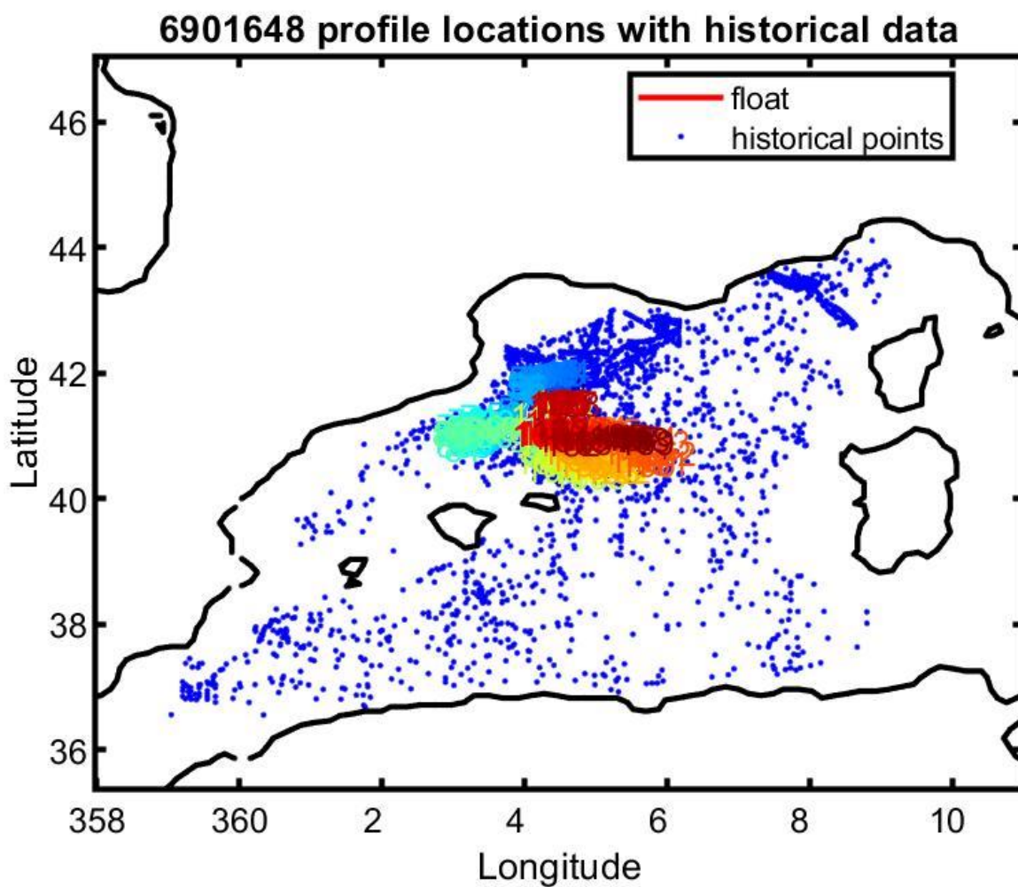
Figure 13: Float 6901648. Location of the float profiles (red line with colored numbers) and the reference data selected for mapping (blue dots).
