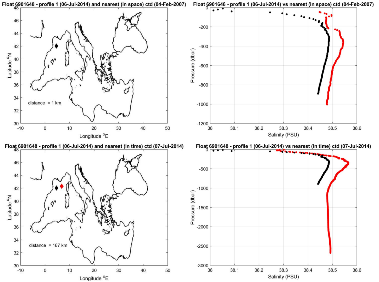
Figure 9: Float 6901648. The salinity float profile number 1 (black dots) are compared to the nearest in space (top) and in time (bottom) reference profile (red dots). The locations of the two profiles and their distance is given in the left panel.
