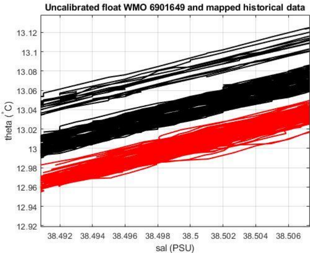
Figure 19: Float 6901649. Uncalibrated float salinity profile (black lines) and mapped historical data (red lines) in the most uniform part of the \theta -S curve.
