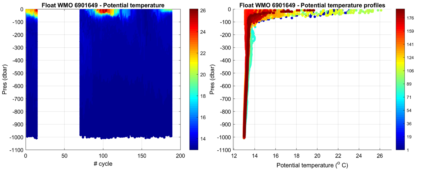
Figure 2: Float 6901649. Time series of Argo float potential temperature ( ^{\circ}\text{C} ) on the left, and potential temperature profiles color-coded per cycle number on the right.
