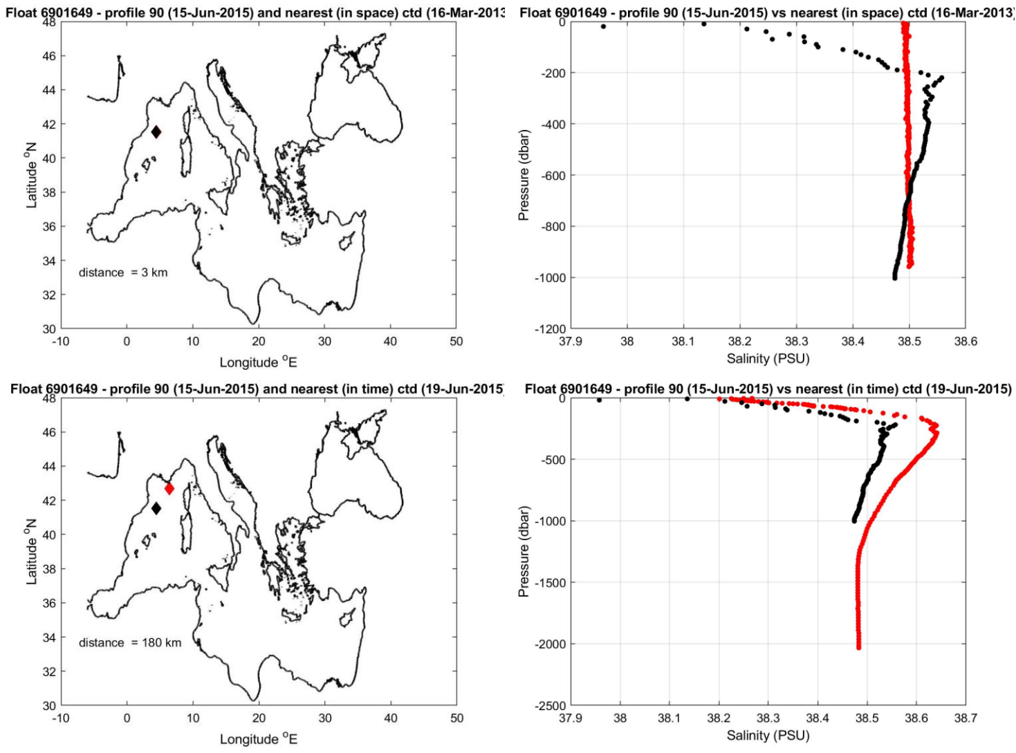
Figure 10: Float 6901649. The salinity float profile number 90 (black dots) are compared to the nearest in space (top) and in time (bottom) reference profile (red dots). The locations of the two profiles and their distance is given in the left panel.
