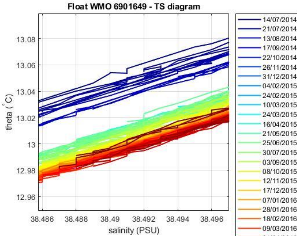
Figure 5: Float 6901649. Area of the \theta -S diagram (color-coded per cycle number) where the \theta -S relationship is more uniform.
