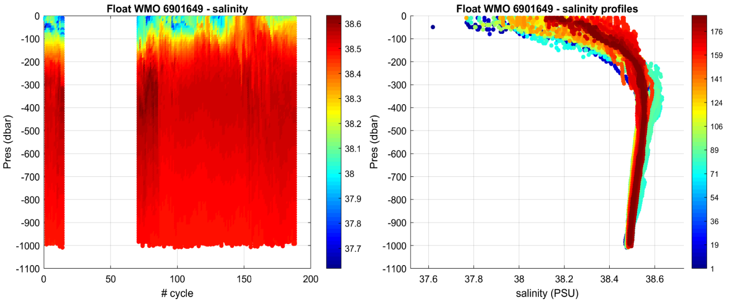
Figure 3: Float 6901649. Time series of Argo float potential salinity (PSS-78) on the left, and salinity profiles color-coded per cycle number on the right.
