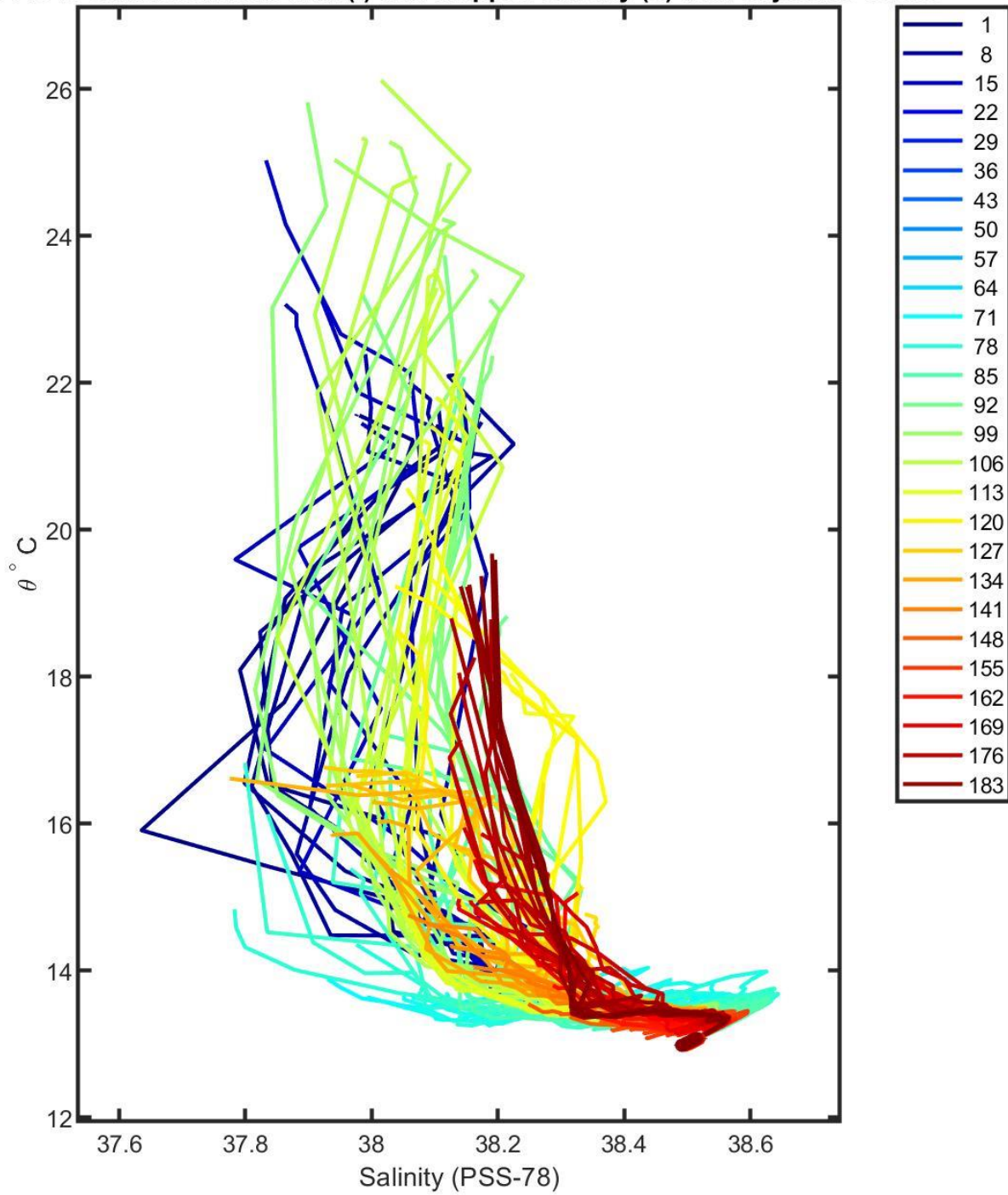
6901649 calibrated float data (-) and mapped salinity (o) with objective errors
