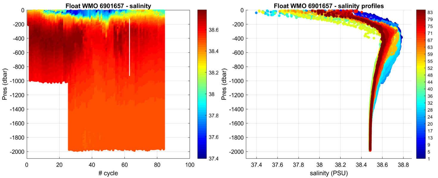
Figure 3: Float 6901657. Time series of Argo float potential salinity (PSS-78) on the left, and salinity profiles color-coded per cycle number on the right.
