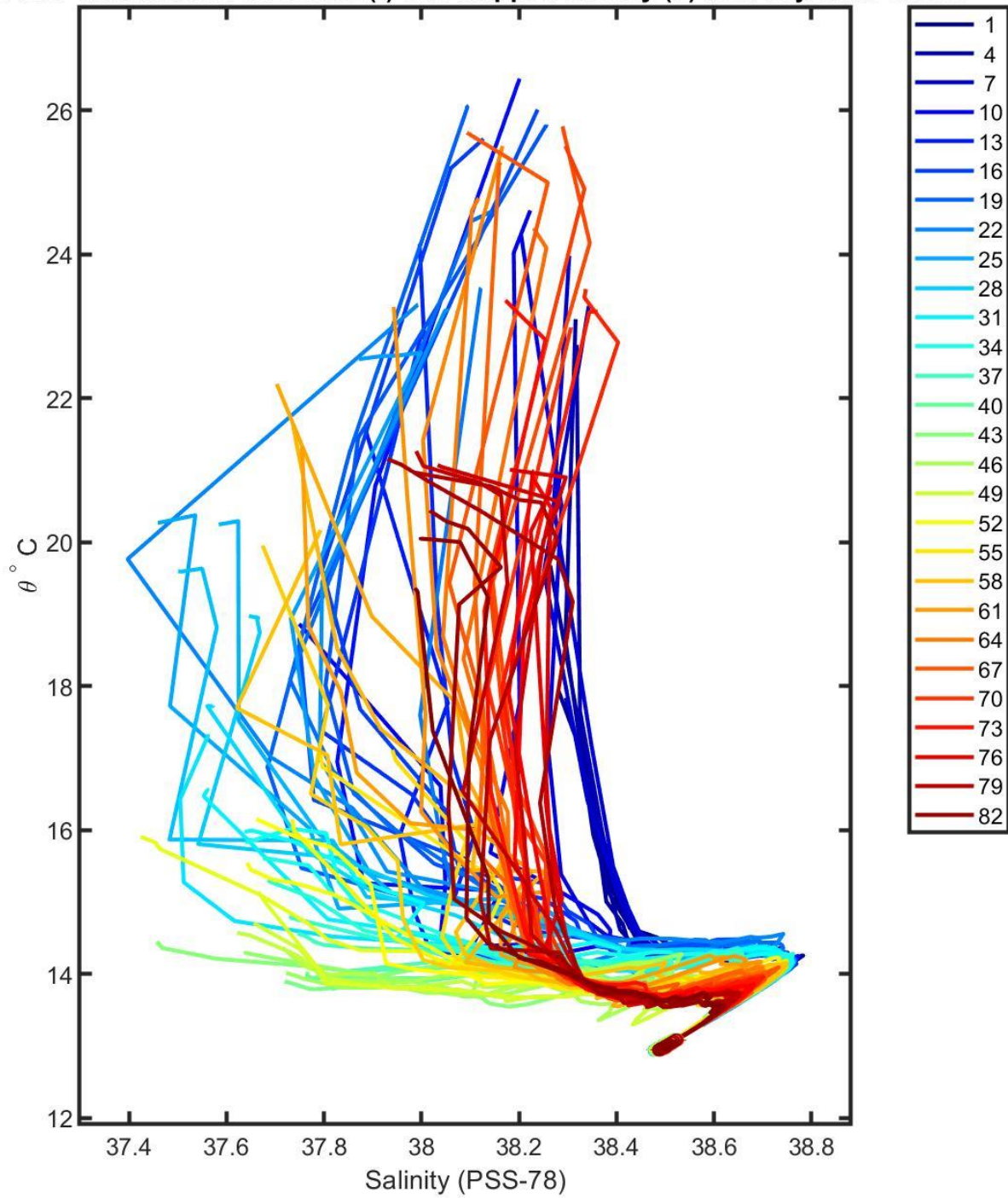
6901657 uncalibrated float data (-) and mapped salinity (o) with objective errors
