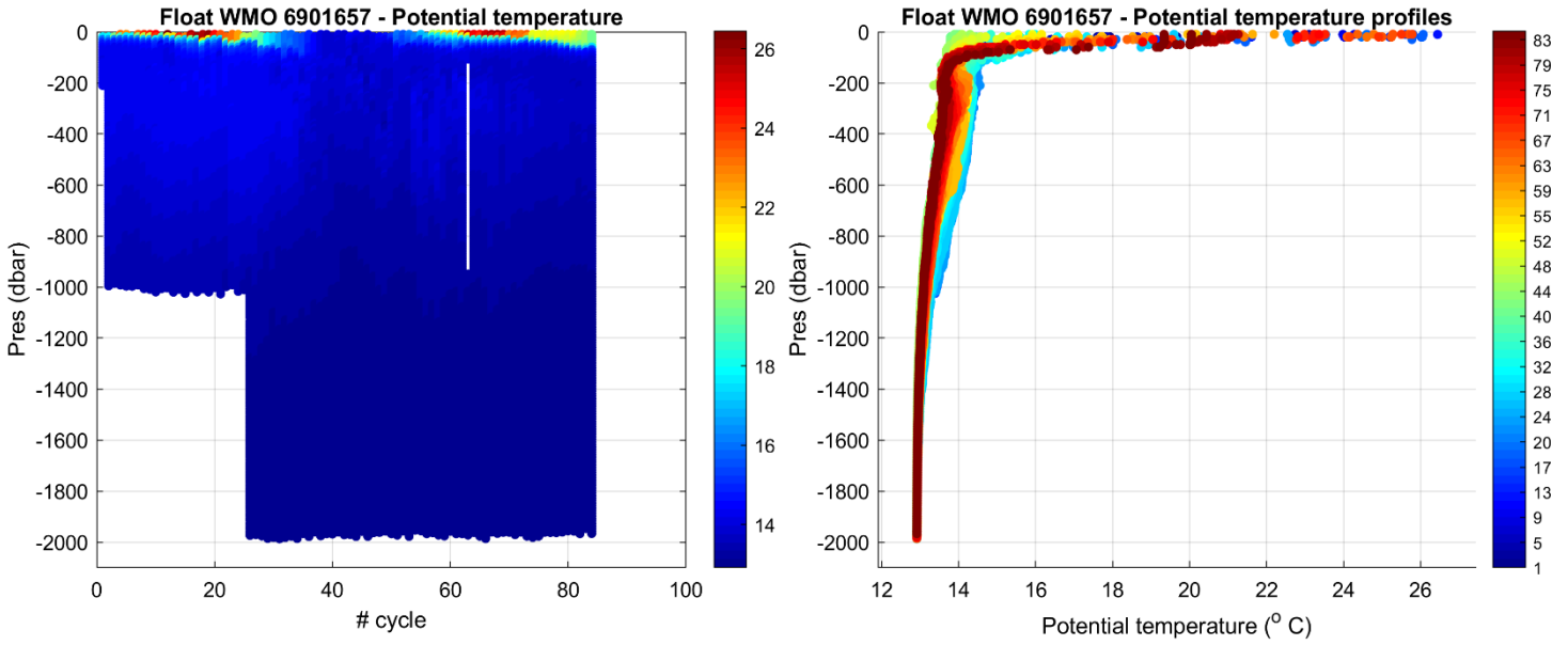
Figure 2: Float 6901657. Time series of Argo float potential temperature ( ^{\circ}\text{C} ) on the left, and potential temperature profiles color-coded per cycle number on the right.
