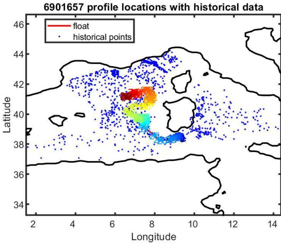
Figure 13: Float 6901657. Location of the float profiles (red line with colored numbers) and the reference data selected for mapping (blue dots).
