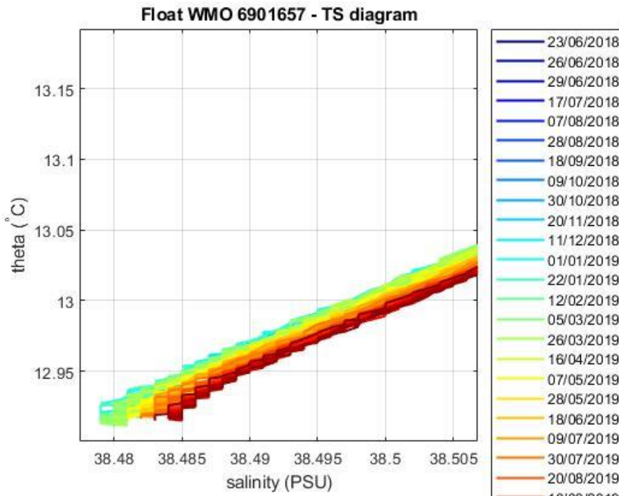
Figure 5: Float 6901657. Area of the \theta -S diagram (color-coded per cycle number) where the \theta -S relationship is more uniform.
