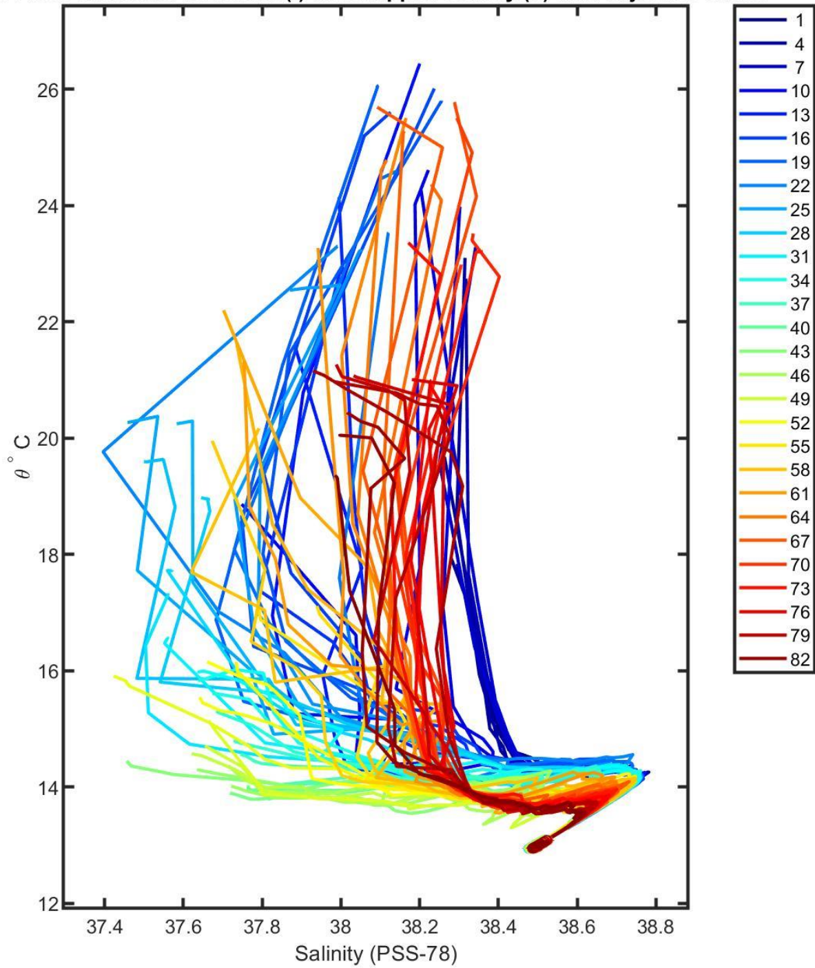
6901657 calibrated float data (-) and mapped salinity (o) with objective errors
