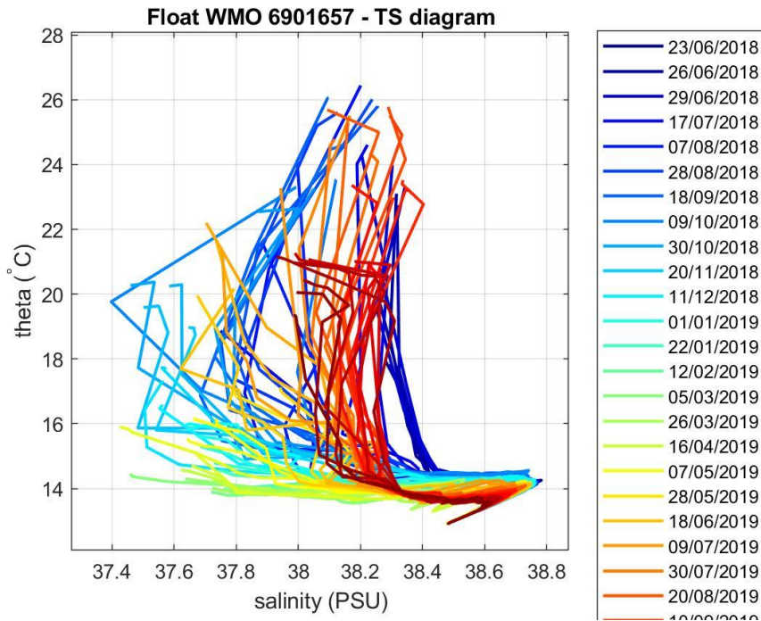
Figure 4: Float 6901657. \theta -S diagram color-coded per cycle number.
