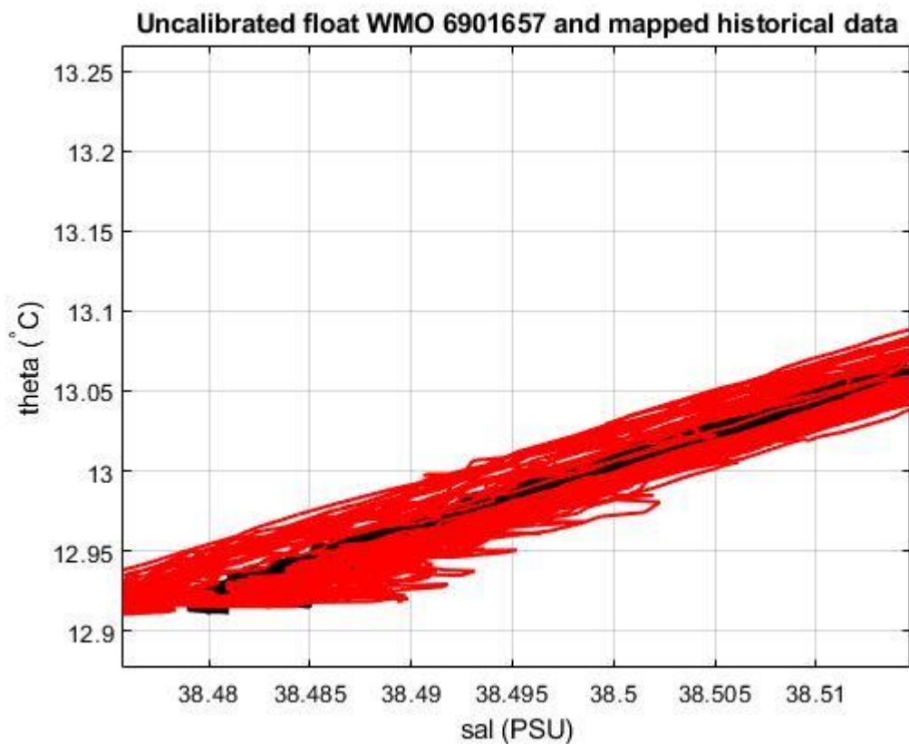
Figure 19: Float 6901657. Uncalibrated float salinity profile (black lines) and mapped historical data (red lines) in the most uniform part of the \theta -S curve.
