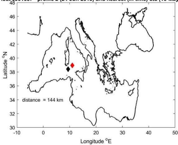
Float 6901657 - profile 2 (24-Jun-2018) and nearest (in time) ctd (16-May-2017)
