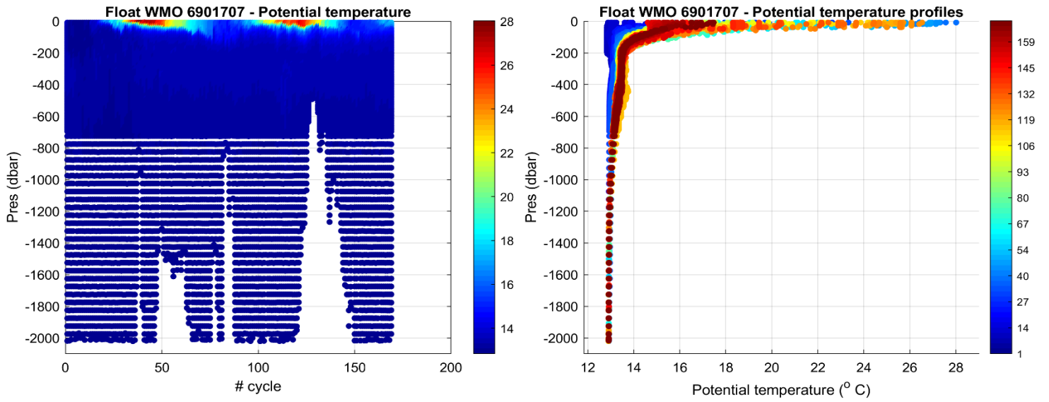
Figure 2: Float 6901707. Time series of Argo float potential temperature ( ^{\circ}\text{C} ) on the left, and potential temperature profiles color-coded per cycle number on the right.
