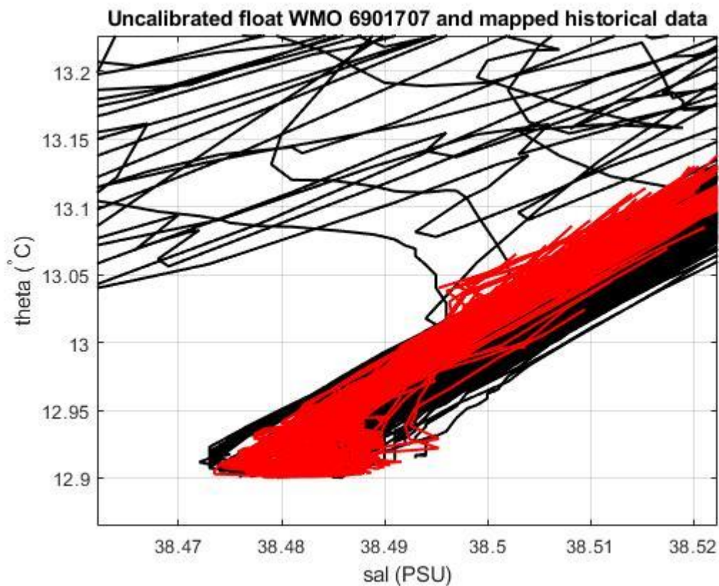
Figure 19: Float 6901707. Uncalibrated float salinity profile (black lines) and mapped historical data (red lines) in the most uniform part of the \theta -S curve.
