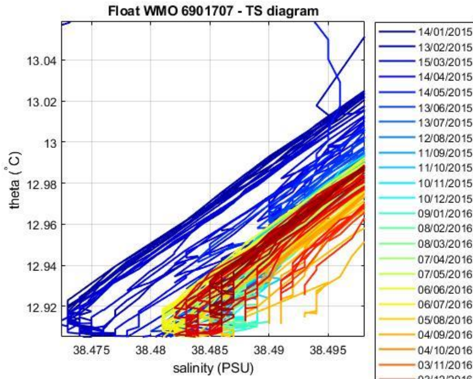
Figure 5: Float 6901707. Area of the \theta -S diagram (color-coded per cycle number) where the \theta -S relationship is more uniform.
