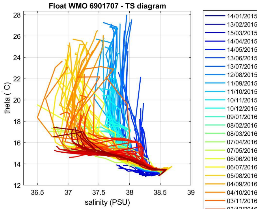
Figure 4: Float 6901707. \theta -S diagram color-coded per cycle number.
