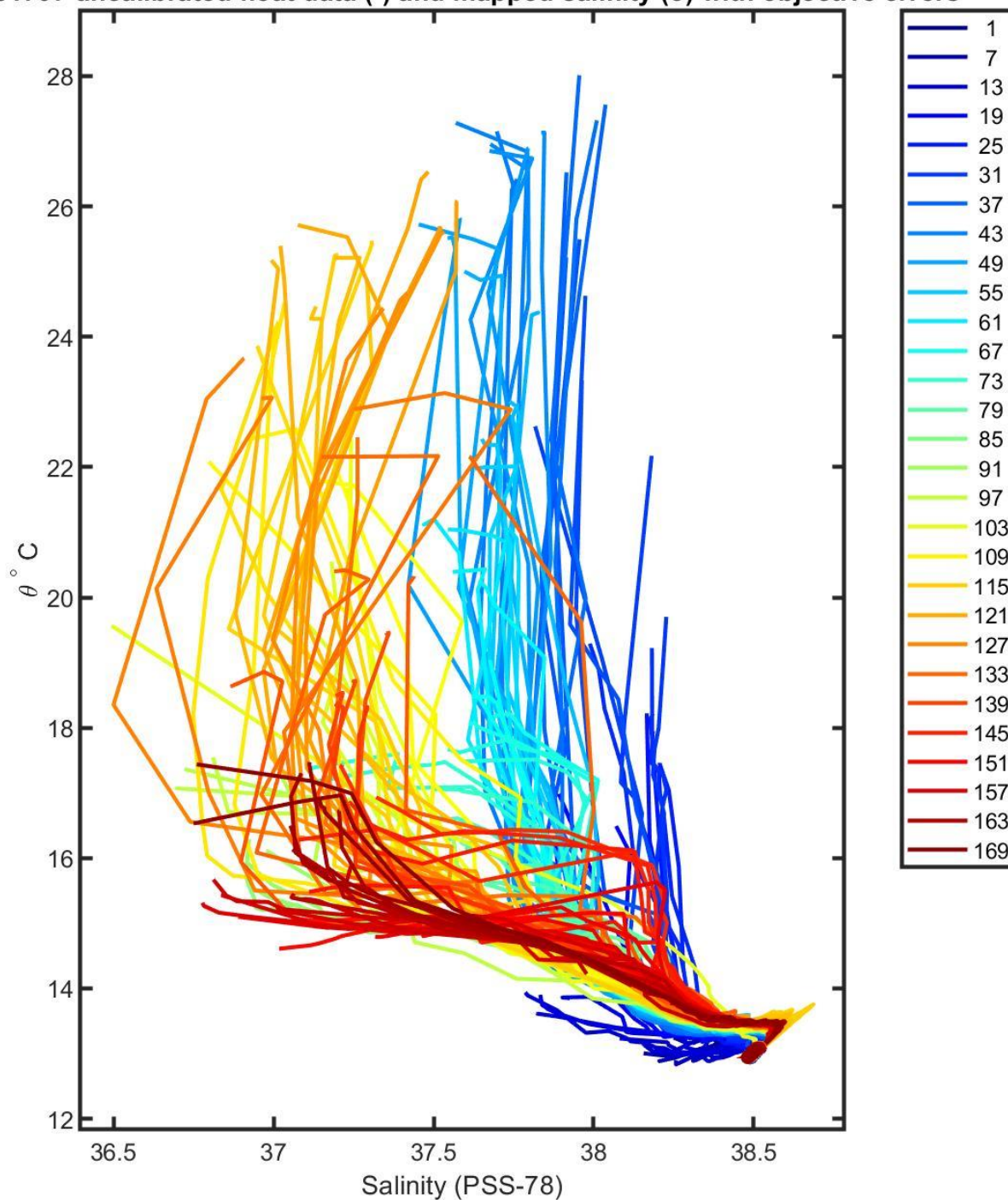
6901707 uncalibrated float data (-) and mapped salinity (o) with objective errors
