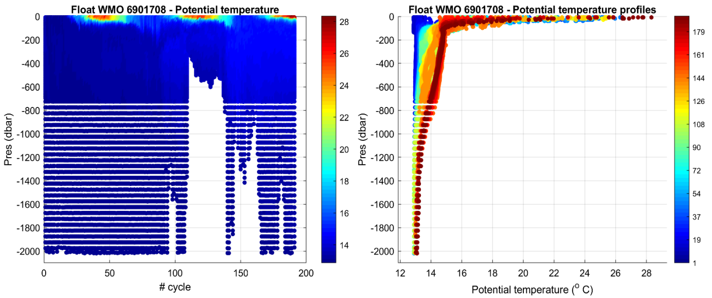
Figure 2: Float 6901708. Time series of Argo float potential temperature ( ^{\circ}\text{C} ) on the left, and potential temperature profiles color-coded per cycle number on the right.
