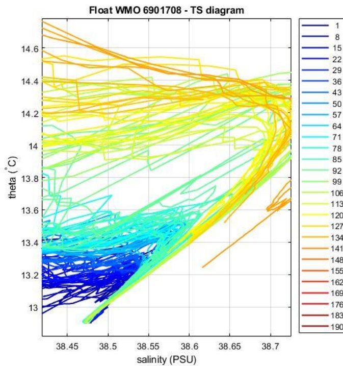
Figure 20: Float 6901708. \theta -S diagram color-coded per cycle number.
