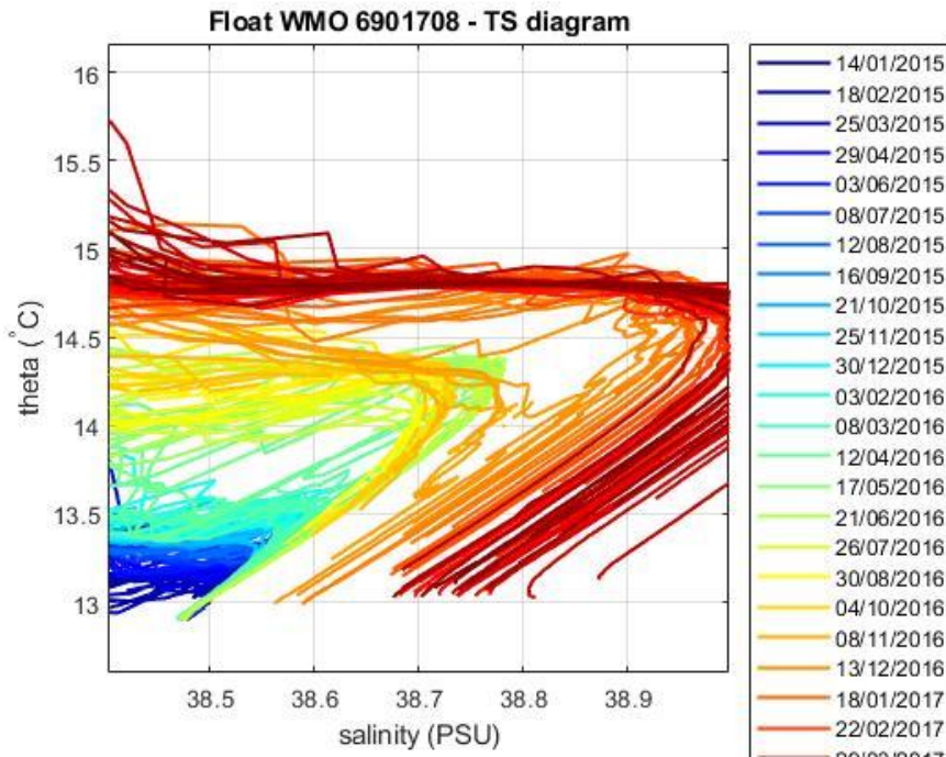
Figure 5: Float 6901708. Area of the \theta -S diagram (color-coded per cycle number) where the \theta -S relationship is more uniform.
