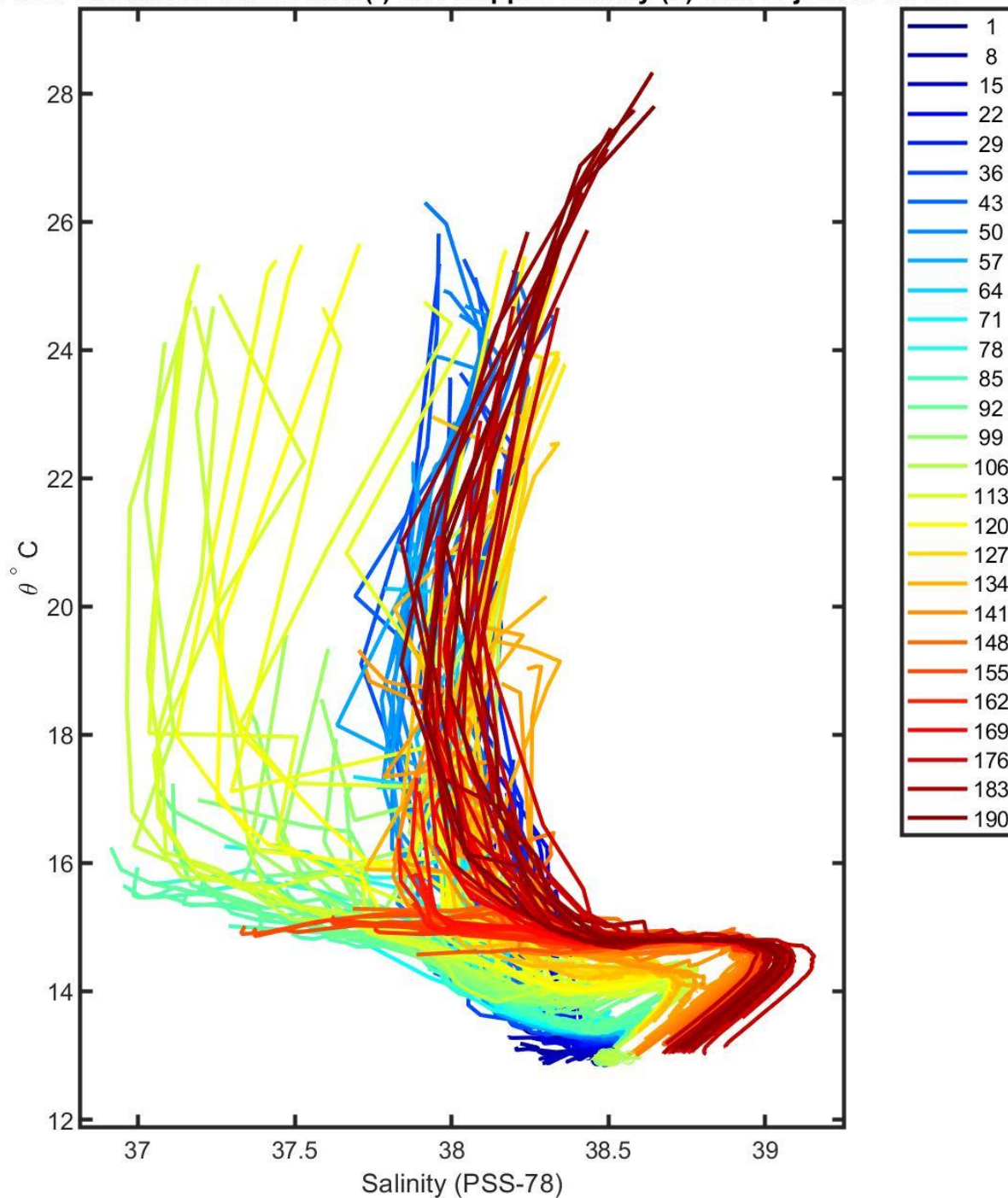
6901708 uncalibrated float data (-) and mapped salinity (o) with objective errors
