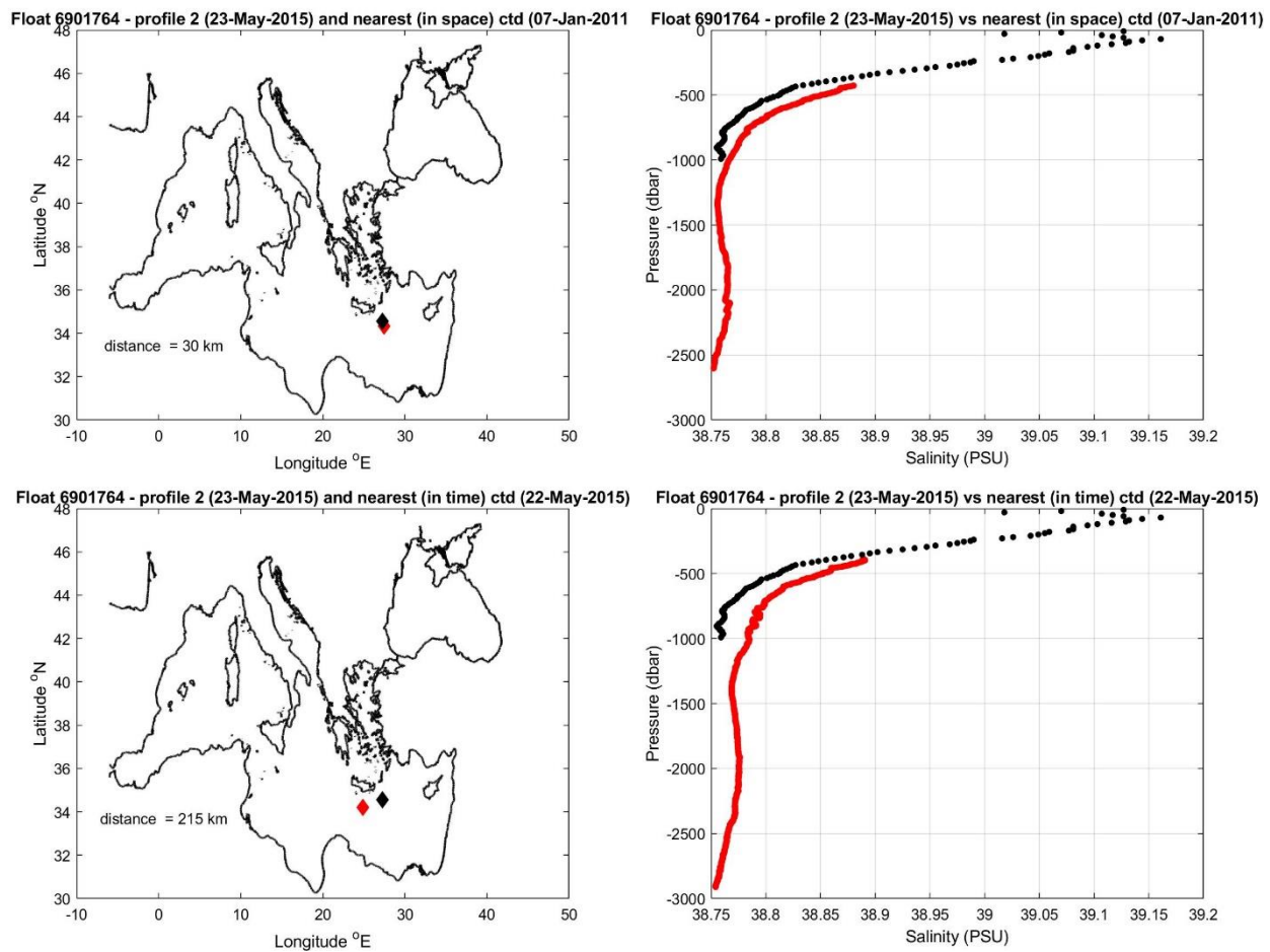
Figure 9: Float 6901764. The salinity float profile number 2 (black dots) are compared to the nearest in space (top) and in time (bottom) reference profile (red dots). The locations of the two profiles and their distance is given in the left panel.
