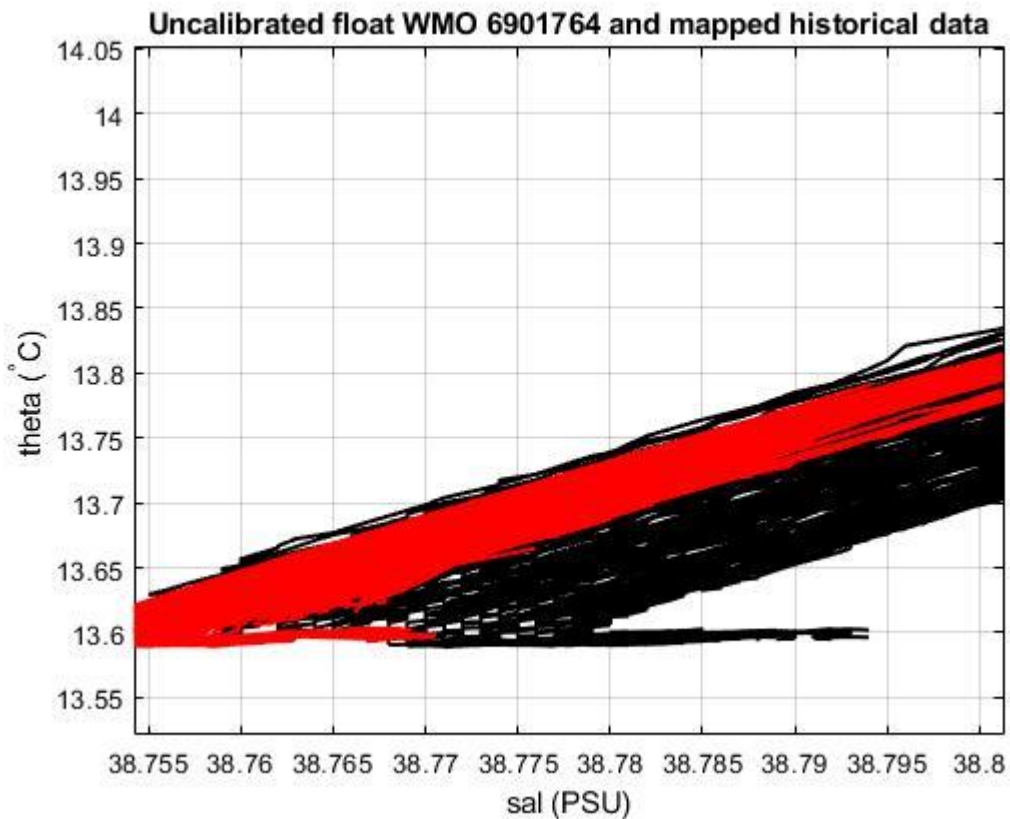
Figure 19: Float 6901764. Uncalibrated float salinity profile (black lines) and mapped historical data (red lines) in the most uniform part of the \theta -S curve.
