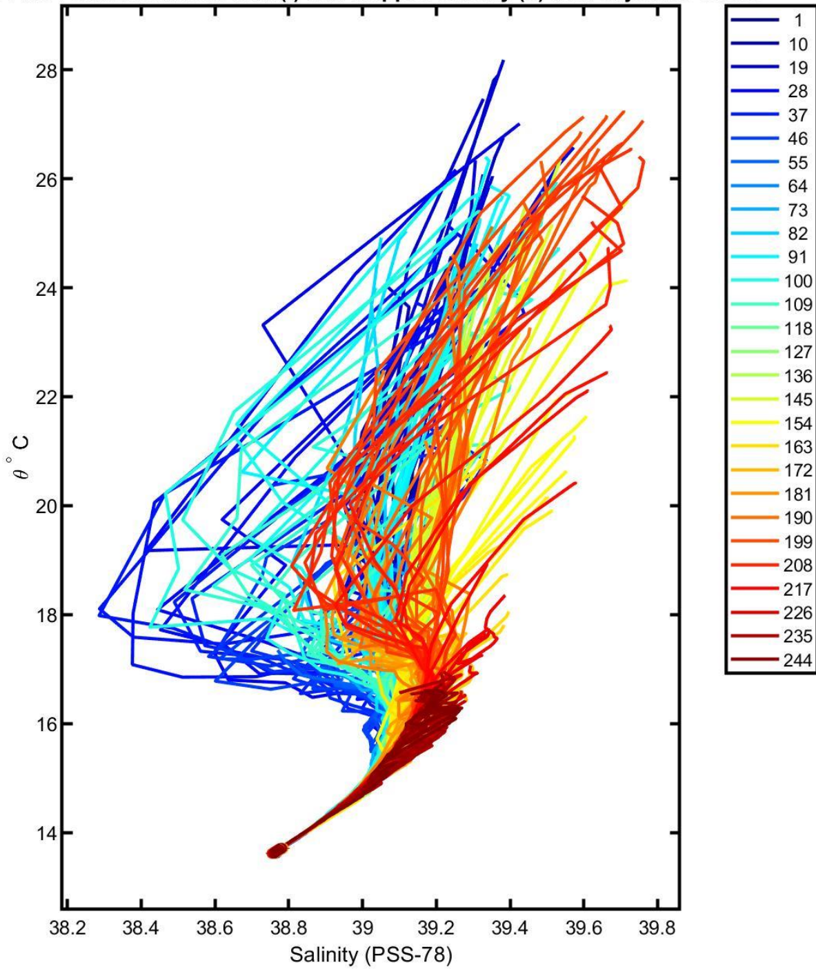
6901764 calibrated float data (-) and mapped salinity (o) with objective errors
