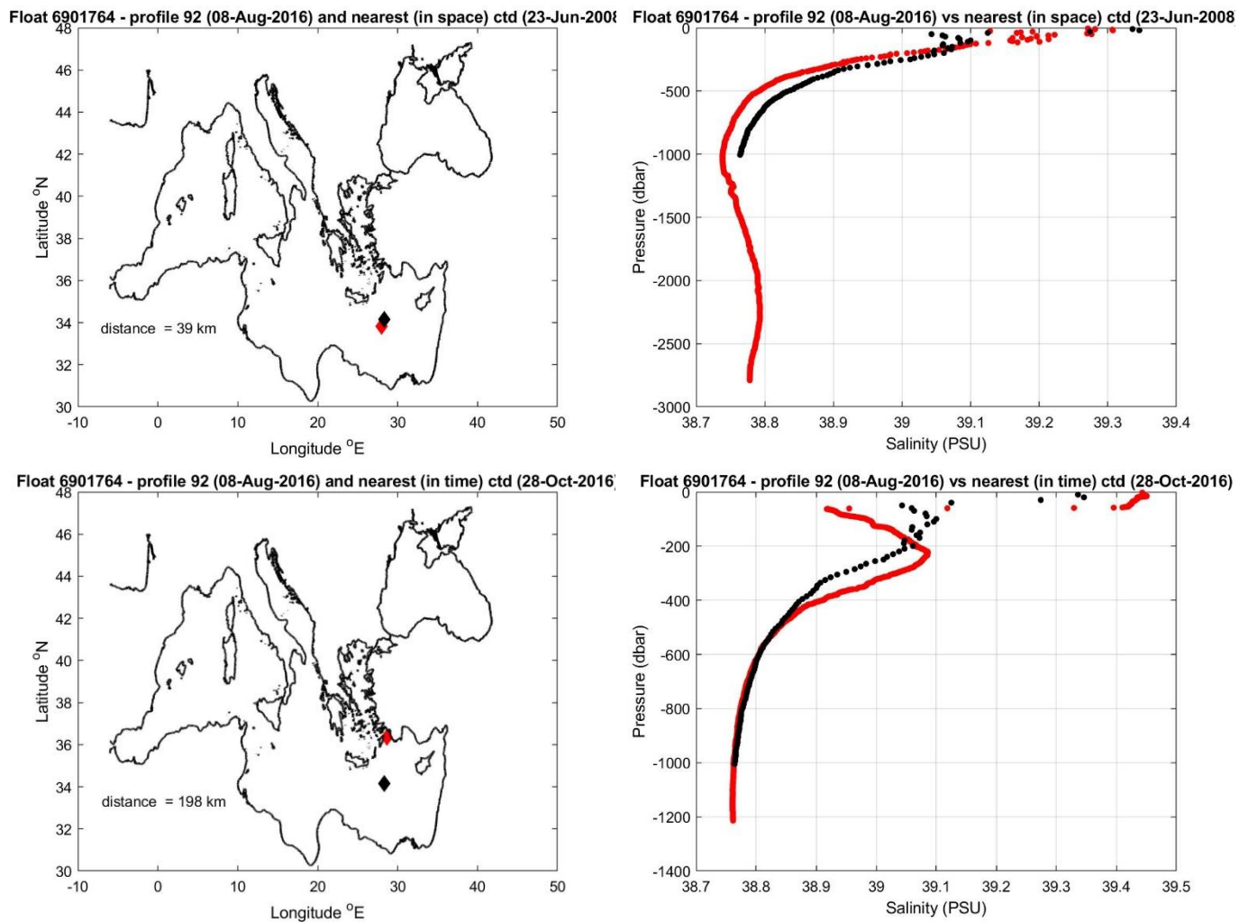
Figure 10: Float 6901764. The salinity float profile number 92 (black dots) are compared to the nearest in space (top) and in time (bottom) reference profile (red dots). The locations of the two profiles and their distance is given in the left panel.
