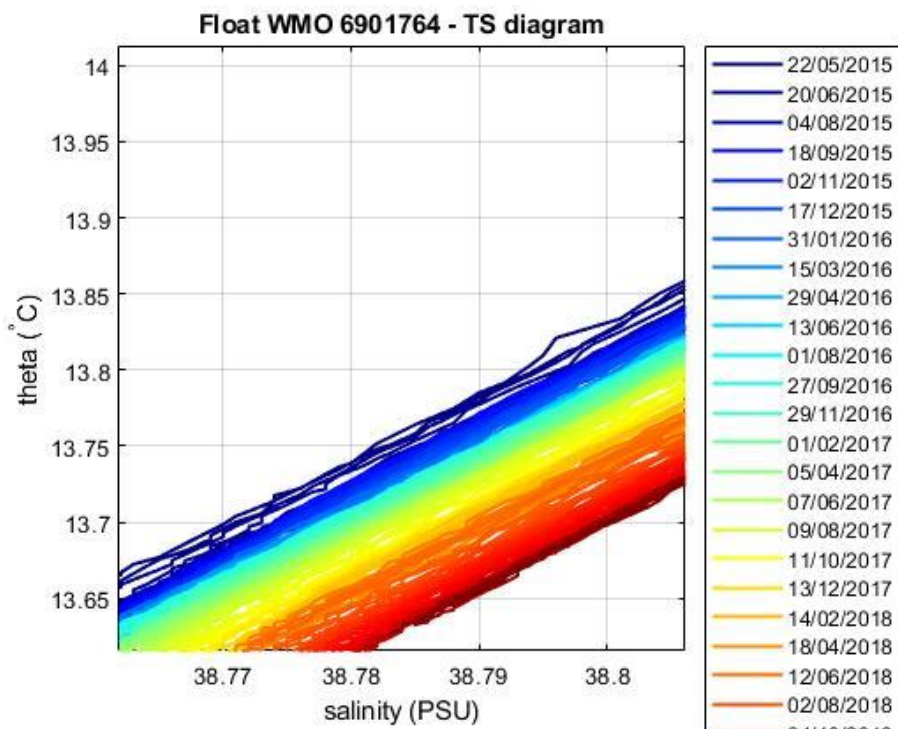
Figure 5: Float 6901764. Area of the \theta -S diagram (color-coded per cycle number) where the \theta -S relationship is more uniform.
