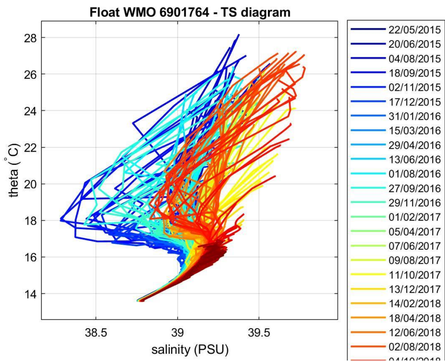
Figure 4: Float 6901764. \theta -S diagram color-coded per cycle number.
