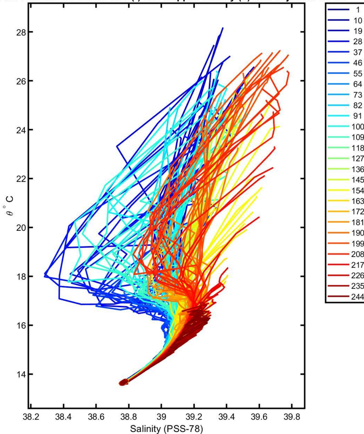
6901764 uncalibrated float data (-) and mapped salinity (o) with objective errors
