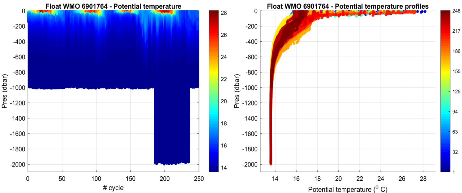
Figure 2: Float 6901764. Time series of Argo float potential temperature ( ^{\circ}\text{C} ) on the left, and potential temperature profiles color-coded per cycle number on the right.
