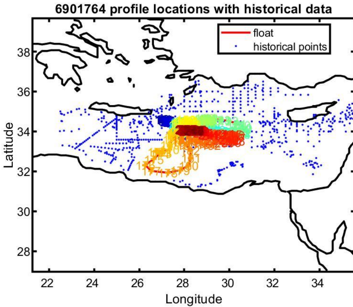
Figure 13: Float 6901764. Location of the float profiles (red line with colored numbers) and the reference data selected for mapping (blue dots).
