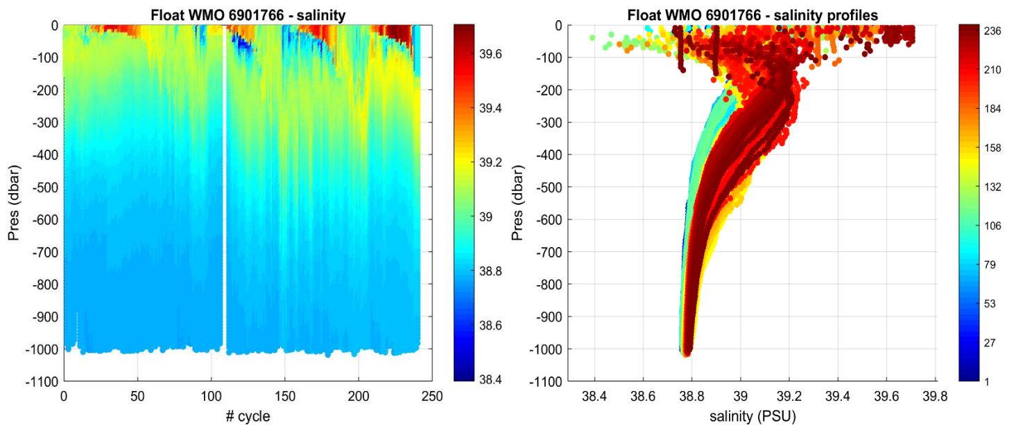
Figure 3: Float 6901766. Time series of Argo float potential salinity (PSS-78) on the left, and salinity profiles color-coded per cycle number on the right.
