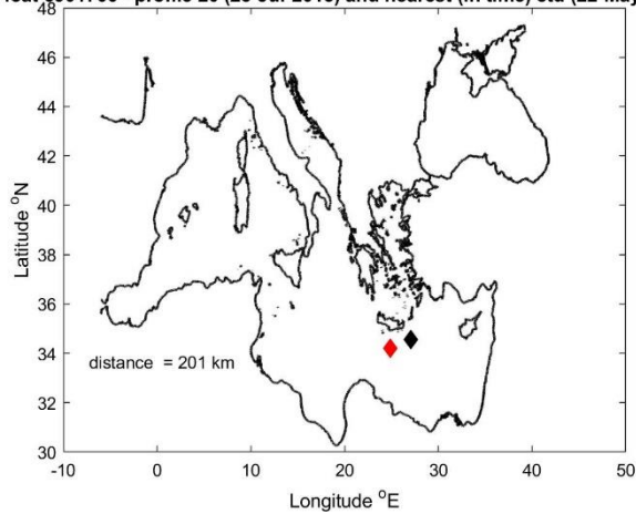
Figure 9: Float 6901766. The salinity float profile number 20 (black dots) are compared to the nearest in space (top) and in time (bottom) reference profile (red dots). The locations of the two profiles and their distance is given in the left panel.
