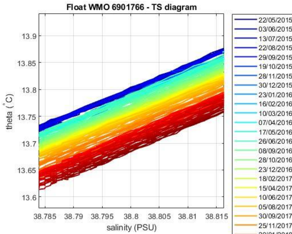
Figure 5: Float 6901766. Area of the \theta -S diagram (color-coded per cycle number) where the \theta -S relationship is more uniform.
