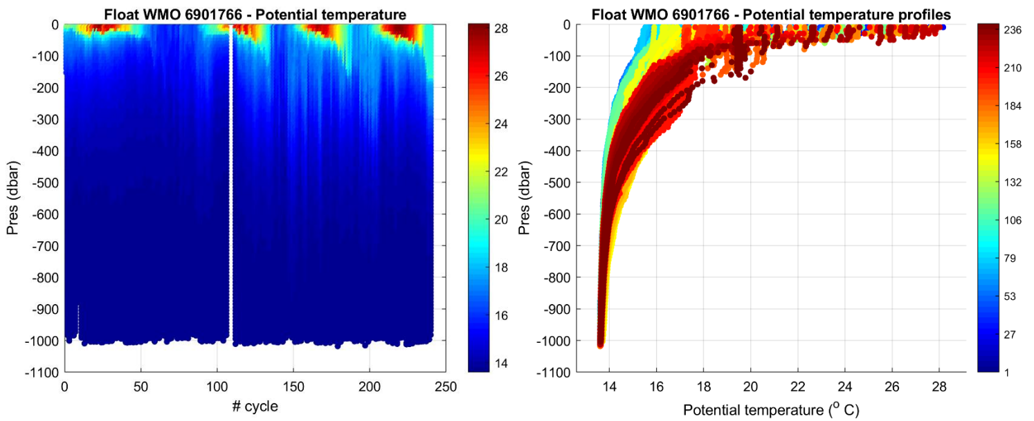
Figure 2: Float 6901766. Time series of Argo float potential temperature ( ^{\circ}\text{C} ) on the left, and potential temperature profiles color-coded per cycle number on the right.
