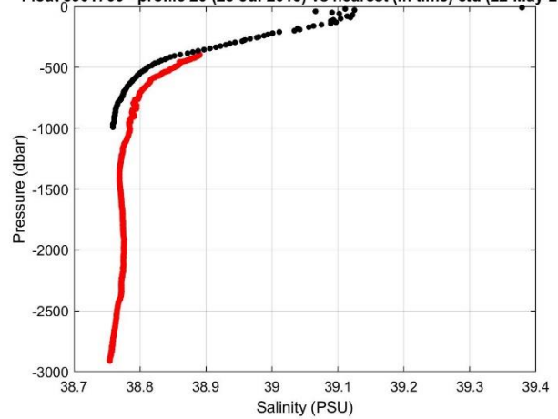
Figure 9: Float 6901766. The salinity float profile number 20 (black dots) are compared to the nearest in space (top) and in time (bottom) reference profile (red dots). The locations of the two profiles and their distance is given in the left panel.
