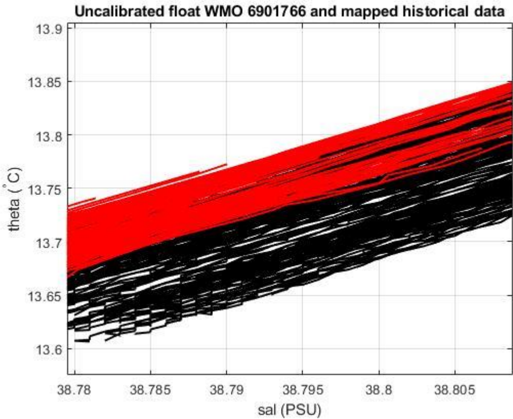
Figure 19: Float 6901766. Uncalibrated float salinity profile (black lines) and mapped historical data (red lines) in the most uniform part of the \theta -S curve.
