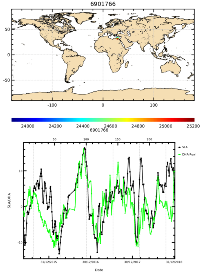
Figure 1: Float 6901766. The comparison between the sea surface height (SSH) from the satellite altimetry and dynamic height anomaly (DHA) extracted from the Argo float temperature and salinity. The figure is created by the CLS/Coriolis and distributed by Ifremer ( http://ftp.ifremer.fr/ifremer/argo/etc/argo-ast9-item13-AltimeterComparison/figures/ ).
