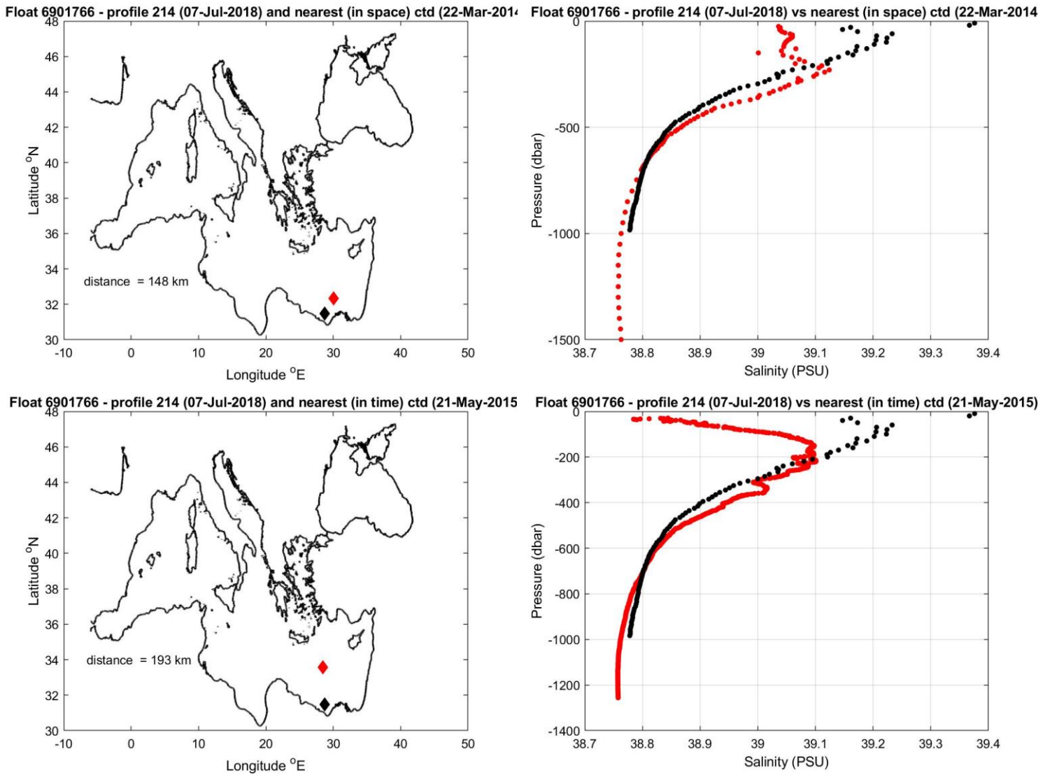
Figure 11: Float 6901766. The salinity float profile number 214 (black dots) are compared to the nearest in space (top) and in time (bottom) reference profile (red dots). The locations of the two profiles and their distance is given in the left panel.
