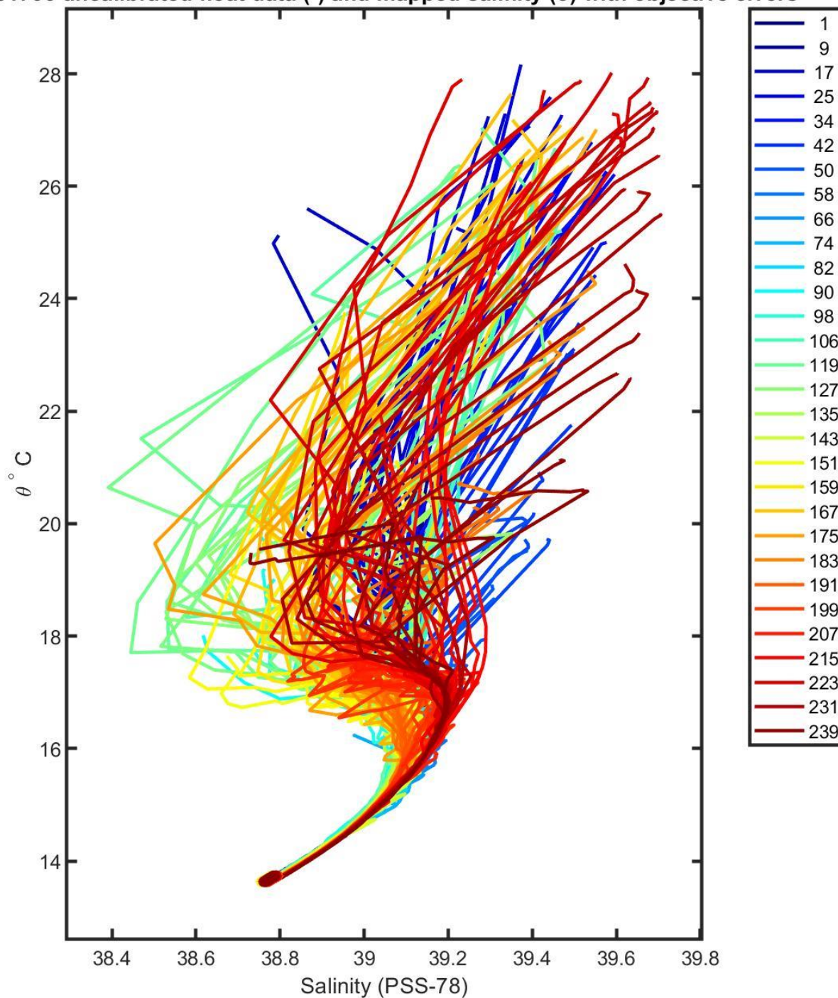
6901766 uncalibrated float data (-) and mapped salinity (o) with objective errors
