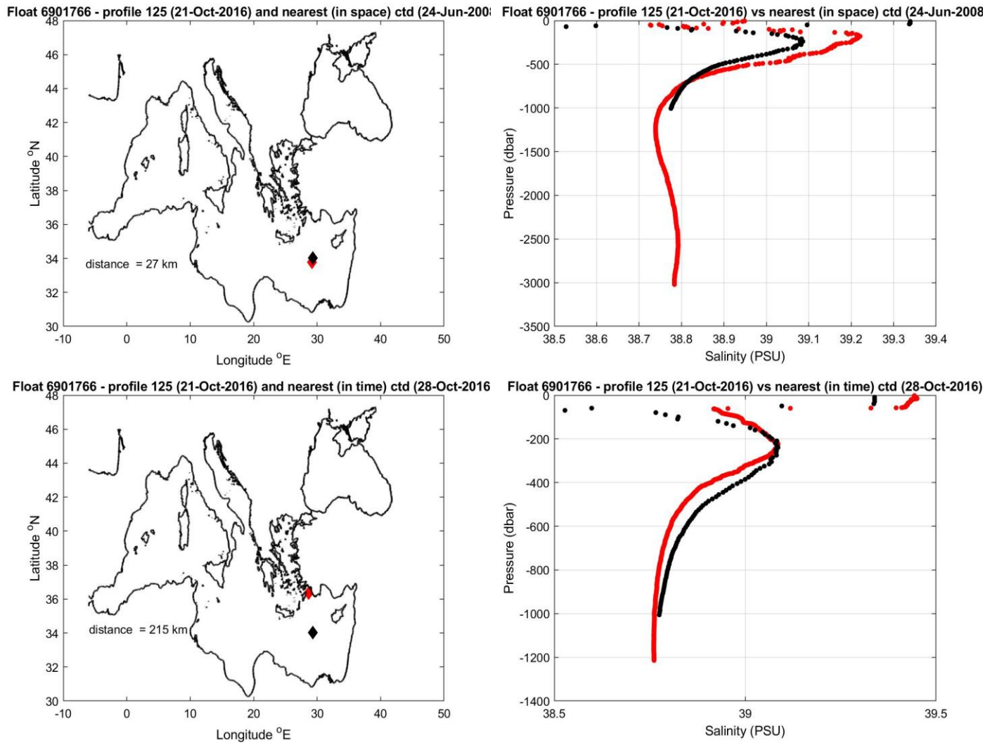
Figure 10: Float 6901766. The salinity float profile number 125 (black dots) are compared to the nearest in space (top) and in time (bottom) reference profile (red dots). The locations of the two profiles and their distance is given in the left panel.
