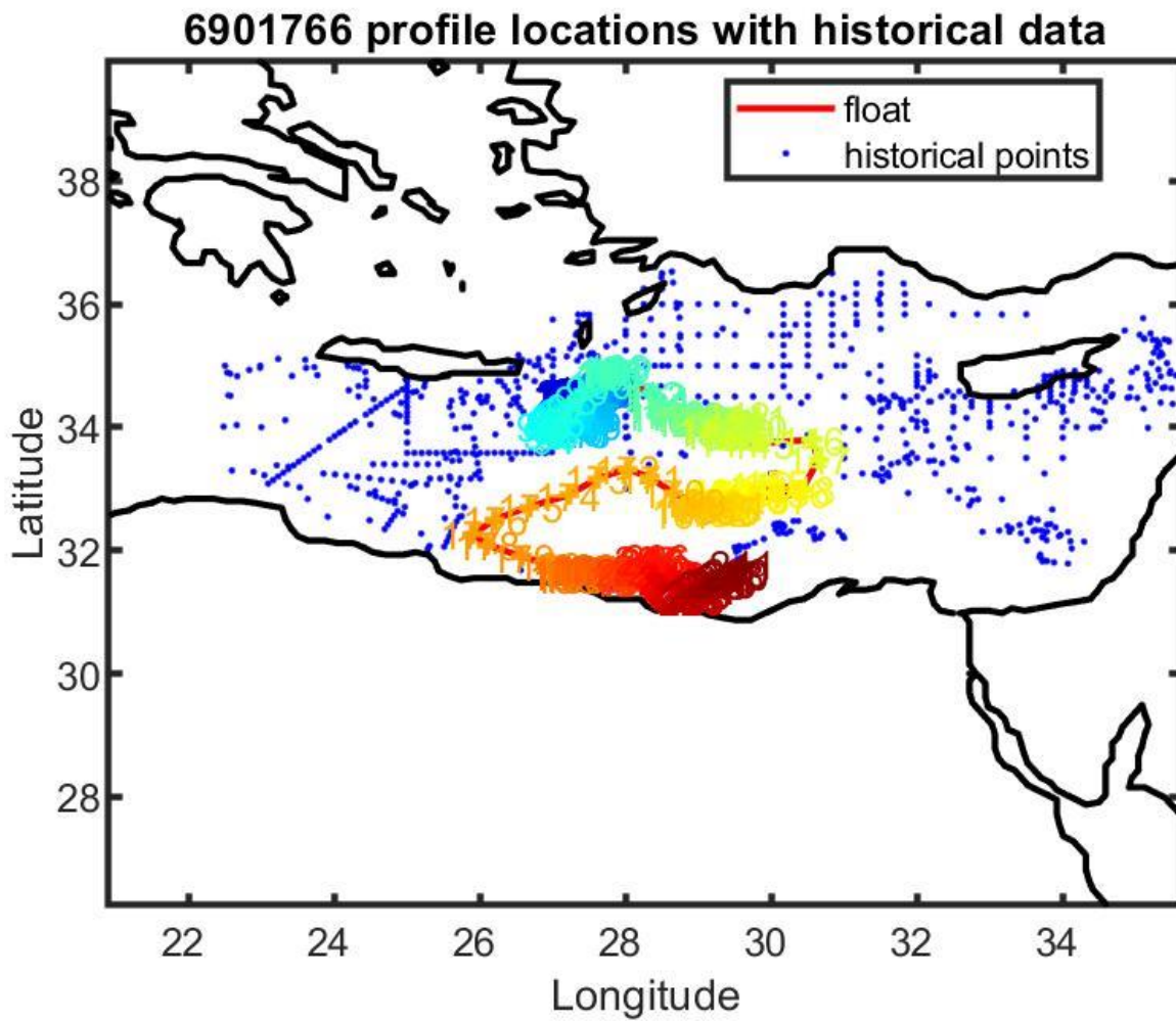
Figure 13: Float 6901766. Location of the float profiles (red line with colored numbers) and the reference data selected for mapping (blue dots).
