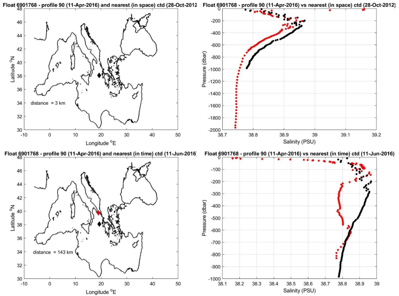
Figure 10: Float 6901768. The salinity float profile number 90 (black dots) are compared to the nearest in space (top) and in time (bottom) reference profile (red dots). The locations of the two profiles and their distance is given in the left panel.
