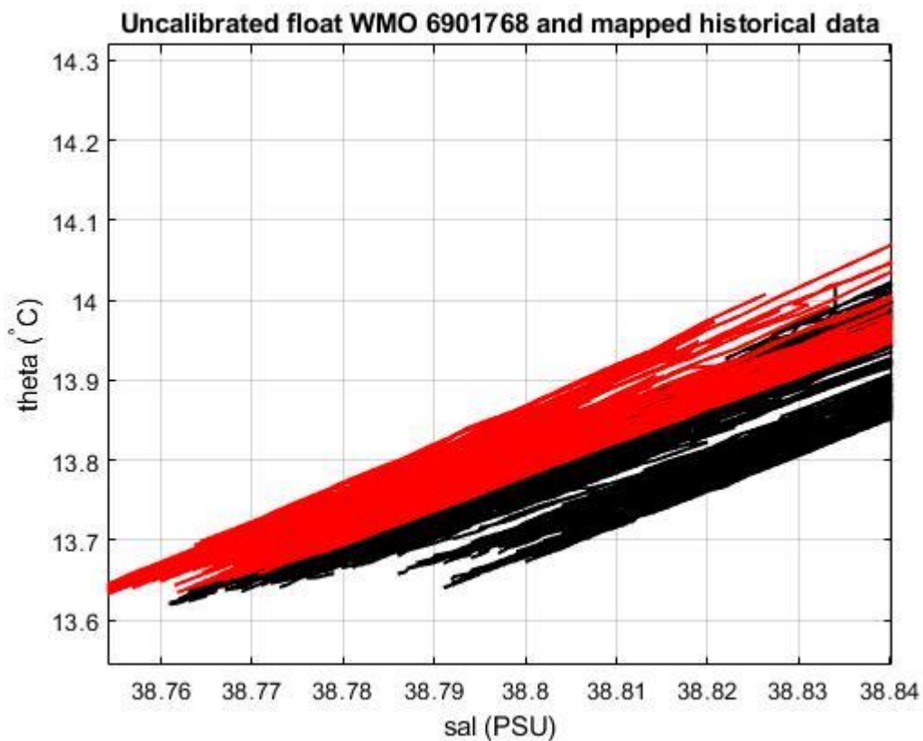
Figure 19: Float 6901768. Uncalibrated float salinity profile (black lines) and mapped historical data (red lines) in the most uniform part of the \theta -S curve.
