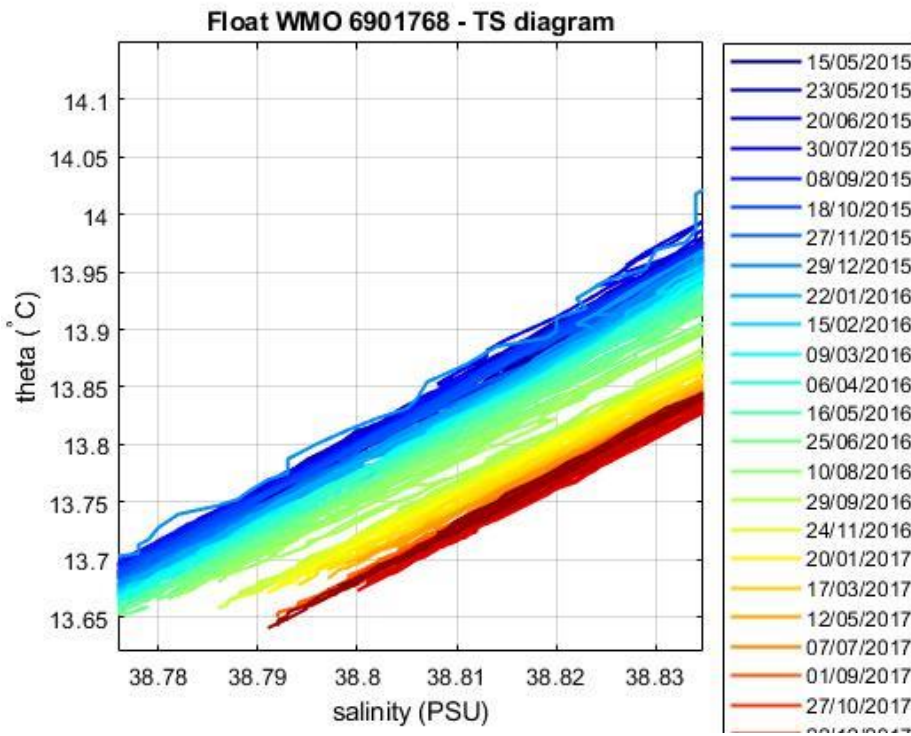
Figure 5: Float 6901768. Area of the \theta -S diagram (color-coded per cycle number) where the \theta -S relationship is more uniform.
