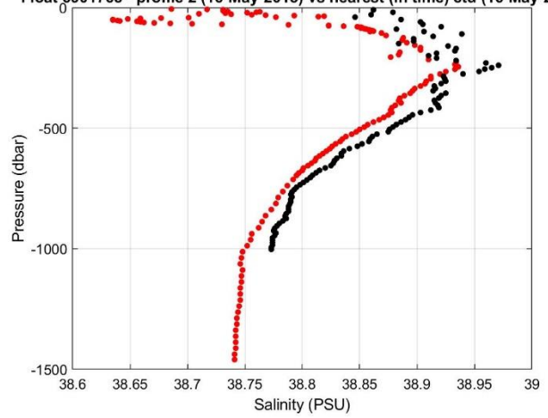
Float 6901768 - profile 2 (16-May-2015) vs nearest (in time) ctd (16-May-2015)
