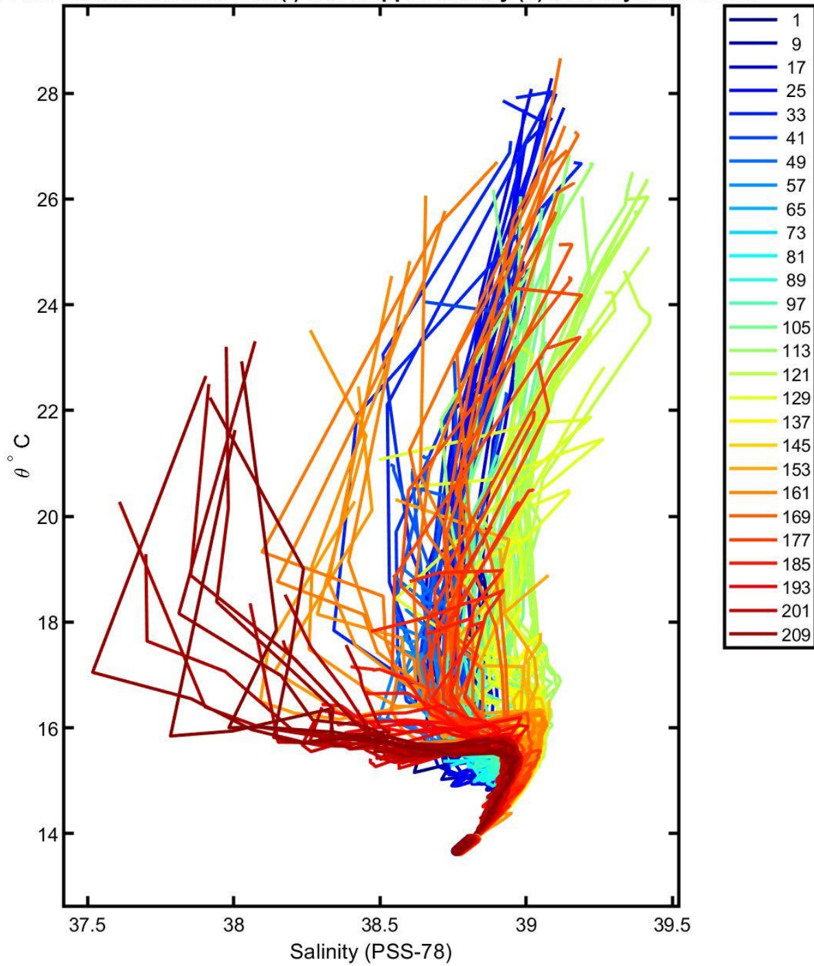
6901768 calibrated float data (-) and mapped salinity (o) with objective errors
