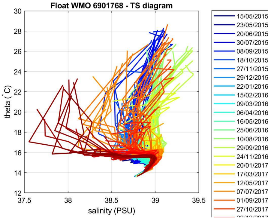
Figure 4: Float 6901768. \theta -S diagram color-coded per cycle number.
