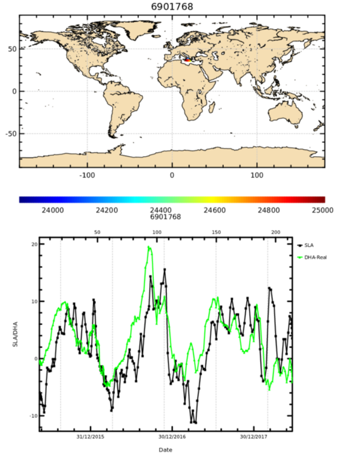
Figure 1: Float 6901768. The comparison between the sea surface height (SSH) from the satellite altimetry and dynamic height anomaly (DHA) extracted from the Argo float temperature and salinity. The figure is created by the CLS/Coriolis and distributed by Ifremer ( ftp://ftp.ifremer.fr/ifremer/argo/etc/argo-ast9-item13-AltimeterComparison/figures/ ).
