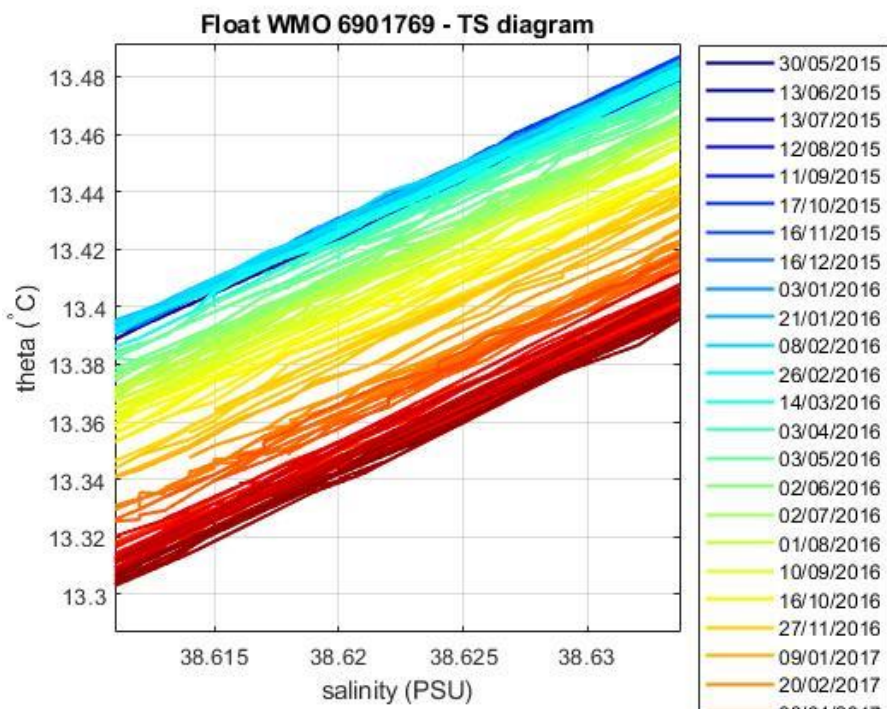
Figure 5: Float 6901769 Area of the \theta -S diagram (color-coded per cycle number) where the \theta -S relationship is more uniform.
