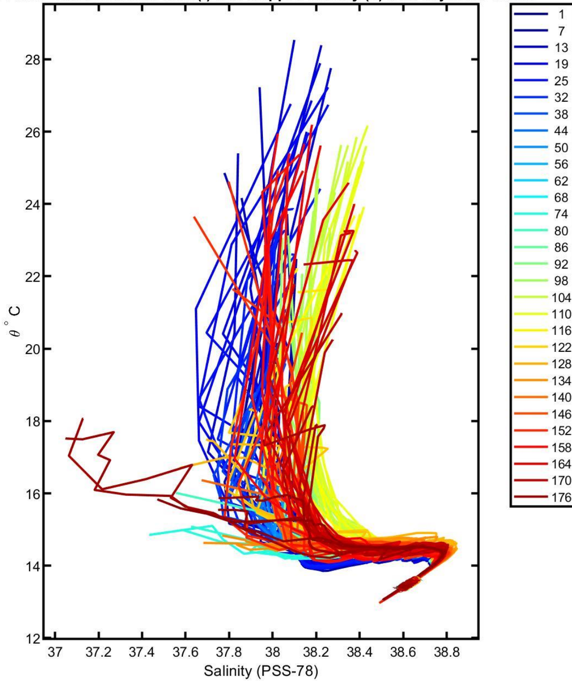
6901769 calibrated float data (-) and mapped salinity (o) with objective errors
