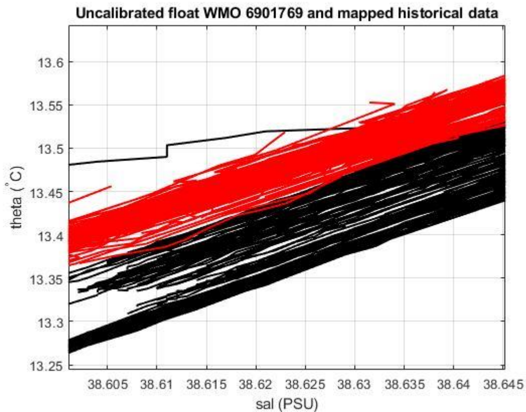
Figure 19: Float 6901769. Uncalibrated float salinity profile (black lines) and mapped historical data (red lines) in the most uniform part of the \theta -S curve.
