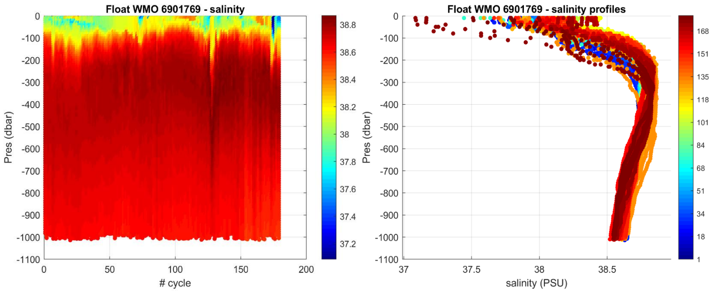
Figure 3: Float 6901769. Time series of Argo float potential salinity (PSS-78) on the left, and salinity profiles color-coded per cycle number on the right.
