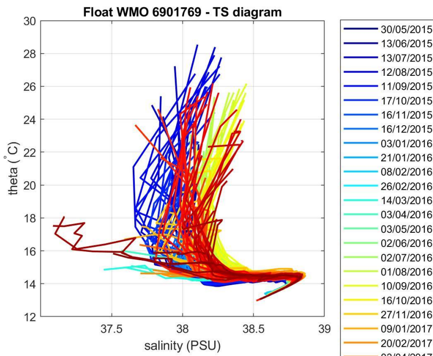
Figure 4: Float 6901769. \theta -S diagram color-coded per cycle number.
