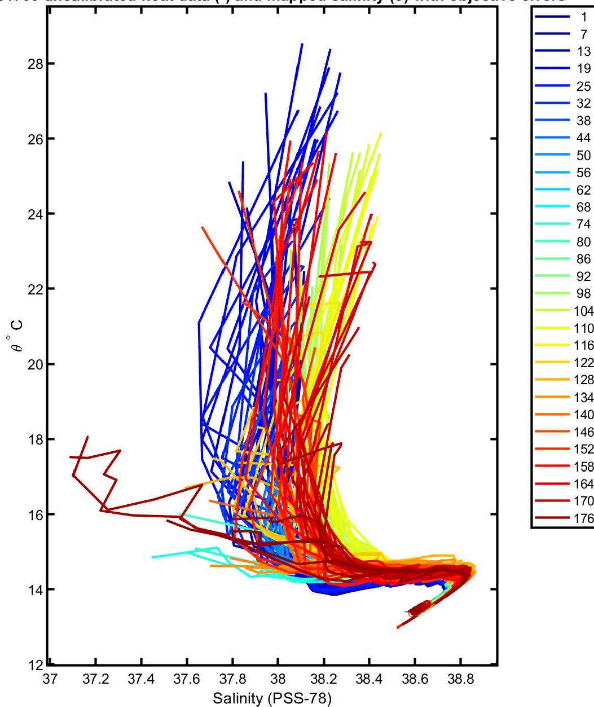
6901769 uncalibrated float data (-) and mapped salinity (o) with objective errors
