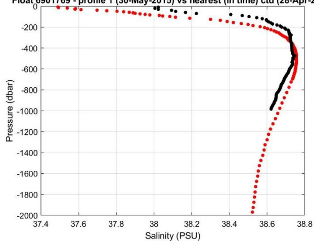
Float 6901769 - profile 1 (30-May-2015) vs nearest (in time) ctd (28-Apr-2014)
