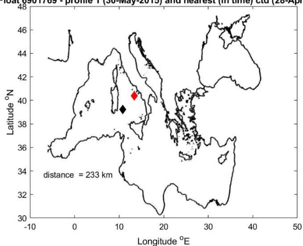
Float 6901769 - profile 1 (30-May-2015) and nearest (in time) ctd (28-Apr-2014)
