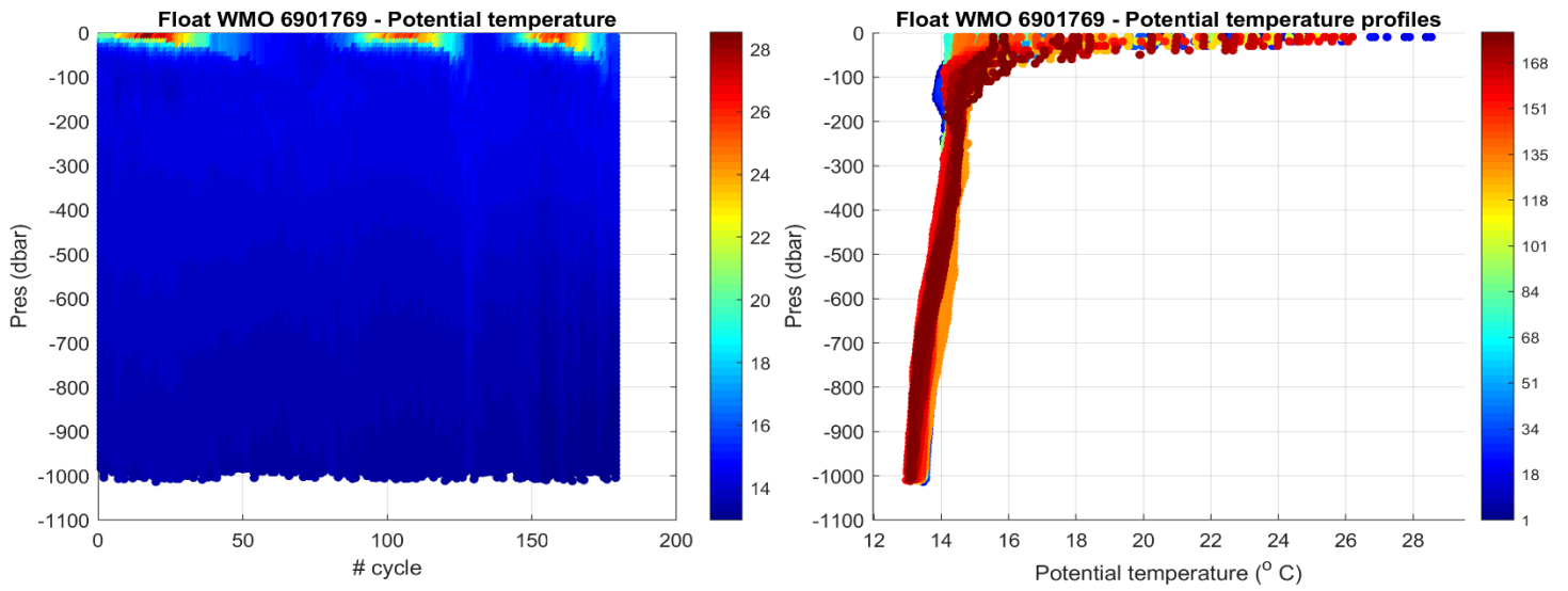
Figure 2: Float 6901769. Time series of Argo float potential temperature ( ^{\circ}\text{C} ) on the left, and potential temperature profiles color-coded per cycle number on the right.
