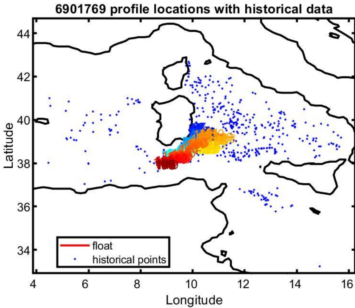
Figure 13: Float 6901769. Location of the float profiles (red line with colored numbers) and the reference data selected for mapping (blue dots).
