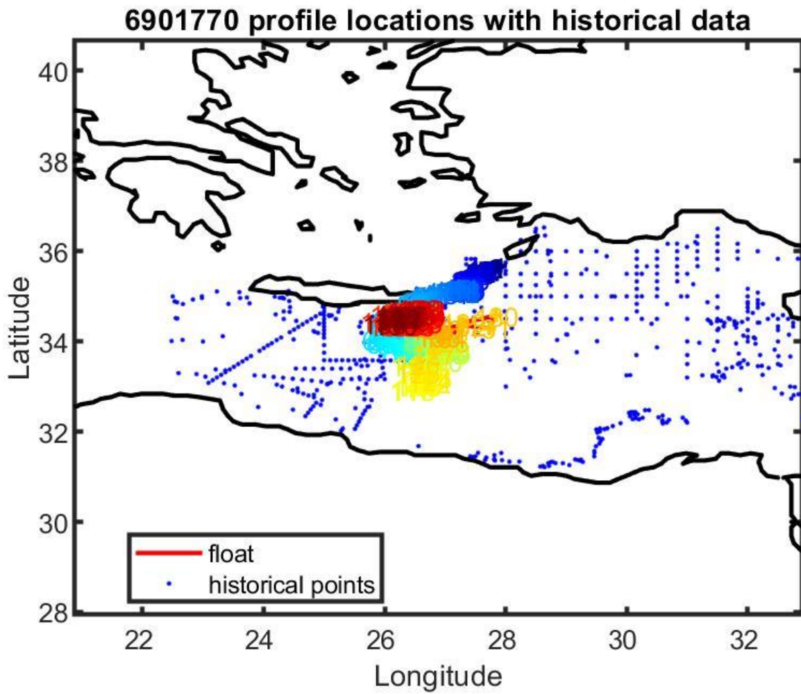
Figure 13: Float 6901770. Location of the float profiles (red line with colored numbers) and the reference data selected for mapping (blue dots).
