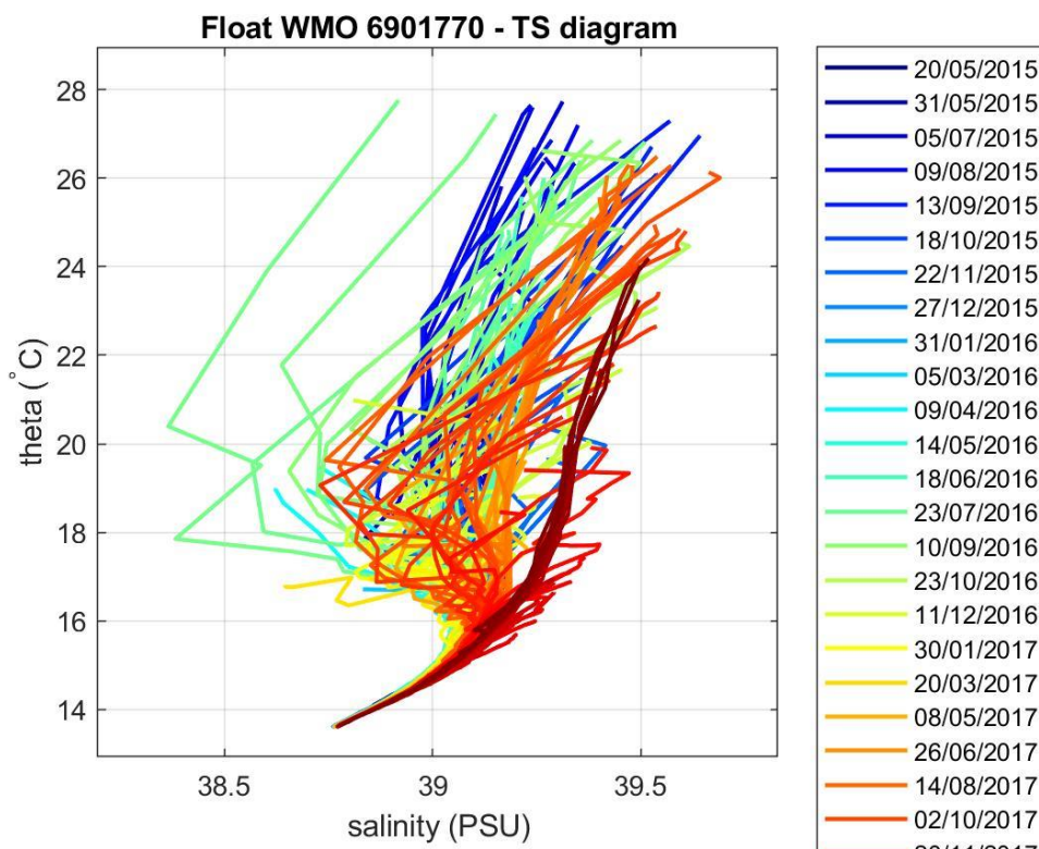
Figure 4: Float 6901770. \theta -S diagram color-coded per cycle number.
