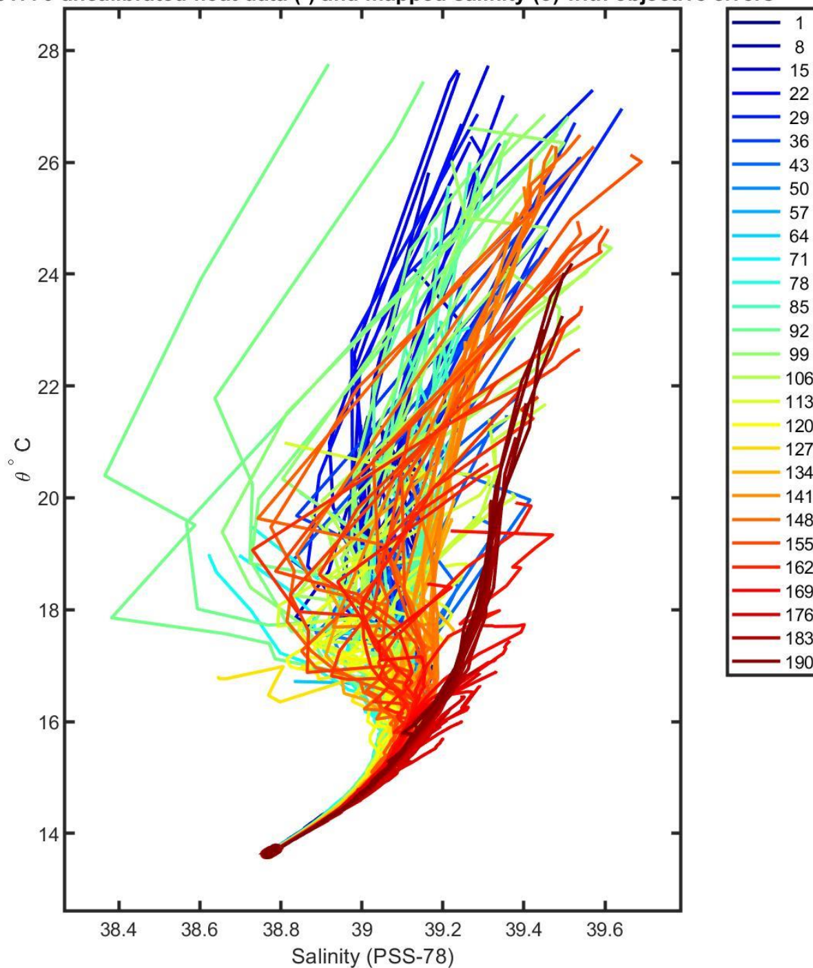
6901770 uncalibrated float data (-) and mapped salinity (o) with objective errors
