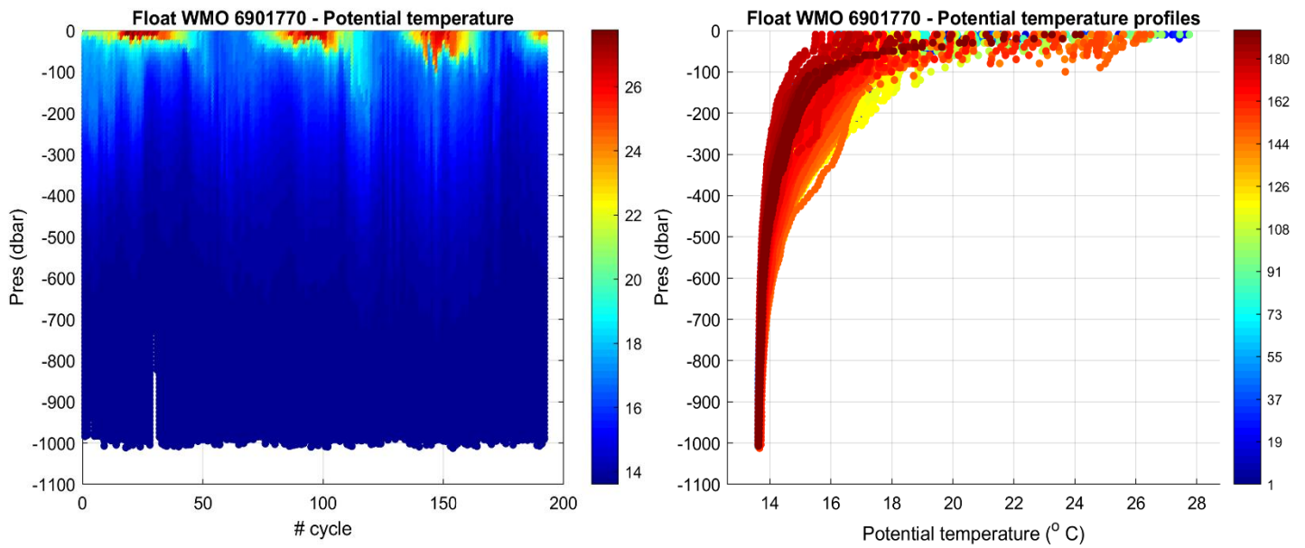
Figure 2: Float 6901770. Time series of Argo float potential temperature ( ^{\circ}\text{C} ) on the left, and potential temperature profiles color-coded per cycle number on the right.
