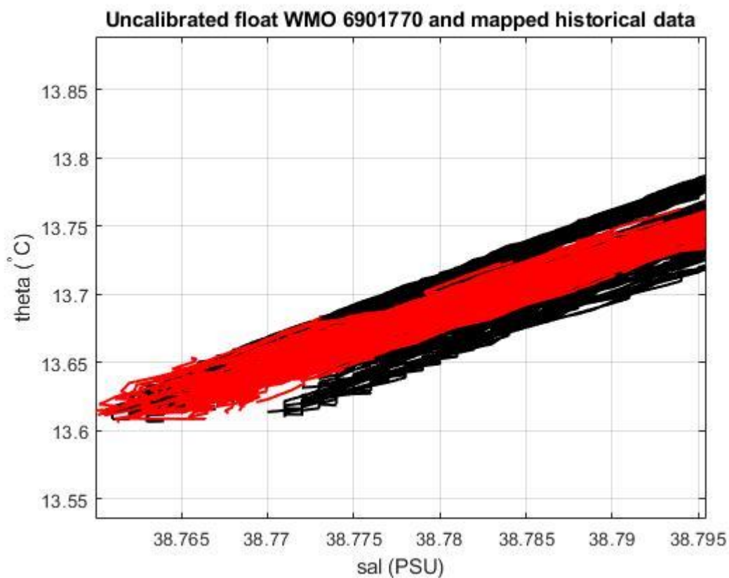
Figure 19: Float 6901770. Uncalibrated float salinity profile (black lines) and mapped historical data (red lines) in the most uniform part of the \theta -S curve.
