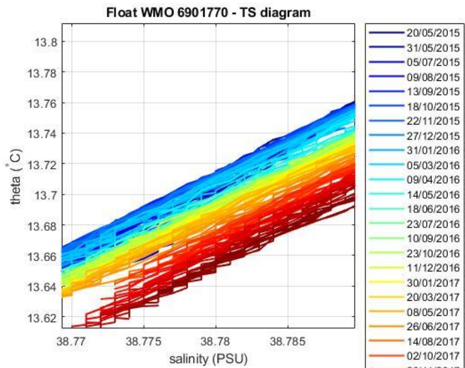
Figure 5: Float 6901770. Area of the \theta -S diagram (color-coded per cycle number) where the \theta -S relationship is more uniform.
