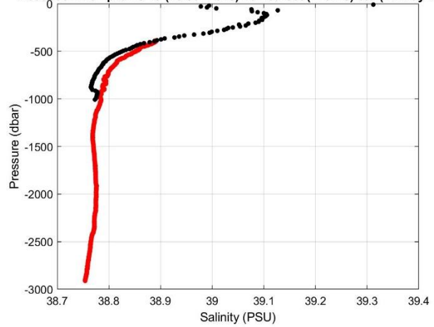
Float 6901770 - profile 19 (25-Jul-2015) vs nearest (in time) ctd (22-May-2015)
