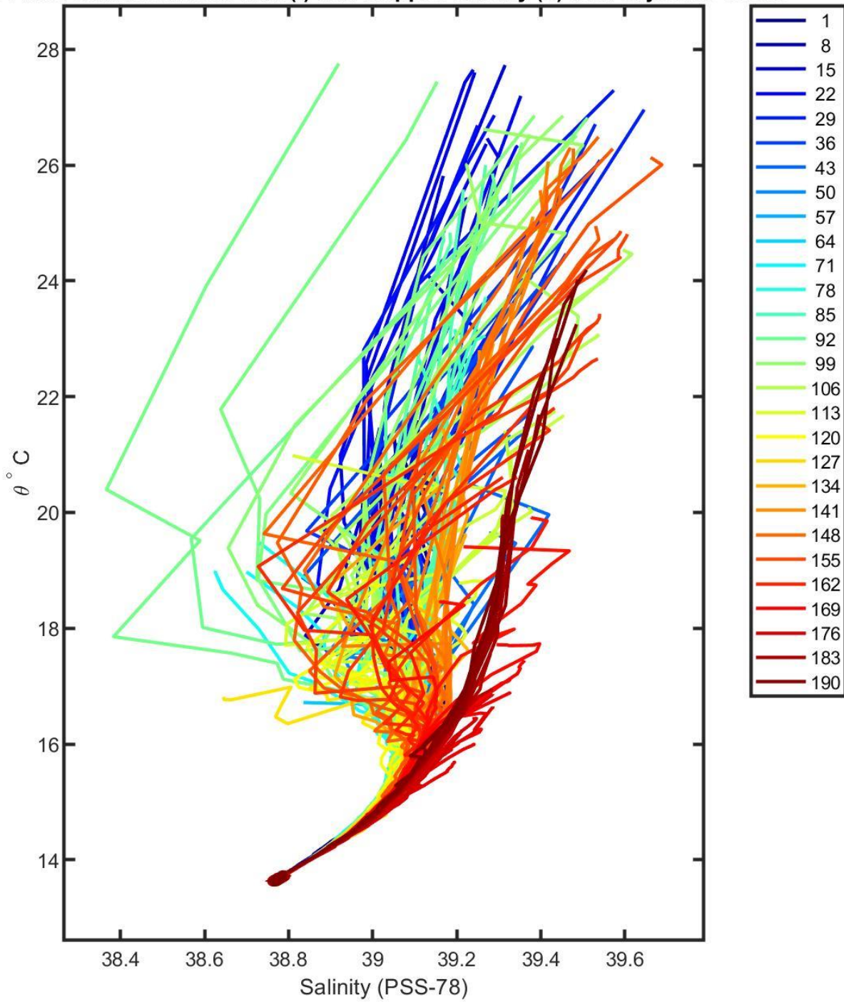
6901770 calibrated float data (-) and mapped salinity (o) with objective errors
