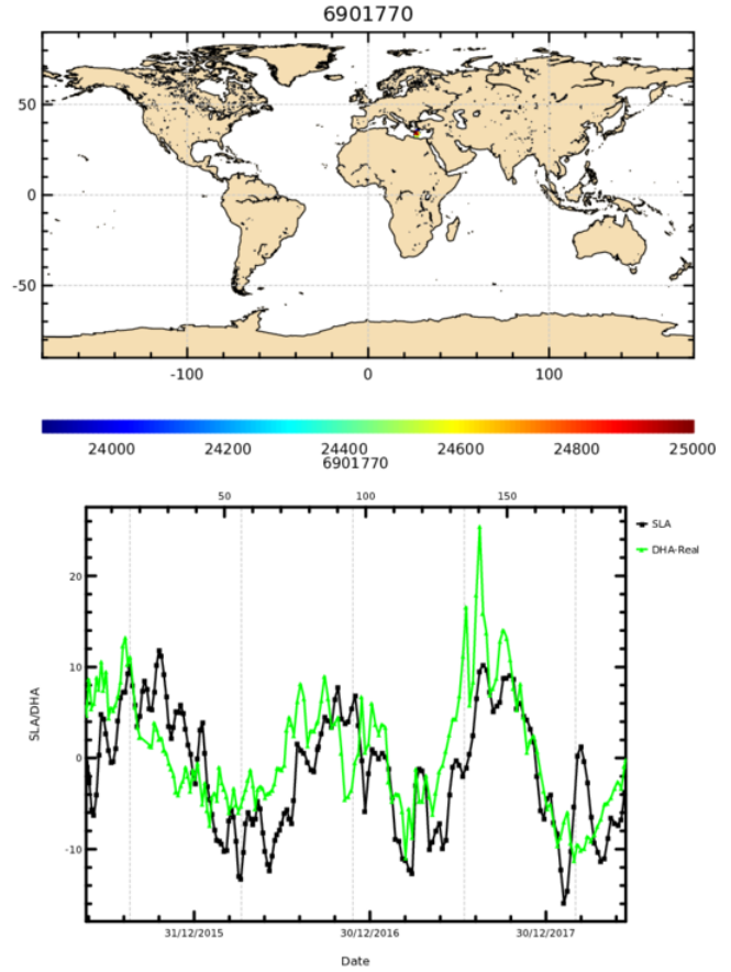
Figure 1: Float 6901770. The comparison between the sea surface height (SSH) from the satellite altimetry and dynamic height anomaly (DHA) extracted from the Argo float temperature and salinity. The figure is created by the CLS/Coriolis and distributed by Ifremer ( ftp://ftp.ifremer.fr/ifremer/argo/etc/argo-ast9-item13-AltimeterComparison/figures/ ).
