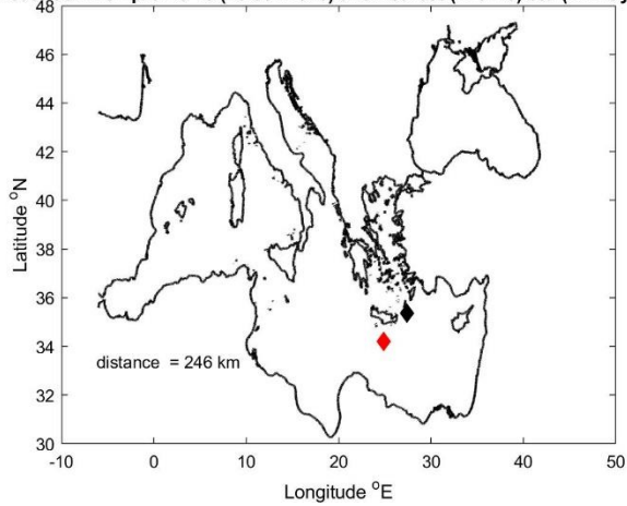
Float 6901770 - profile 19 (25-Jul-2015) and nearest (in time) ctd (22-May-2015)
