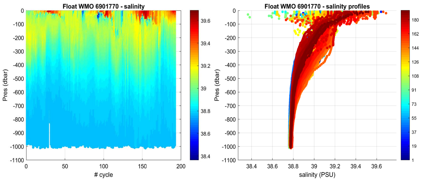
Figure 3: Float 6901770. Time series of Argo float potential salinity (PSS-78) on the left, and salinity profiles color-coded per cycle number on the right.
