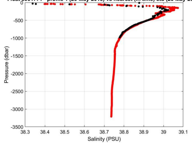
Float 6901771 - profile 1 (26-May-2015) vs nearest (in time) ctd (26-May-2015)
