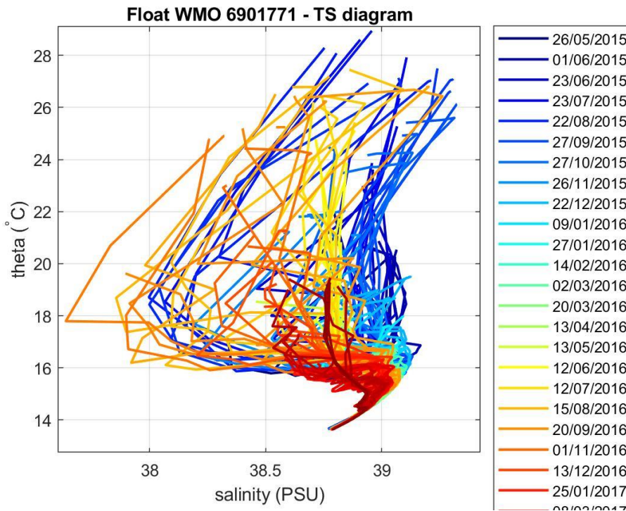
Figure 4: Float 6901771. \theta -S diagram color-coded per cycle number.
