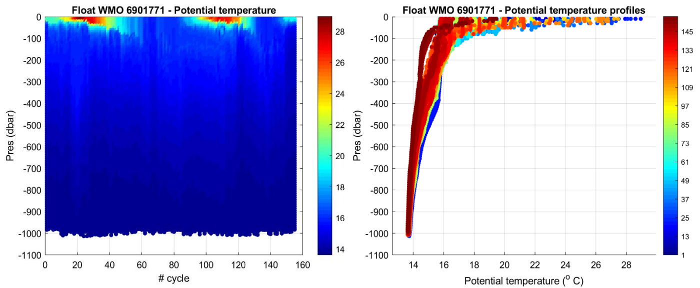
Figure 2: Float 6901771. Time series of Argo float potential temperature ( ^{\circ}\text{C} ) on the left, and potential temperature profiles color-coded per cycle number on the right.
