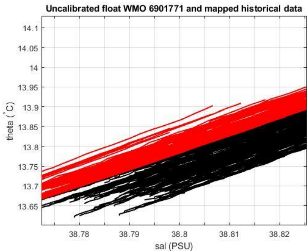
Figure 19: Float 6901771. Uncalibrated float salinity profile (black lines) and mapped historical data (red lines) in the most uniform part of the \theta -S curve.
