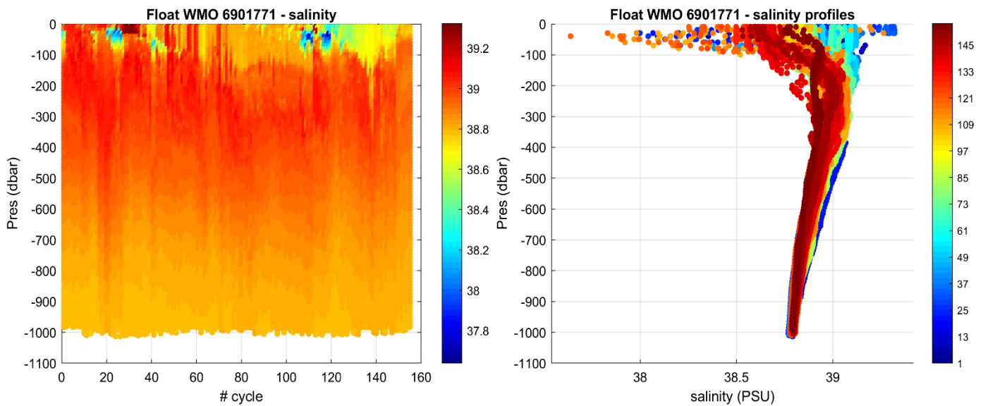
Figure 3: Float 6901771. Time series of Argo float potential salinity (PSS-78) on the left, and salinity profiles color-coded per cycle number on the right.
