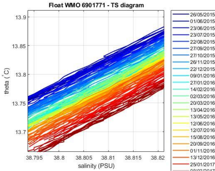
Figure 5: Float 6901771. Area of the \theta -S diagram (color-coded per cycle number) where the \theta -S relationship is more uniform.
