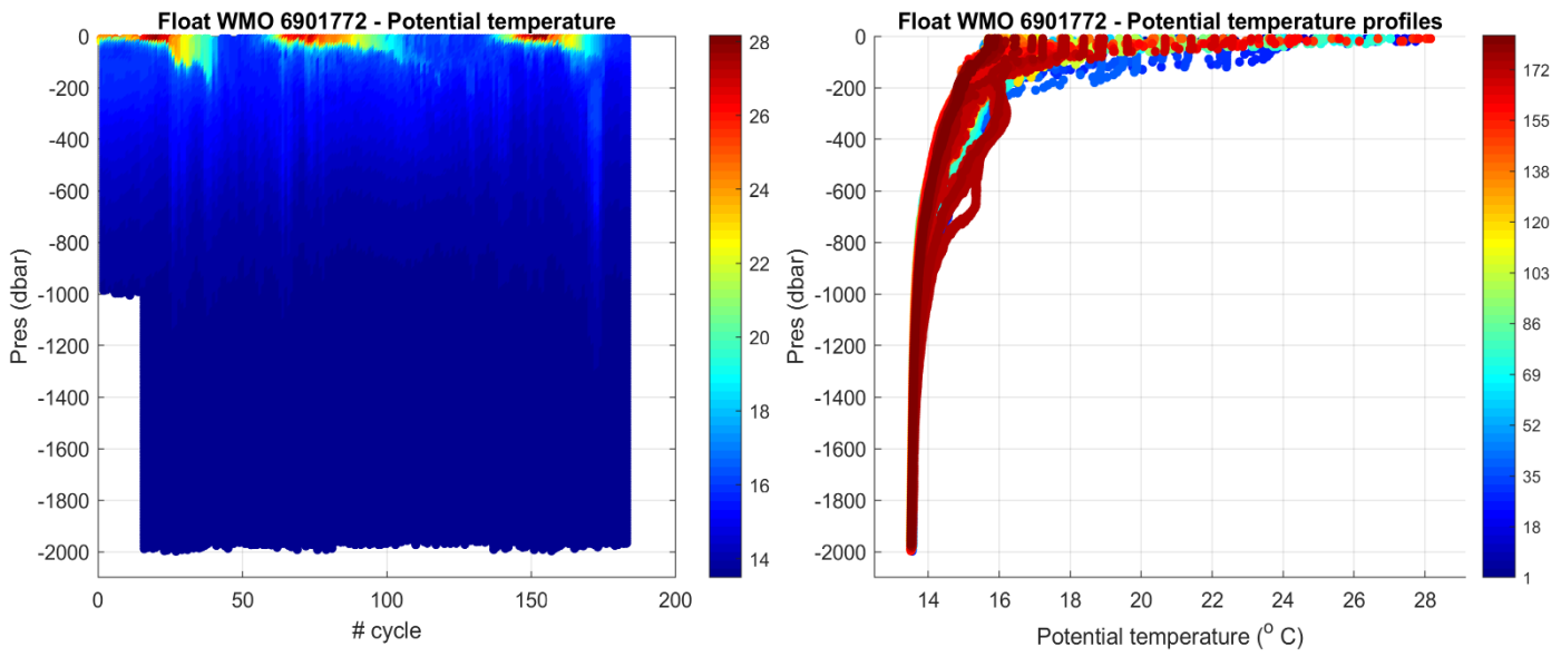
Figure 2: Float 6901772. Time series of Argo float potential temperature ( ^{\circ}\text{C} ) on the left, and potential temperature profiles color-coded per cycle number on the right.
