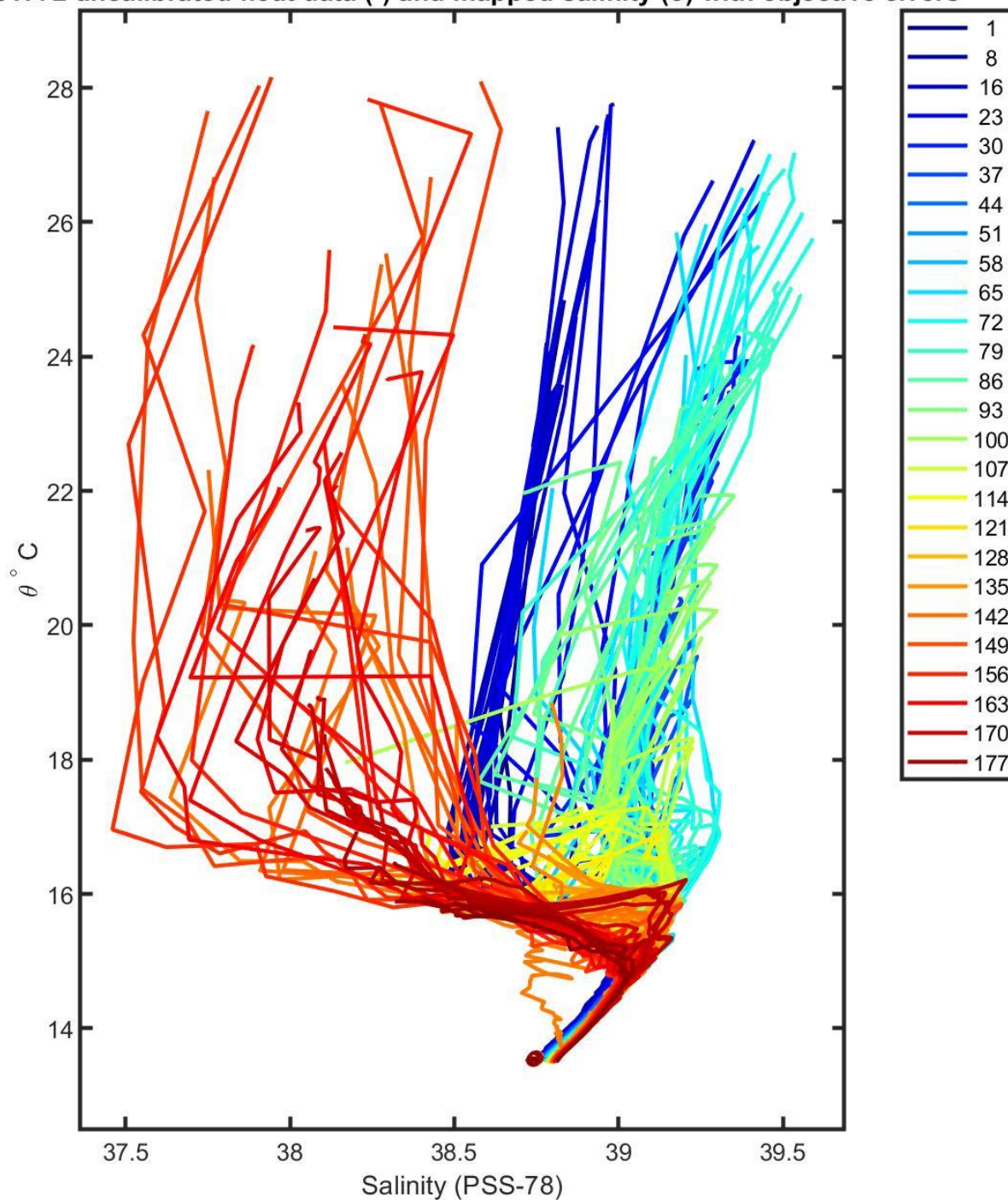
6901772 uncalibrated float data (-) and mapped salinity (o) with objective errors
