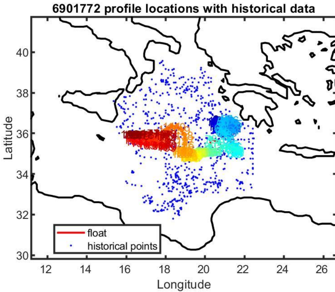
Figure 13: Float 6901772. Location of the float profiles (red line with colored numbers) and the reference data selected for mapping (blue dots).
