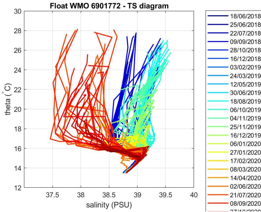
Figure 4: Float 6901772. \theta -S diagram color-coded per cycle number.
