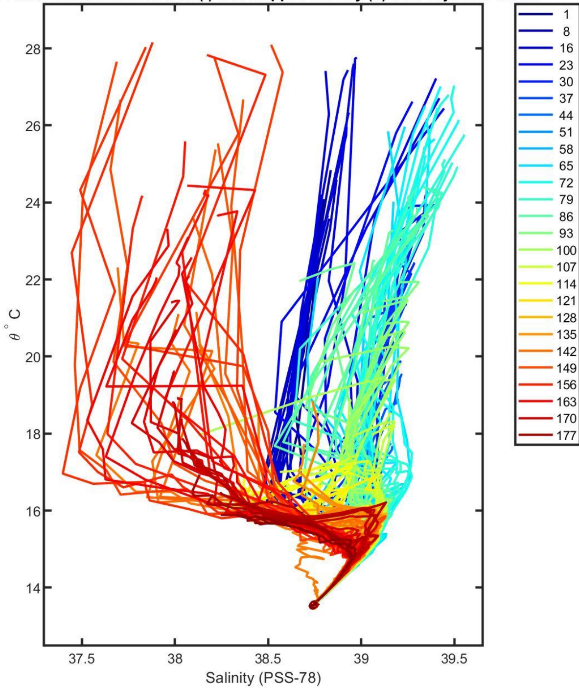
6901772 calibrated float data (-) and mapped salinity (o) with objective errors
