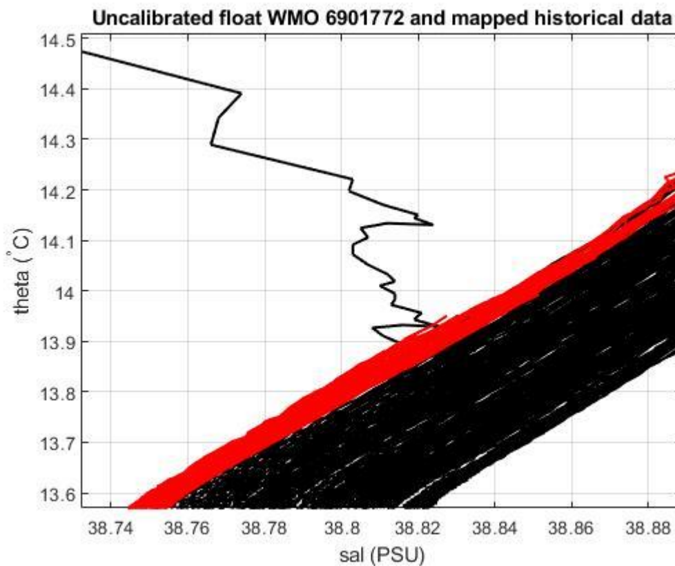
Figure 19: Float 6901772. Uncalibrated float salinity profile (black lines) and mapped historical data (red lines) in the most uniform part of the \theta -S curve.
