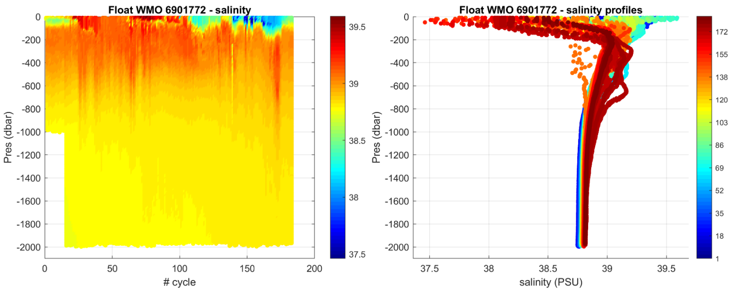
Figure 3: Float 6901772. Time series of Argo float potential salinity (PSS-78) on the left, and salinity profiles color-coded per cycle number on the right.
