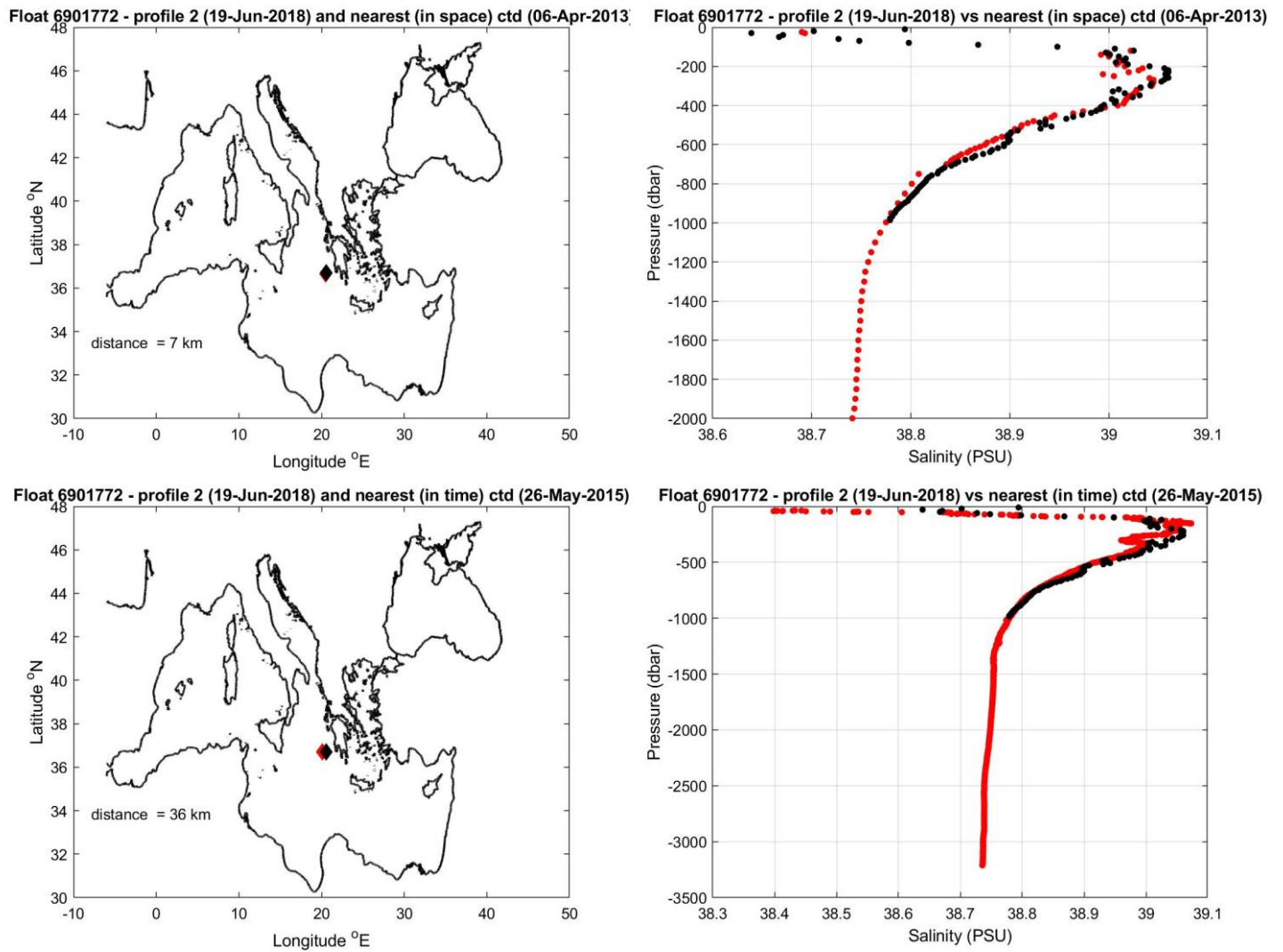
Figure 9: Float 6901772. The salinity float profile number 2 (black dots) are compared to the nearest in space (top) and in time (bottom) reference profile (red dots). The locations of the two profiles and their distance is given in the left panel.
