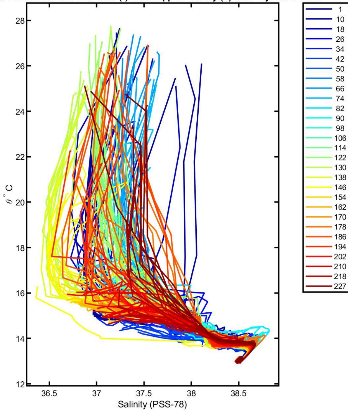
901774 uncalibrated float data (-) and mapped salinity (o) with objective errors
