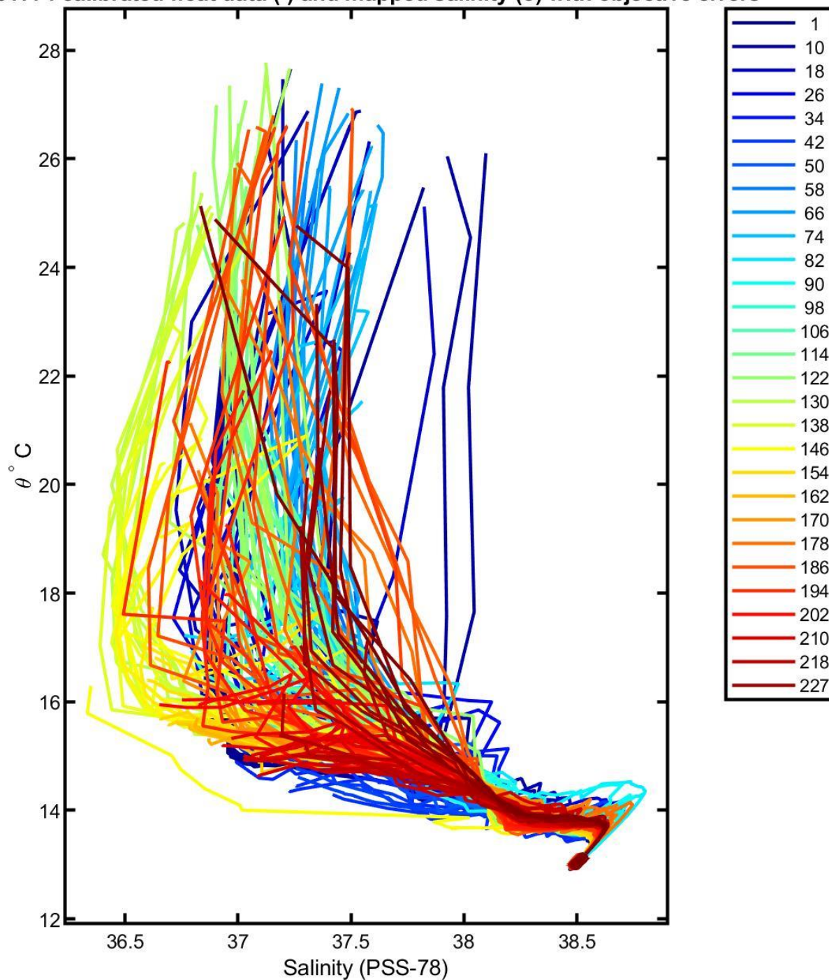
6901774 calibrated float data (-) and mapped salinity (o) with objective errors
