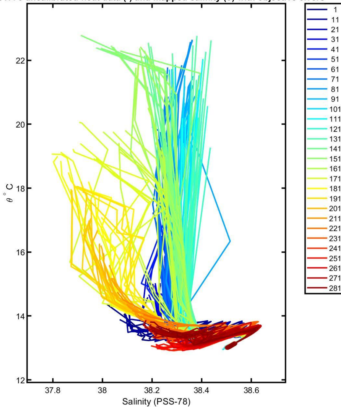
6901776 uncalibrated float data (-) and mapped salinity (o) with objective errors
