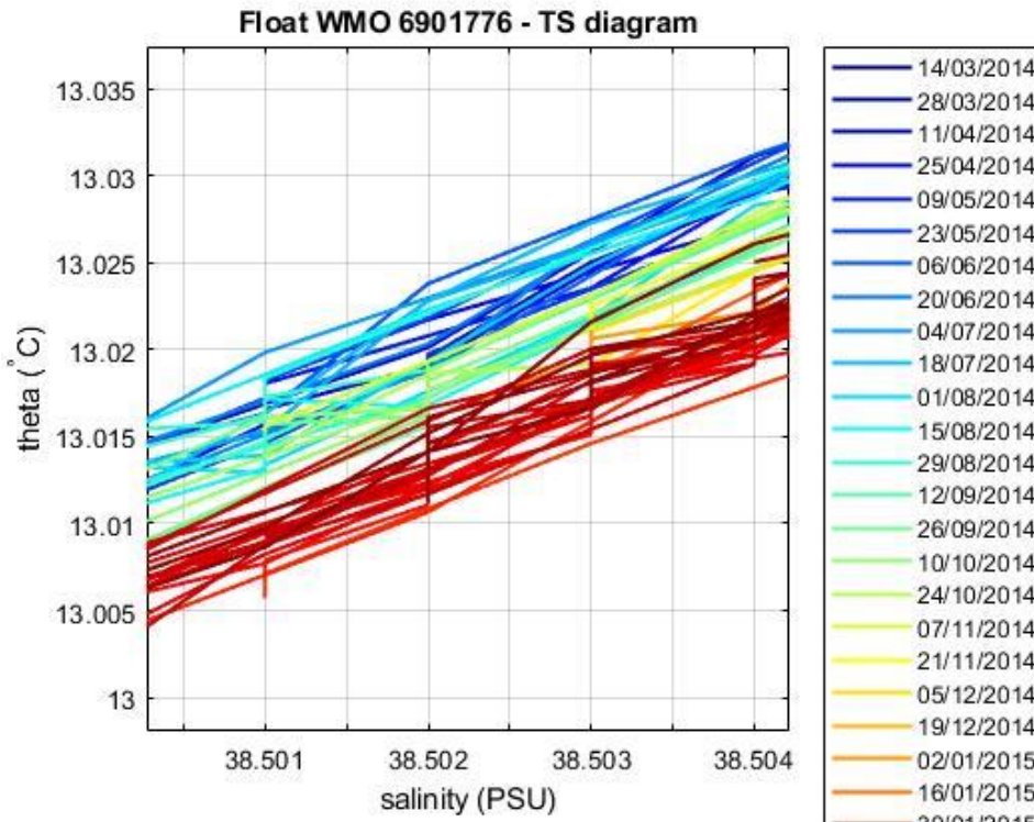
Figure 5: Float 6901776. Area of the \theta -S diagram (color-coded per cycle number) where the \theta -S relationship is more uniform.
