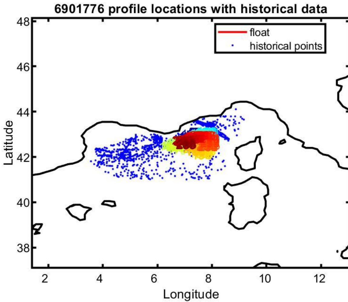
Figure 13: Float 6901776. Location of the float profiles (red line with colored numbers) and the reference data selected for mapping (blue dots).
