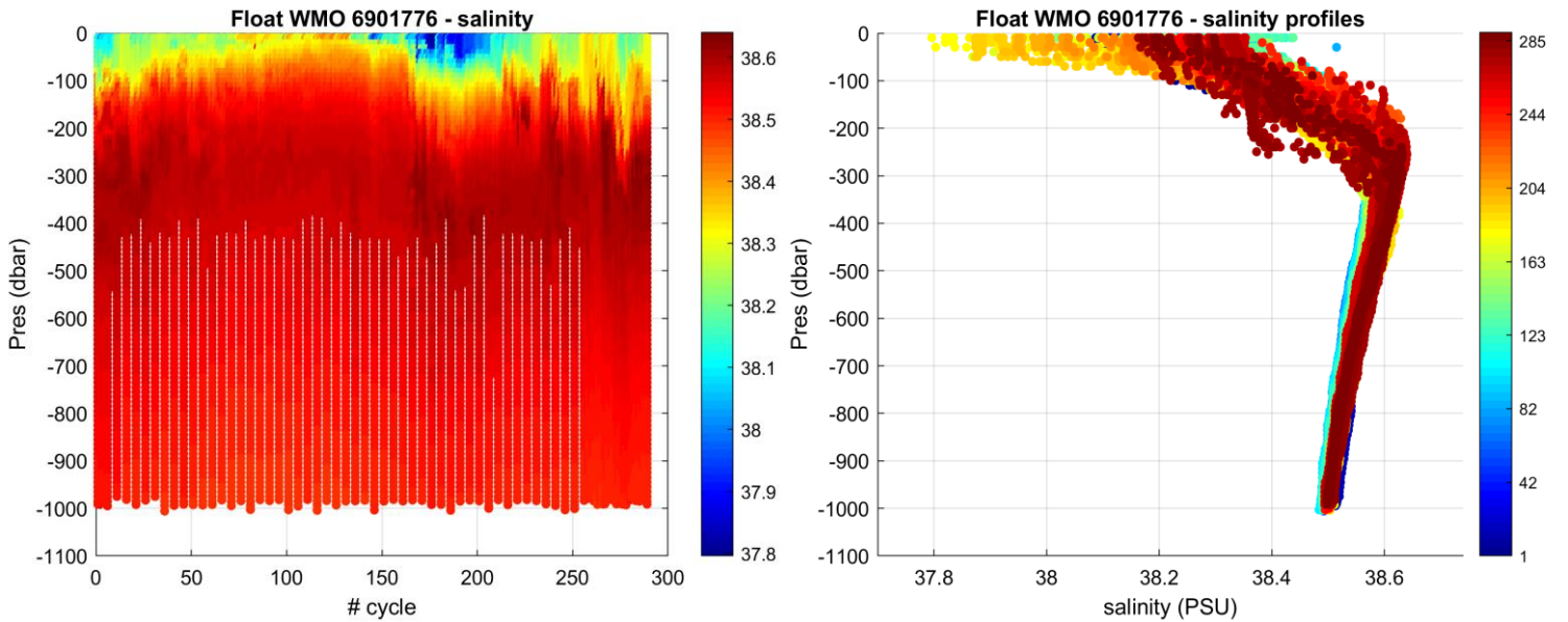
Figure 3: Float 6901776. Time series of Argo float potential salinity (PSS-78) on the left, and salinity profiles color-coded per cycle number on the right.
