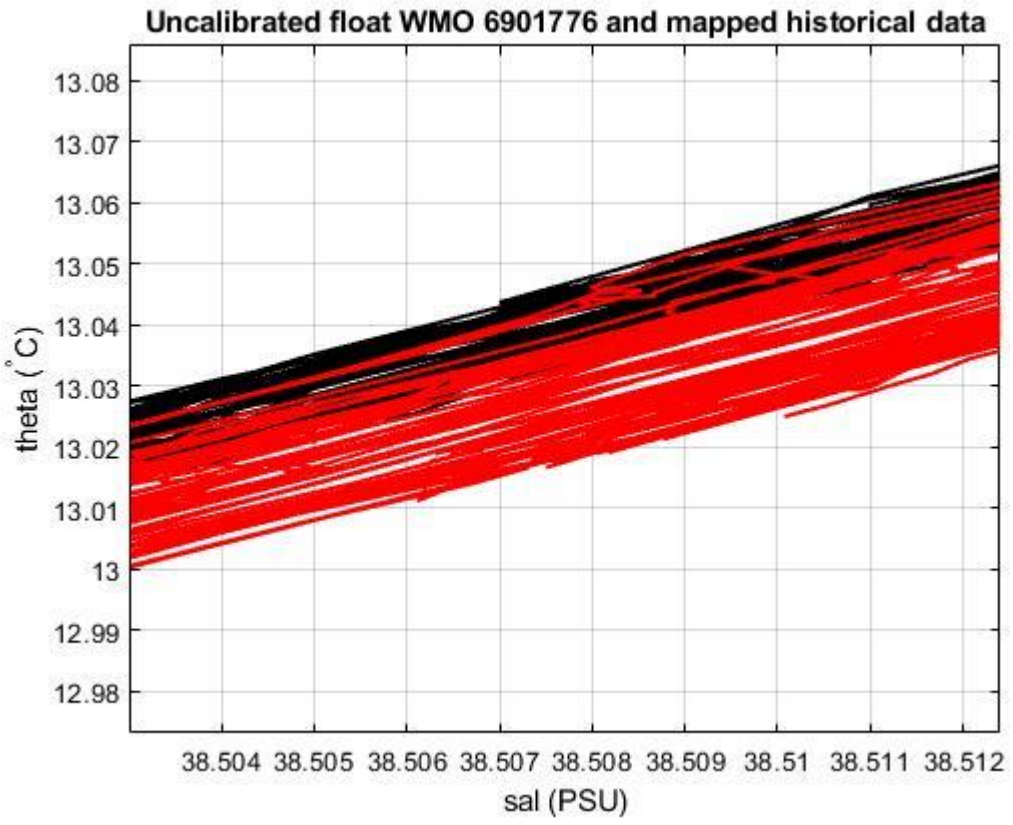
Figure 19: Float 6901776. Uncalibrated float salinity profile (black lines) and mapped historical data (red lines) in the most uniform part of the \theta -S curve.
