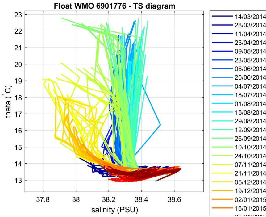
Figure 4: Float 6901776. \theta -S diagram color-coded per cycle number.
