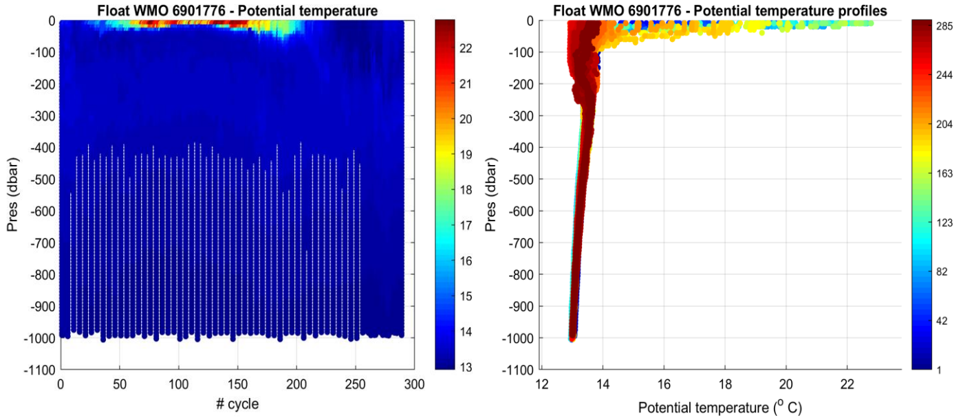
Figure 2: Float 6901776. Time series of Argo float potential temperature ( ^{\circ}\text{C} ) on the left, and potential temperature profiles color-coded per cycle number on the right.
