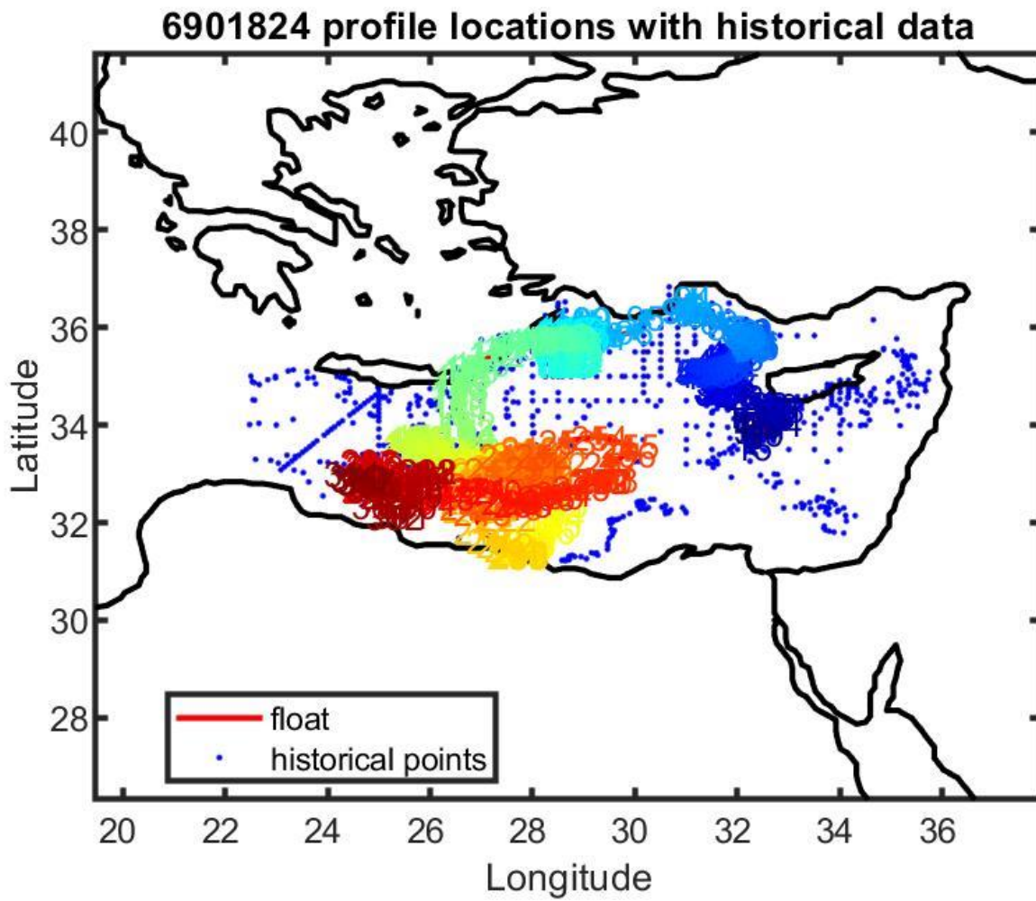
Figure 13: Float 6901824. Location of the float profiles (red line with colored numbers) and the reference data selected for mapping (blue dots).
