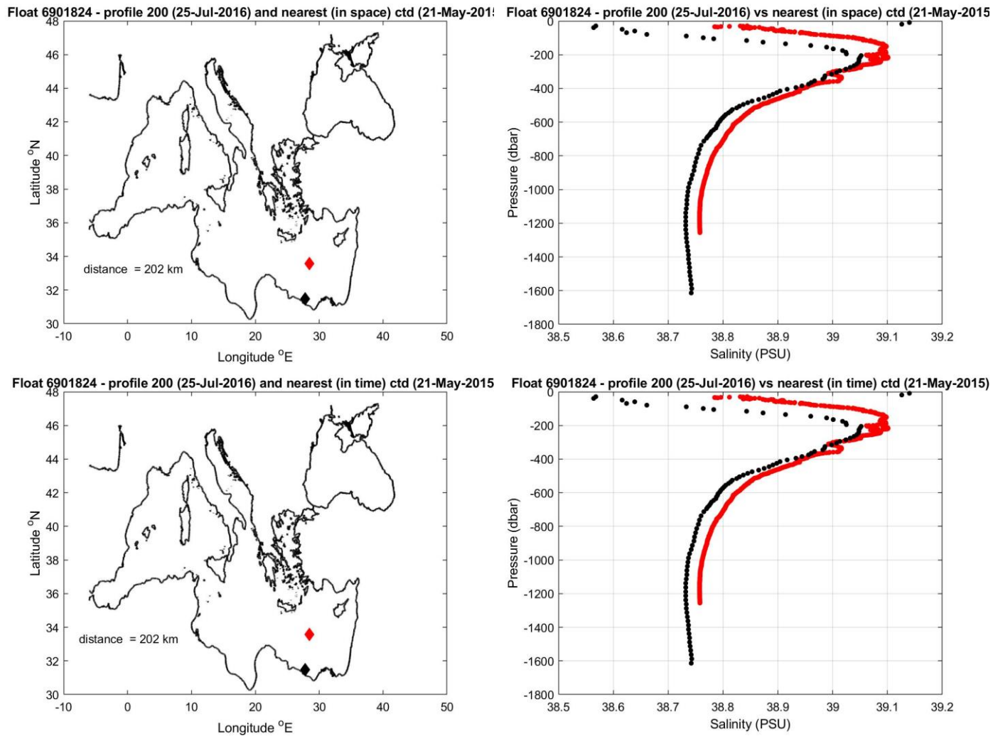
Figure 10: Float 6901824. The salinity float profile number 200 (black dots) are compared to the nearest in space (top) and in time (bottom) reference profile (red dots). The locations of the two profiles and their distance is given in the left panel.
