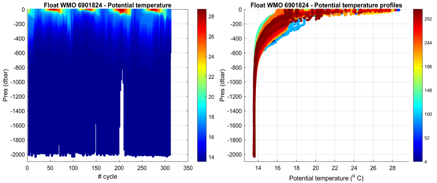
Figure 2: Float 6901824. Time series of Argo float potential temperature ( ^{\circ}\text{C} ) on the left, and potential temperature profiles color-coded per cycle number on the right.
