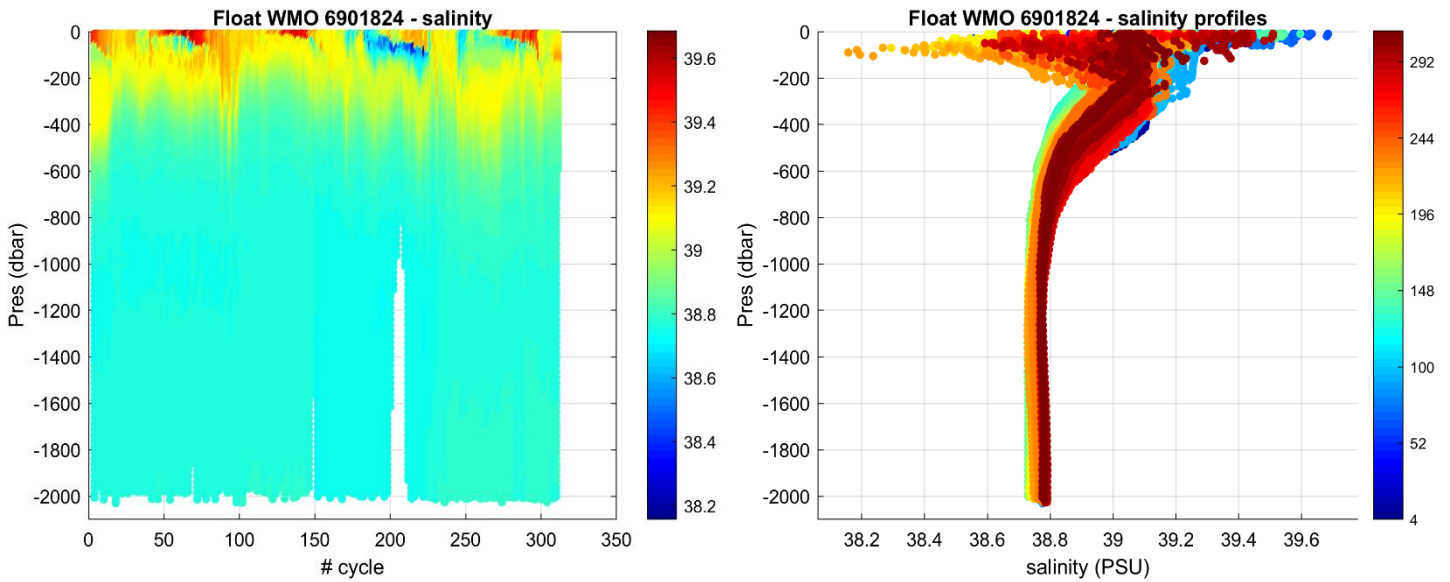
Figure 3: Float 6901824. Time series of Argo float potential salinity (PSS-78) on the left, and salinity profiles color-coded per cycle number on the right.
