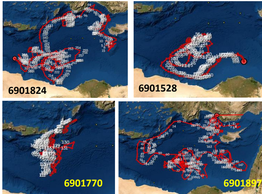
Figure 20: Float 6901824. Trajectory of the floats used for the comparison.
