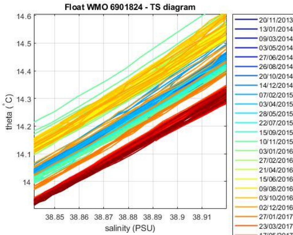
Figure 5: Float 6901824. Area of the \theta -S diagram (color-coded per cycle number) where the \theta -S relationship is more uniform.
