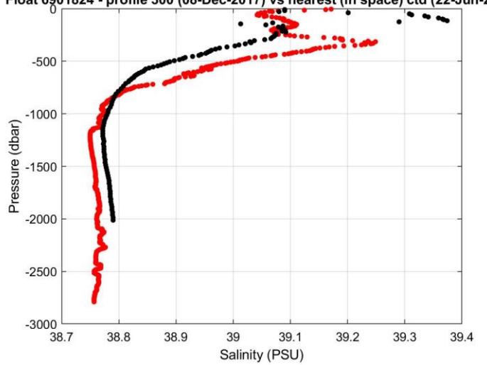
Float 6901824 - profile 300 (08-Dec-2017) vs nearest (in space) ctd (22-Jun-2008)
