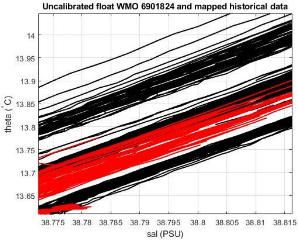
Figure 19: Float 6901824. Uncalibrated float salinity profile (black lines) and mapped historical data (red lines) in the most uniform part of the \theta -S curve.
