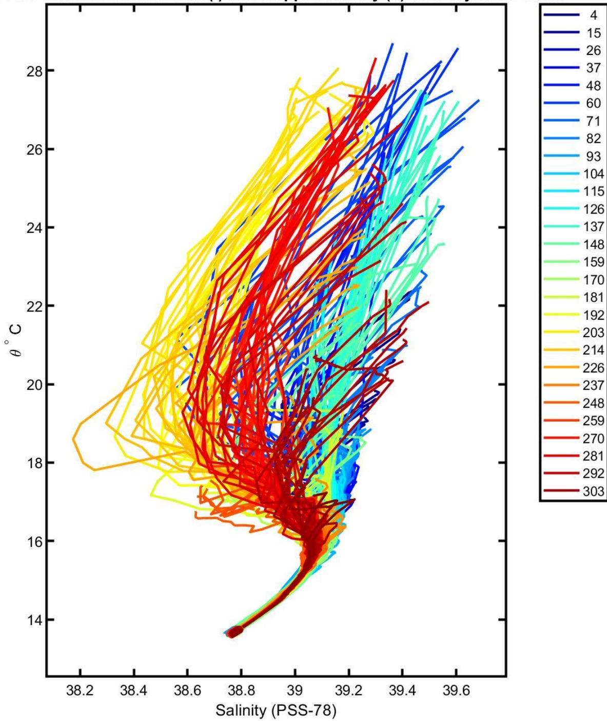
6901824 calibrated float data (-) and mapped salinity (o) with objective errors
