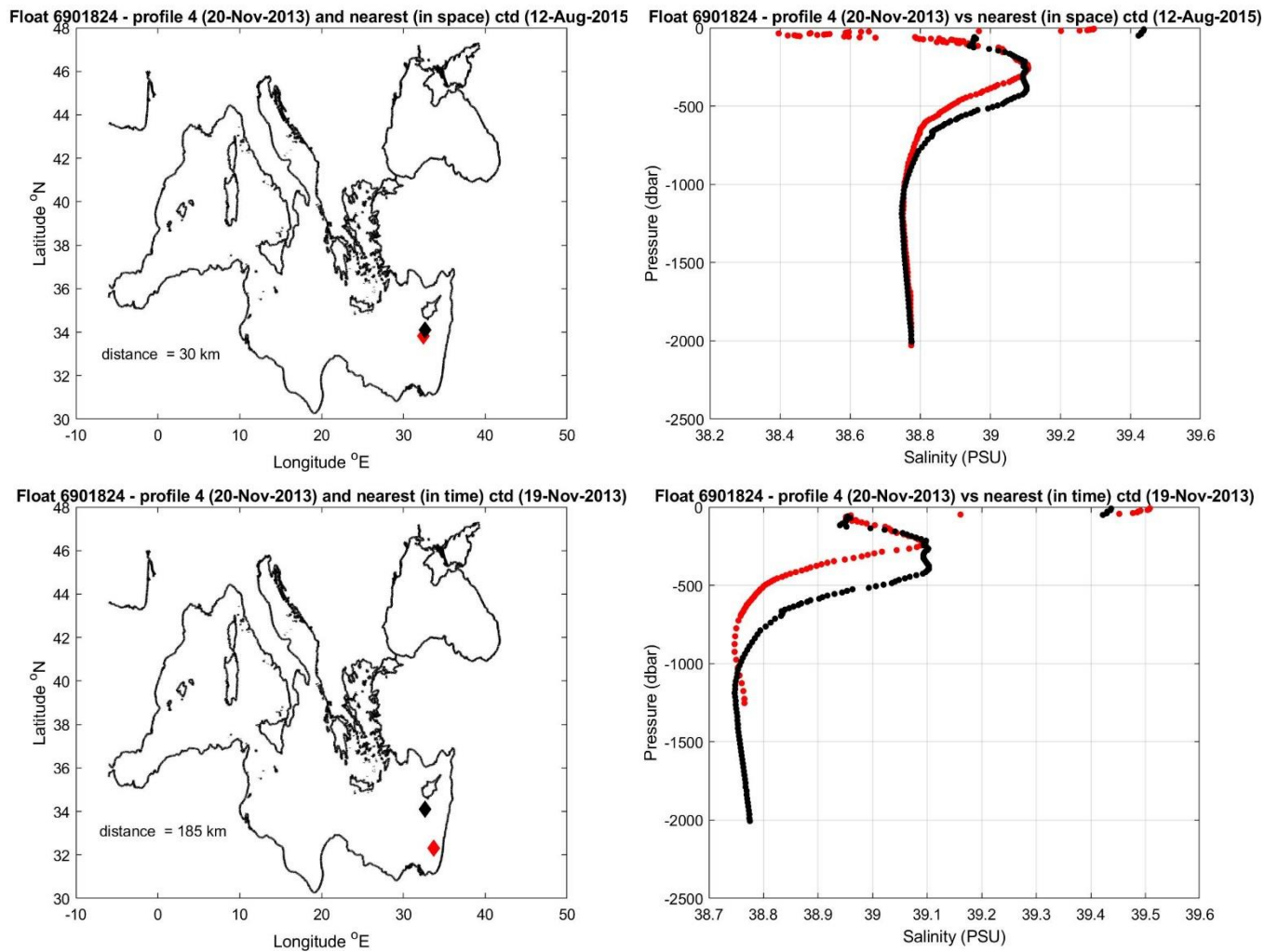
Figure 9: Float 6901824. The salinity float profile number 4 (black dots) are compared to the nearest in space (top) and in time (bottom) reference profile (red dots). The locations of the two profiles and their distance is given in the left panel.
