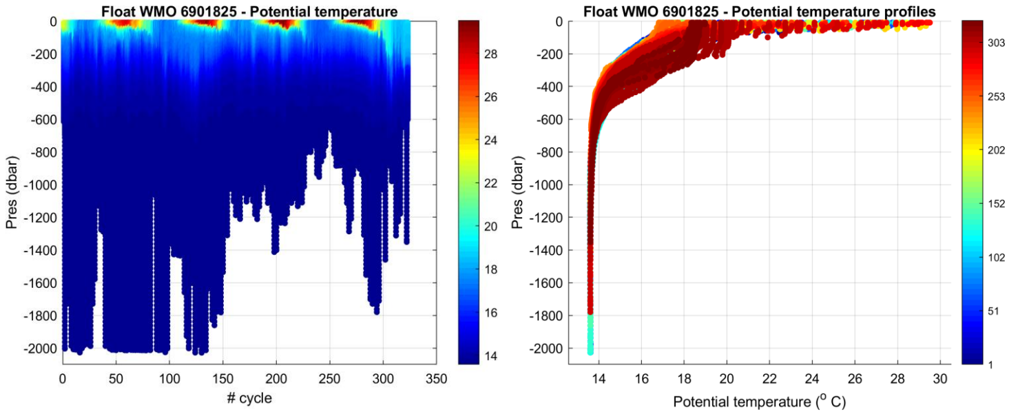
Figure 2: Float 6901825. Time series of Argo float potential temperature ( ^{\circ}\text{C} ) on the left, and potential temperature profiles color-coded per cycle number on the right.
