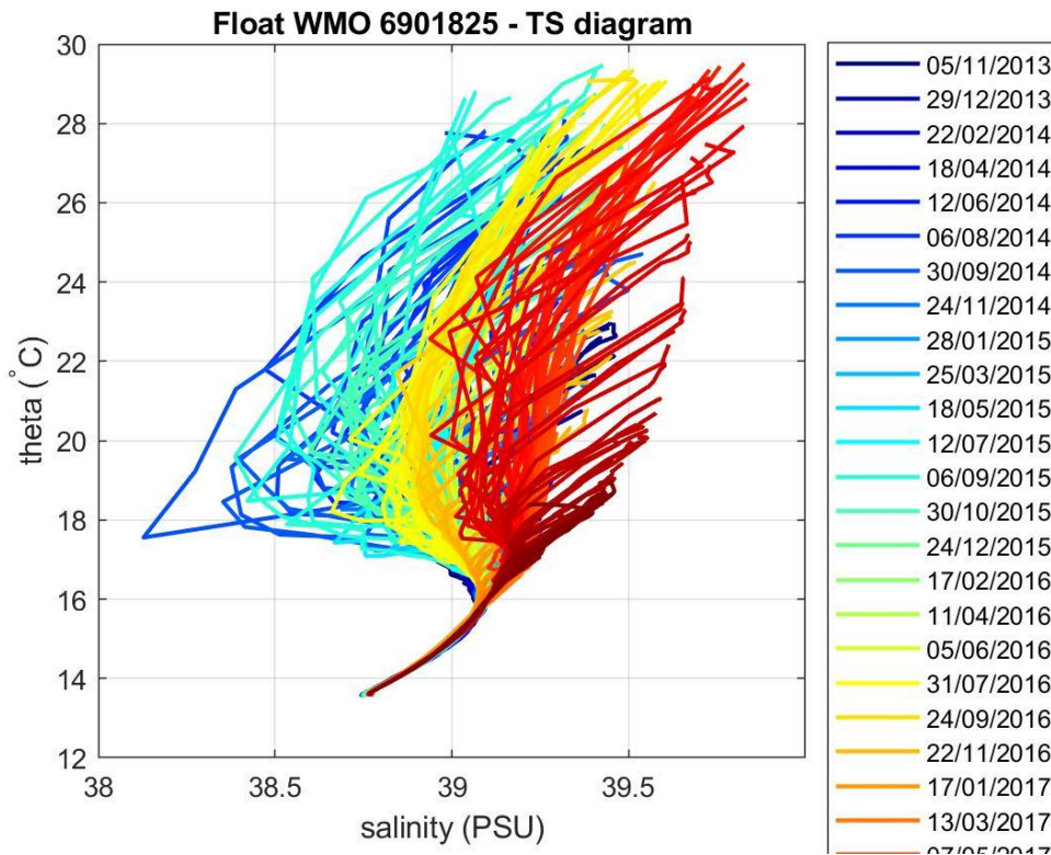
Figure 4: Float 6901825. \theta -S diagram color-coded per cycle number.
