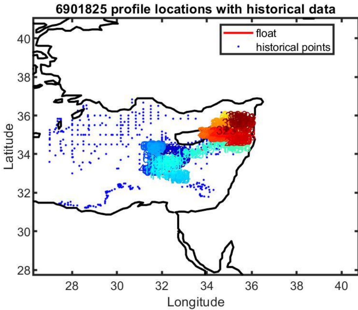
Figure 13: Float 6901825. Location of the float profiles (red line with colored numbers) and the reference data selected for mapping (blue dots).
