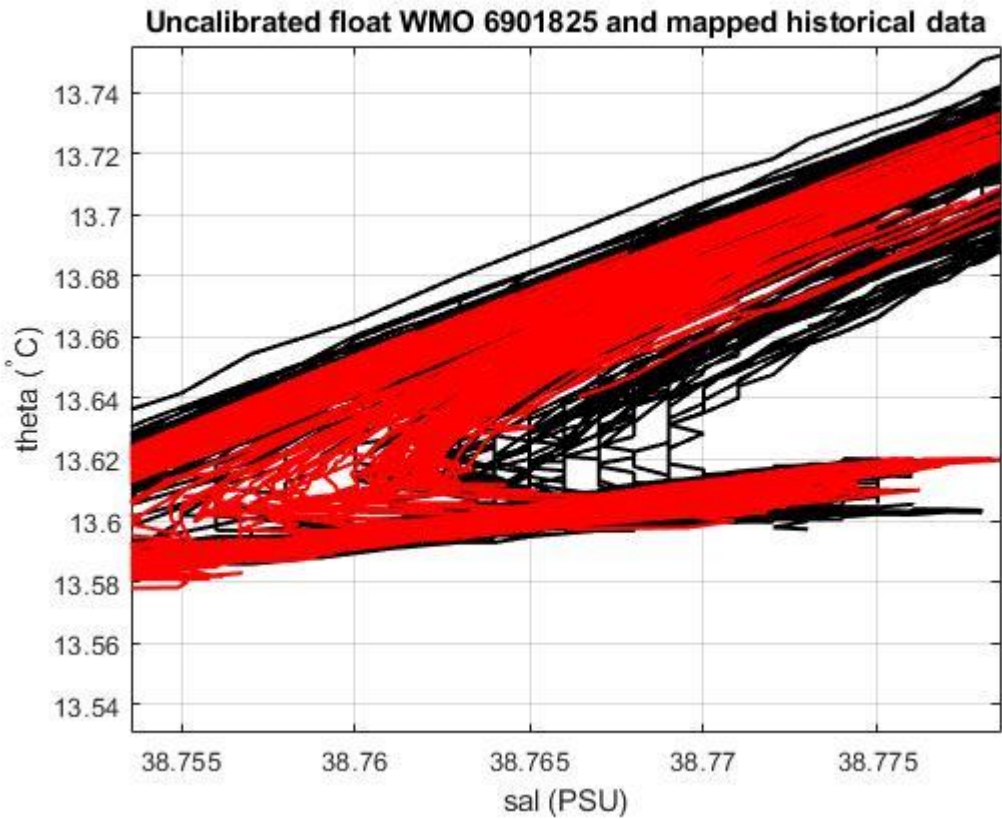
Figure 19: Float 6901825. Uncalibrated float salinity profile (black lines) and mapped historical data (red lines) in the most uniform part of the \theta -S curve.
