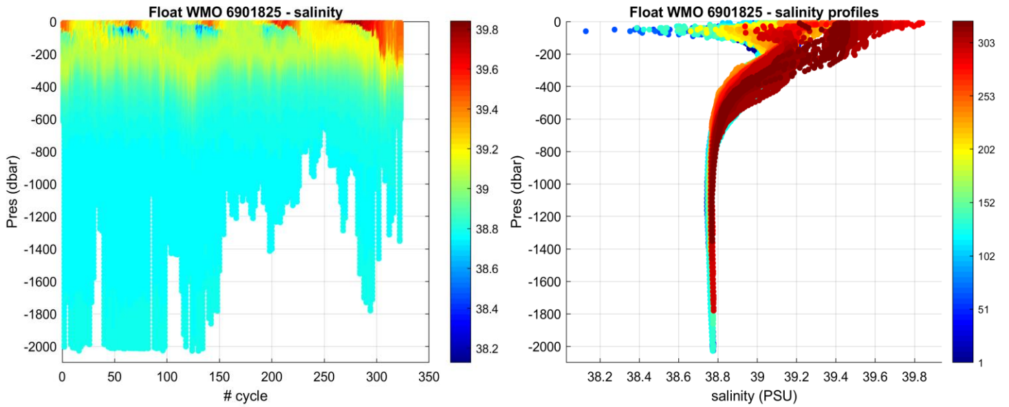
Figure 3: Float 6901825. Time series of Argo float potential salinity (PSS-78) on the left, and salinity profiles color-coded per cycle number on the right.
