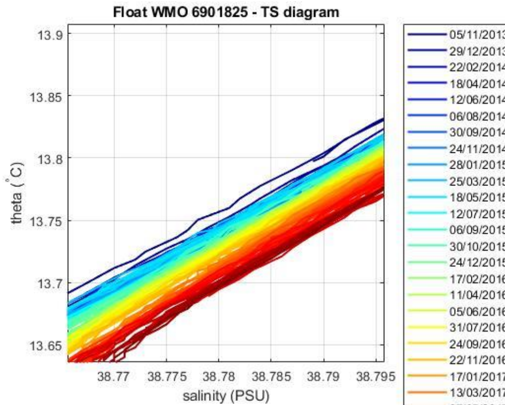
Figure 5: Float 6901825. Area of the \theta -S diagram (color-coded per cycle number) where the \theta -S relationship is more uniform.
