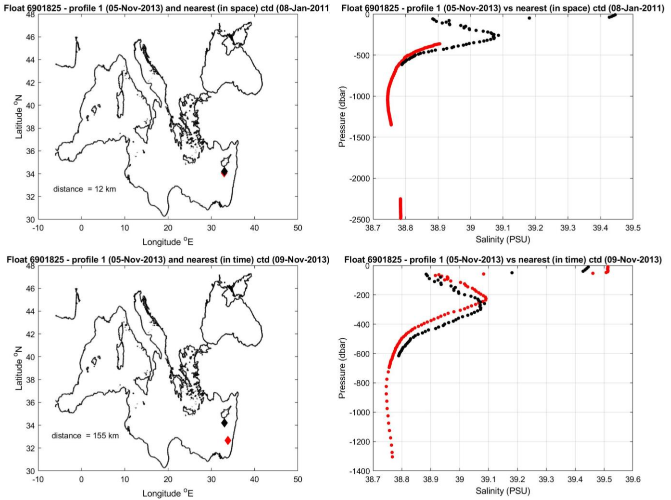
Figure 9: Float 6901825. The salinity float profile number 1 (black dots) are compared to the nearest in space (top) and in time (bottom) reference profile (red dots). The locations of the two profiles and their distance is given in the left panel.
