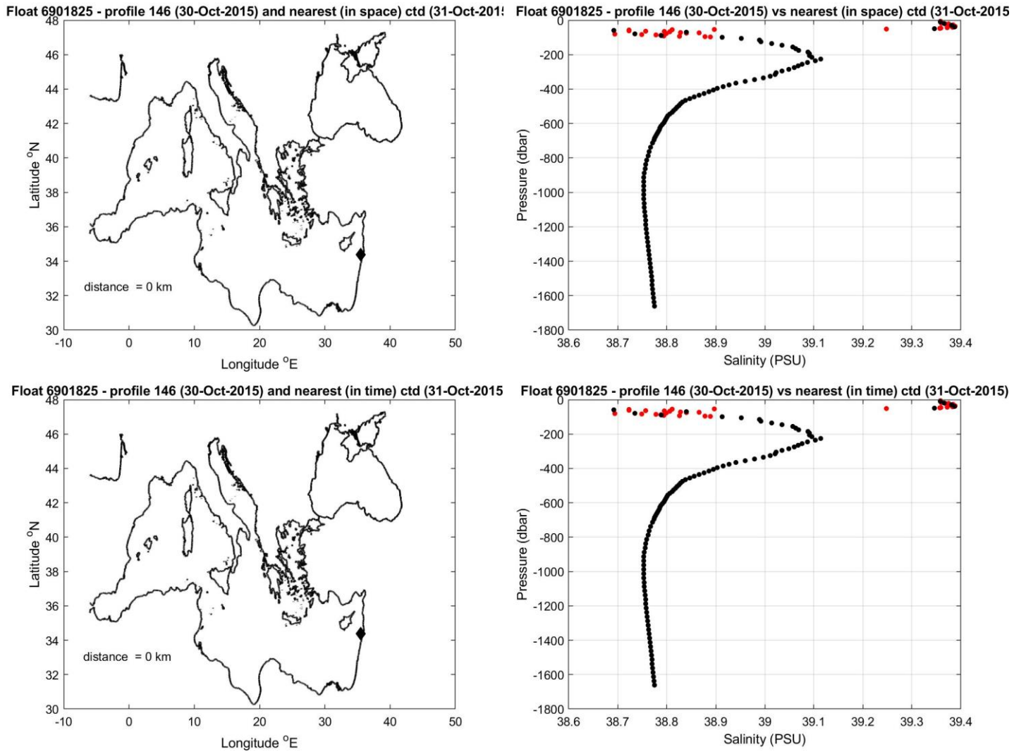
Figure 10: Float 6901825. The salinity float profile number 146 (black dots) are compared to the nearest in space (top) and in time (bottom) reference profile (red dots). The locations of the two profiles and their distance is given in the left panel.
