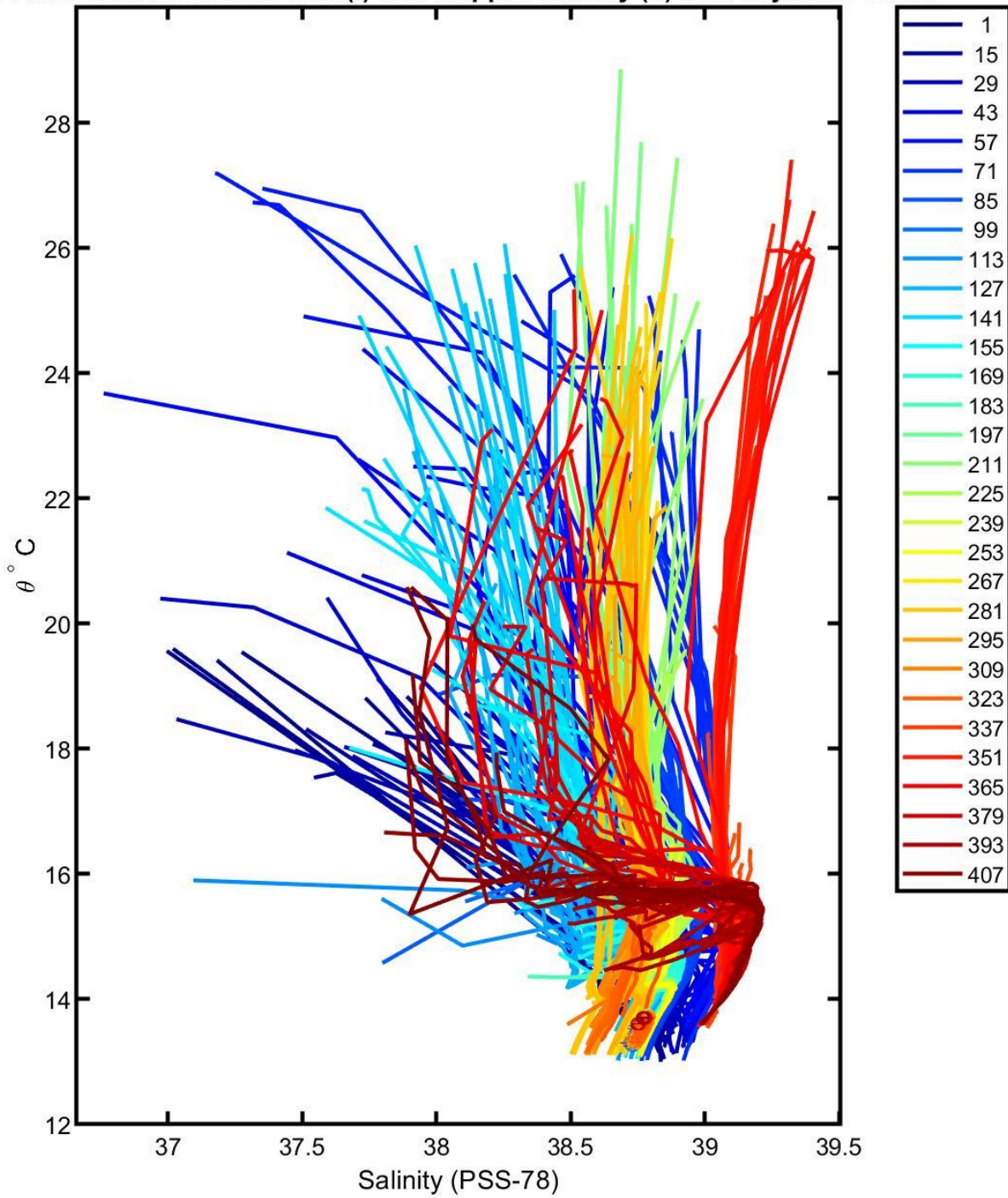
6901826 calibrated float data (-) and mapped salinity (o) with objective errors
