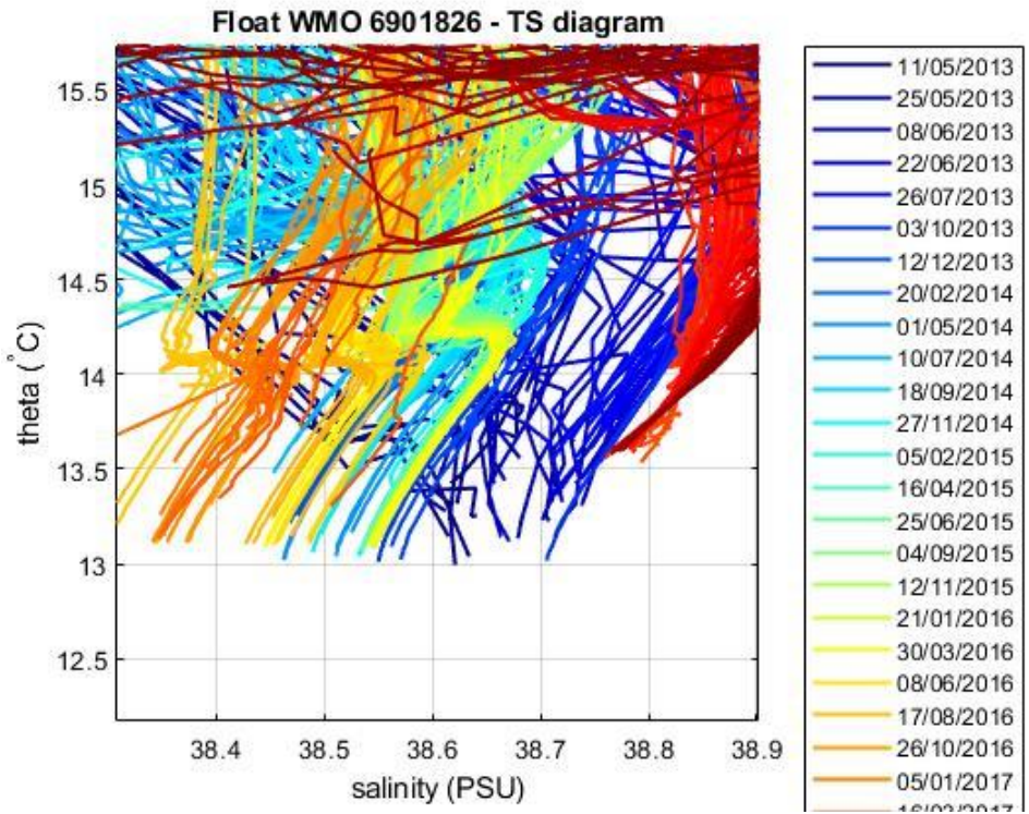
Figure 5: Float 6901826. Area of the \theta -S diagram (color-coded per cycle number) where the \theta -S relationship is more uniform.
