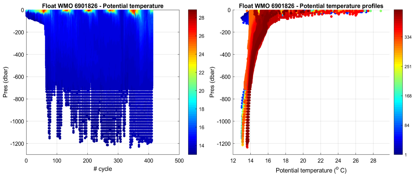
Figure 2: Float 6901826. Time series of Argo float potential temperature ( ^{\circ}\text{C} ) on the left, and potential temperature profiles color-coded per cycle number on the right.
