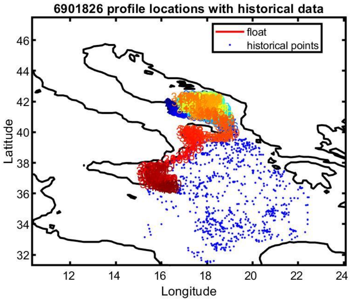
Figure 13: Float 6901826. Location of the float profiles (red line with colored numbers) and the reference data selected for mapping (blue dots).
