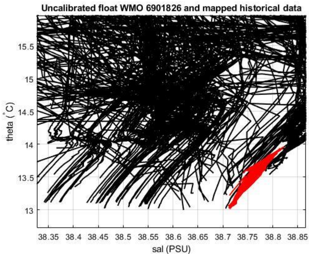
Figure 19: Float 6901826. Uncalibrated float salinity profile (black lines) and mapped historical data (red lines) in the most uniform part of the \theta -S curve.
