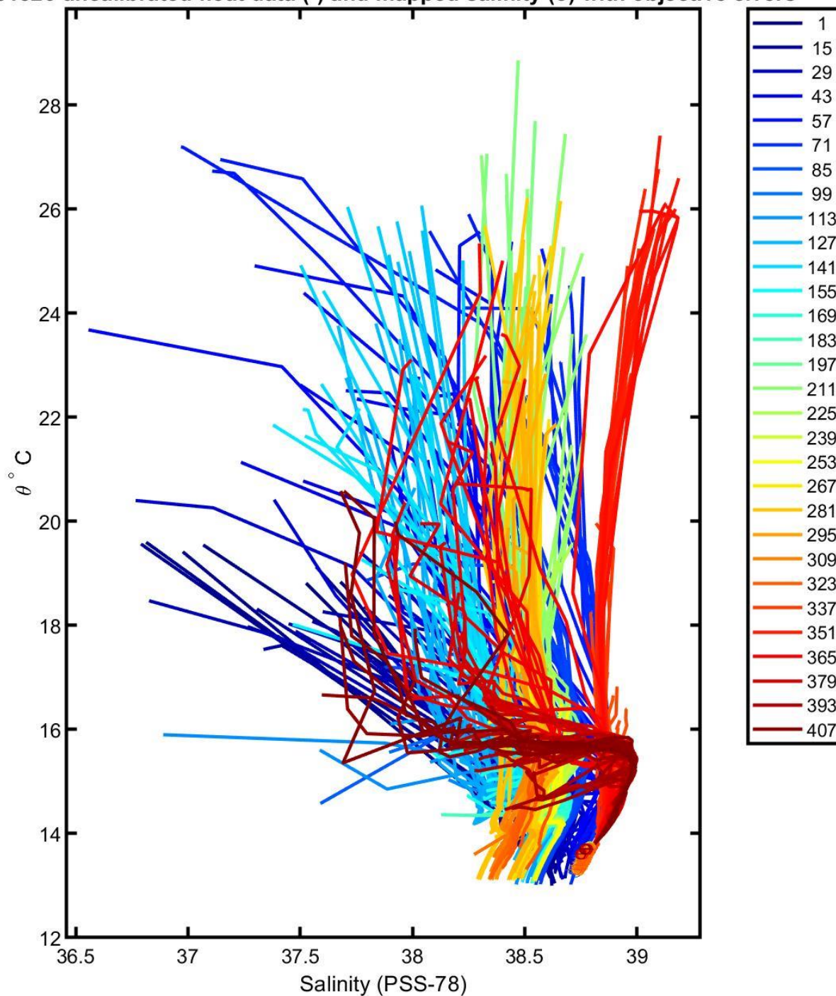
6901826 uncalibrated float data (-) and mapped salinity (o) with objective errors
