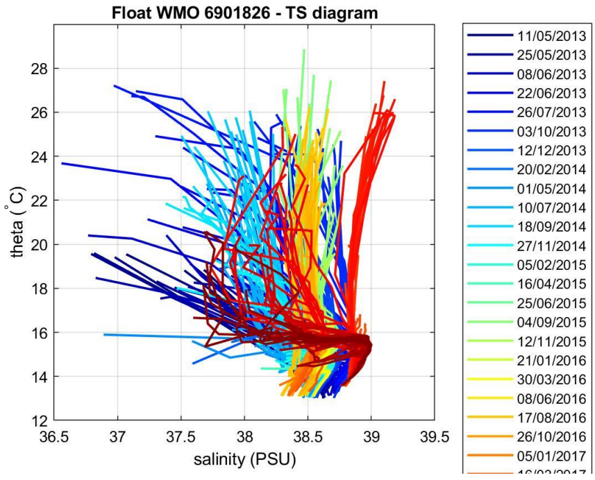
Figure 4: Float 6901826. \theta -S diagram color-coded per cycle number.
