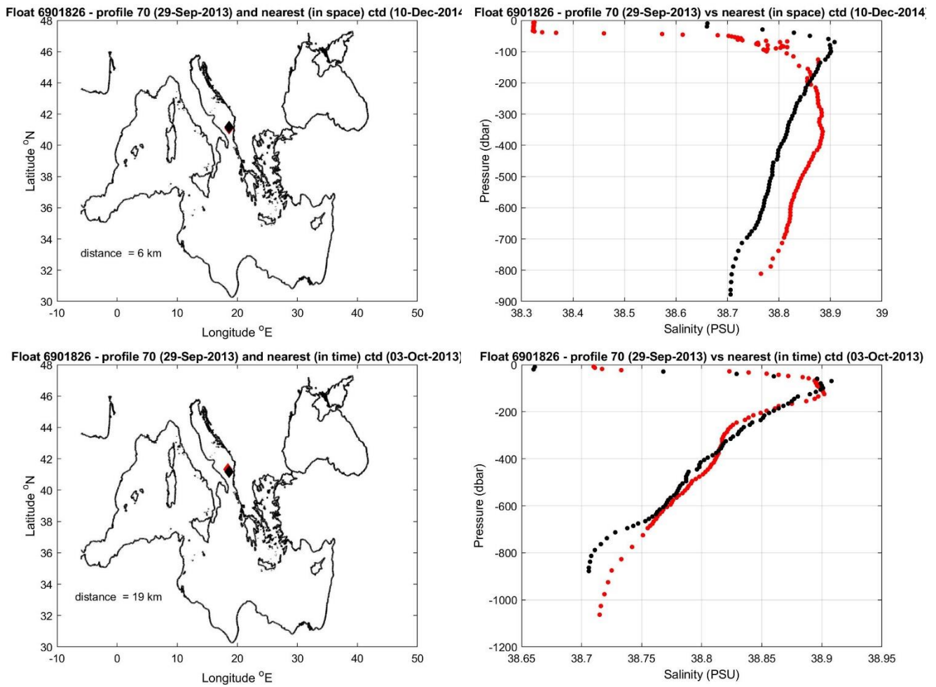
Figure 9: Float 6901826. The salinity float profile number 70 (black dots) are compared to the nearest in space (top) and in time (bottom) reference profile (red dots). The locations of the two profiles and their distance is given in the left panel.
