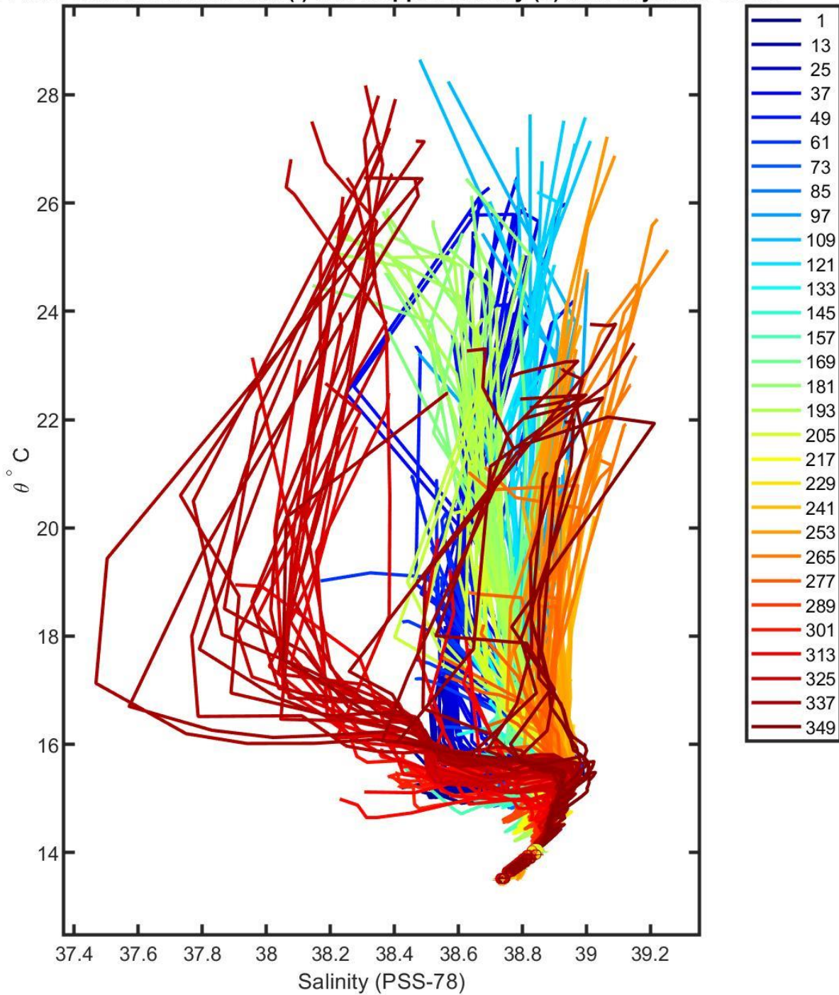
6901829 calibrated float data (-) and mapped salinity (o) with objective errors
