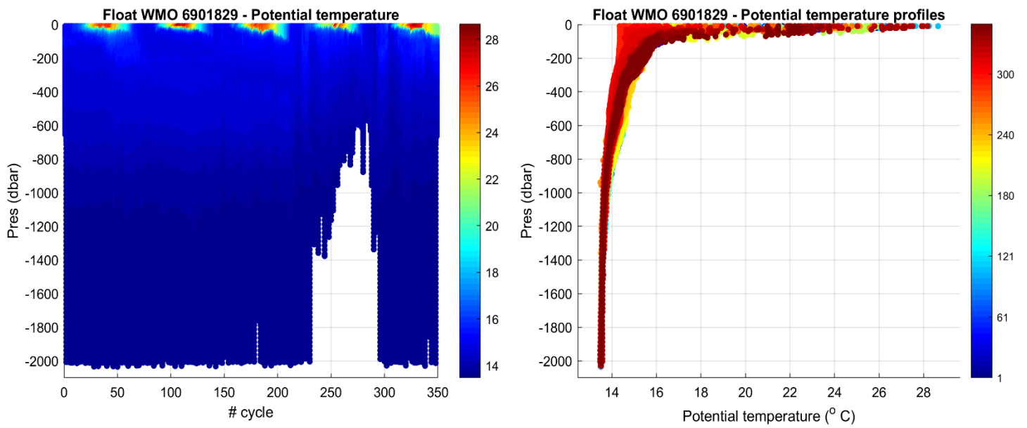
Figure 2: Float 6901829. Time series of Argo float potential temperature ( ^{\circ}\text{C} ) on the left, and potential temperature profiles color-coded per cycle number on the right.
