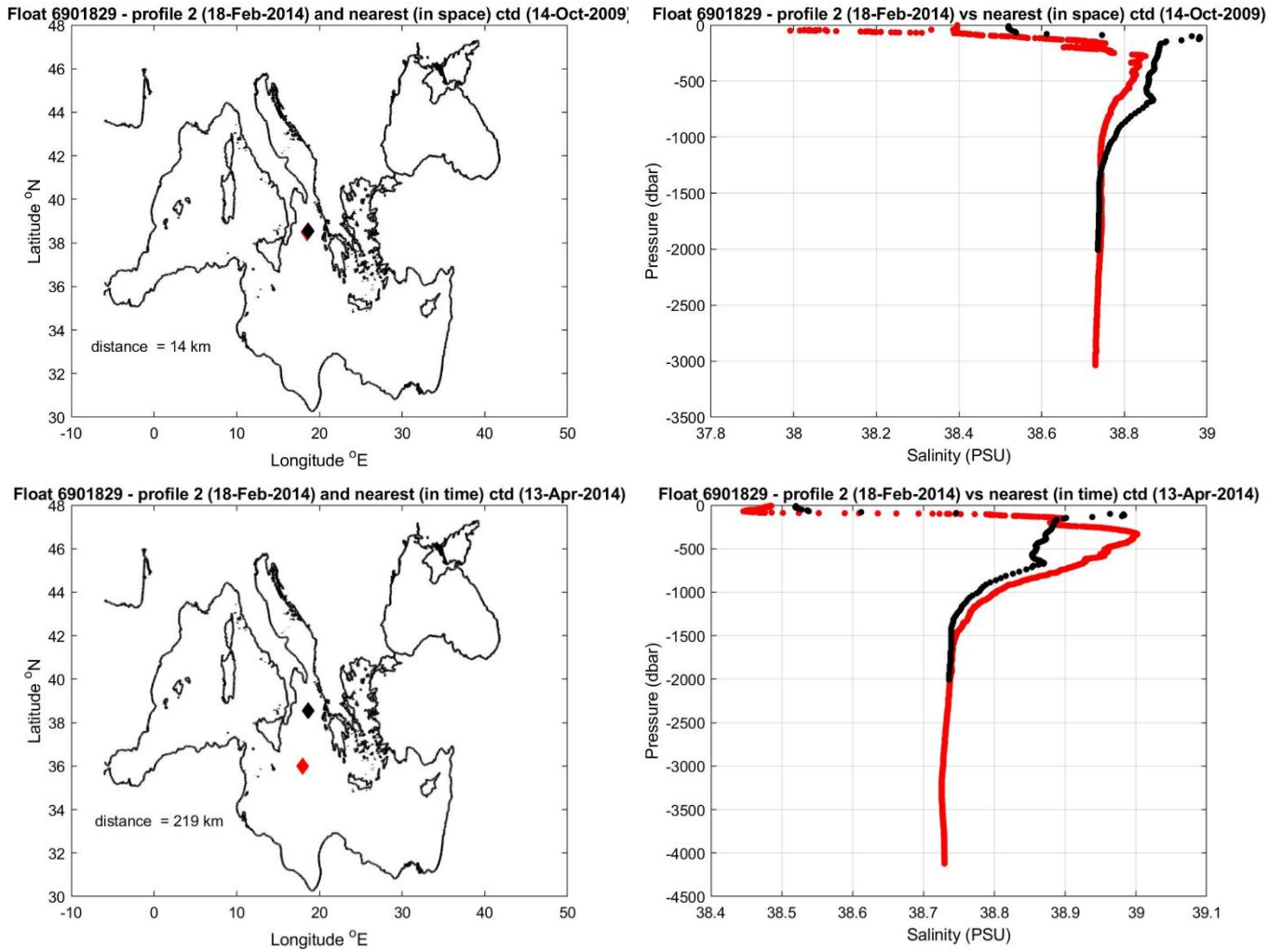
Figure 9: Float 6901829. The salinity float profile number 2 (black dots) are compared to the nearest in space (top) and in time (bottom) reference profile (red dots). The locations of the two profiles and their distance is given in the left panel.
