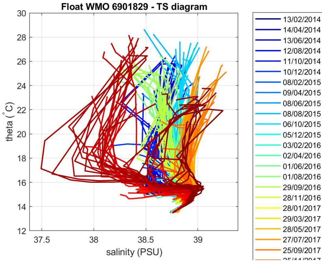
Figure 4: Float 6901829. \theta -S diagram color-coded per cycle number.
