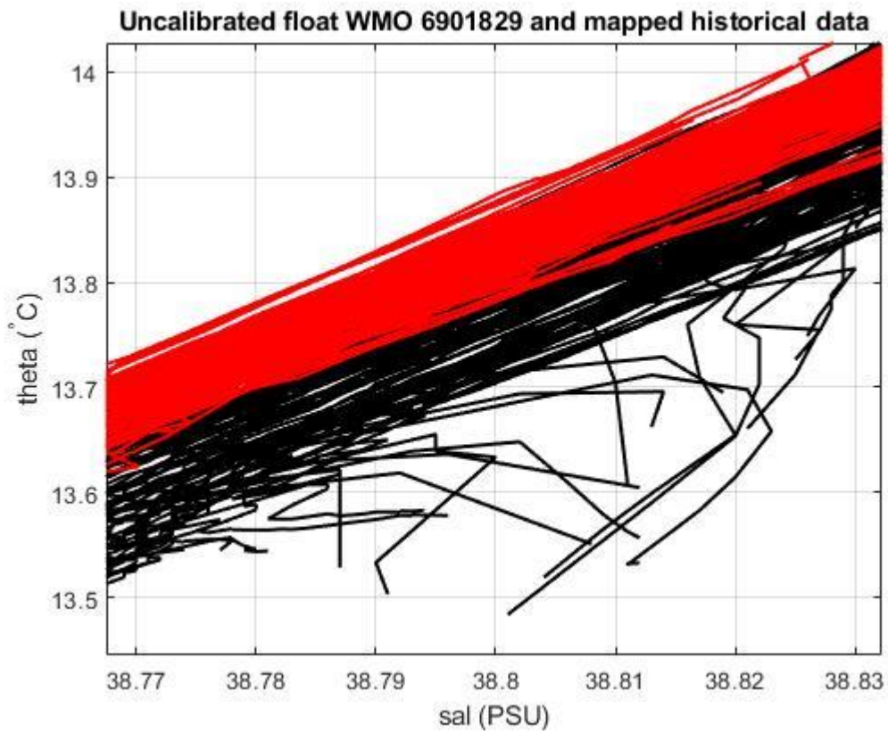
Figure 19: Float 6901829. Uncalibrated float salinity profile (black lines) and mapped historical data (red lines) in the most uniform part of the \theta -S curve.
