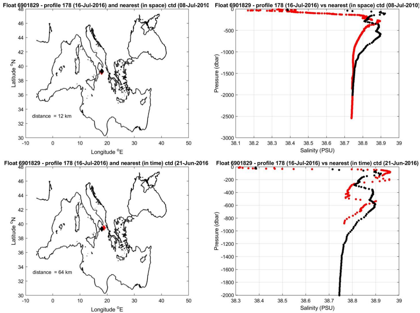
Figure 10: Float 6901829. The salinity float profile number 178 (black dots) are compared to the nearest in space (top) and in time (bottom) reference profile (red dots). The locations of the two profiles and their distance is given in the left panel.
