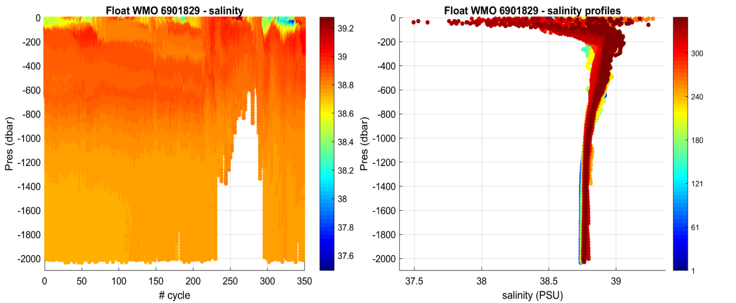
Figure 3: Float 6901829. Time series of Argo float potential salinity (PSS-78) on the left, and salinity profiles color-coded per cycle number on the right.
