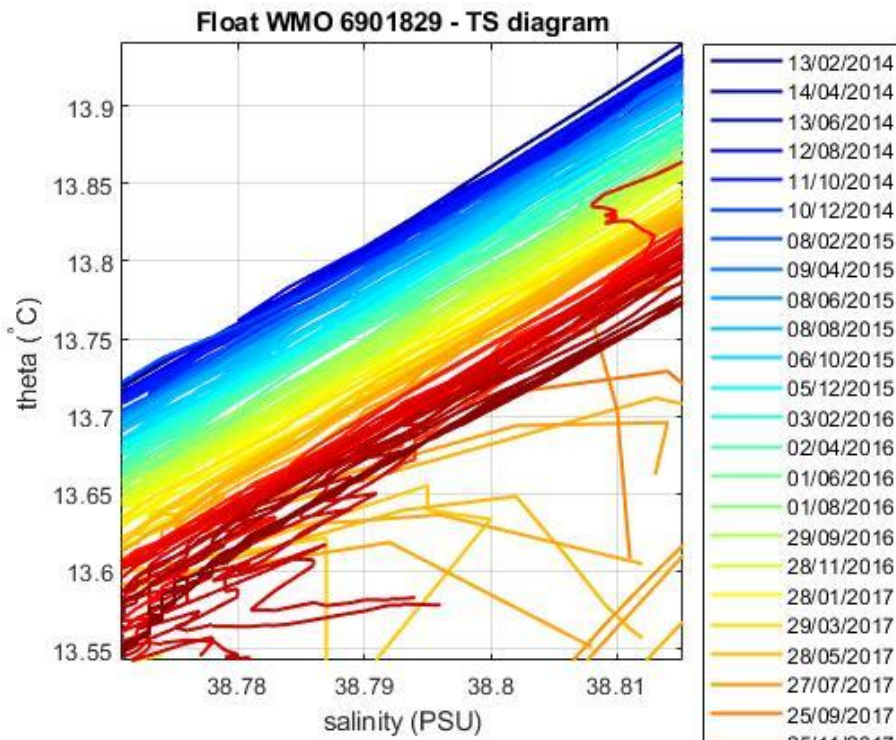
Figure 5: Float 6901829. Area of the \theta -S diagram (color-coded per cycle number) where the \theta -S relationship is more uniform.
