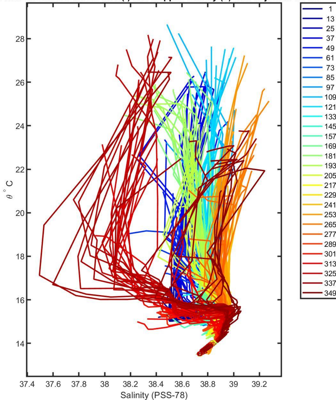
6901829 uncalibrated float data (-) and mapped salinity (o) with objective errors
