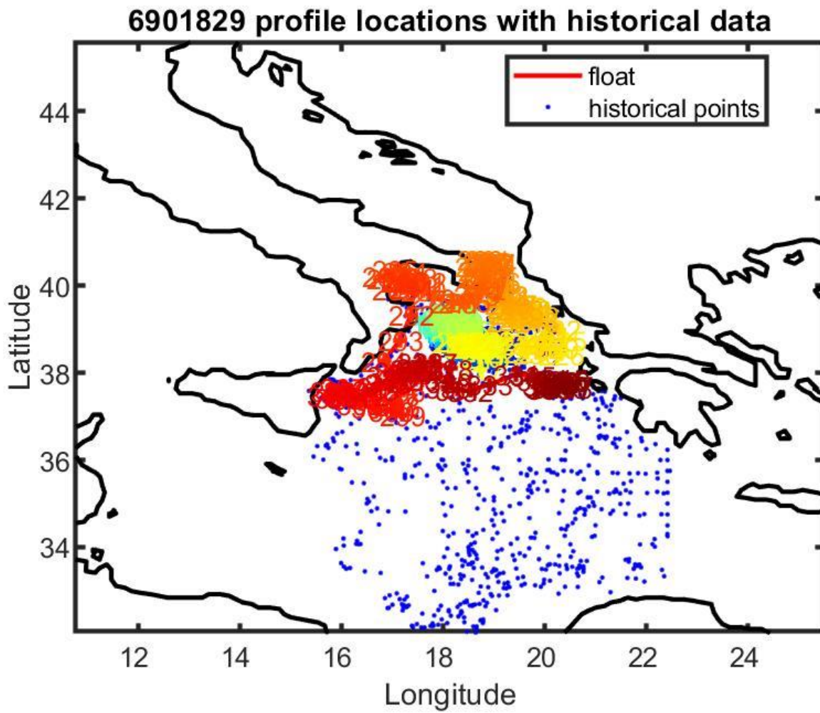
Figure 13: Float 6901829. Location of the float profiles (red line with colored numbers) and the reference data selected for mapping (blue dots).
