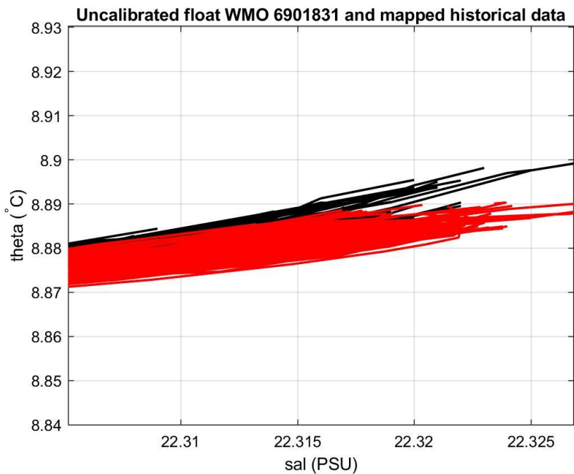
Figure 19: Float 6901831. Uncalibrated float salinity profile (black lines) and mapped historical data (red lines) in the most uniform part of the \theta -S curve.
