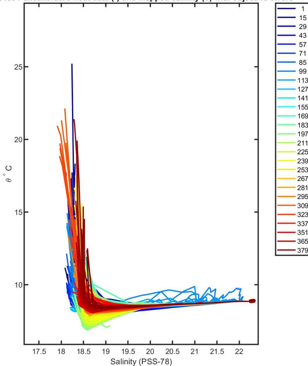
6901831 uncalibrated float data (-) and mapped salinity (o) with objective errors
