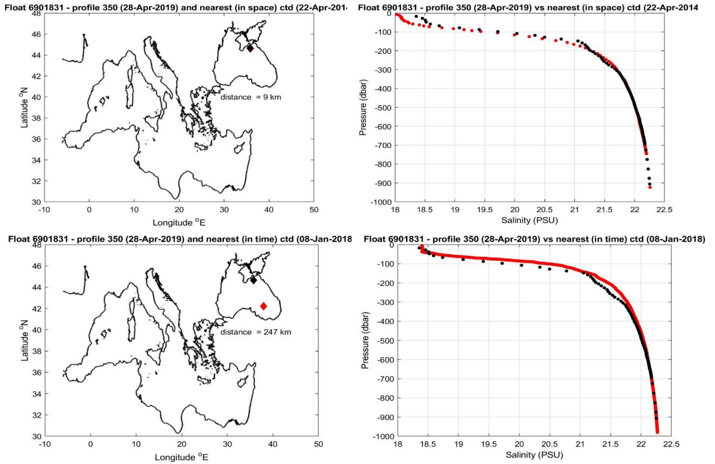
Figure 11: Float 6901831. The salinity float profile number 350 (black dots) are compared to the nearest in space (top) and in time (bottom) reference profile (red dots). The locations of the two profiles and their distance is given in the left panel.
