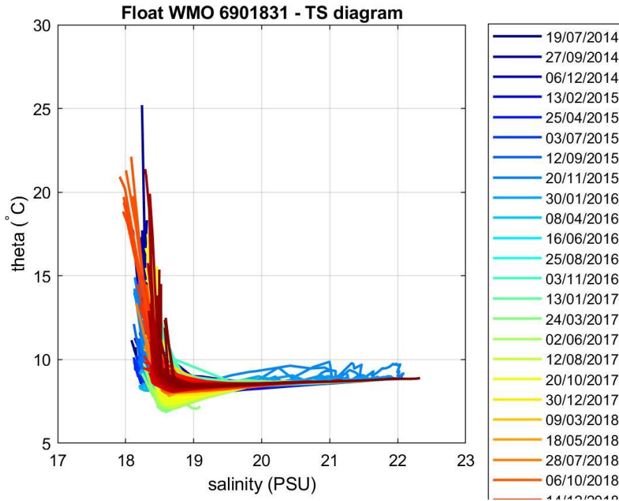
Figure 4: Float 6901831. \theta -S diagram color-coded per cycle number.
