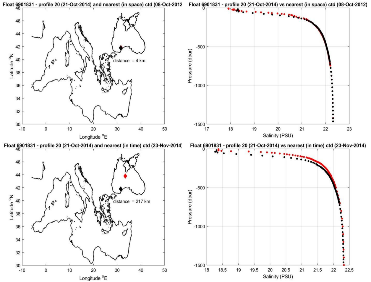
Figure 9: Float 6901831. The salinity float profile number 20 (black dots) are compared to the nearest in space (top) and in time (bottom) reference profile (red dots). The locations of the two profiles and their distance is given in the left panel.
