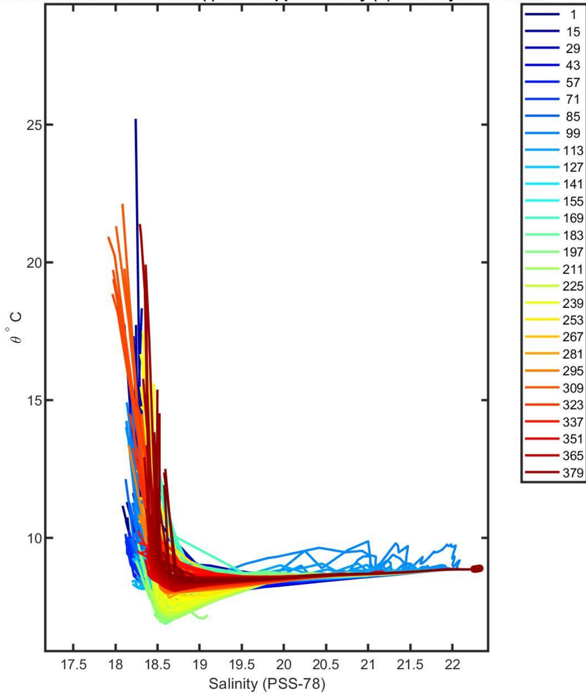
6901831 calibrated float data (-) and mapped salinity (o) with objective errors
