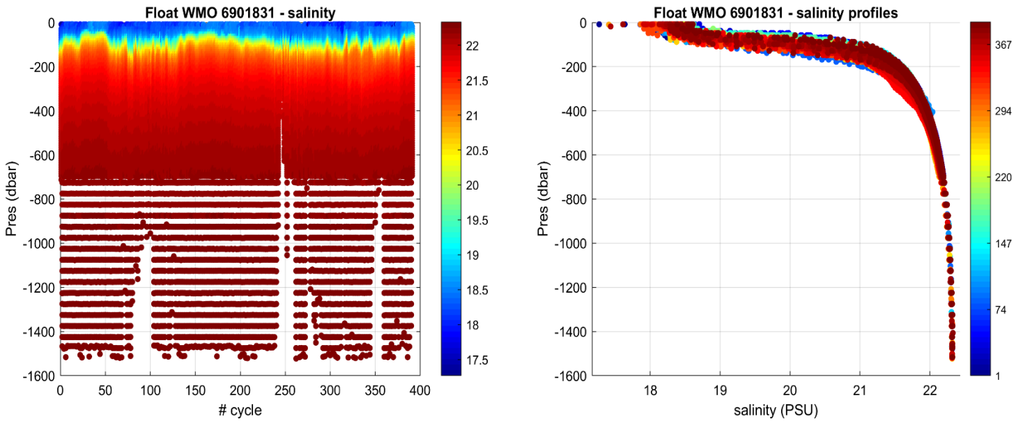
Figure 3: Float 6901831. Time series of Argo float potential salinity (PSS-78) on the left, and salinity profiles color-coded per cycle number on the right.
