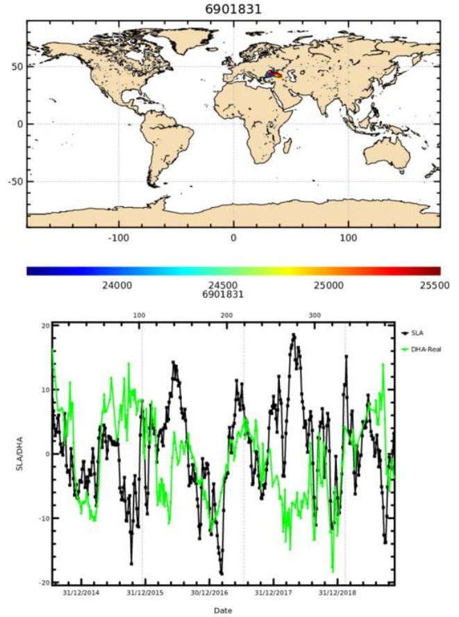
Figure 1: Float 6901831. The comparison between the sea surface height (SSH) from the satellite altimetry and dynamic height anomaly (DHA) extracted from the Argo float temperature and salinity. The figure is created by the CLS/Coriolis and distributed by Ifremer ( ftp://ftp.ifremer.fr/ifremer/argo/etc/argo-ast9-item13-AltimeterComparison/figures/ ).
