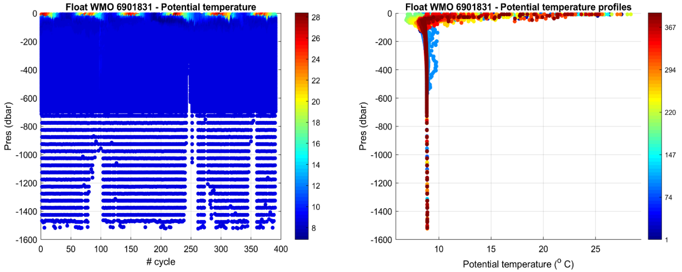
Figure 2: Float 6901831. Time series of Argo float potential temperature ( ^{\circ}\text{C} ) on the left, and potential temperature profiles color-coded per cycle number on the right.
