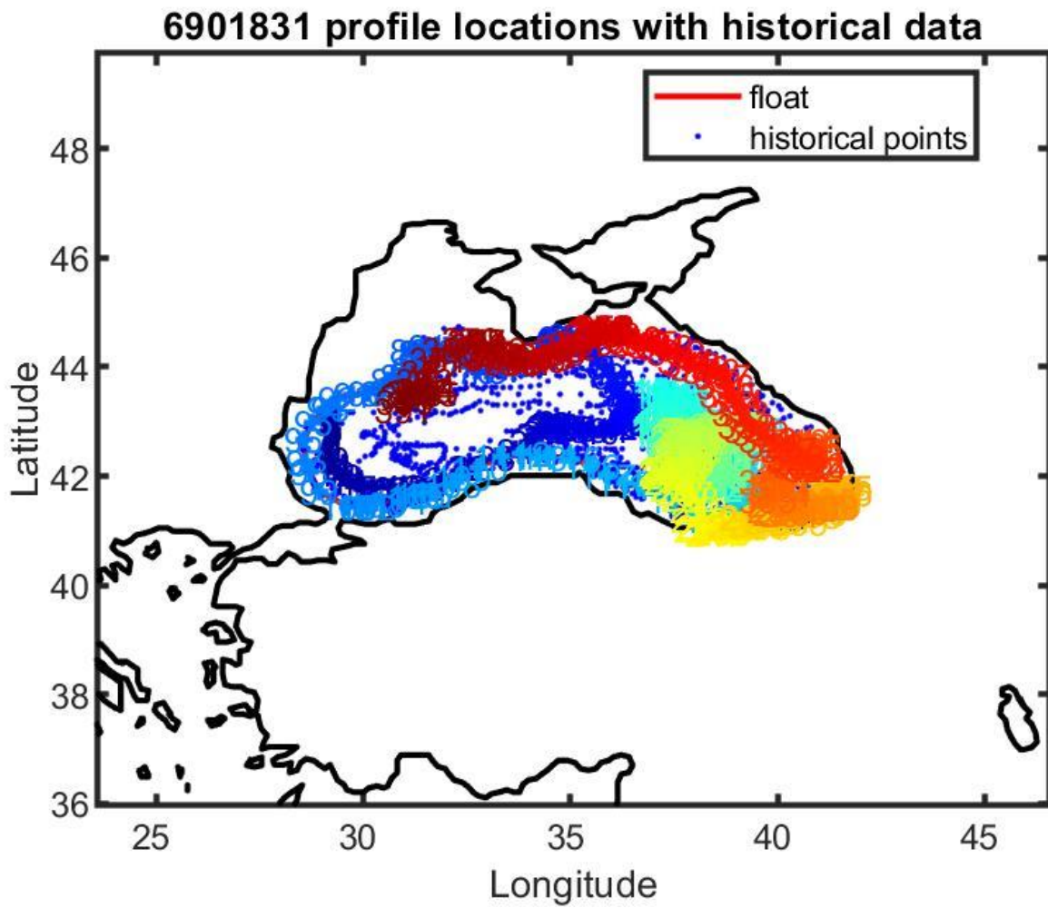
Figure 13: Float 6901831. Location of the float profiles (red line with colored numbers) and the reference data selected for mapping (blue dots).
