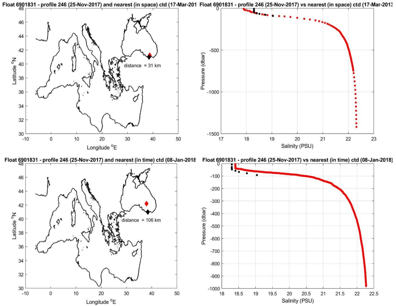
Figure 10: Float 6901831. The salinity float profile number 246 (black dots) are compared to the nearest in space (top) and in time (bottom) reference profile (red dots). The locations of the two profiles and their distance is given in the left panel.
