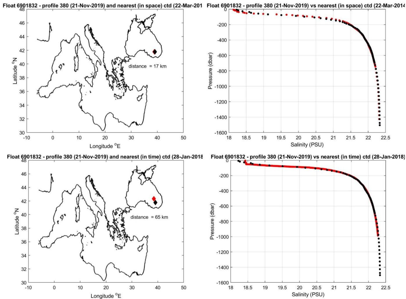
Figure 11: Float 6901832. The salinity float profile number 380 (black dots) are compared to the nearest in space (top) and in time (bottom) reference profile (red dots). The locations of the two profiles and their distance is given in the left panel.
