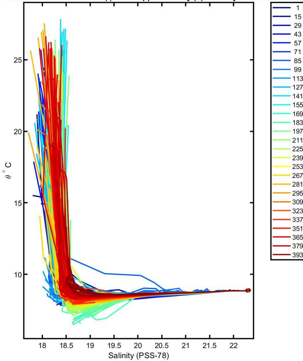
6901832 calibrated float data (-) and mapped salinity (o) with objective errors
