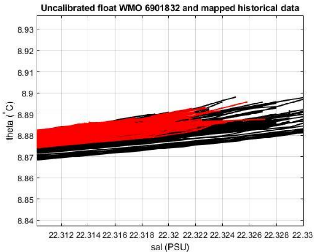
Figure 19: Float 6901832. Uncalibrated float salinity profile (black lines) and mapped historical data (red lines) in the most uniform part of the \theta -S curve.
