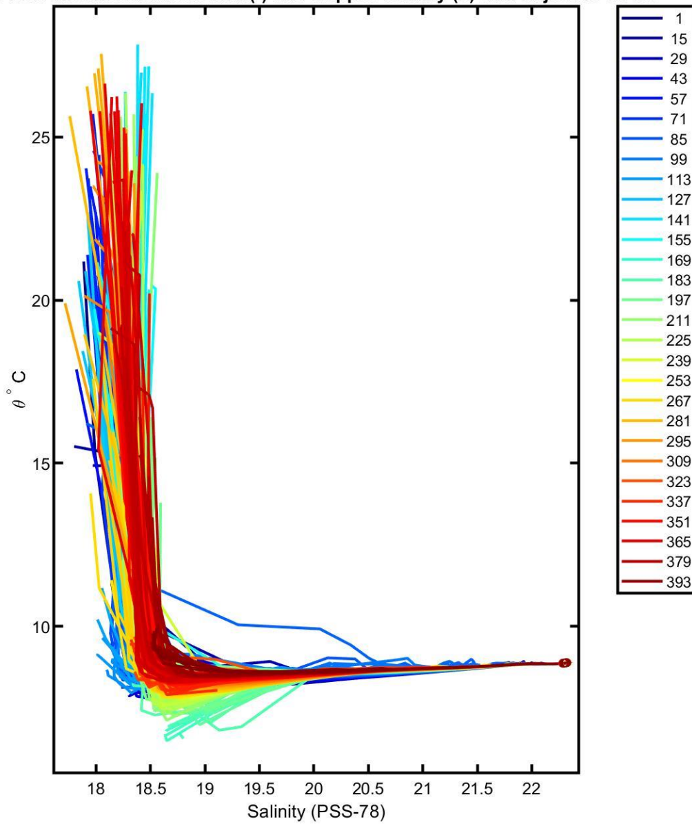
6901832 uncalibrated float data (-) and mapped salinity (o) with objective errors
