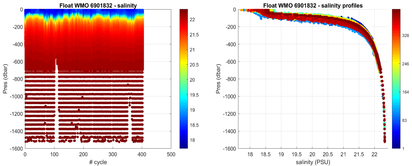
Figure 3: Float 6901832. Time series of Argo float potential salinity (PSS-78) on the left, and salinity profiles color-coded per cycle number on the right.
