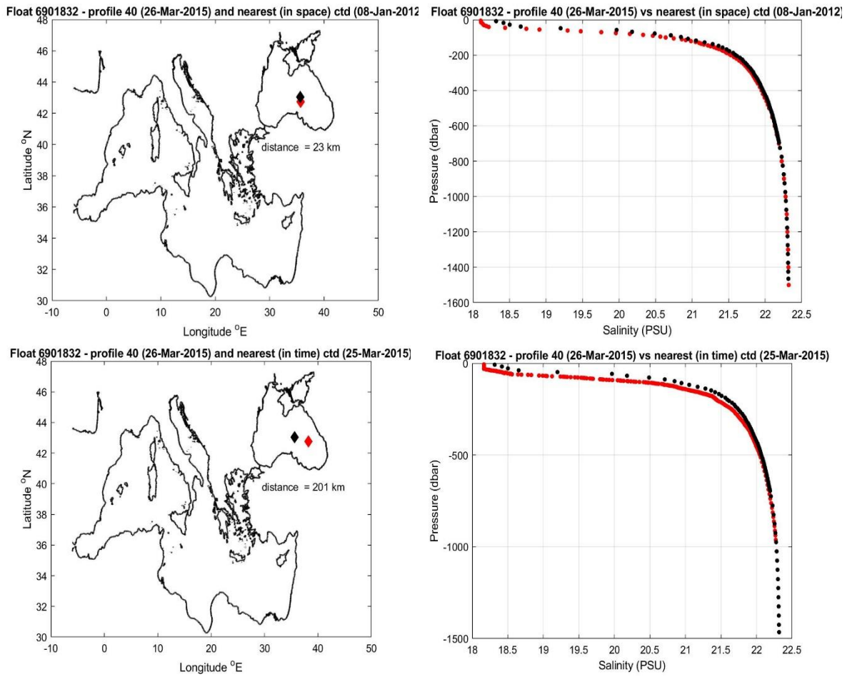
Figure 9: Float 6901832. The salinity float profile number 40 (black dots) are compared to the nearest in space (top) and in time (bottom) reference profile (red dots). The locations of the two profiles and their distance is given in the left panel.
