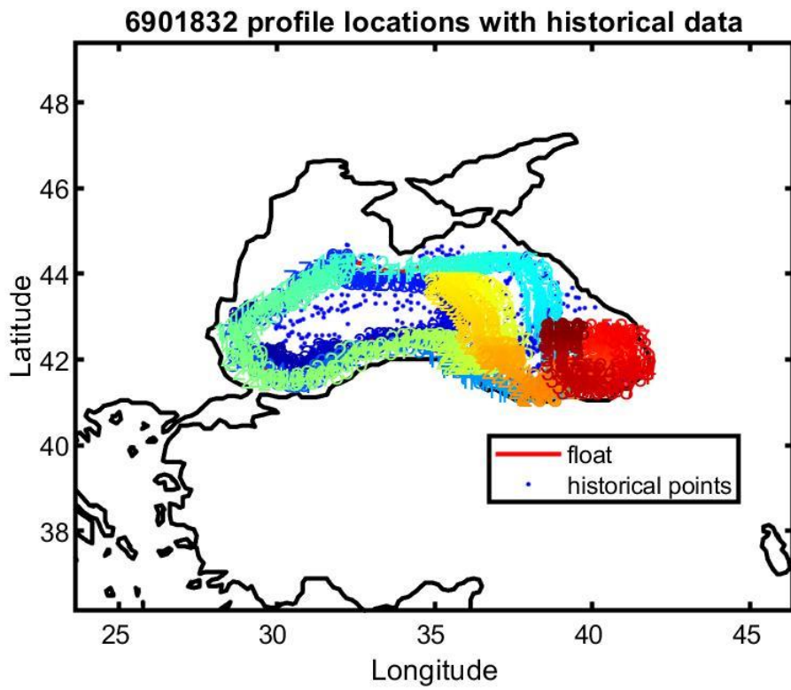
Figure 13: Float 6901832. Location of the float profiles (red line with colored numbers) and the reference data selected for mapping (blue dots).
