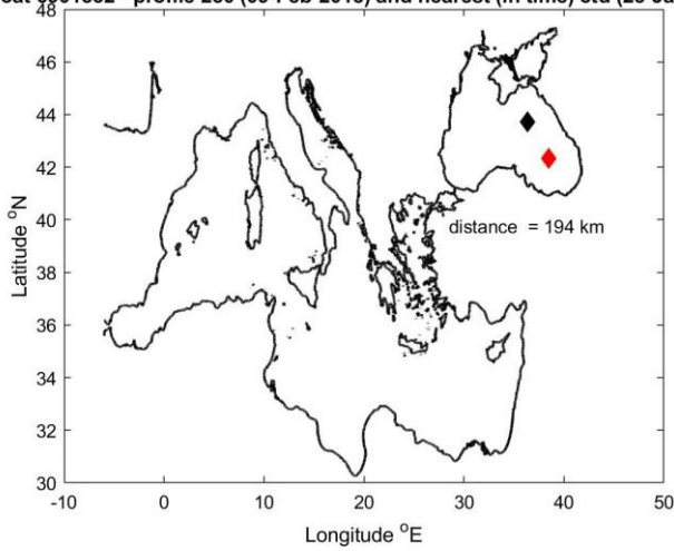
Float 6901832 - profile 250 (09-Feb-2018) and nearest (in time) ctd (28-Jan-2018)
