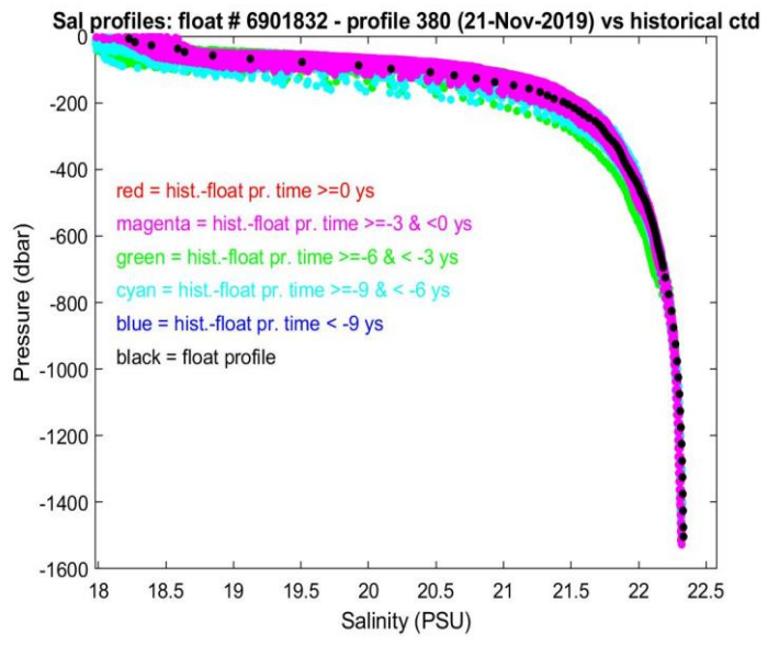
Figure 8: Float 6901832. Locations of the salinity float profile number 380 and historical CTD data (right panel) and the respective salinity profiles (left panel).
