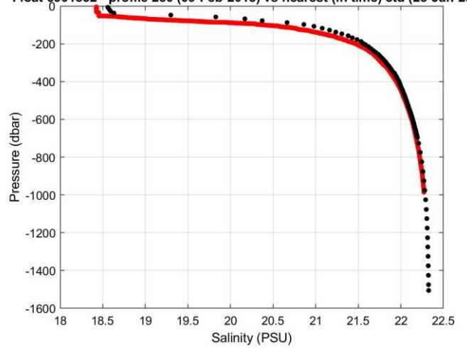
Float 6901832 - profile 250 (09-Feb-2018) vs nearest (in time) ctd (28-Jan-2018)
