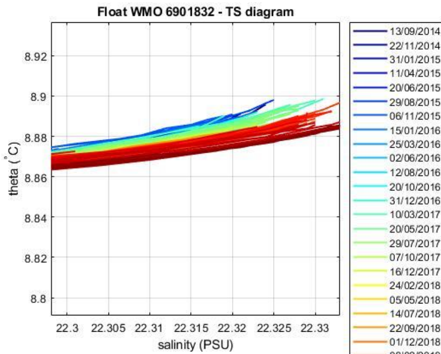
Figure 5: Float 6901832. Area of the \theta -S diagram (color-coded per cycle number) where the \theta -S relationship is more uniform.
