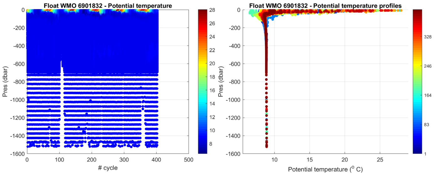
Figure 2: Float 6901832. Time series of Argo float potential temperature ( ^{\circ}\text{C} ) on the left, and potential temperature profiles color-coded per cycle number on the right.
