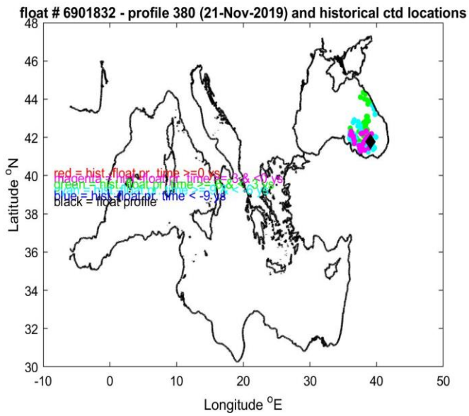
Figure 8: Float 6901832. Locations of the salinity float profile number 380 and historical CTD data (right panel) and the respective salinity profiles (left panel).
