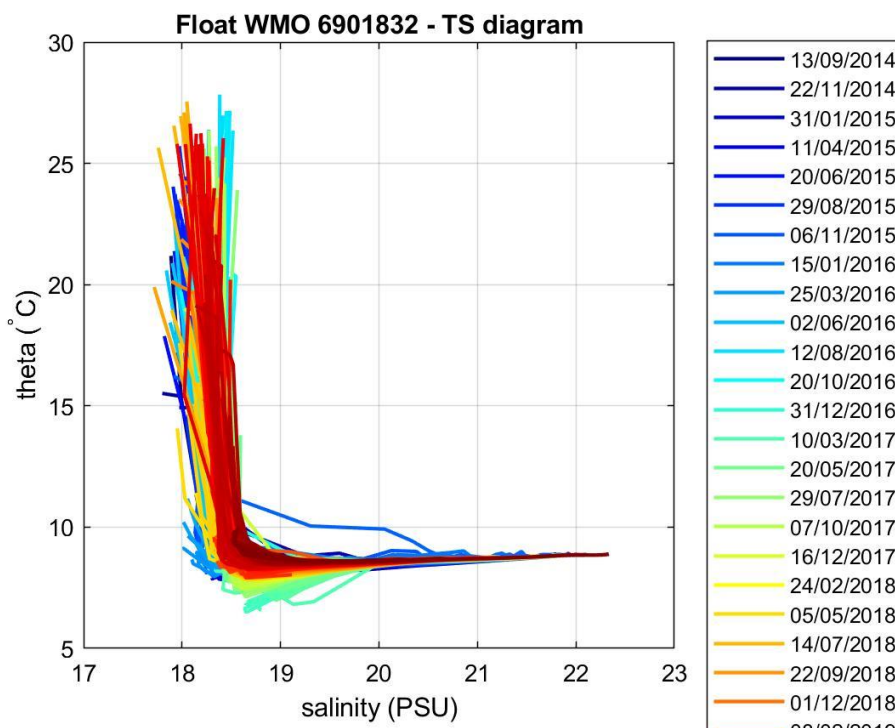
Figure 4: Float 6901832. \theta -S diagram color-coded per cycle number.
