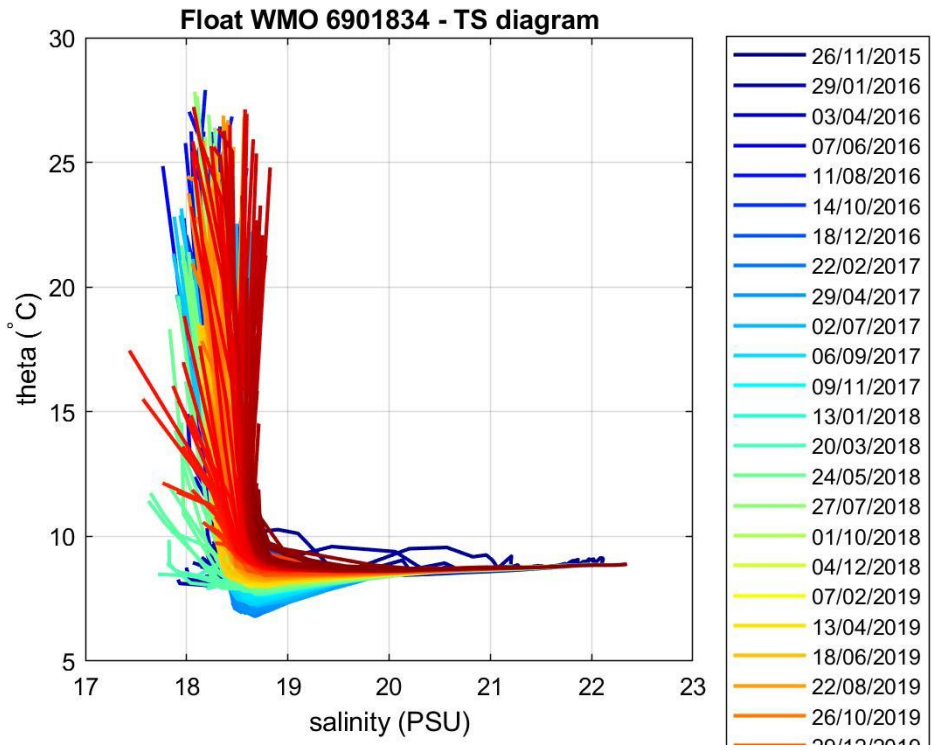
Figure 4: Float 6901834. \theta -S diagram color-coded per cycle number.
