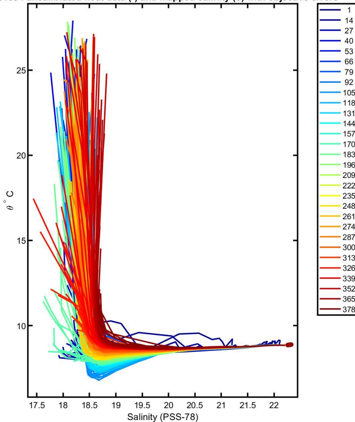
6901834 uncalibrated float data (-) and mapped salinity (o) with objective errors
