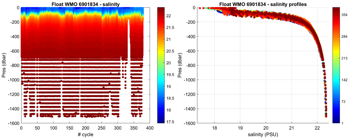
Figure 3: Float 6901834. Time series of Argo float potential salinity (PSS-78) on the left, and salinity profiles color-coded per cycle number on the right.
