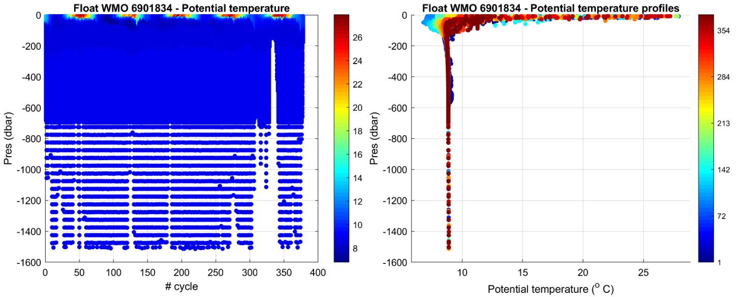
Figure 2: Float 6901834. Time series of Argo float potential temperature ( ^{\circ} C) on the left, and potential temperature profiles color-coded per cycle number on the right.
