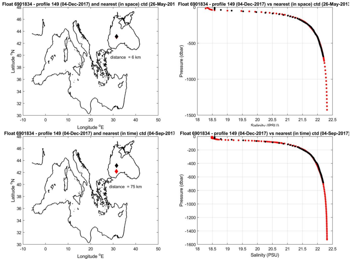
Figure 10: Float 6901834. The salinity float profile number 149 (black dots) are compared to the nearest in space (top) and in time (bottom) reference profile (red dots). The locations of the two profiles and their distance is given in the left panel.
