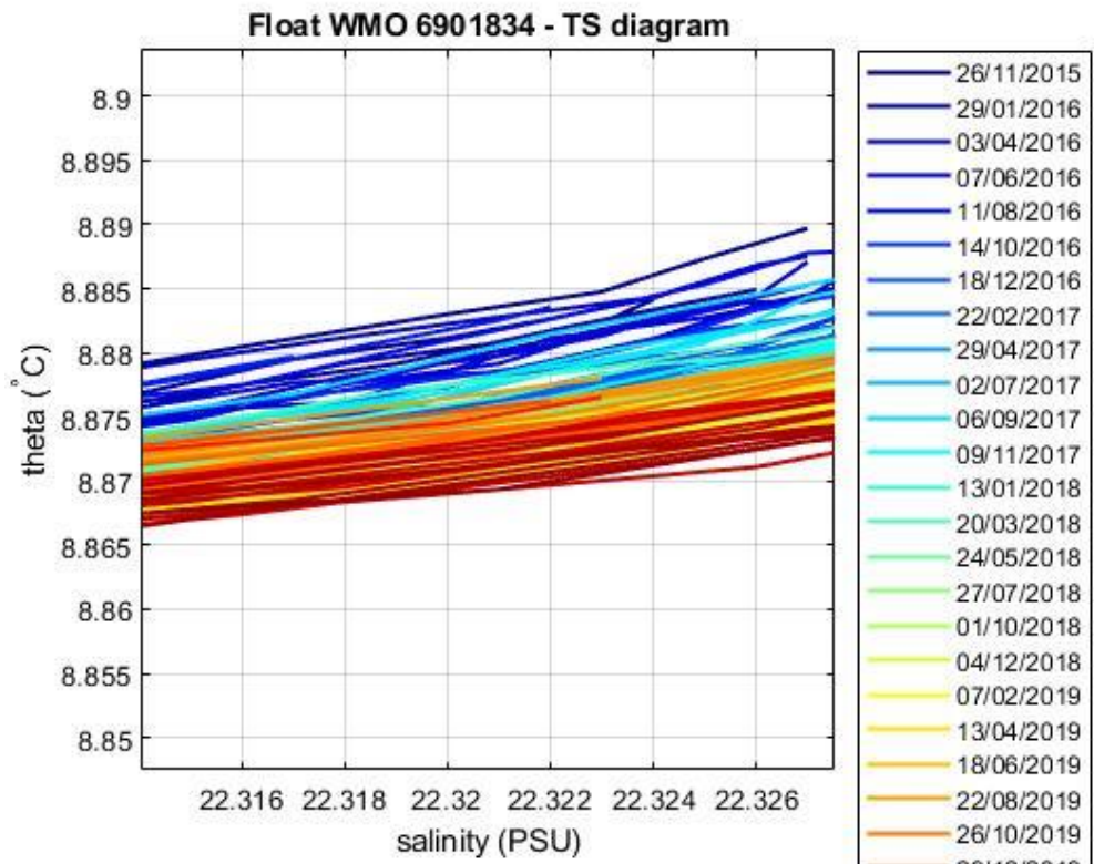
Figure 5: Float 6901834. Area of the \theta -S diagram (color-coded per cycle number) where the \theta -S relationship is more uniform.
