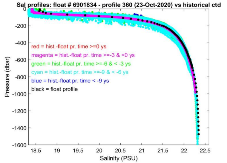
Figure 8: Float 6901834. Locations of the salinity float profile number 360 and historical CTD data (right panel) and the respective salinity profiles (left panel).
