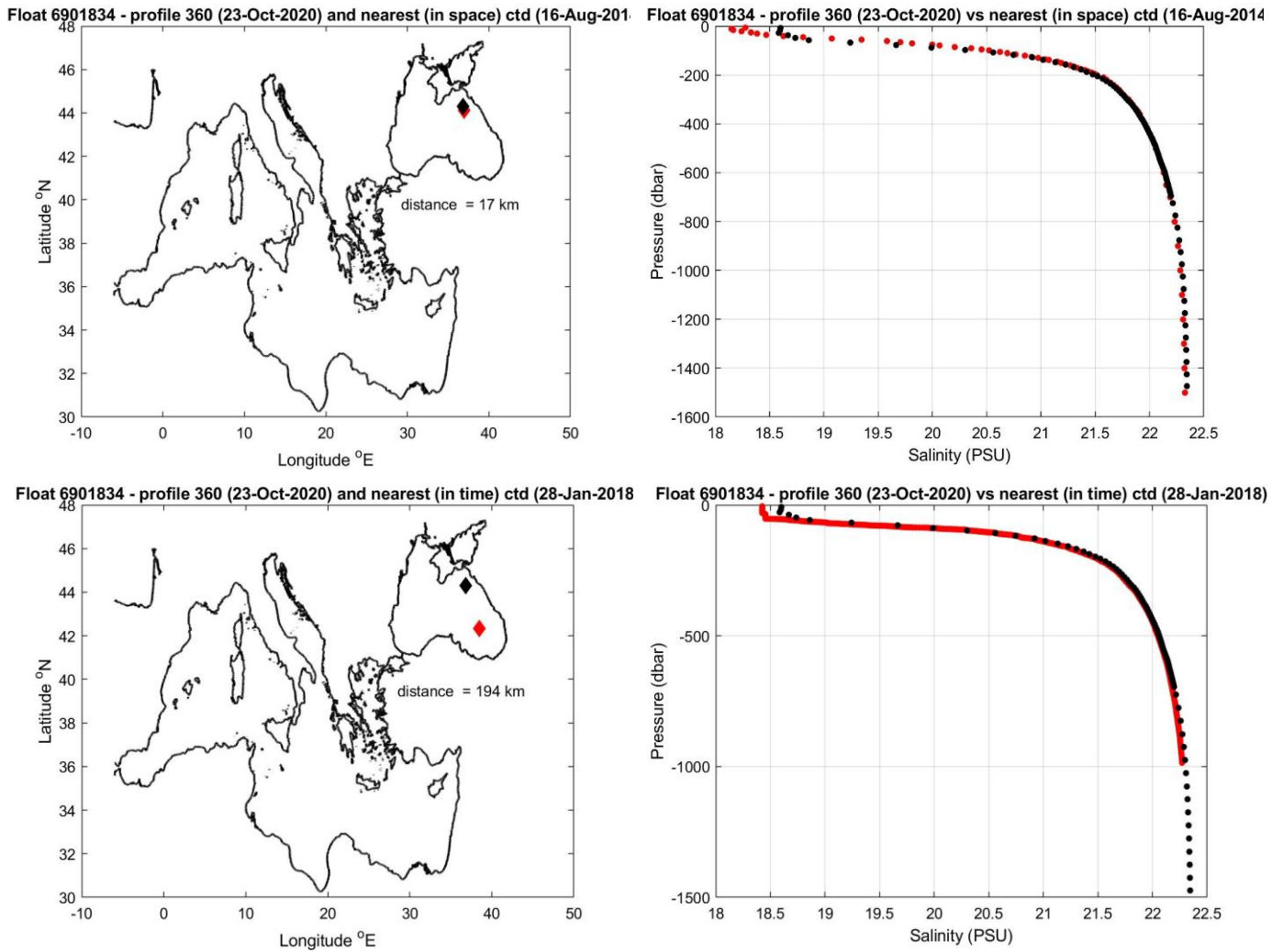
Figure 11: Float 6901834. The salinity float profile number 360 (black dots) are compared to the nearest in space (top) and in time (bottom) reference profile (red dots). The locations of the two profiles and their distance is given in the left panel.
