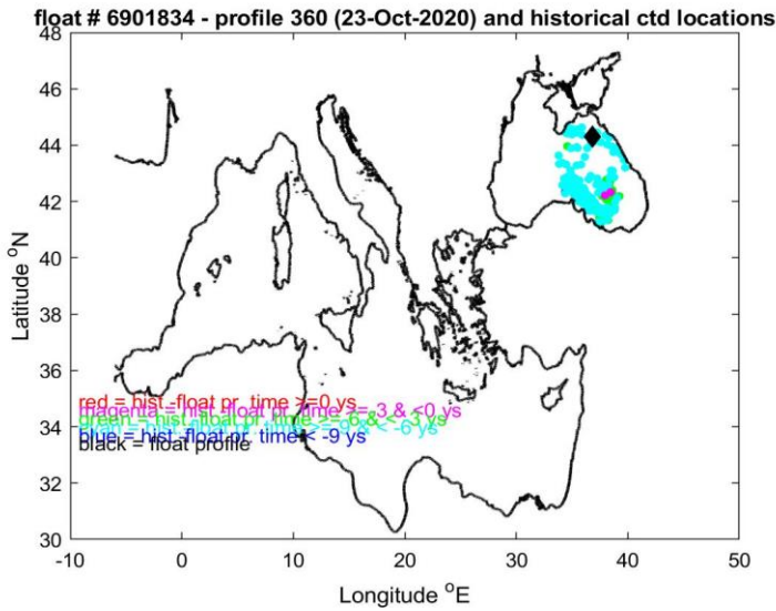
Figure 8: Float 6901834. Locations of the salinity float profile number 360 and historical CTD data (right panel) and the respective salinity profiles (left panel).
