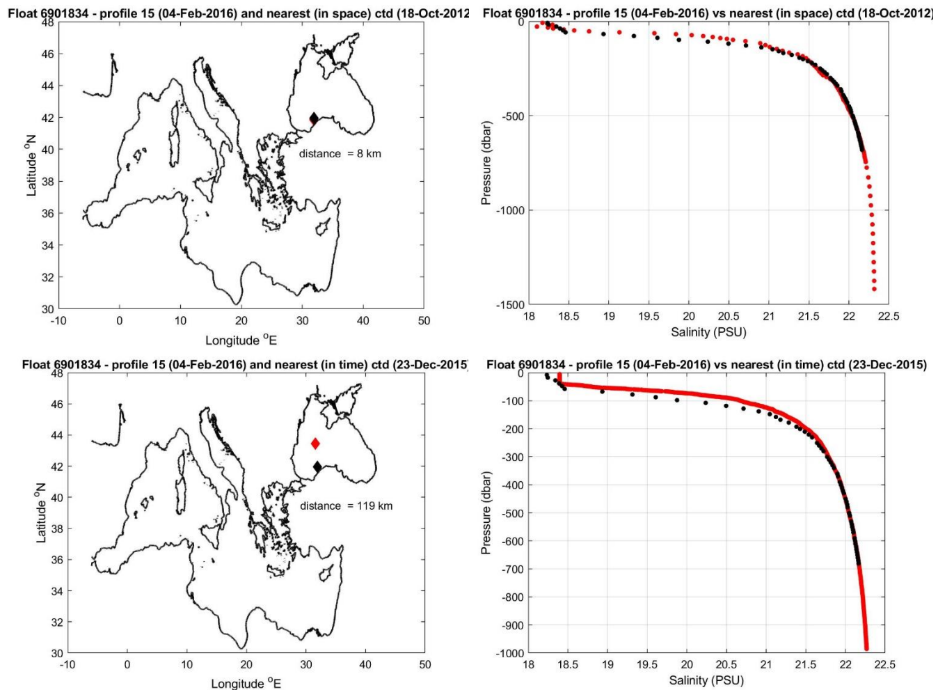
Figure 9: Float 6901834. The salinity float profile number 15 (black dots) are compared to the nearest in space (top) and in time (bottom) reference profile (red dots). The locations of the two profiles and their distance is given in the left panel.
