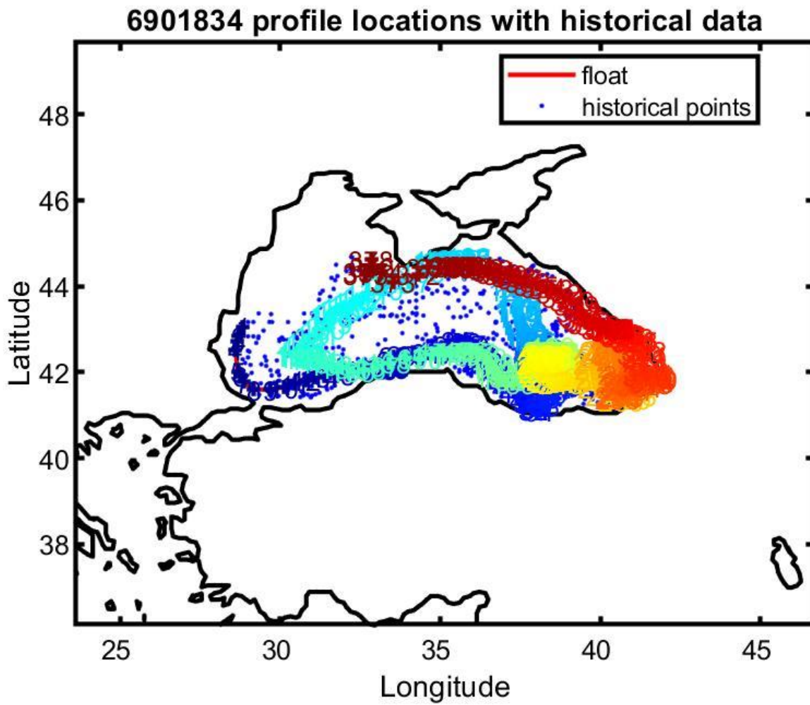
Figure 13: Float 6901834. Location of the float profiles (red line with colored numbers) and the reference data selected for mapping (blue dots).
