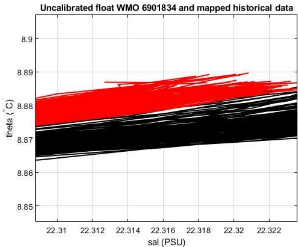
Figure 19: Float 6901834. Uncalibrated float salinity profile (black lines) and mapped historical data (red lines) in the most uniform part of the \theta -S curve.
