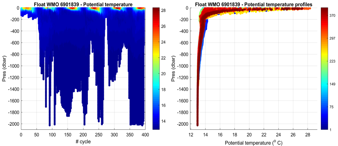
Figure 1: Float 6901839. Time series of Argo float potential temperature ( ^{\circ}\text{C} ) on the left, and potential temperature profiles color-coded per cycle number on the right.
