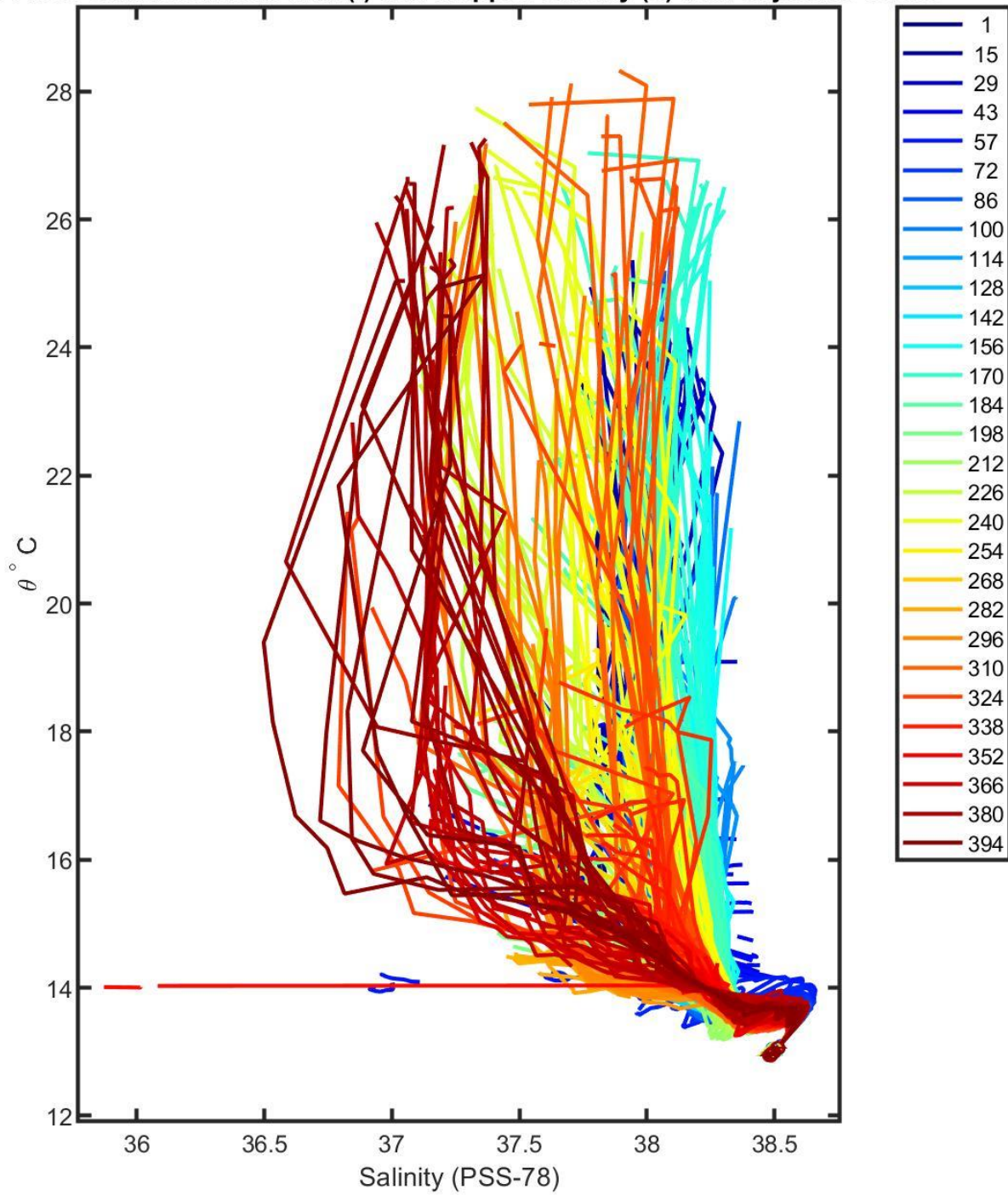
6901839 calibrated float data (-) and mapped salinity (o) with objective errors
