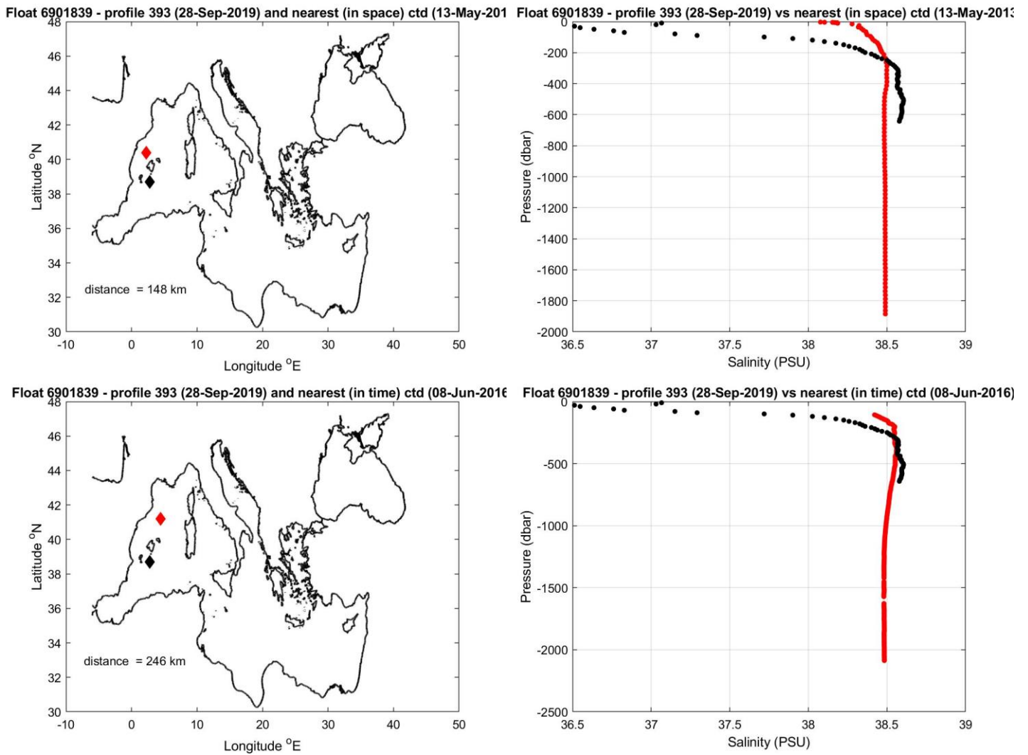
Figure 10: Float 6901839. The salinity float profile number 393 (black dots) are compared to the nearest in space (top) and in time (bottom) reference profile (red dots). The locations of the two profiles and their distance is given in the left panel.
