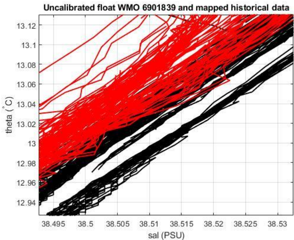
Figure 18: Float 6901839. Uncalibrated float salinity profile (black lines) and mapped historical data (red lines) in the most uniform part of the \theta -S curve.
