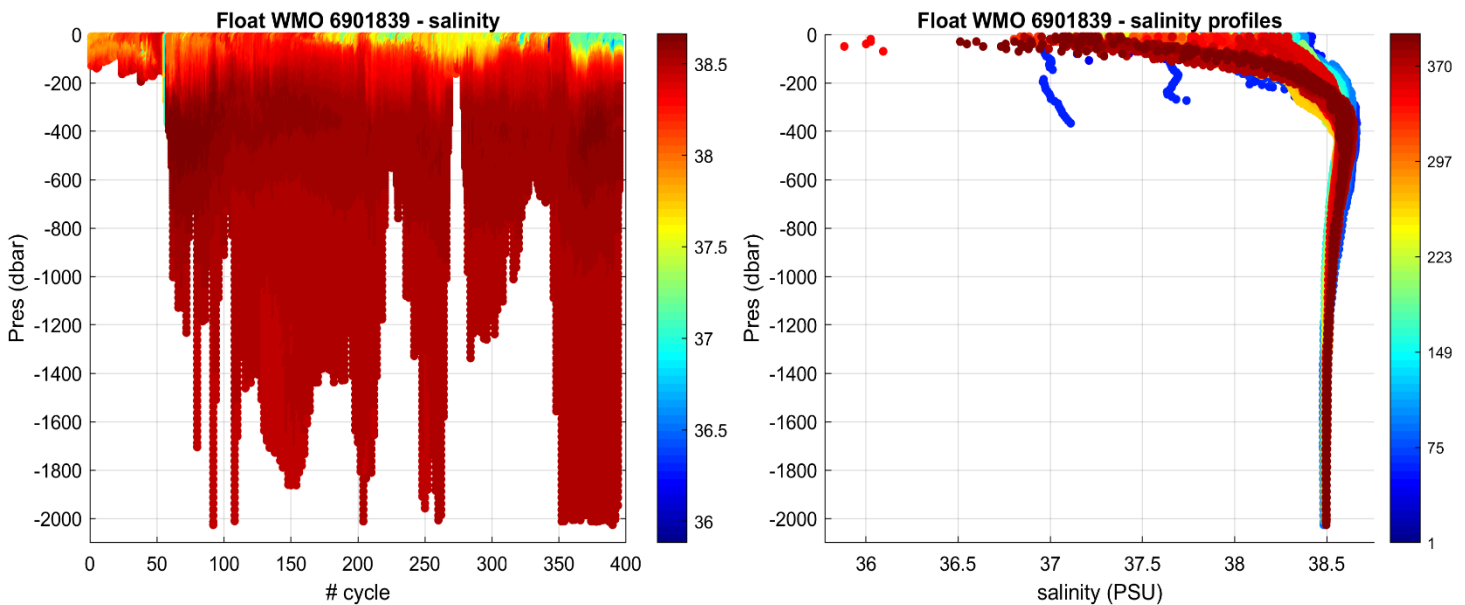
Figure 2: Float 6901839. Time series of Argo float potential salinity (PSS-78) on the left, and salinity profiles color-coded per cycle number on the right.
