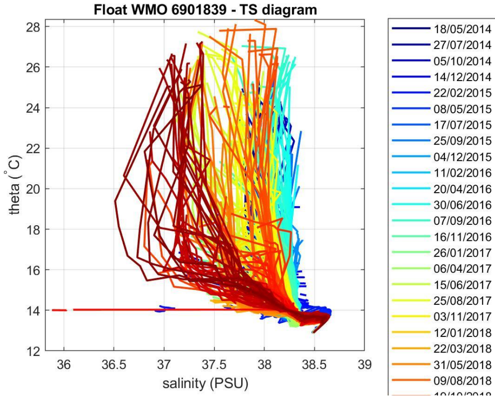
Figure 3: Float 6901839. \theta -S diagram color-coded per cycle number.
