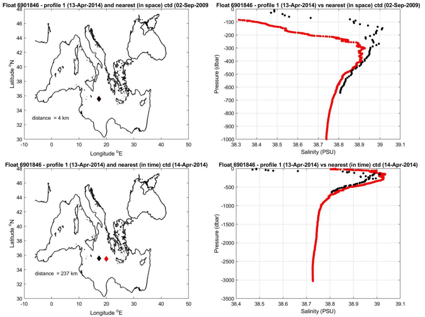
Figure 9: Float 6901846. The salinity float profile number 1 (black dots) are compared to the nearest in space (top) and in time (bottom) reference profile (red dots). The locations of the two profiles and their distance is given in the left panel.
