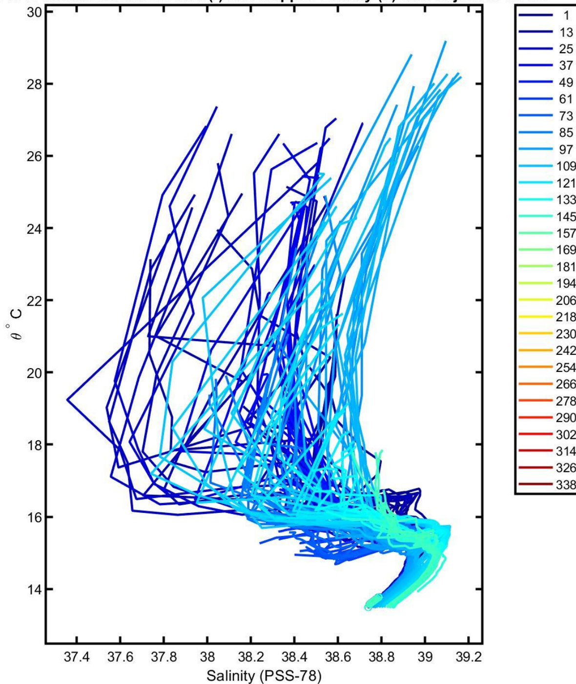
6901846 uncalibrated float data (-) and mapped salinity (o) with objective errors
