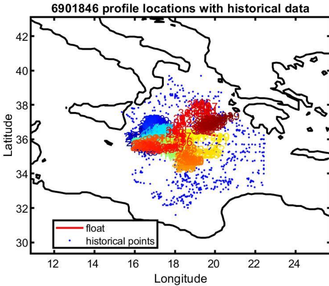
Figure 13: Float 6901846. Location of the float profiles (red line with colored numbers) and the reference data selected for mapping (blue dots).
