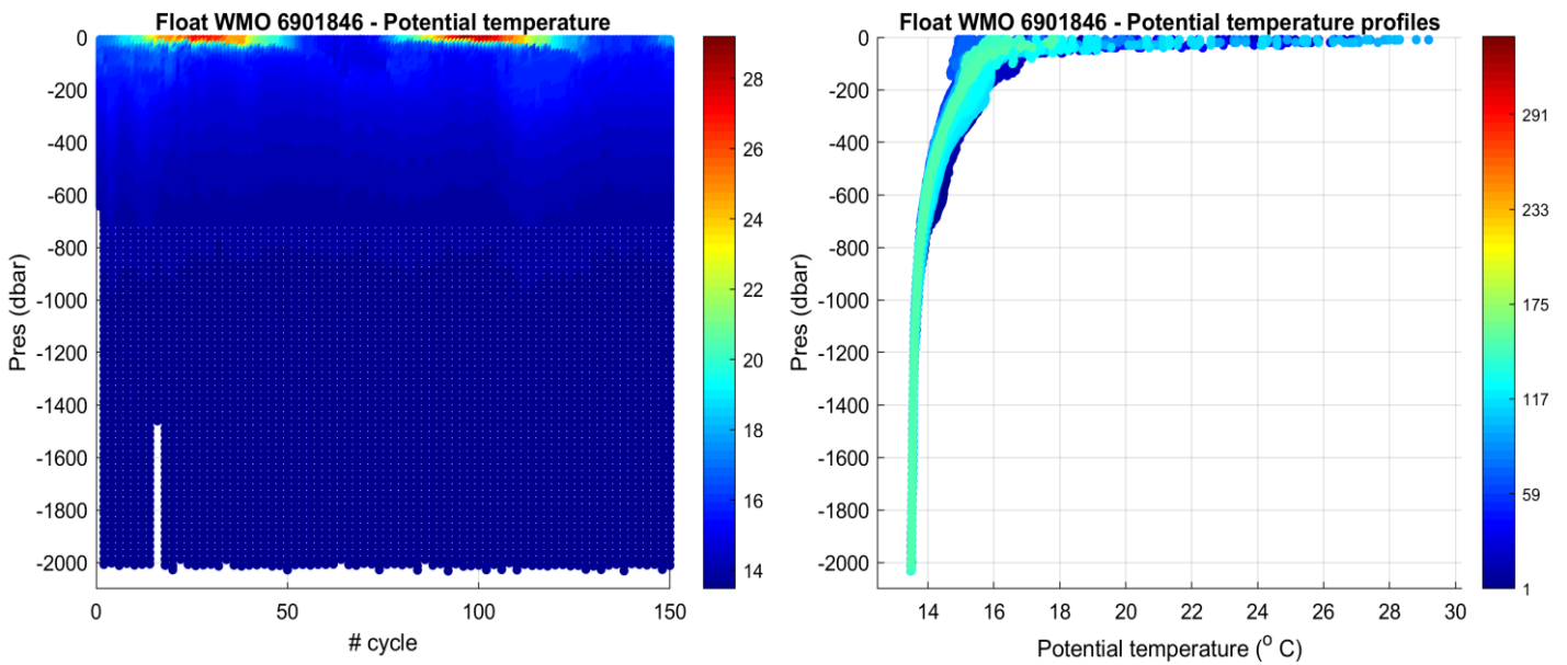
Figure 2: Float 6901846. Time series of Argo float potential temperature ( ^{\circ}\text{C} ) on the left, and potential temperature profiles color-coded per cycle number on the right.
