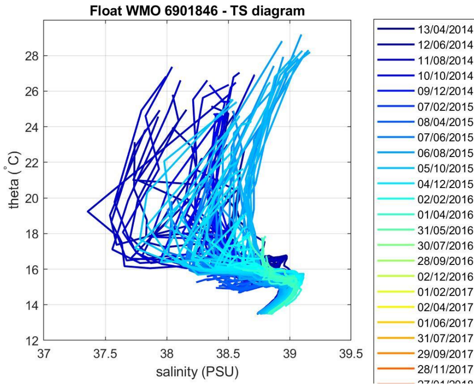
Figure 4: Float 6901846. \theta -S diagram color-coded per cycle number.
