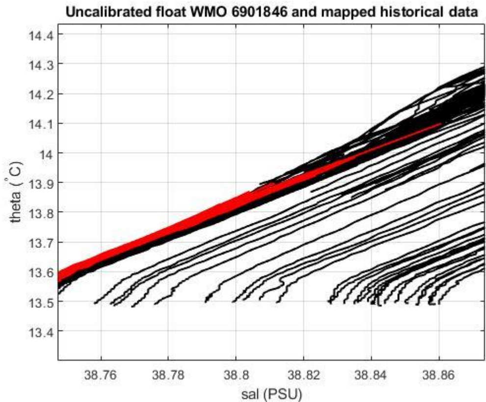
Figure 19: Float 6901846. Uncalibrated float salinity profile (black lines) and mapped historical data (red lines) in the most uniform part of the \theta -S curve.
