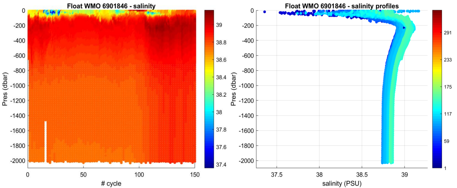
Figure 3: Float 6901846. Time series of Argo float potential salinity (PSS-78) on the left, and salinity profiles color-coded per cycle number on the right.
