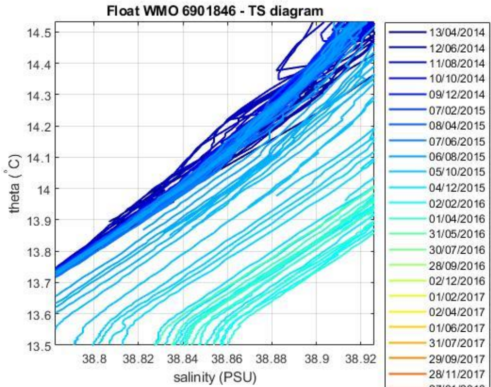
Figure 5: Float 6901846. Area of the \theta -S diagram (color-coded per cycle number) where the \theta -S relationship is more uniform.
