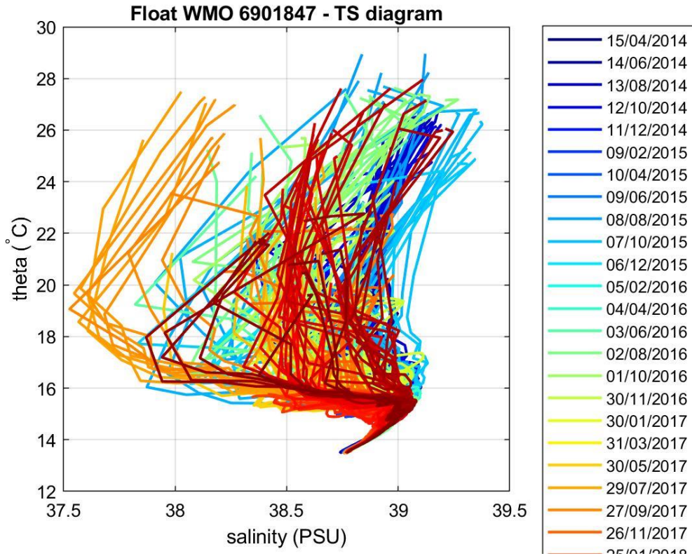
Figure 4: Float 6901847. \theta -S diagram color-coded per cycle number.
