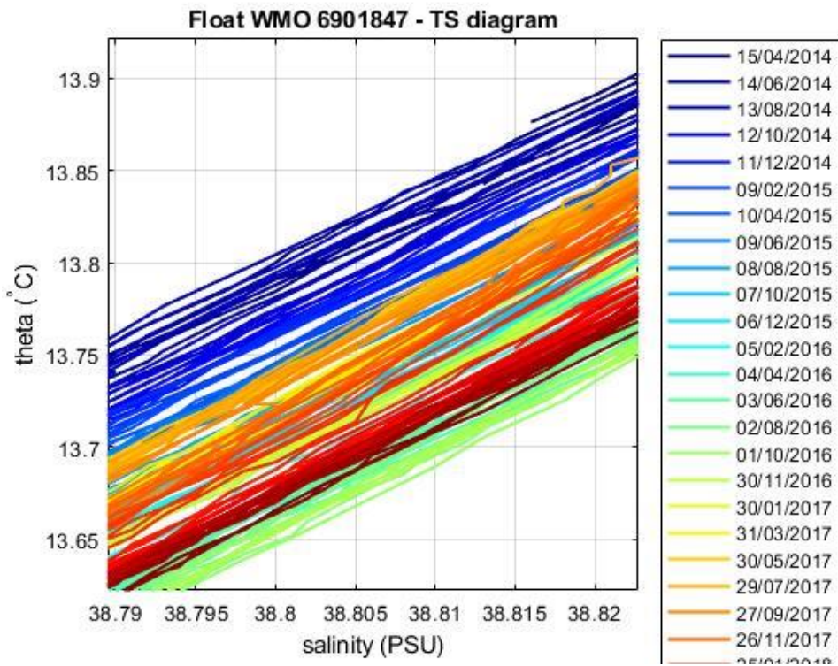
Figure 5: Float 6901847. Area of the \theta -S diagram (color-coded per cycle number) where the \theta -S relationship is more uniform.
