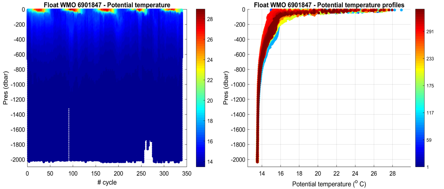
Figure 2: Float 6901847. Time series of Argo float potential temperature ( ^{\circ}\text{C} ) on the left, and potential temperature profiles color-coded per cycle number on the right.
