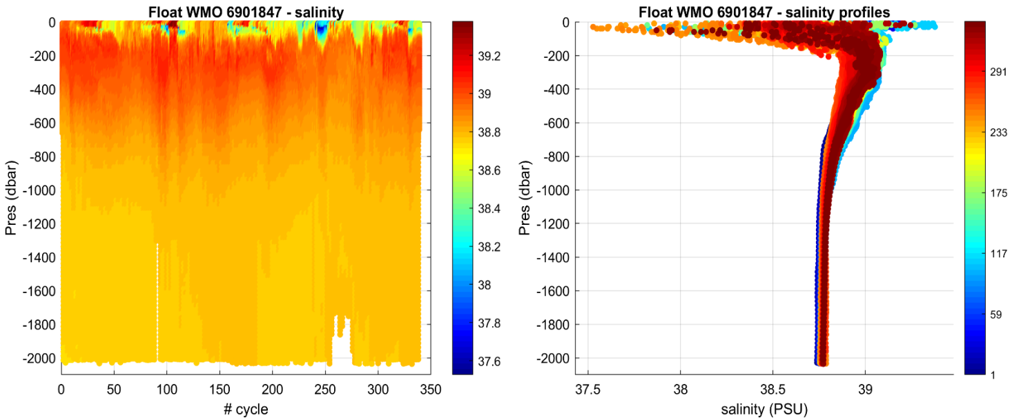
Figure 3: Float 6901847. Time series of Argo float potential salinity (PSS-78) on the left, and salinity profiles color-coded per cycle number on the right.
