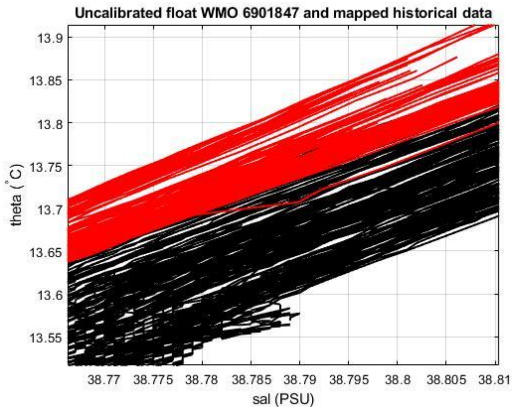
Figure 19: Float 6901847. Uncalibrated float salinity profile (black lines) and mapped historical data (red lines) in the most uniform part of the \theta -S curve.
