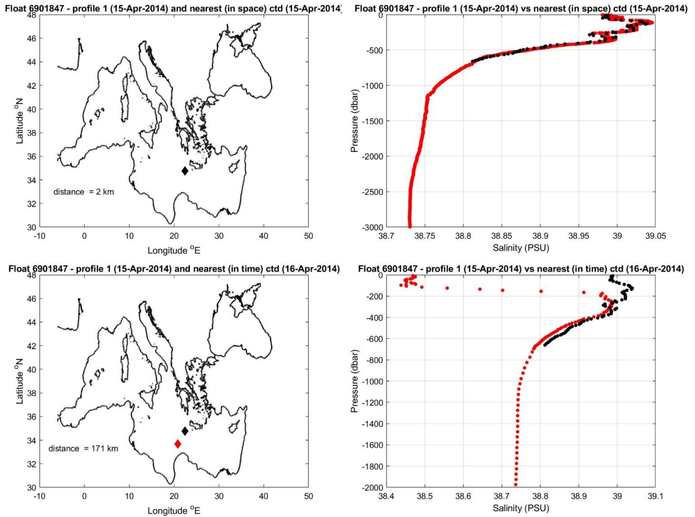
Figure 9: Float 6901847. The salinity float profile number 1 (black dots) are compared to the nearest in space (top) and in time (bottom) reference profile (red dots). The locations of the two profiles and their distance is given in the left panel.
