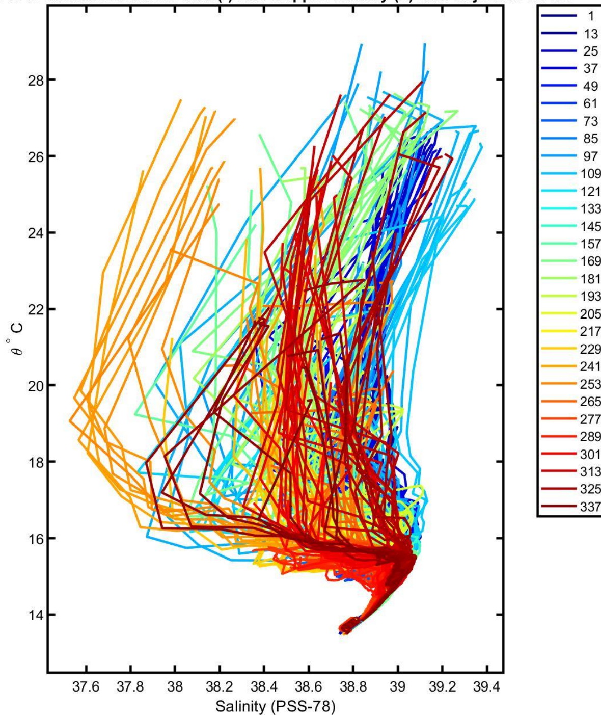
6901847 uncalibrated float data (-) and mapped salinity (o) with objective errors
