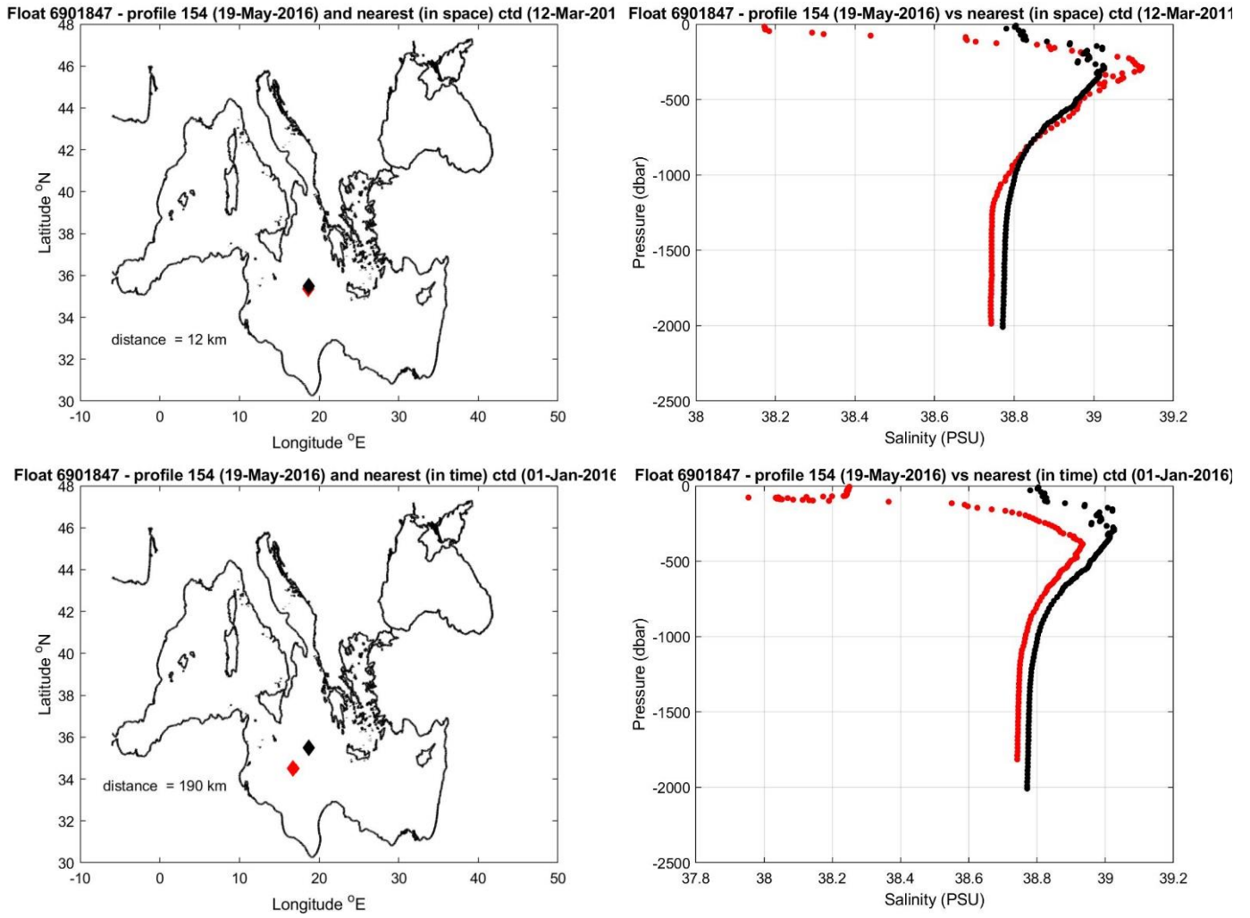
Figure 10: Float 6901847. The salinity float profile number 154 (black dots) are compared to the nearest in space (top) and in time (bottom) reference profile (red dots). The locations of the two profiles and their distance is given in the left panel.
