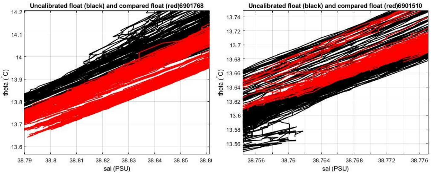
Figure 21: Float 6901847. Comparison between float 6901847 (black line) and other floats (red line), in the most uniform part of the \theta -S curve.
