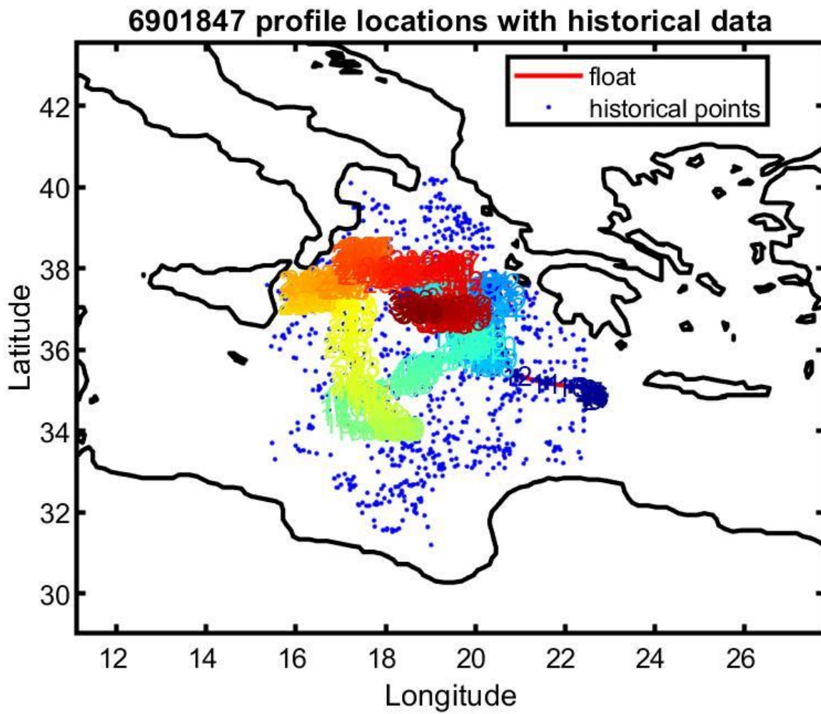
Figure 13: Float 6901847. Location of the float profiles (red line with colored numbers) and the reference data selected for mapping (blue dots).
