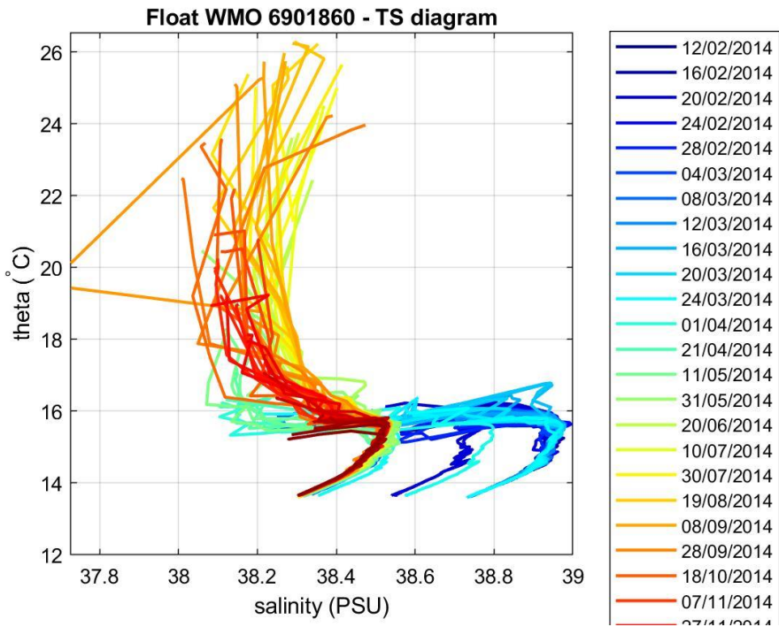
Figure 3: Float 6901860. \theta -S diagram color-coded per cycle number.
