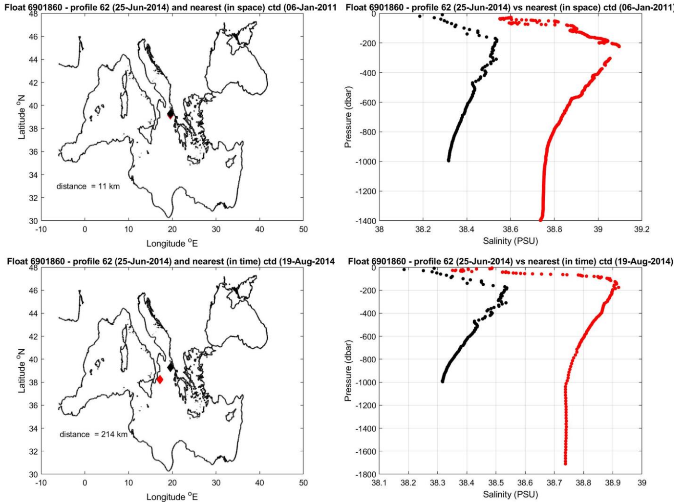
Figure 9: Float 6901860. The salinity float profile number 62 (black dots) are compared to the nearest in space (top) and in time (bottom) reference profile (red dots). The locations of the two profiles and their distance is given in the left panel.
