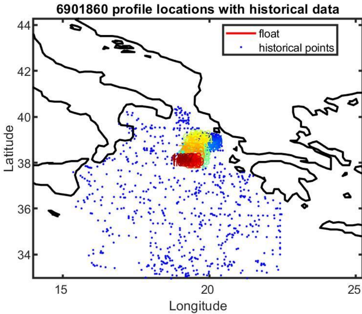
Figure 12: Float 6901860. Location of the float profiles (red line with colored numbers) and the reference data selected for mapping (blue dots).
