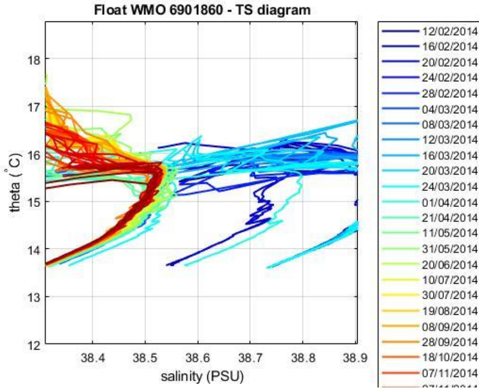
Figure 4: Float 6901860. Area of the \theta -S diagram (color-coded per cycle number) where the \theta -S relationship is more uniform.
