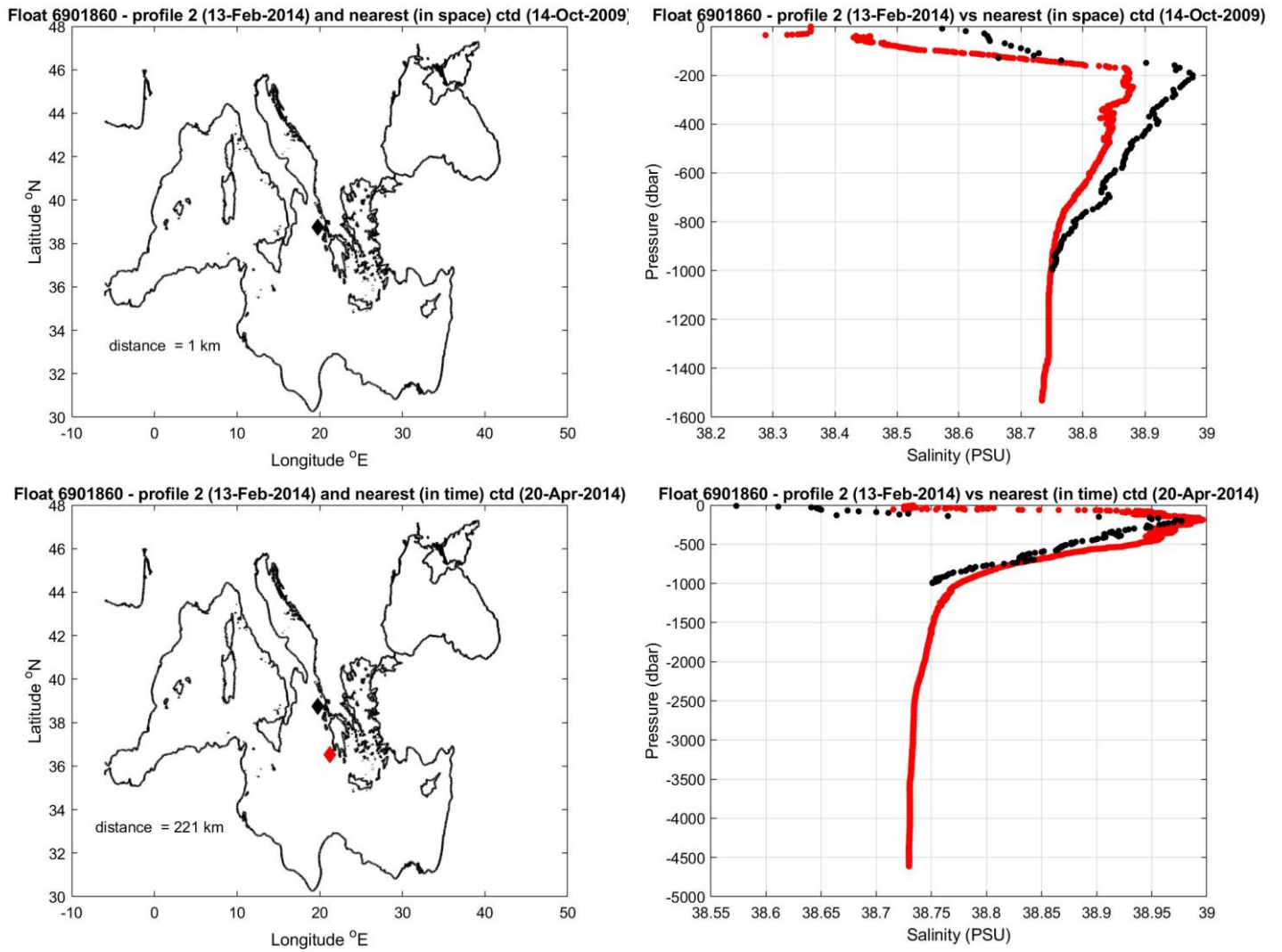
Figure 8: Float 6901860. The salinity float profile number 2 (black dots) are compared to the nearest in space (top) and in time (bottom) reference profile (red dots). The locations of the two profiles and their distance is given in the left panel.
