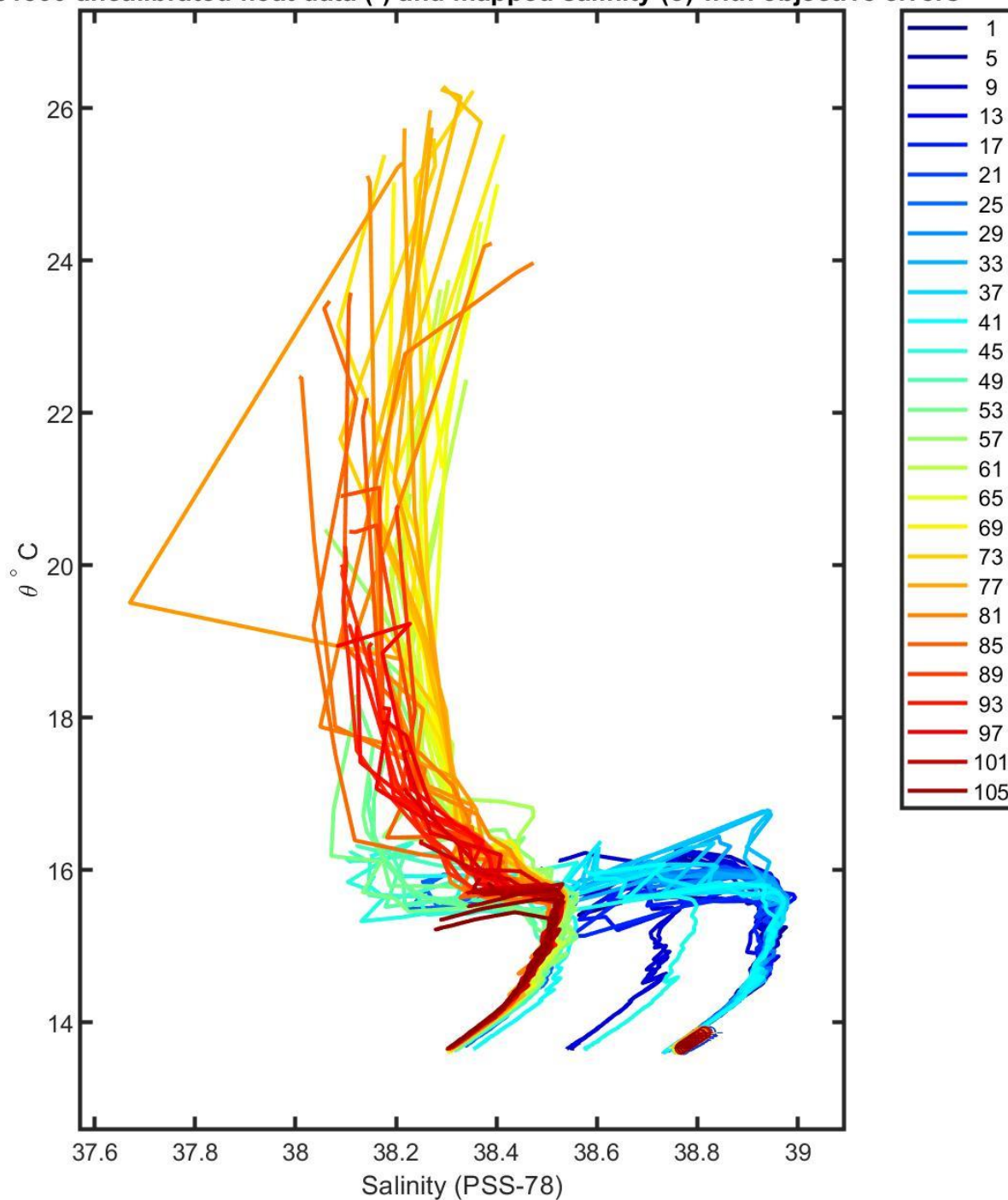
6901860 uncalibrated float data (-) and mapped salinity (o) with objective errors
