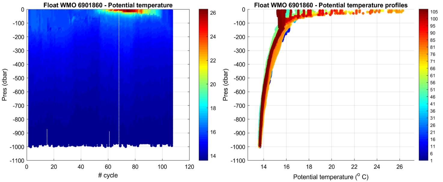
Figure 1: Float 6901860. Time series of Argo float potential temperature ( ^{\circ}\text{C} ) on the left, and potential temperature profiles color-coded per cycle number on the right.
