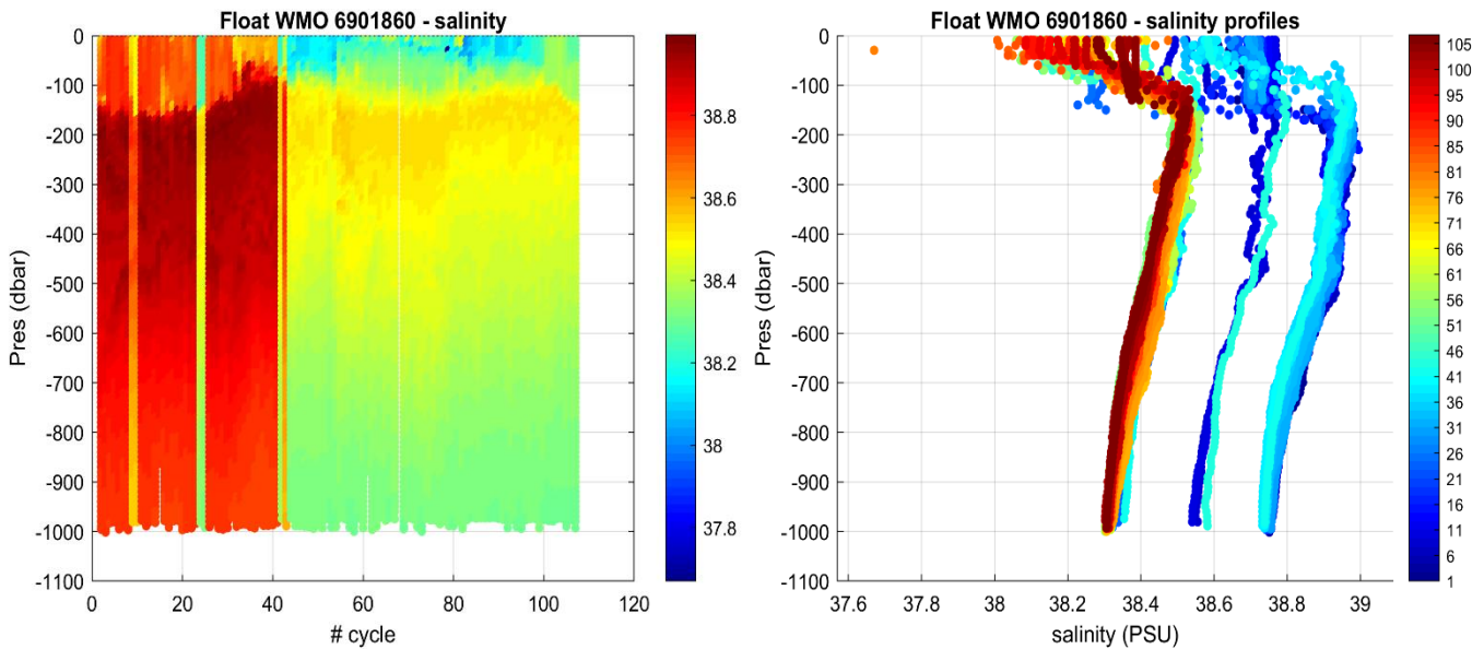
Figure 2: Float 6901860. Time series of Argo float potential salinity (PSS-78) on the left, and salinity profiles color-coded per cycle number on the right.
