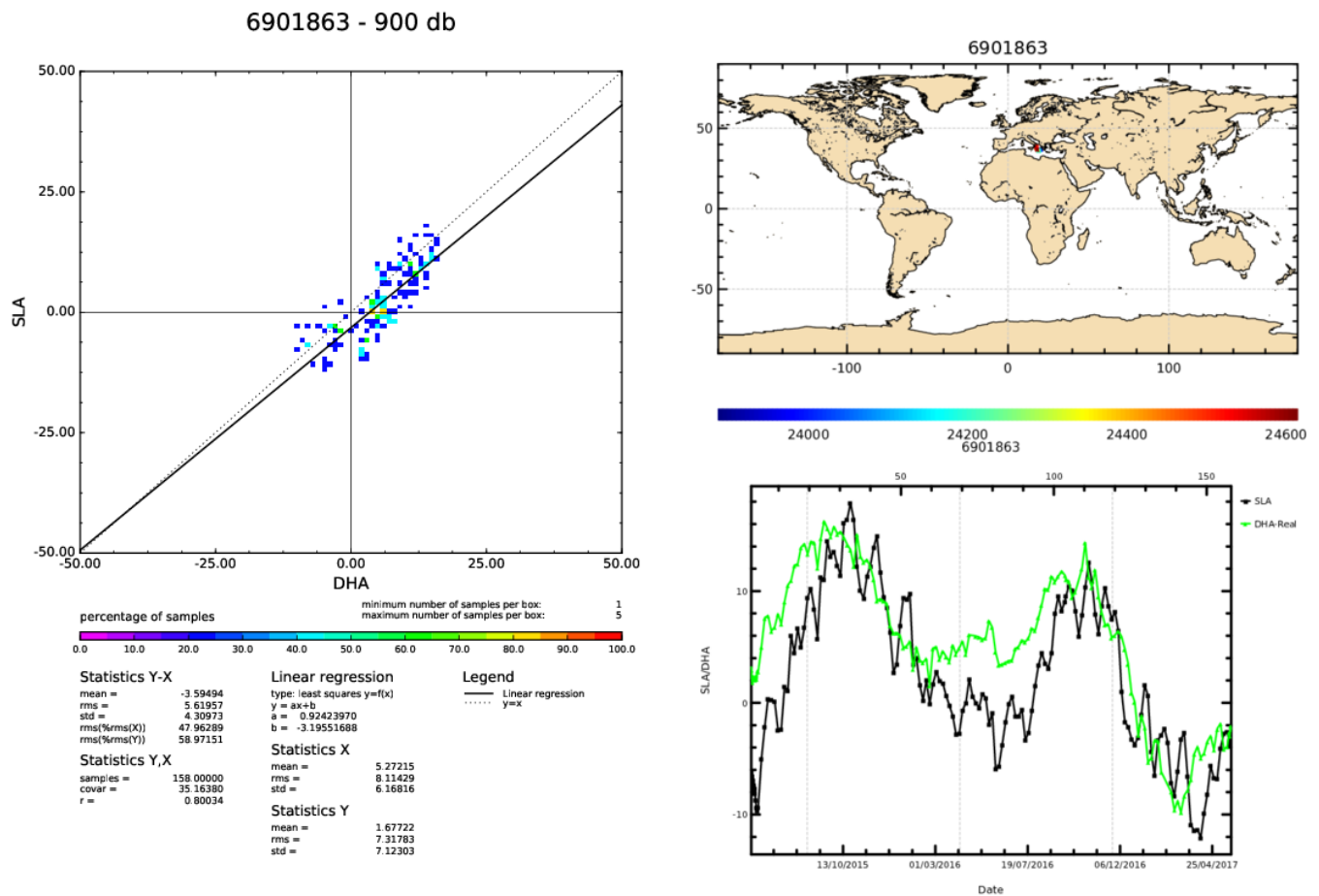
Figure 1: Float 6901863. The comparison between the sea surface height (SSH) from the satellite altimetry and dynamic height anomaly (DHA) extracted from the Argo float temperature and salinity. The figure is created by the CLS/Coriolis and distributed by Ifremer ( ftp://ftp.ifremer.fr/ifremer/argo/etc/argo-ast9-item13-AltimeterComparison/figures/ ).
