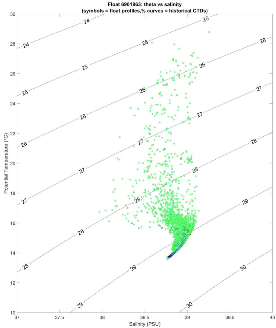
Figure 12: Float 6901863. T/S diagram plotted with and data from WMO boxes of CTD reference data +/- 10° of latitude and longitude. The black and blue cycles indicate the first and the last Argo profile, respectively. Green symbols represent other Argo profiles from this float. The thin colours lines indicate the reference data.
