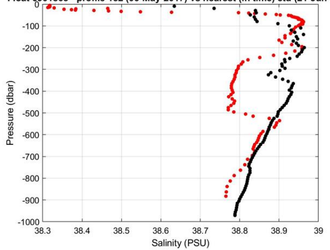
Float 6901863 - profile 152 (06-May-2017) vs nearest (in time) ctd (21-Jun-2016)
