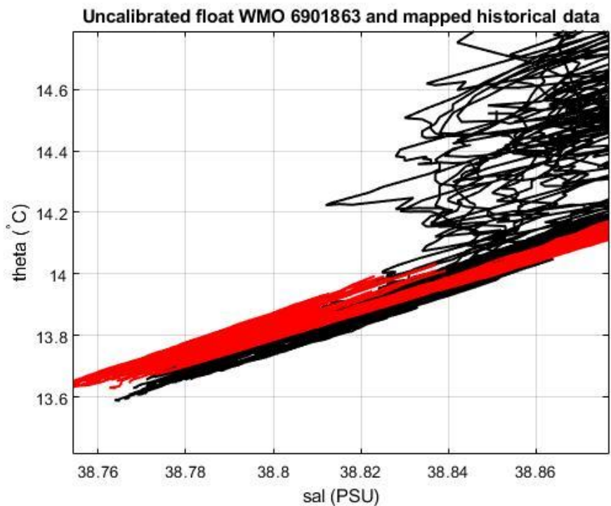
Figure 19: Float 6901863. Uncalibrated float salinity profile (black lines) and mapped historical data (red lines) in the most uniform part of the \theta -S curve.
