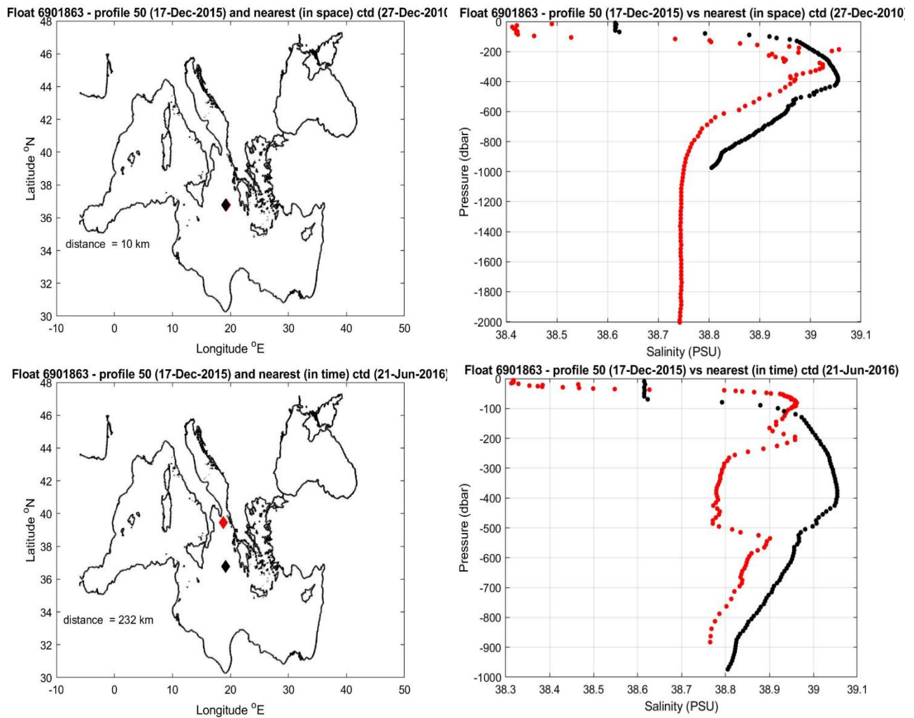
Figure 10: Float 6901863. The salinity float profile number 50 (black dots) are compared to the nearest in space (top) and in time (bottom) reference profile (red dots). The locations of the two profiles and their distance is given in the left panel.
