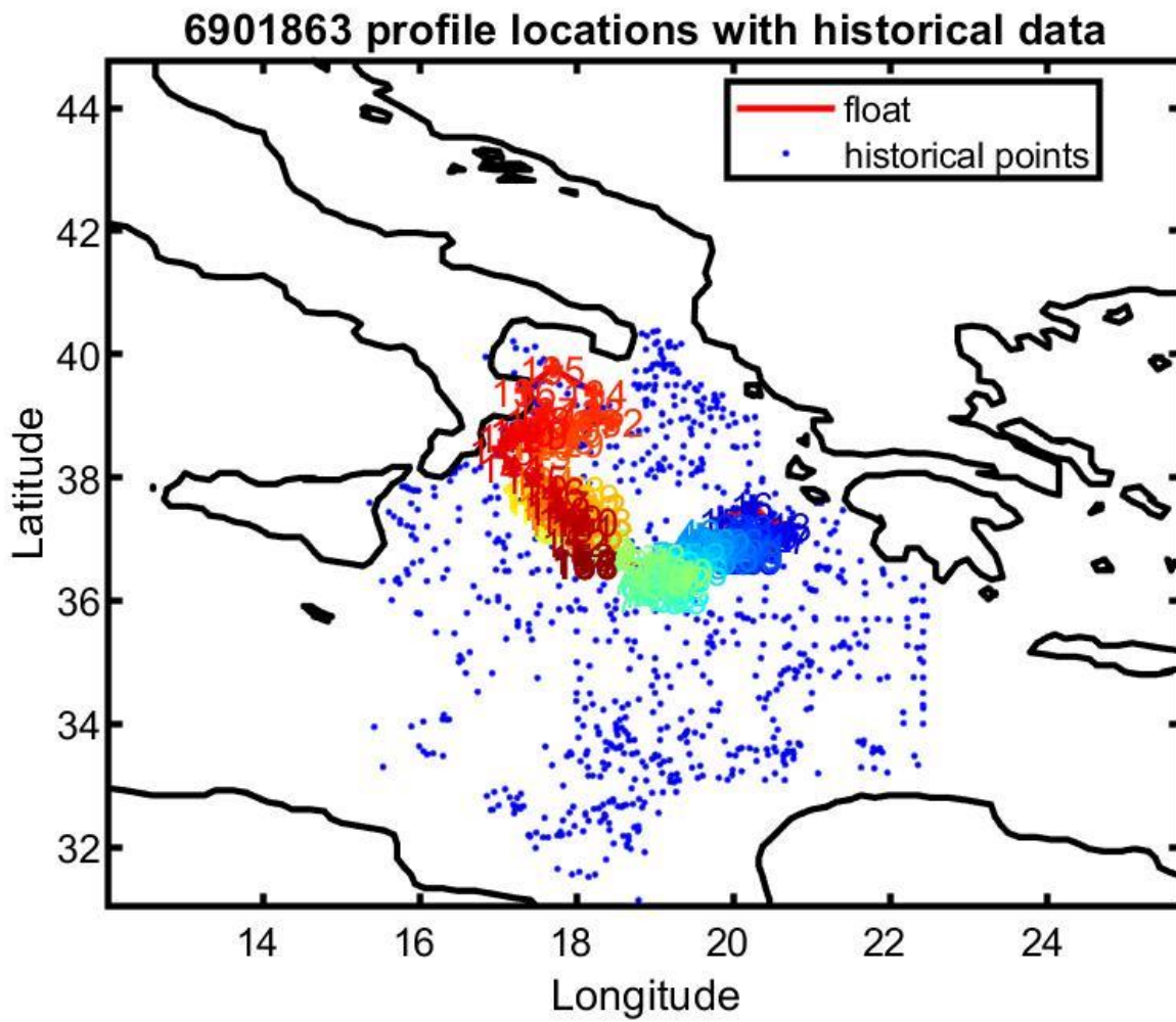
Figure 13: Float 6901863. Location of the float profiles (red line with colored numbers) and the reference data selected for mapping (blue dots).
