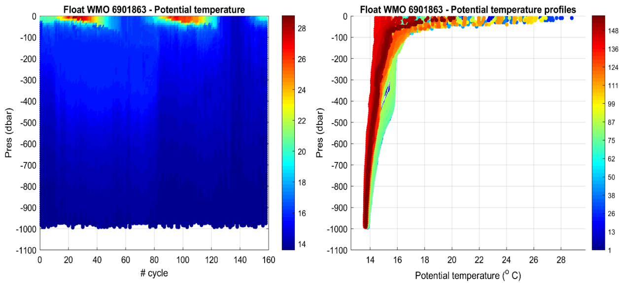
Figure 2: Float 6901863. Time series of Argo float potential temperature ( ^{\circ}\text{C} ) on the left, and potential temperature profiles color-coded per cycle number on the right.
