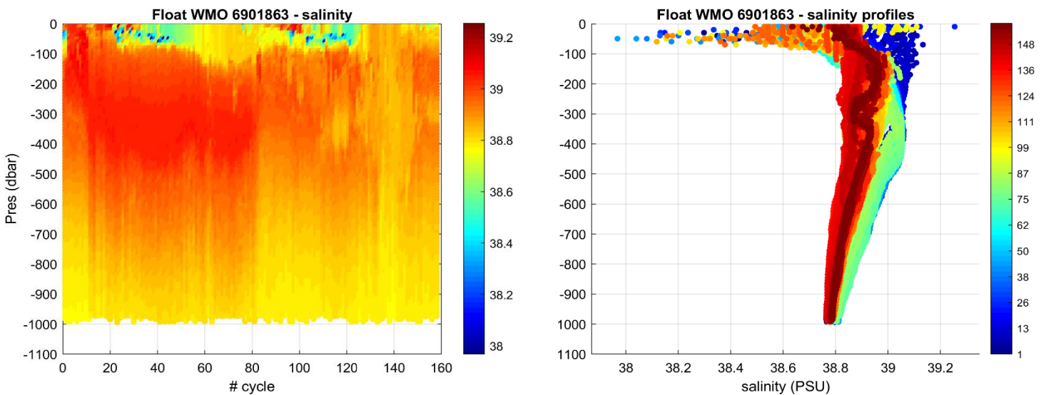
Figure 3: Float 6901863. Time series of Argo float potential salinity (PSS-78) on the left, and salinity profiles color-coded per cycle number on the right.
