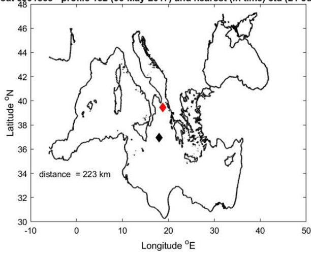
Figure 11: Float 6901863. The salinity float profile number 152 (black dots) are compared to the nearest in space (top) and in time (bottom) reference profile (red dots). The locations of the two profiles and their distance is given in the left panel.
