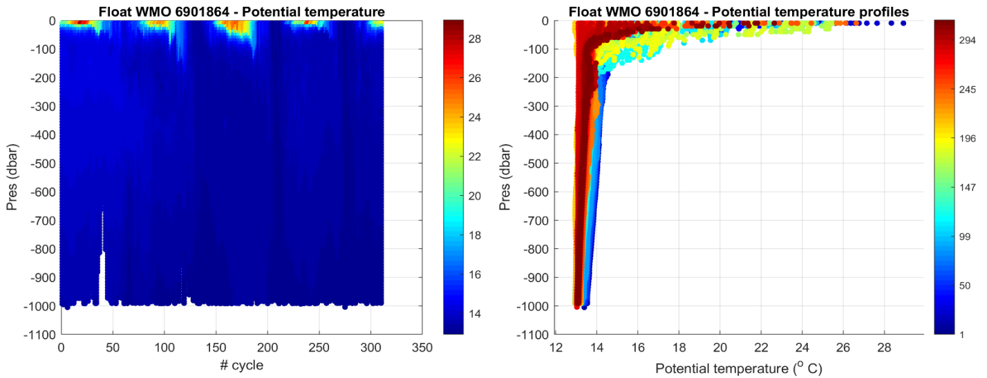
Figure 2: Float 6901864. Time series of Argo float potential temperature ( ^{\circ}\text{C} ) on the left, and potential temperature profiles color-coded per cycle number on the right.
