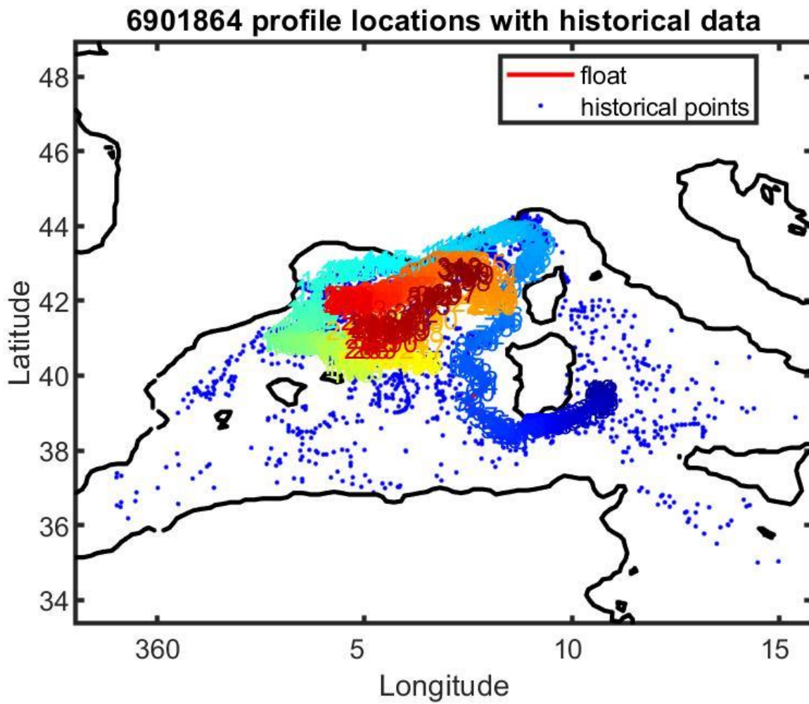
Figure 13: Float 6901864. Location of the float profiles (red line with colored numbers) and the reference data selected for mapping (blue dots).
