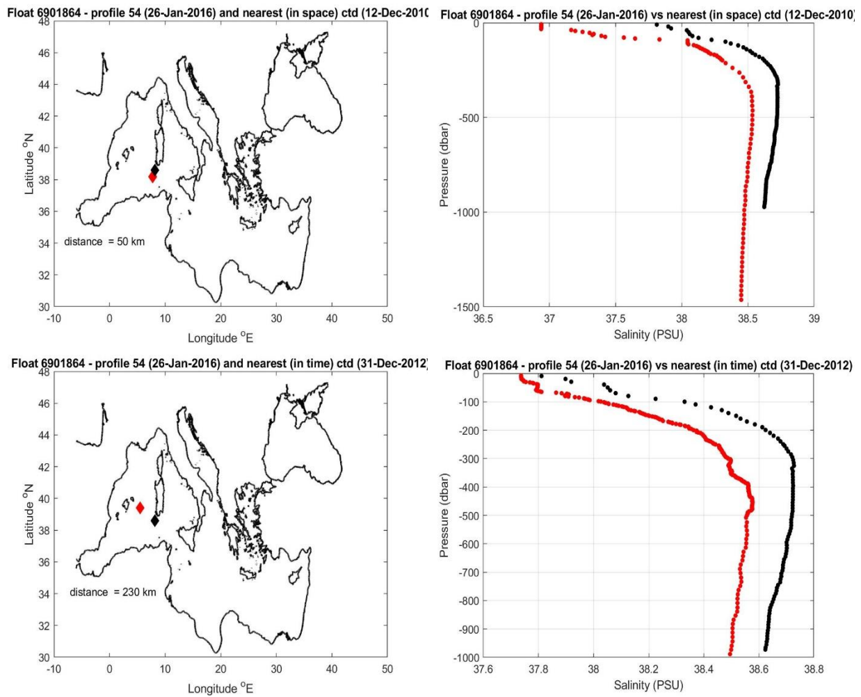
Figure 10: Float 6901864. The salinity float profile number 54 (black dots) are compared to the nearest in space (top) and in time (bottom) reference profile (red dots). The locations of the two profiles and their distance is given in the left panel.
