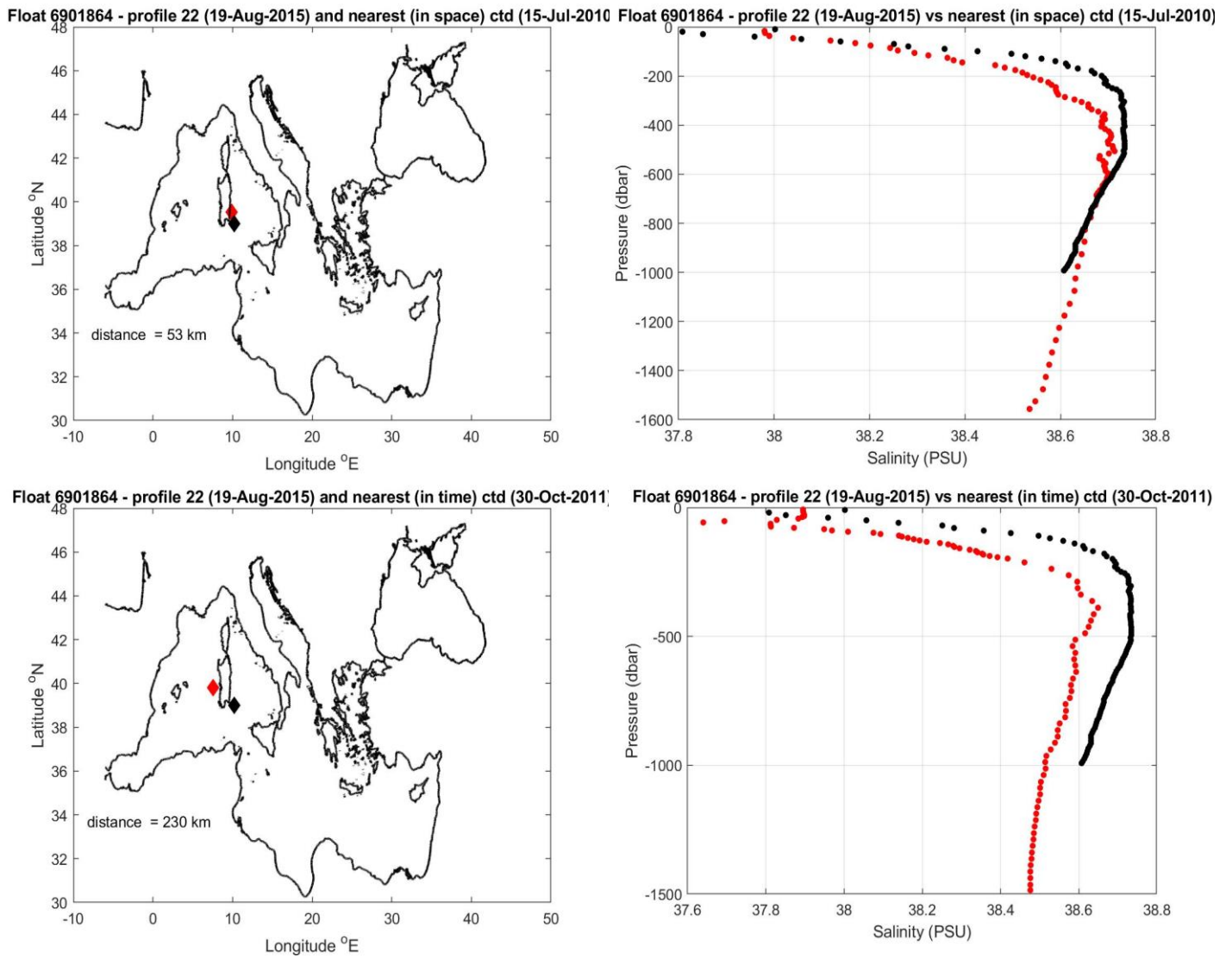
Figure 9: Float 6901864. The salinity float profile number 22 (black dots) are compared to the nearest in space (top) and in time (bottom) reference profile (red dots). The locations of the two profiles and their distance is given in the left panel.
