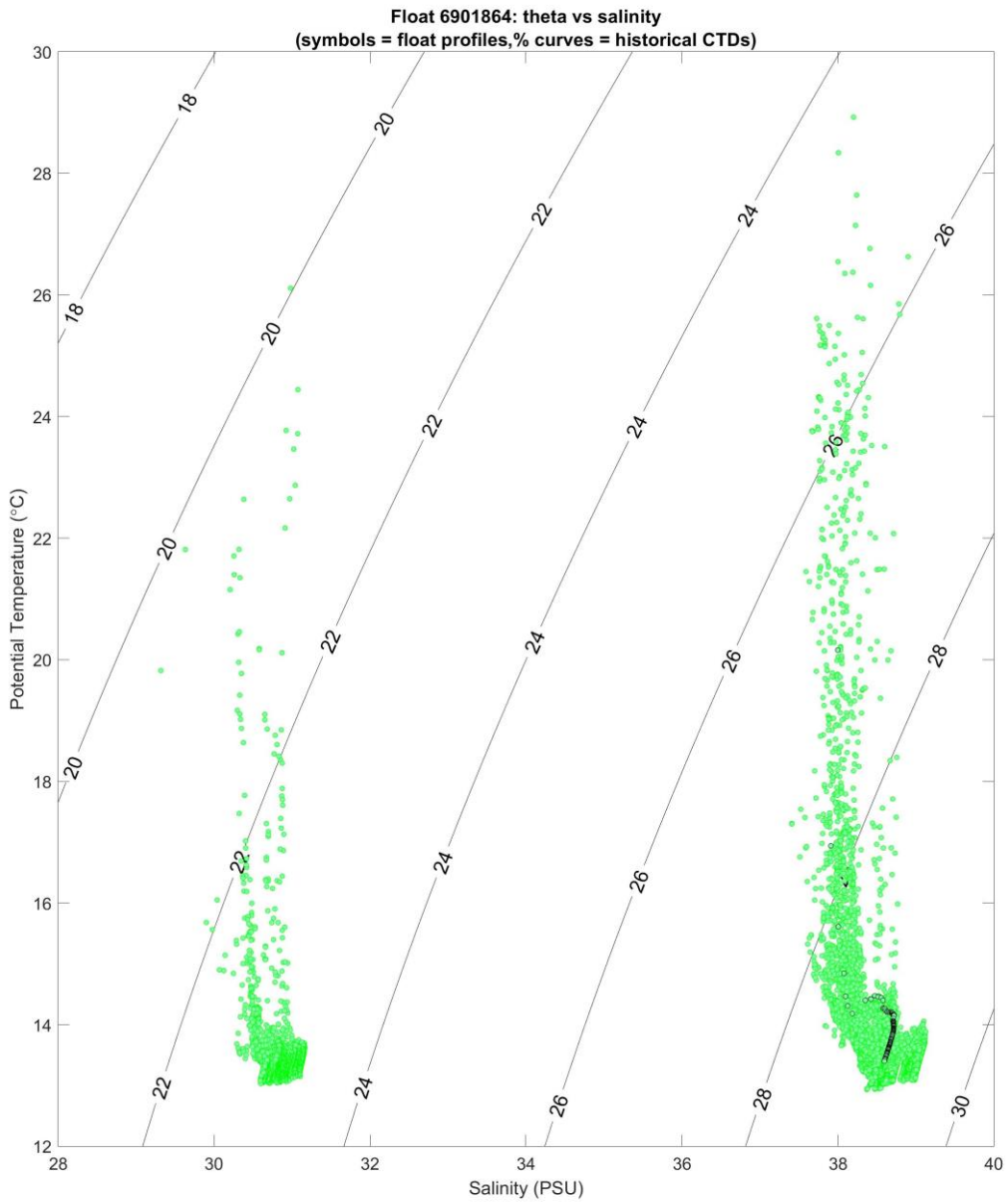
Figure 12: Float 6901864. T/S diagram plotted with and data from WMO boxes of CTD reference data +/- 10° of latitude and longitude. The black and blue cycles indicate the first and the last Argo profile, respectively. Green symbols represent other Argo profiles from this float. The thin colour lines indicate the reference data.
