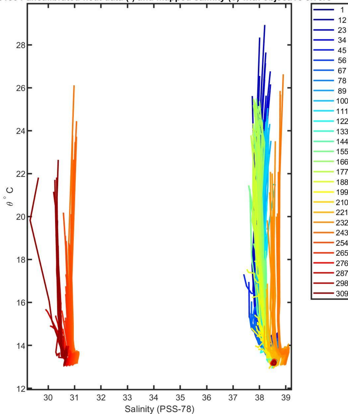
6901864 uncalibrated float data (-) and mapped salinity (o) with objective errors
