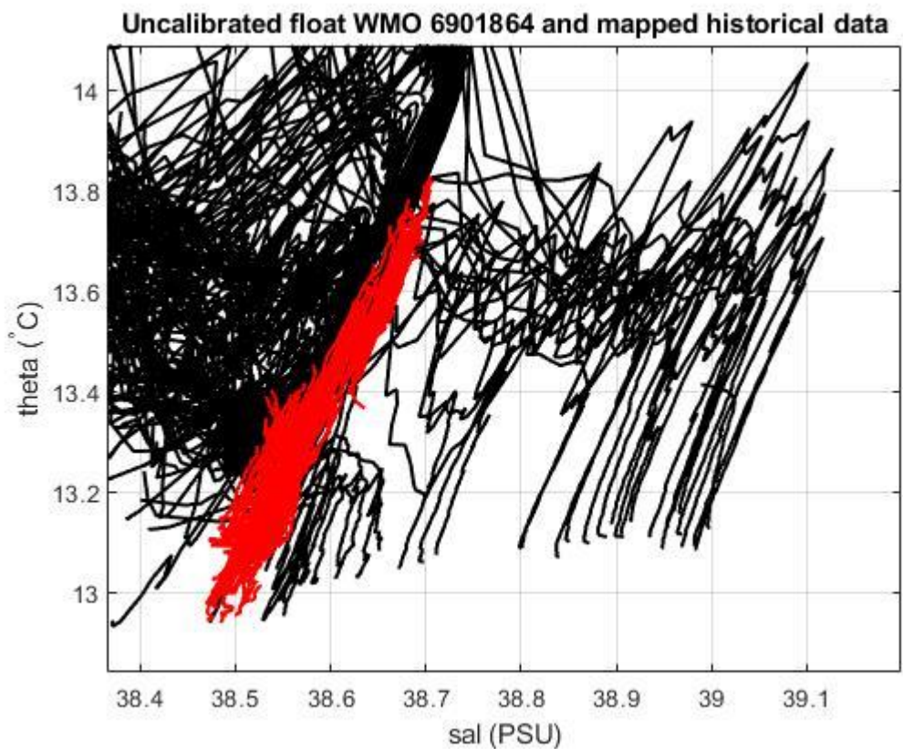
Figure 19: Float 6901864. Uncalibrated float salinity profile (black lines) and mapped historical data (red lines) in the most uniform part of the \theta -S curve.
