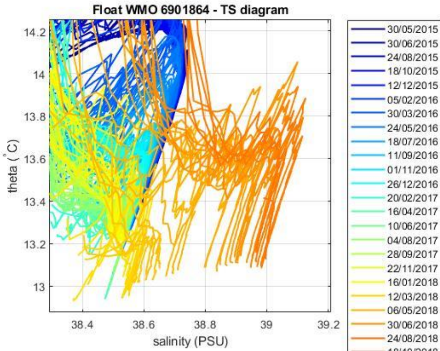
Figure 5: Float 6901864. Area of the \theta -S diagram (color-coded per cycle number) where the \theta -S relationship is more uniform.
