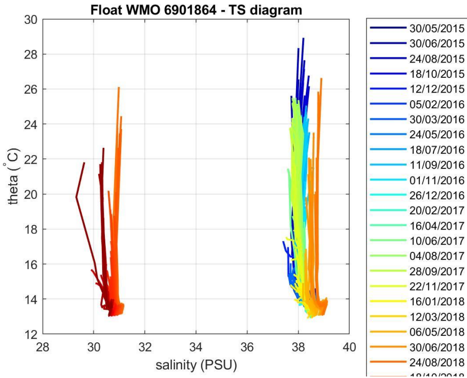
Figure 4: Float 6901863. \theta -S diagram color-coded per cycle number.
