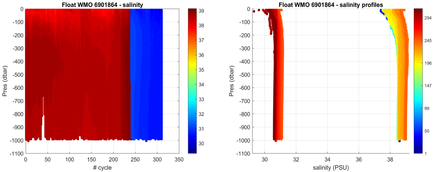
Figure 3: Float 6901864. Time series of Argo float potential salinity (PSS-78) on the left, and salinity profiles color-coded per cycle number on the right.
