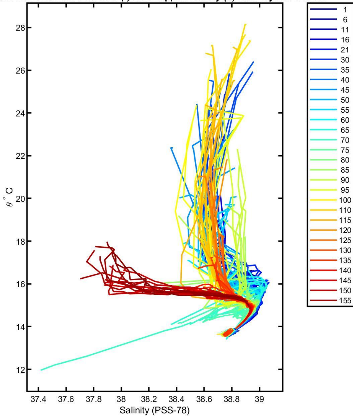
6901882 uncalibrated float data (-) and mapped salinity (o) with objective errors
