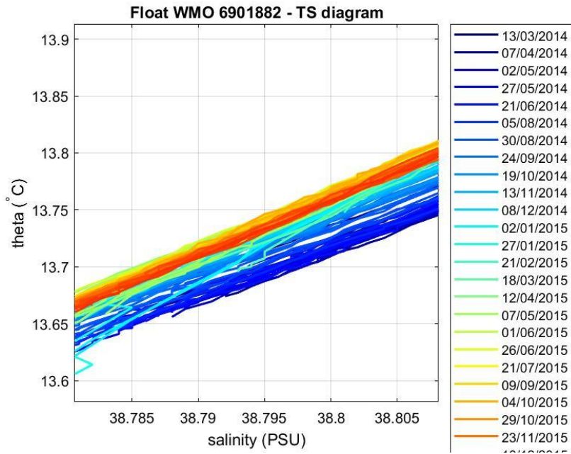
Figure 5: Float 6901882. Area of the \theta -S diagram (color-coded per cycle number) where the \theta -S relationship is more uniform.
