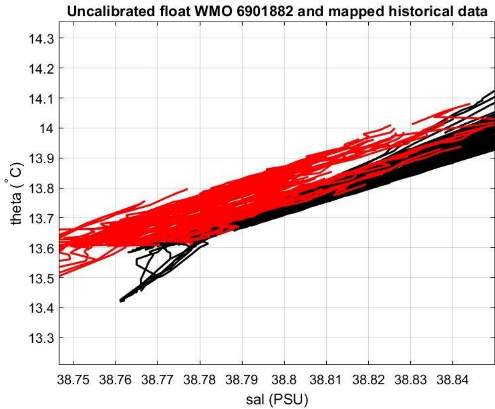
Figure 19: Float 6901882. Uncalibrated float salinity profile (black lines) and mapped historical data (red lines) in the most uniform part of the \theta -S curve.
