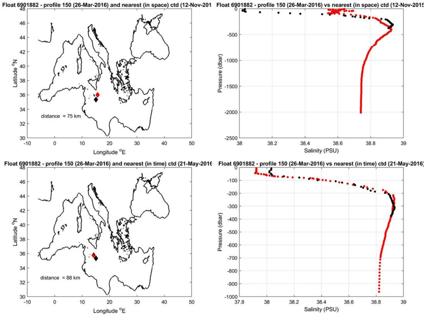
Figure 11: Float 6901882. The salinity float profile number 150 (black dots) are compared to the nearest in space (top) and in time (bottom) reference profile (red dots). The locations of the two profiles and their distance is given in the left panel.
