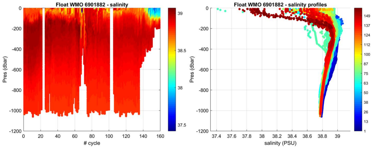
Figure 3: Float 6901882. Time series of Argo float potential salinity (PSS-78) on the left, and salinity profiles color-coded per cycle number on the right.
