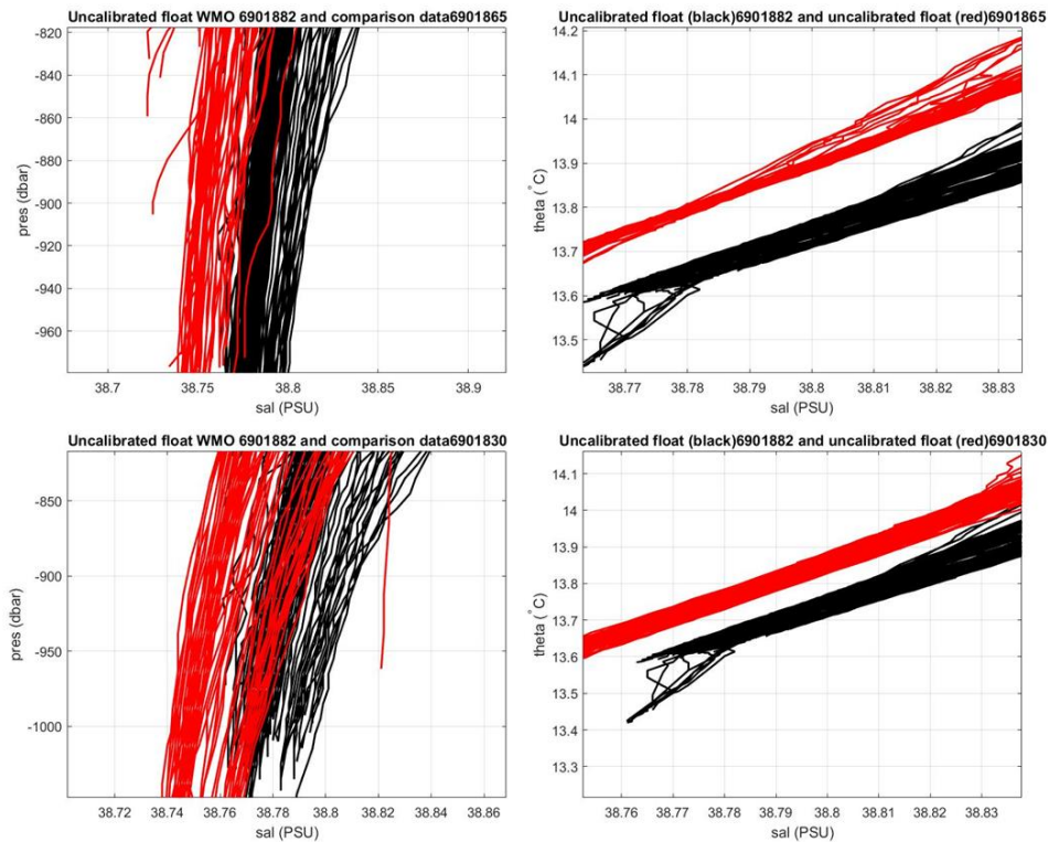
Figure 21: Float 6901882. Comparison between float 6901882 (black line) with 6901865 (up) and 6901830 (below) (red line), in the most uniform part of the \theta -S curve. On the left salinity profiles, on the right the \theta -S diagram.
