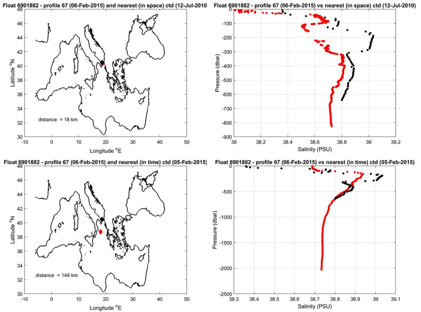
Figure 10: Float 6901882. The salinity float profile number 67 (black dots) are compared to the nearest in space (top) and in time (bottom) reference profile (red dots). The locations of the two profiles and their distance is given in the left panel.
