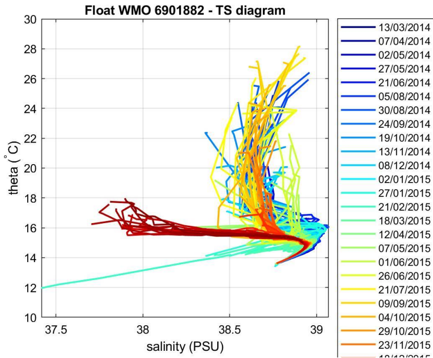
Figure 4: Float 6901882. \theta -S diagram color-coded per cycle number.
