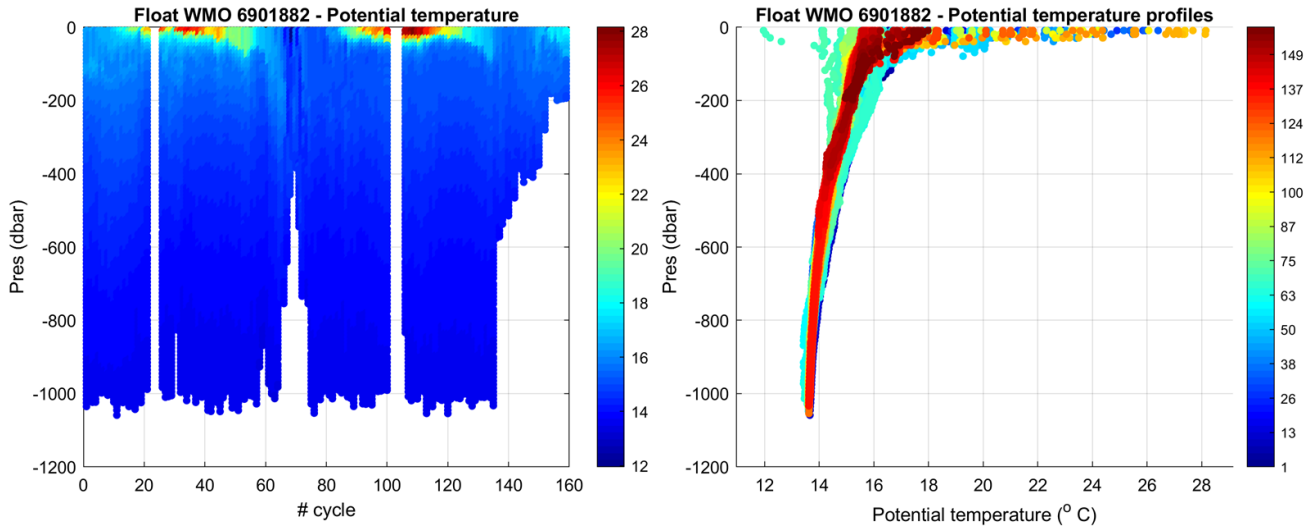
Figure 2: Float 6901882. Time series of Argo float potential temperature ( ^{\circ}\text{C} ) on the left, and potential temperature profiles color-coded per cycle number on the right.
