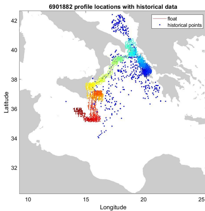
Figure 13: Float 6901882. Location of the float profiles (red line with colored numbers) and the reference data selected for mapping (blue dots).
