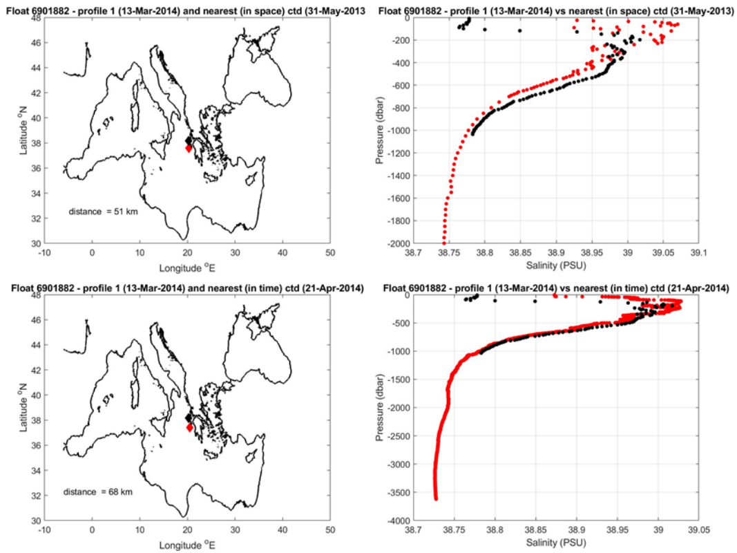
Figure 9: Float 6901882. The salinity float profile number 1 (black dots) are compared to the nearest in space (top) and in time (bottom) reference profile (red dots). The locations of the two profiles and their distance is given in the left panel.
