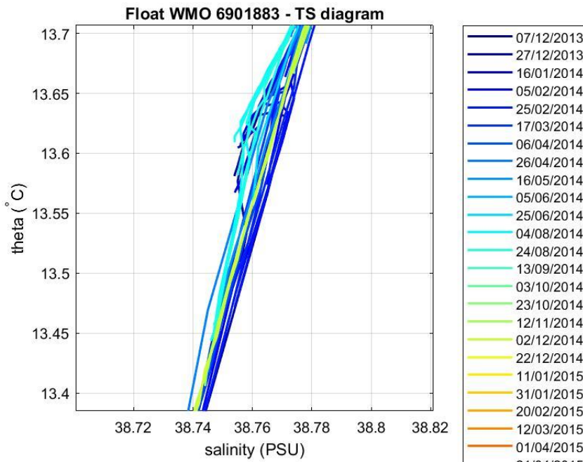
Figure 4: Float 6901883. Area of the \theta -S diagram (color-coded per cycle number) where the \theta -S relationship is more uniform.
