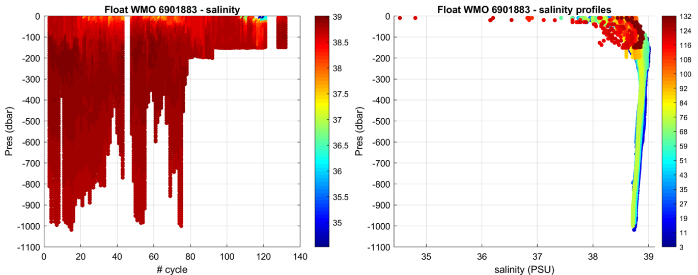
Figure 2: Float 6901883. Time series of Argo float potential salinity (PSS-78) on the left, and salinity profiles color-coded per cycle number on the right.
