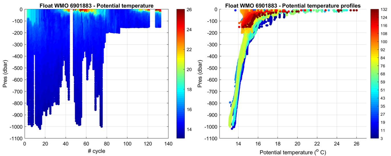
Figure 1: Float 6901883. Time series of Argo float potential temperature ( ^{\circ}\text{C} ) on the left, and potential temperature profiles color-coded per cycle number on the right.
