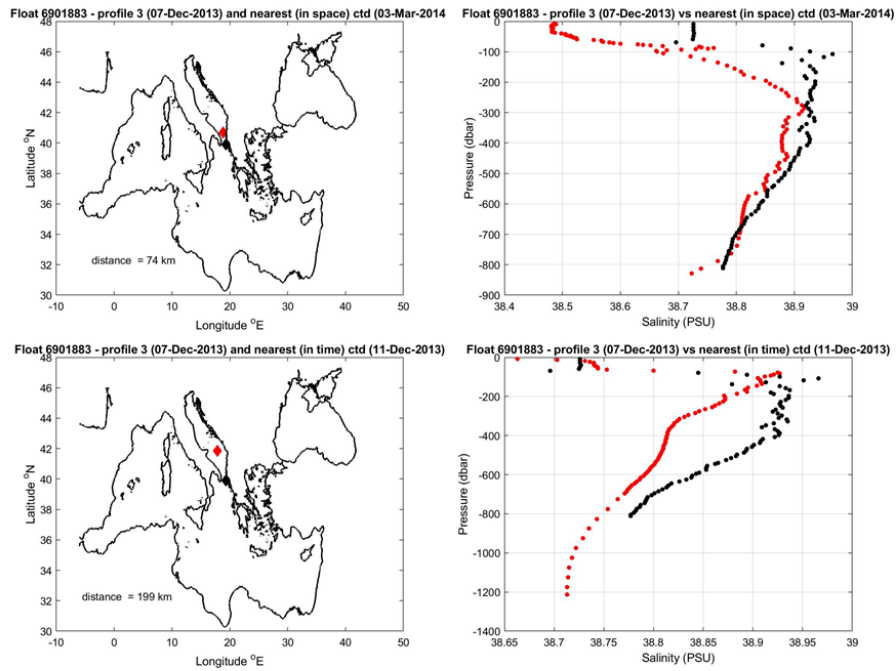
Figure 8: Float 6901883. The salinity float profile number 3 (black dots) are compared to the nearest in space (top) and in time (bottom) reference profile (red dots). The locations of the two profiles and their distance is given in the left panel.
