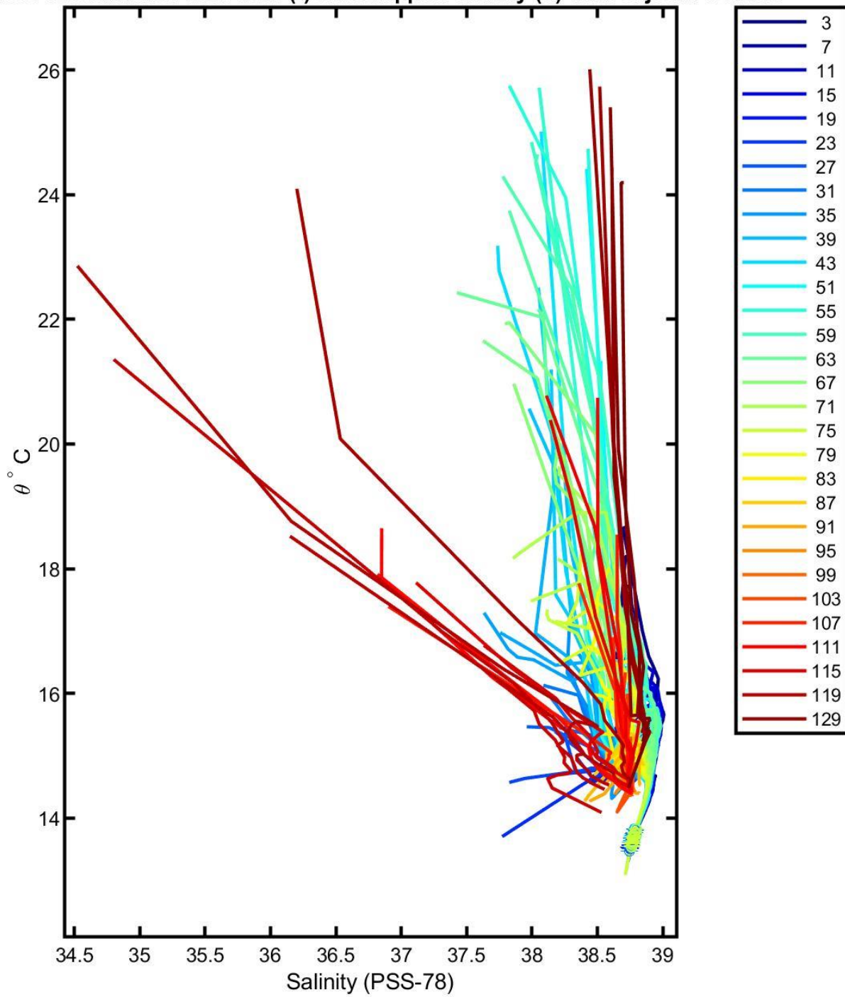
6901883 uncalibrated float data (-) and mapped salinity (o) with objective errors
