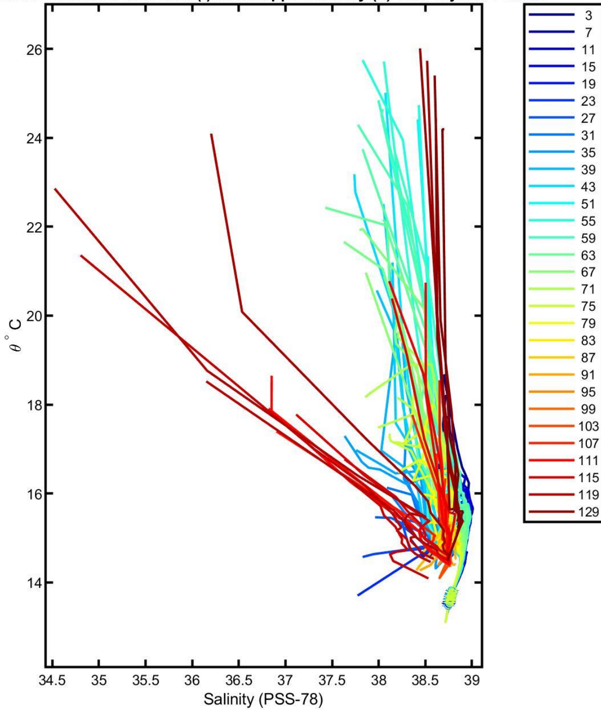
6901883 calibrated float data (-) and mapped salinity (o) with objective errors
