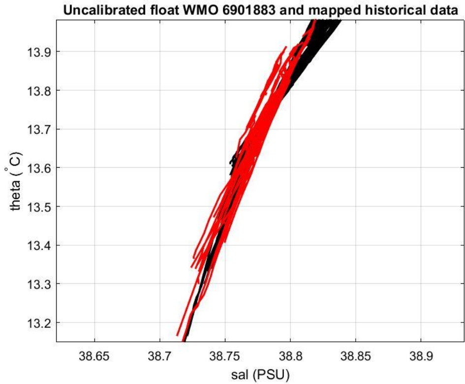
Figure 19: Float 6901883. Uncalibrated float salinity profile (black lines) and mapped historical data (red lines) in the most uniform part of the \theta -S curve.
