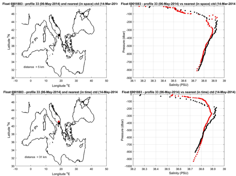
Figure 9: Float 6901883. The salinity float profile number 33 (black dots) are compared to the nearest in space (top) and in time (bottom) reference profile (red dots). The locations of the two profiles and their distance is given in the left panel.
