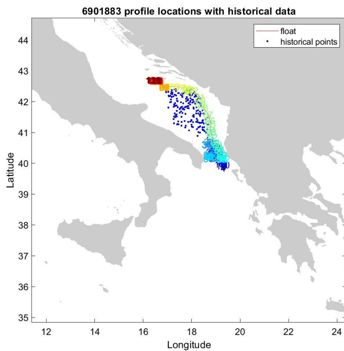
Figure 13: Float 6901883. Location of the float profiles (red line with colored numbers) and the reference data selected for mapping (blue dots).
