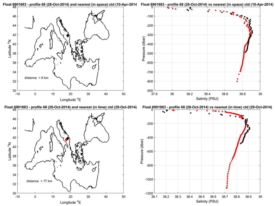
Figure 10: Float 6901883. The salinity float profile number 68 (black dots) are compared to the nearest in space (top) and in time (bottom) reference profile (red dots). The locations of the two profiles and their distance is given in the left panel.
