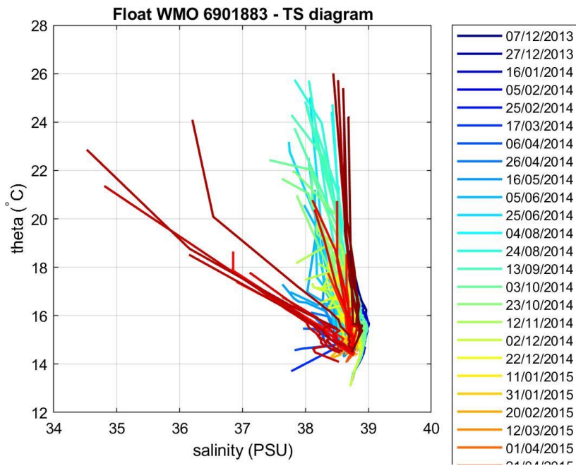
Figure 3: Float 6901883. \theta -S diagram color-coded per cycle number.
