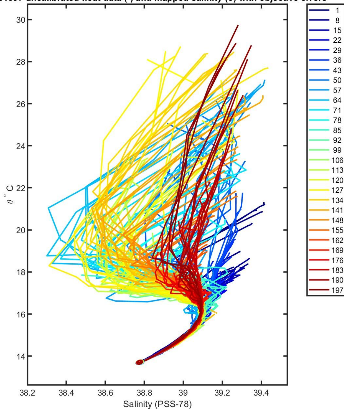
6901897 uncalibrated float data (-) and mapped salinity (o) with objective errors
