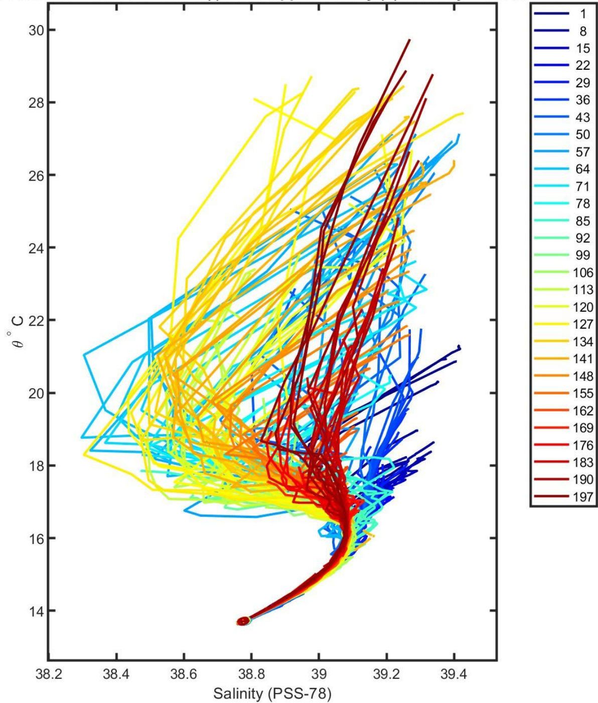
6901897 calibrated float data (-) and mapped salinity (o) with objective errors
