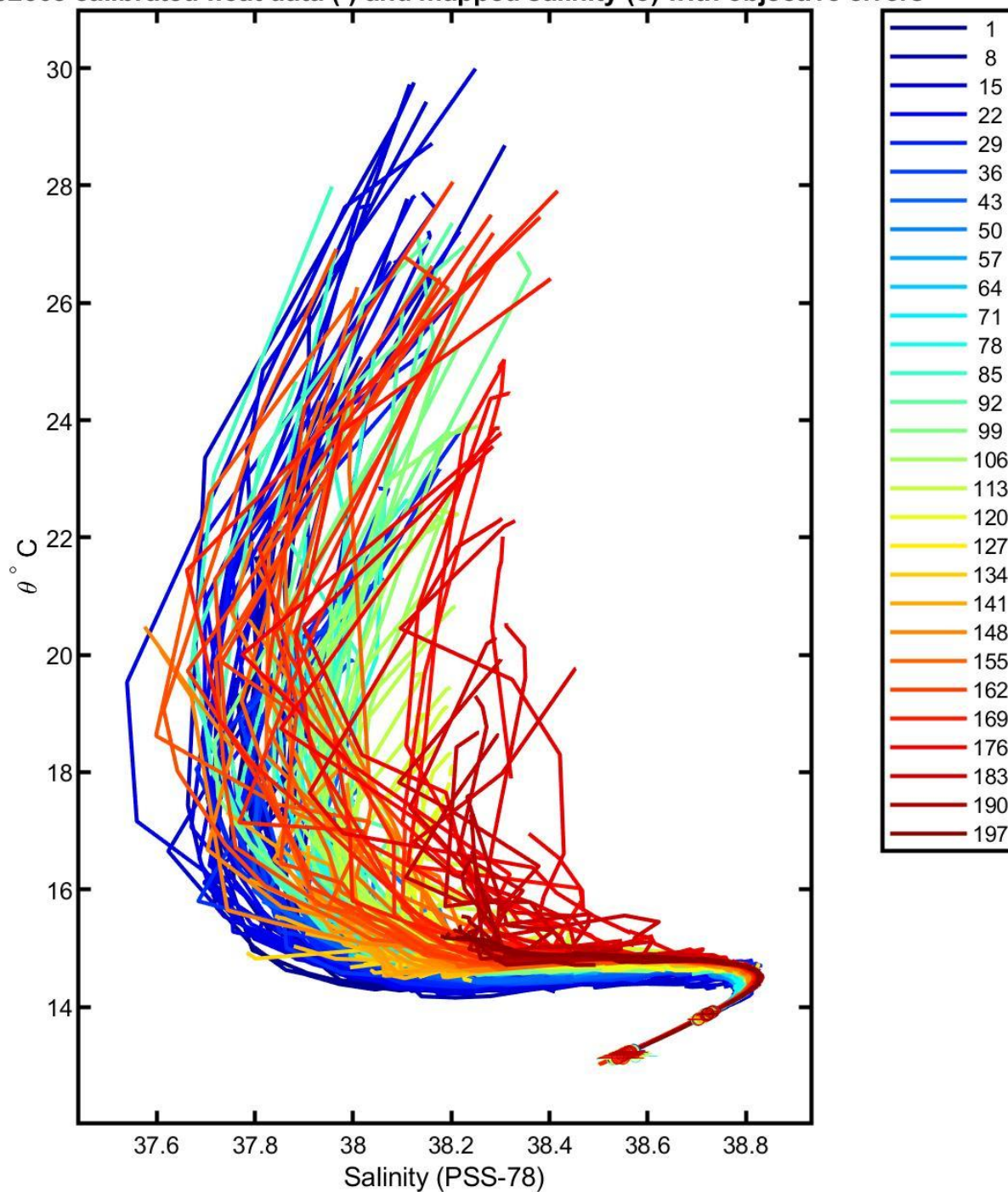
6902568 calibrated float data (-) and mapped salinity (o) with objective errors
