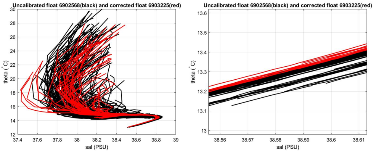
Figure 21: Float 6902568. Comparison between float 6902568 (black line) and 6903225 (red line), in the most uniform part of the \theta -S curve.
