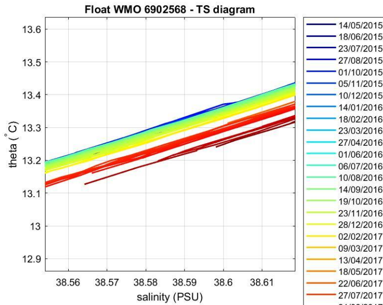
Figure 4: Float 6902568. Area of the \theta -S diagram (color-coded per cycle number) where the \theta -S relationship is more uniform.
