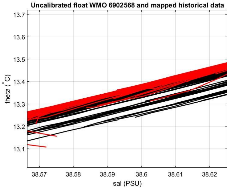
Figure 19: Float 6902568. Uncalibrated float salinity profile (black lines) and mapped historical data (red lines) in the most uniform part of the \theta -S curve.
