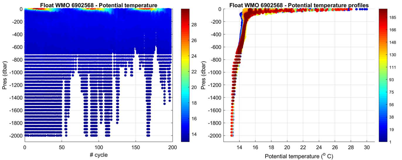
Figure 1: Float 6902568. Time series of Argo float potential temperature ( ^{\circ}\text{C} ) on the left, and potential temperature profiles color-coded per cycle number on the right.
