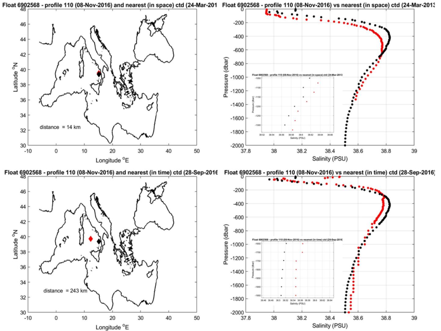
Figure 9: Float 6902568. The salinity float profile number 110 (black dots) are compared to the nearest in space (top) and in time (bottom) reference profile (red dots). In the small plots the comparison in the deeper layers is shown. The locations of the two profiles and their distance is given in the left panel.
