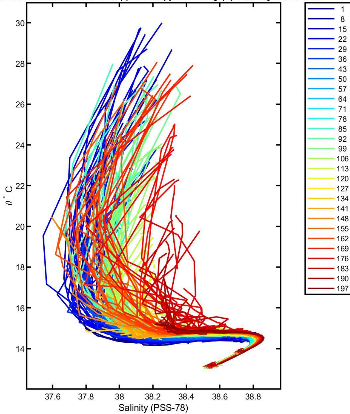
6902568 uncalibrated float data (-) and mapped salinity (o) with objective errors
