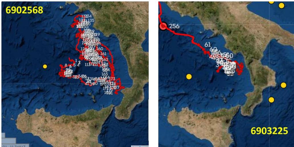
Figure 20: Float 6902568. Trajectory of the floats used for the comparison.
