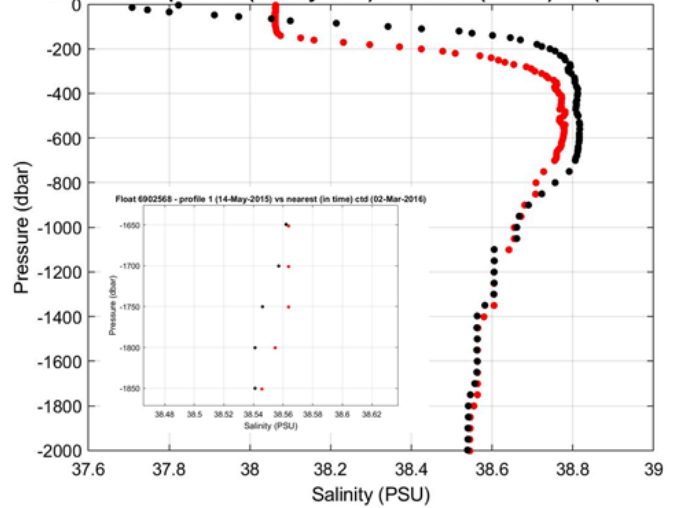
Float 6902568 - profile 1 (14-May-2015) vs nearest (in time) ctd (02-Mar-2016)
