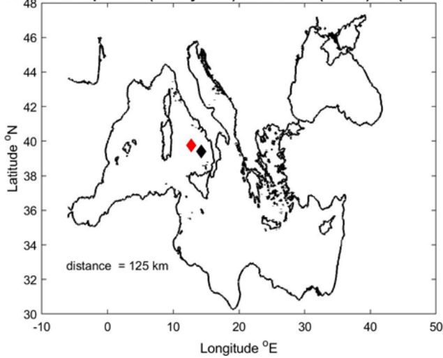
Float 6902568 - profile 1 (14-May-2015) and nearest (in time) ctd (02-Mar-2016)
