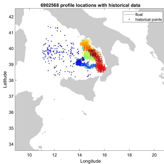
Figure 13: Float 6902568. Location of the float profiles (red line with colored numbers) and the reference data selected for mapping (blue dots).
