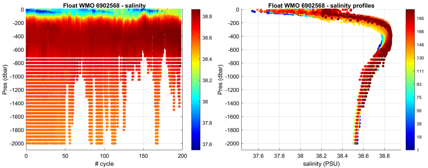
Figure 2: Float 6902568. Time series of Argo float potential salinity (PSS-78) on the left, and salinity profiles color-coded per cycle number on the right.
