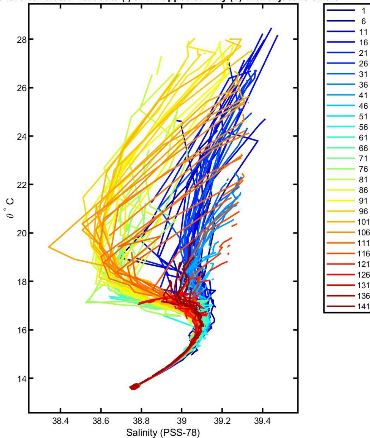
6902570 calibrated float data (-) and mapped salinity (o) with objective errors
