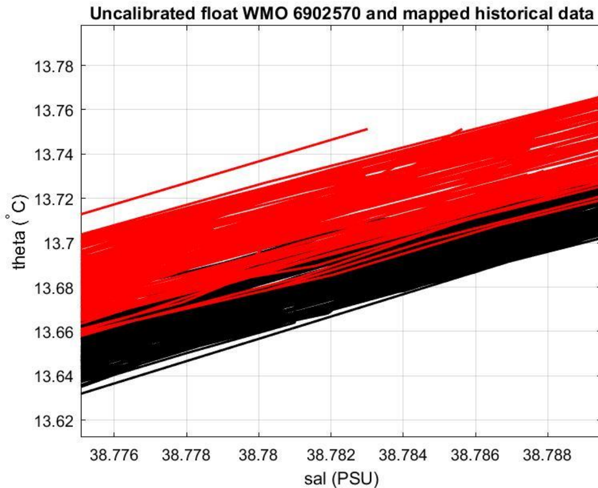
Figure 19: Float 6902570. Uncalibrated float salinity profile (black lines) and mapped historical data (red lines) in the most uniform part of the \theta -S curve.
