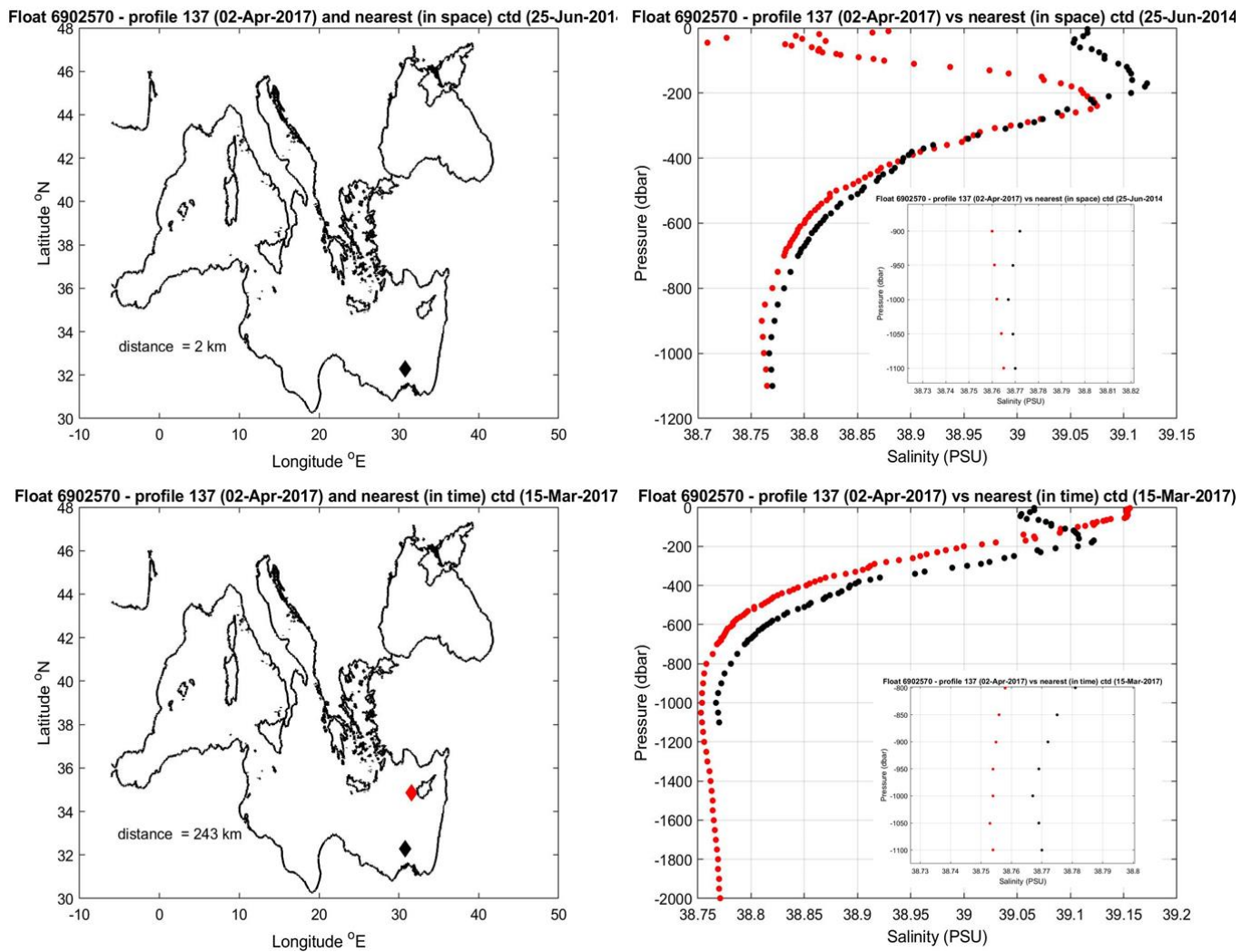
Figure 10: Float 6902570. The salinity float profile number 137 (black dots) are compared to the nearest in space (top) and in time (bottom) reference profile (red dots). In the small plots the comparison in the deeper layers is showed. The locations of the two profiles and their distance is given in the left panel.
