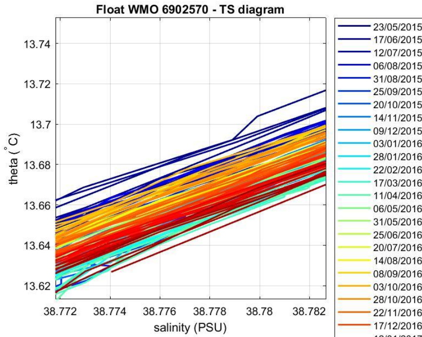
Figure 4: Float 6902570. Area of the \theta -S diagram (color-coded per cycle number) where the \theta -S relationship is more uniform.
