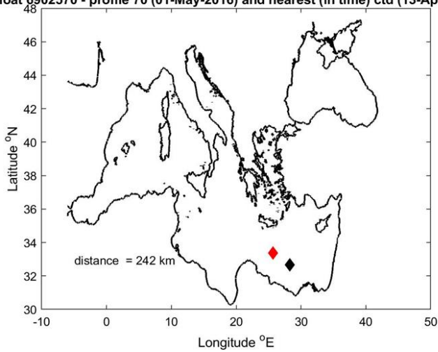
Figure 9: Float 6902570. The salinity float profile number 70 (black dots) are compared to the nearest in space (top) and in time (bottom) reference profile (red dots). In the small plots the comparison in the deeper layers is shown. The locations of the two profiles and their distance is given in the left panel.
