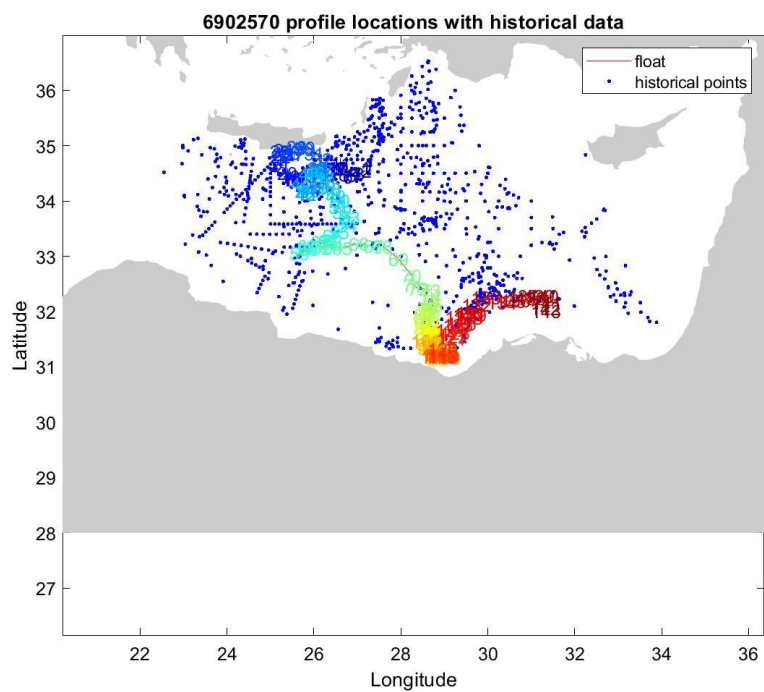
Figure 13: Float 6902570. Location of the float profiles (red line with colored numbers) and the reference data selected for mapping (blue dots).
