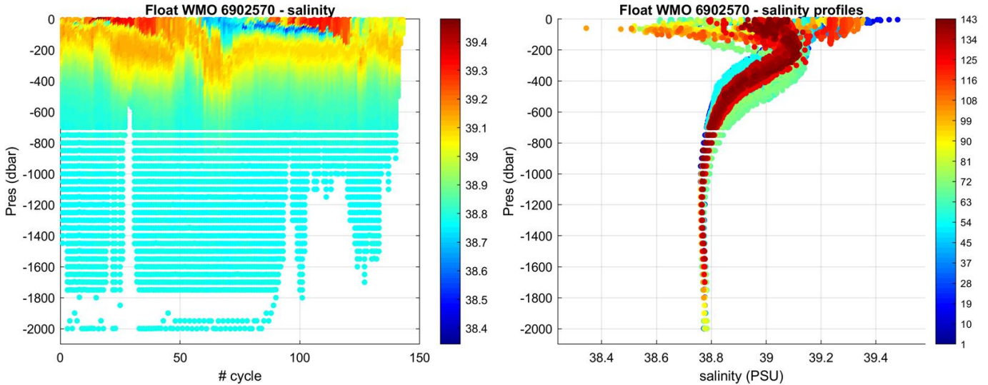
Figure 2: Float 6902570. Time series of Argo float potential salinity (PSS-78) on the left, and salinity profiles color-coded per cycle number on the right.
