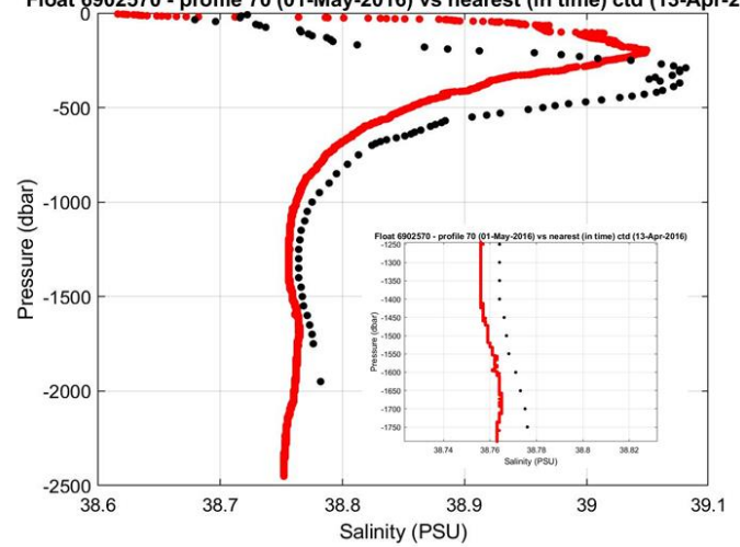
Figure 9: Float 6902570. The salinity float profile number 70 (black dots) are compared to the nearest in space (top) and in time (bottom) reference profile (red dots). In the small plots the comparison in the deeper layers is shown. The locations of the two profiles and their distance is given in the left panel.
