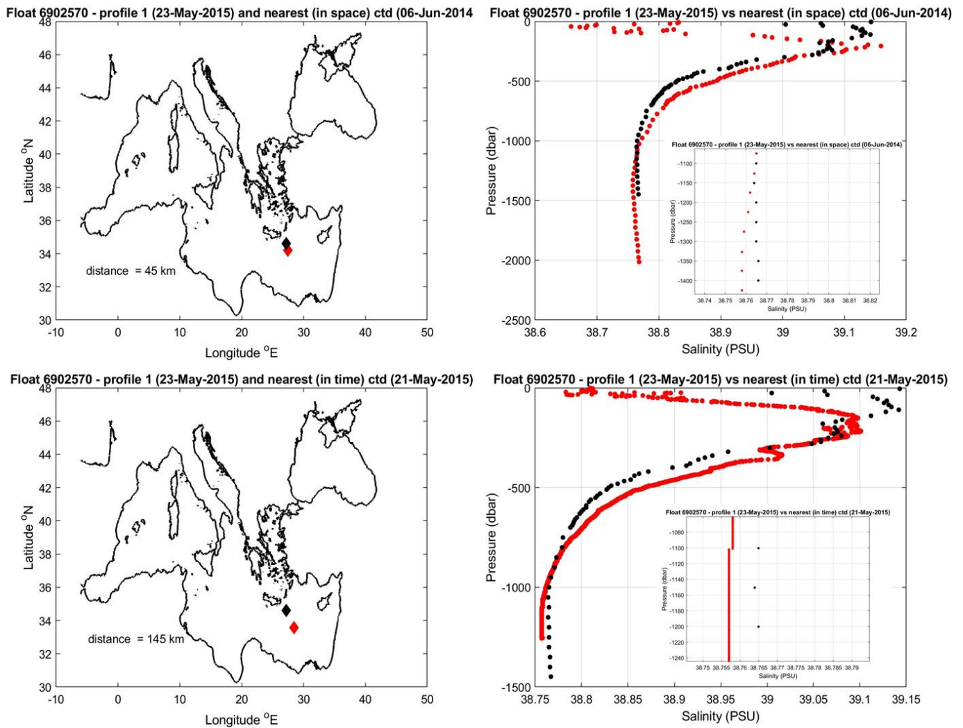
Figure 8: Float 6902570. The salinity float profile number 1 (black dots) are compared to the nearest in space (top) and in time (bottom) reference profile (red dots). In the small plots the comparison in the deeper layers is showed. The locations of the two profiles and their distance is given in the left panel.
