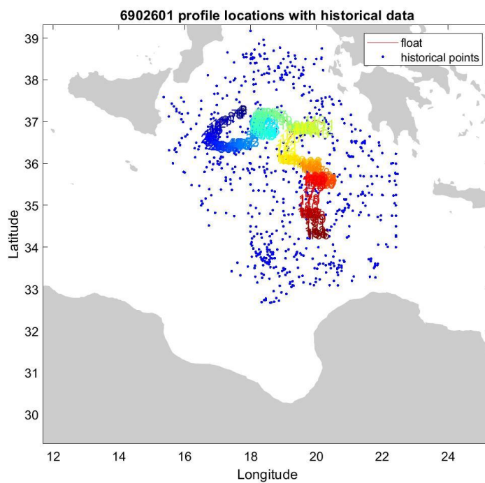
Figure 13: Float 6902601. Location of the float profiles (red line with colored numbers) and the reference data selected for mapping (blue dots).
