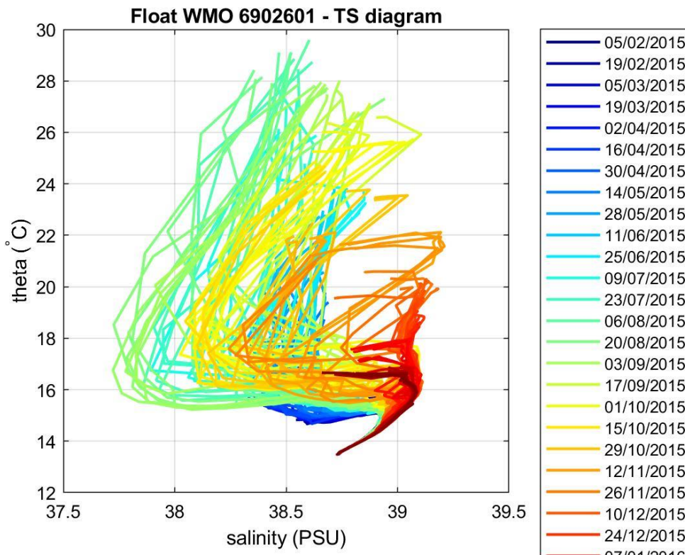
Figure 3: Float 6902601. \theta -S diagram color-coded per cycle number.
