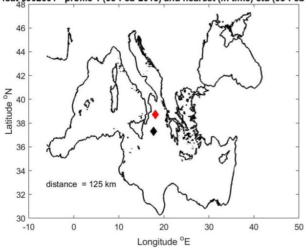
Float 6902601 - profile 1 (05-Feb-2015) and nearest (in time) ctd (05-Feb-2015)
