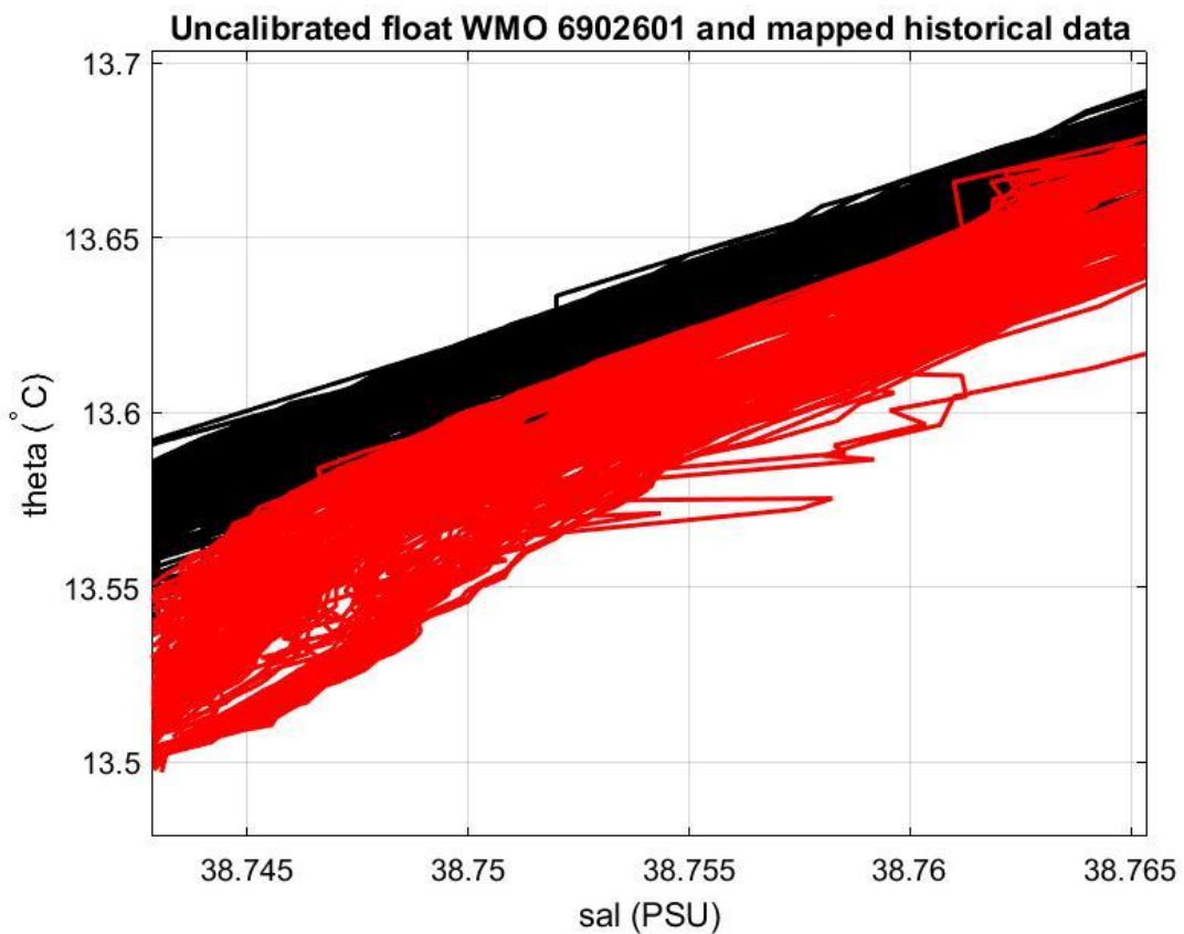
Figure 19: Float 6902601. Uncalibrated float salinity profile (black lines) and mapped historical data (red lines) in the most uniform part of the \theta -S curve.
