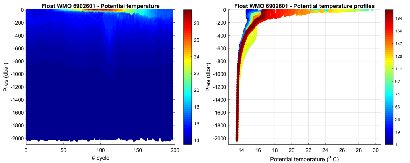
Figure 1: Float 6902601. Time series of Argo float potential temperature ( ^{\circ}\text{C} ) on the left, and potential temperature profiles color-coded per cycle number on the right.
