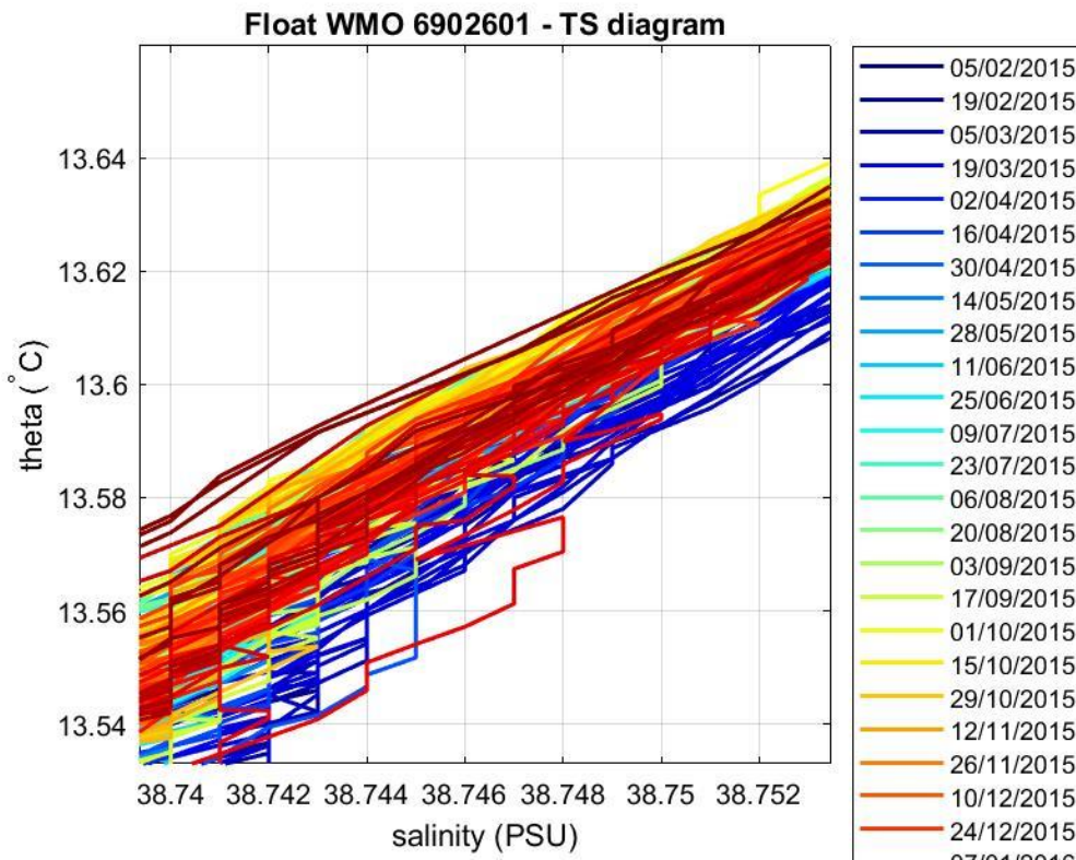
Figure 4: Float 6902601. Area of the \theta -S diagram (color-coded per cycle number) where the \theta -S relationship is more uniform.
