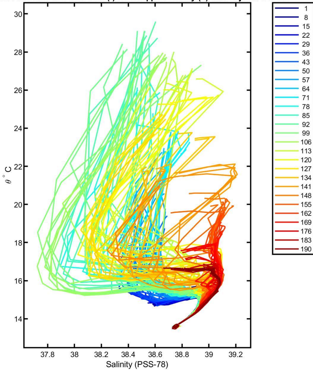
6902601 uncalibrated float data (-) and mapped salinity (o) with objective errors
