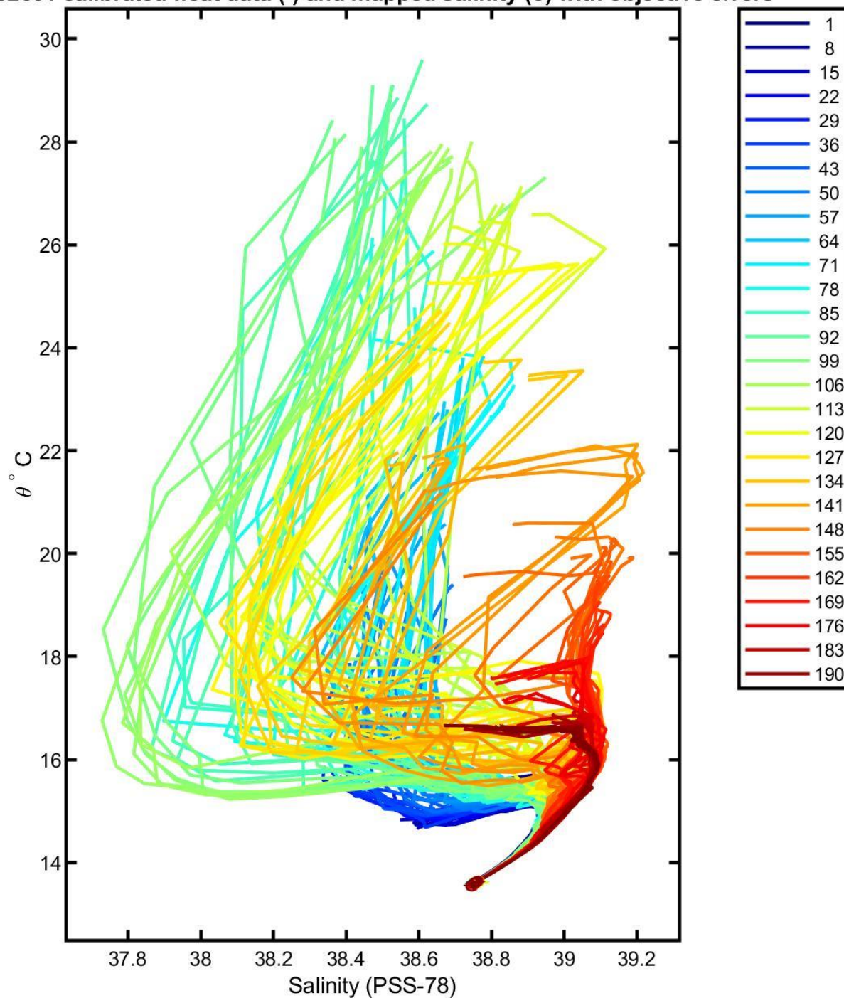
6902601 calibrated float data (-) and mapped salinity (o) with objective errors
