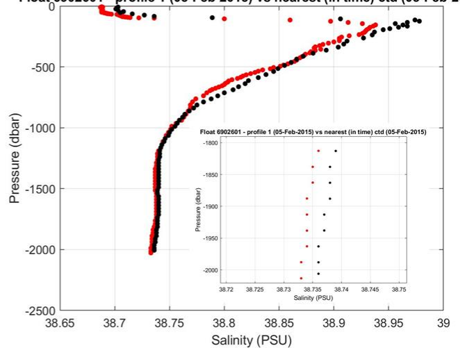
Float 6902601 - profile 1 (05-Feb-2015) vs nearest (in time) ctd (05-Feb-2015)
