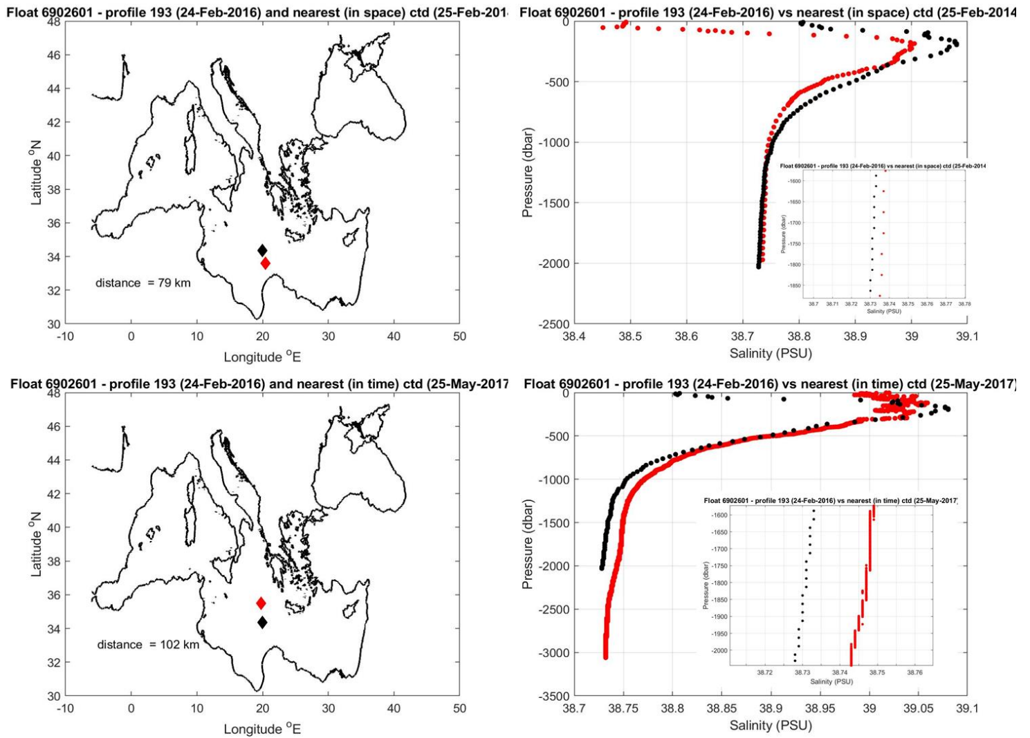
Figure 10: Float 6902601. The salinity float profile number 193 (black dots) are compared to the nearest in space (top) and in time (bottom) reference profile (red dots). In the small plots the comparison in the deeper layers is shown. The locations of the two profiles and their distance is given in the left panel.
