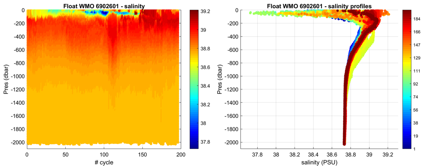
Figure 2: Float 6902601. Time series of Argo float potential salinity (PSS-78) on the left, and salinity profiles color-coded per cycle number on the right.
