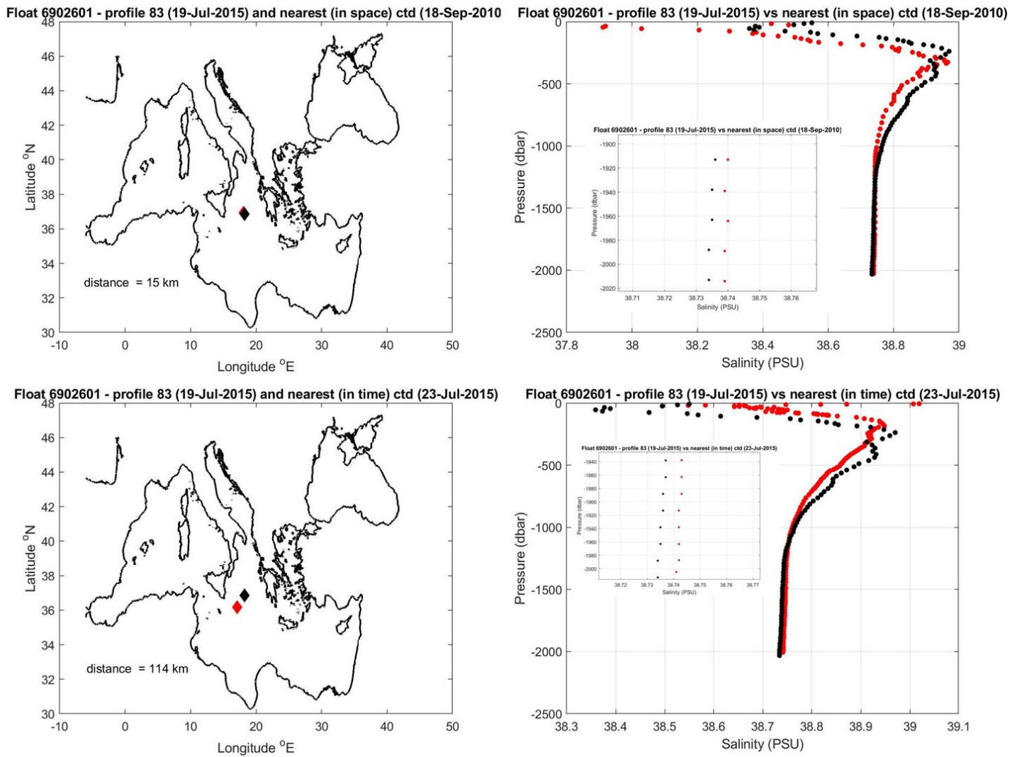
Figure 9: Float 6902601. The salinity float profile number 83 (black dots) are compared to the nearest in space (top) and in time (bottom) reference profile (red dots). In the small plots the comparison in the deeper layers is showed. The locations of the two profiles and their distance is given in the left panel.
