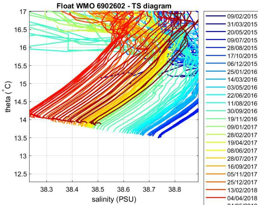
Figure 4: Float 6902602. Area of the \theta -S diagram (color-coded per cycle number) where the \theta -S relationship is more uniform.
