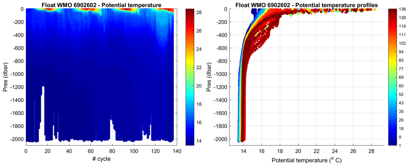
Figure 1: Float 6902602. Time series of Argo float potential temperature ( ^{\circ}\text{C} ) on the left, and potential temperature profiles color-coded per cycle number on the right.
