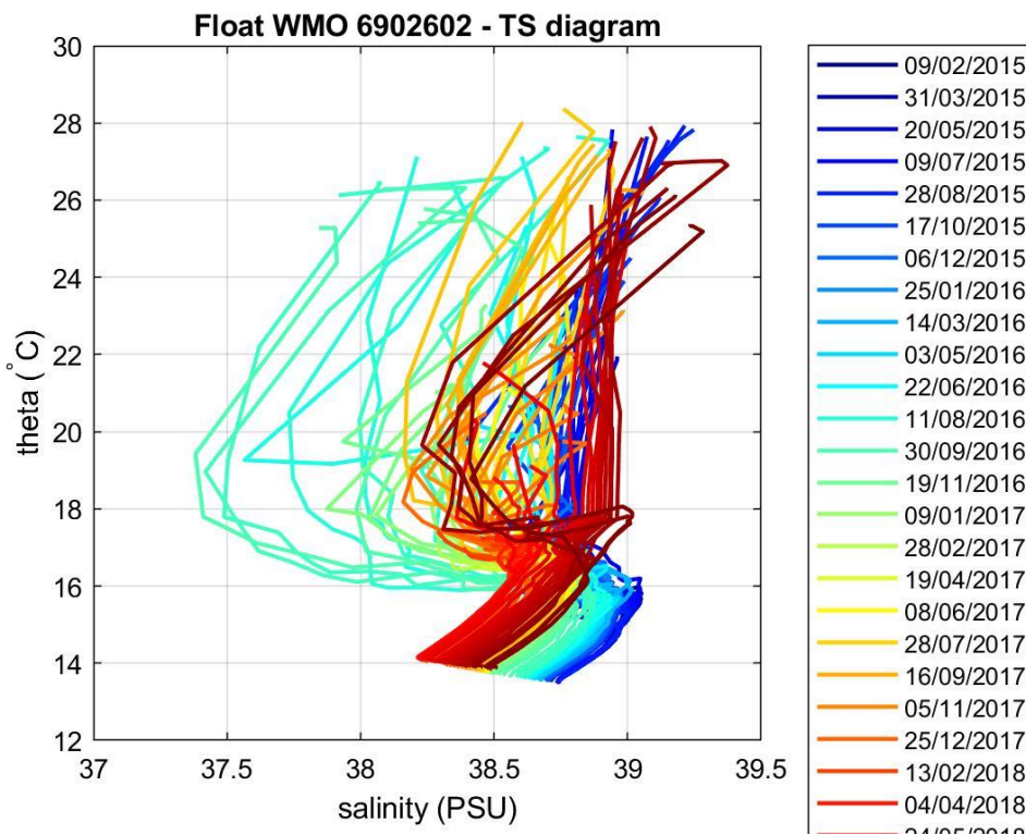
Figure 3: Float 6902602. \theta -S diagram color-coded per cycle number.
