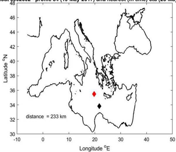
Float 6902602 - profile 84 (19-May-2017) and nearest (in time) ctd (25-May-2017)
