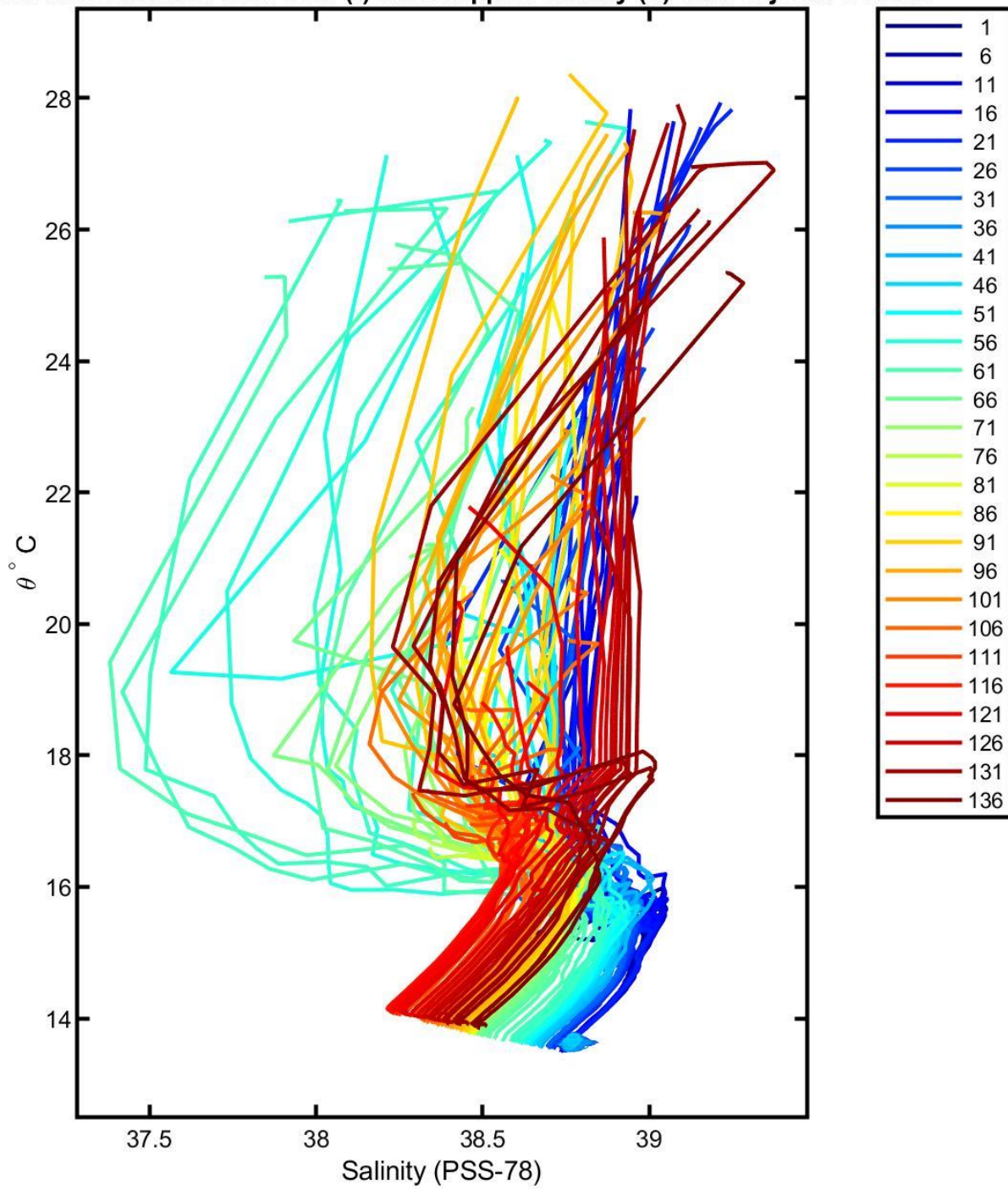
6902602 uncalibrated float data (-) and mapped salinity (o) with objective errors
