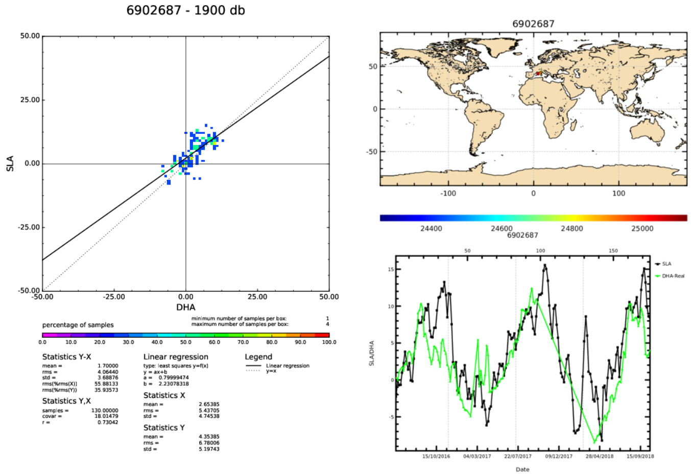
Figure 1: Float 6902687. The comparison between the sea surface height (SSH) from the satellite altimetry and dynamic height anomaly (DHA) extracted from the Argo float temperature and salinity. The figure is created by the CLS/Coriolis and distributed by Ifremer ( ftp://ftp.ifremer.fr/ifremer/argo/etc/argo-ast9-item13-AltimeterComparison/figures/ ).
