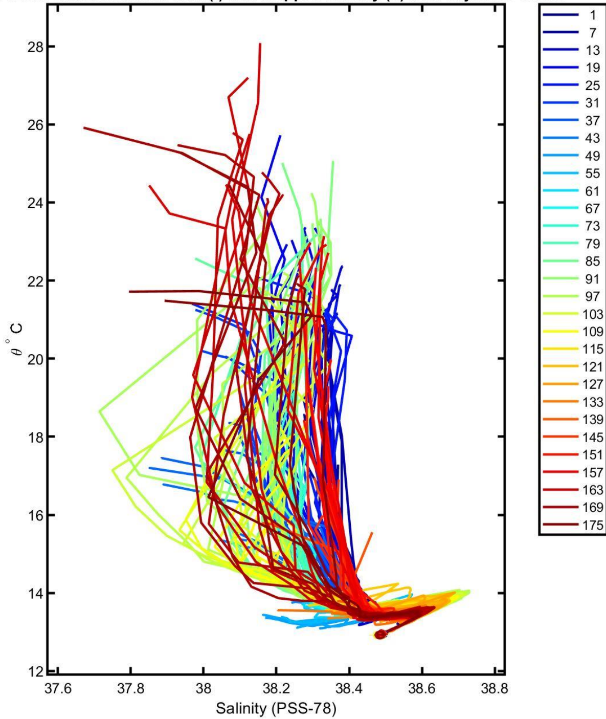
6902687 calibrated float data (-) and mapped salinity (o) with objective errors
