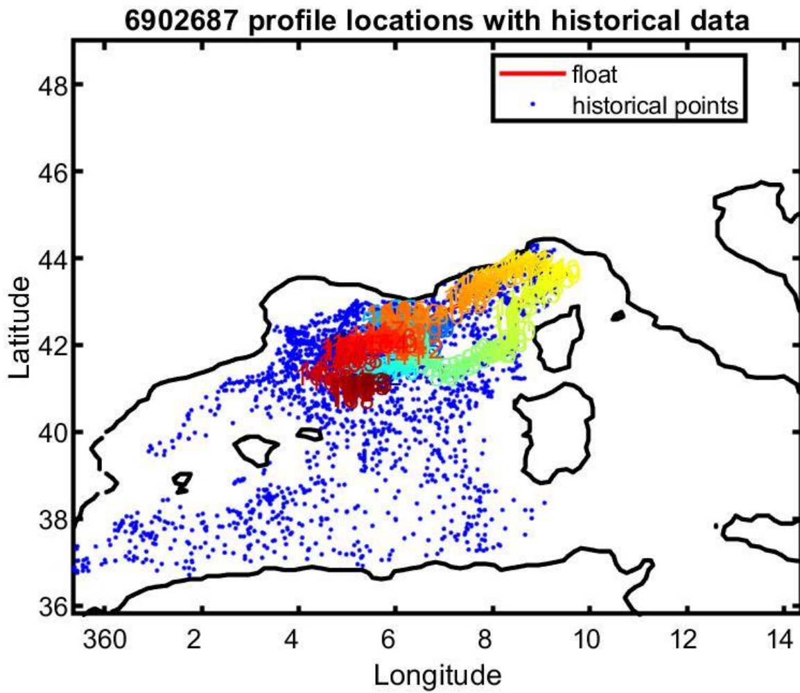
Figure 13: Float 6902687. Location of the float profiles (red line with colored numbers) and the reference data selected for mapping (blue dots).
