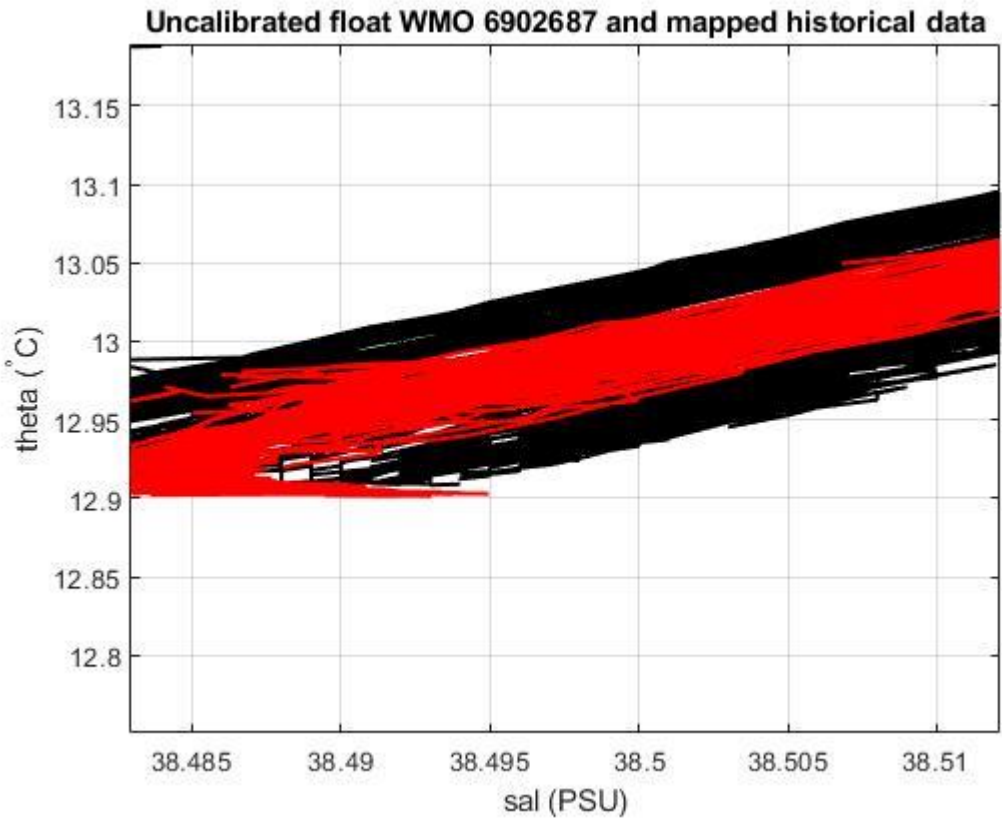
Figure 19: Float 6902687. Uncalibrated float salinity profile (black lines) and mapped historical data (red lines) in the most uniform part of the \theta -S curve.
