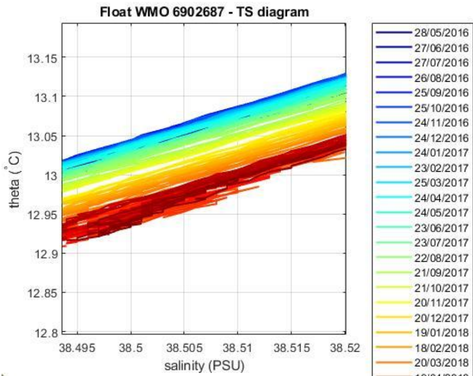
Figure 5: Float 6902687. Area of the \theta -S diagram (color-coded per cycle number) where the \theta -S relationship is more uniform.
