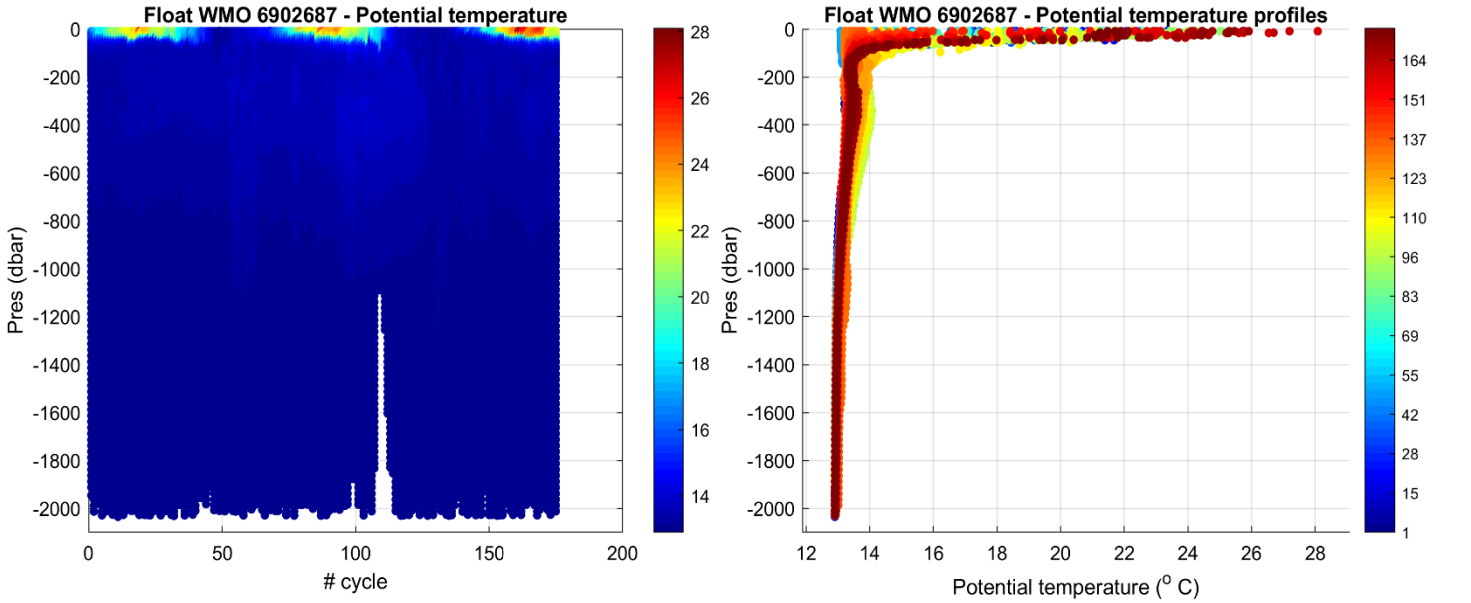
Figure 2: Float 6902687. Time series of Argo float potential temperature ( ^{\circ}\text{C} ) on the left, and potential temperature profiles color-coded per cycle number on the right.
