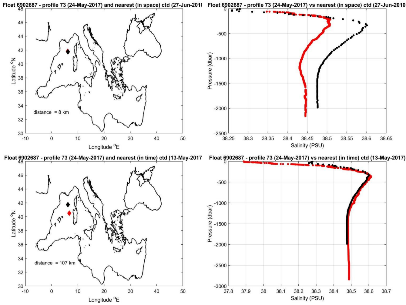
Figure 10: Float 6902687. The salinity float profile number 73 (black dots) are compared to the nearest in space (top) and in time (bottom) reference profile (red dots). The locations of the two profiles and their distance is given in the left panel.
