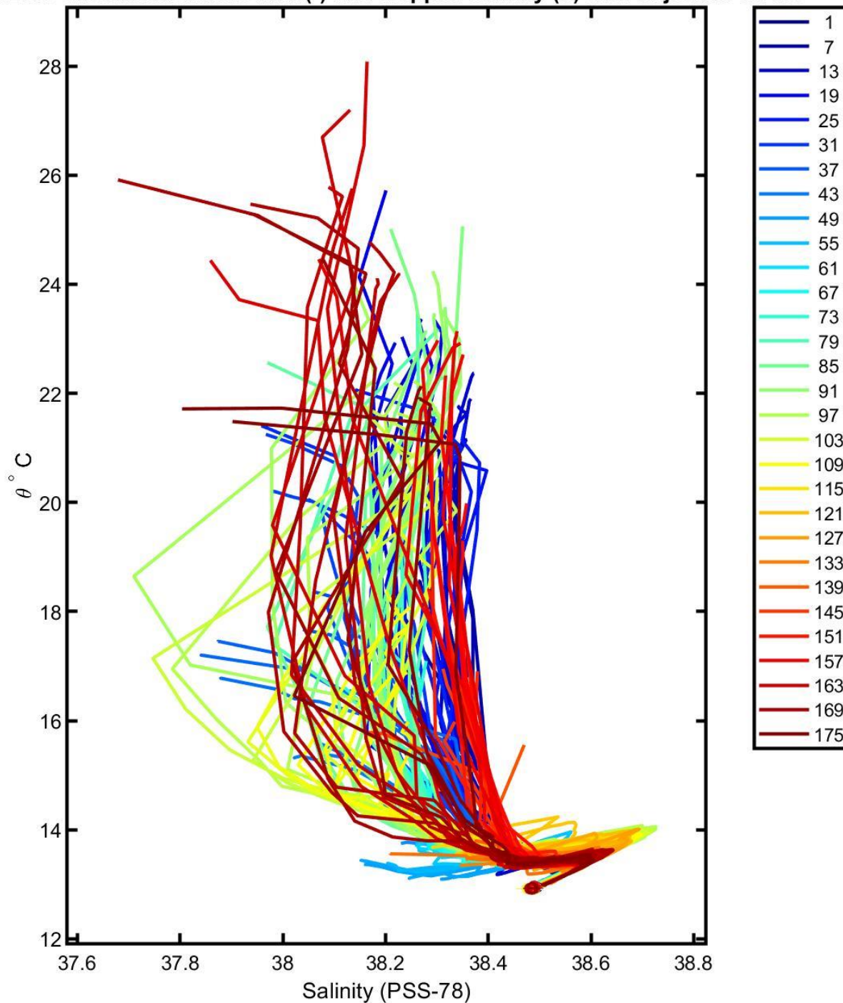
6902687 uncalibrated float data (-) and mapped salinity (o) with objective errors
