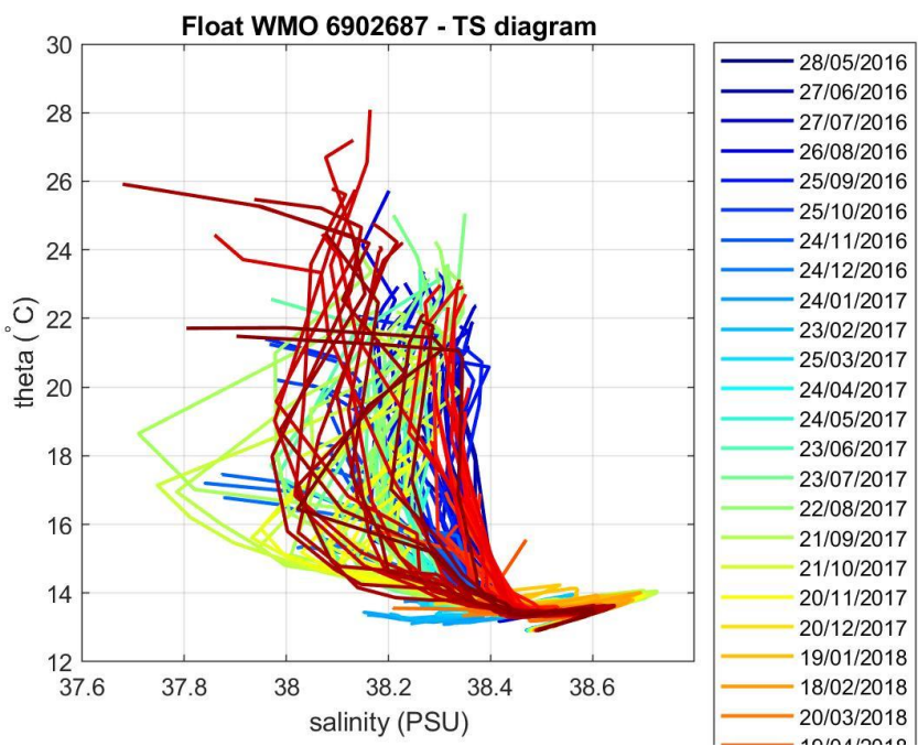
Figure 4: Float 6902687. \theta -S diagram color-coded per cycle number.
