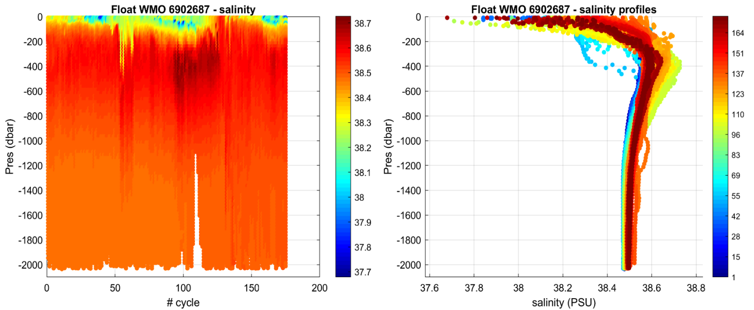
Figure 3: Float 6902687. Time series of Argo float potential salinity (PSS-78) on the left, and salinity profiles color-coded per cycle number on the right.
