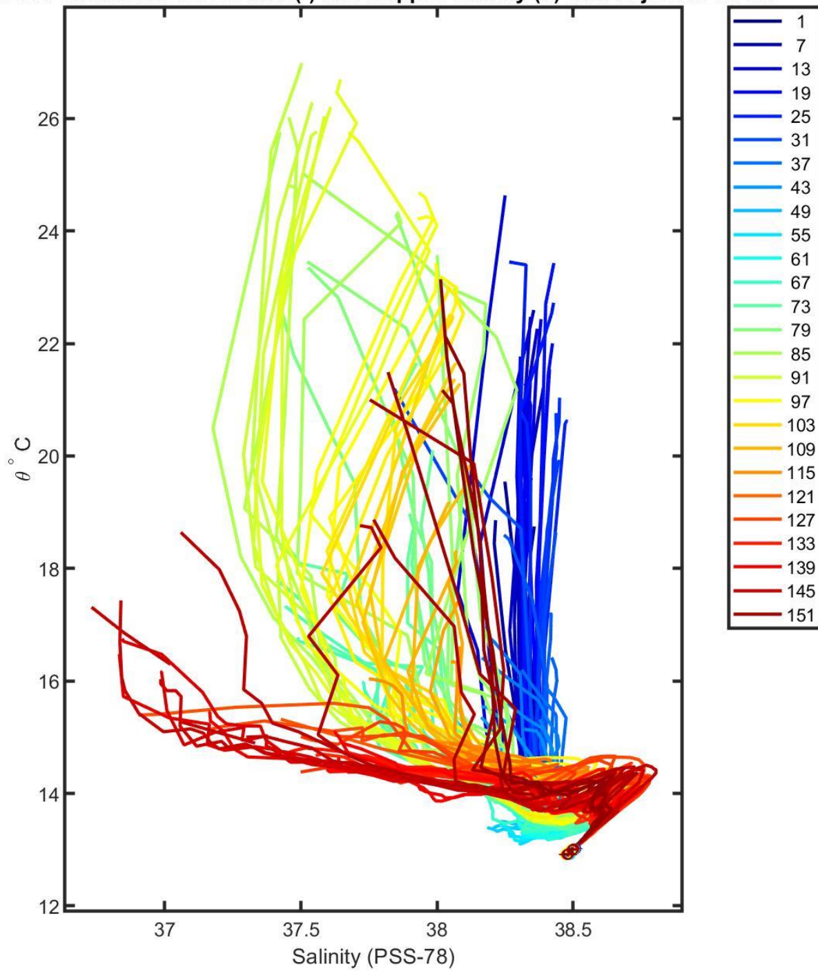
6902688 uncalibrated float data (-) and mapped salinity (o) with objective errors
