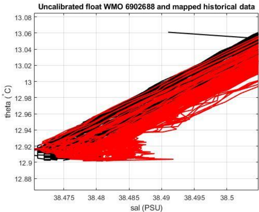
Figure 19: Float 6902688. Uncalibrated float salinity profile (black lines) and mapped historical data (red lines) in the most uniform part of the \theta -S curve.
