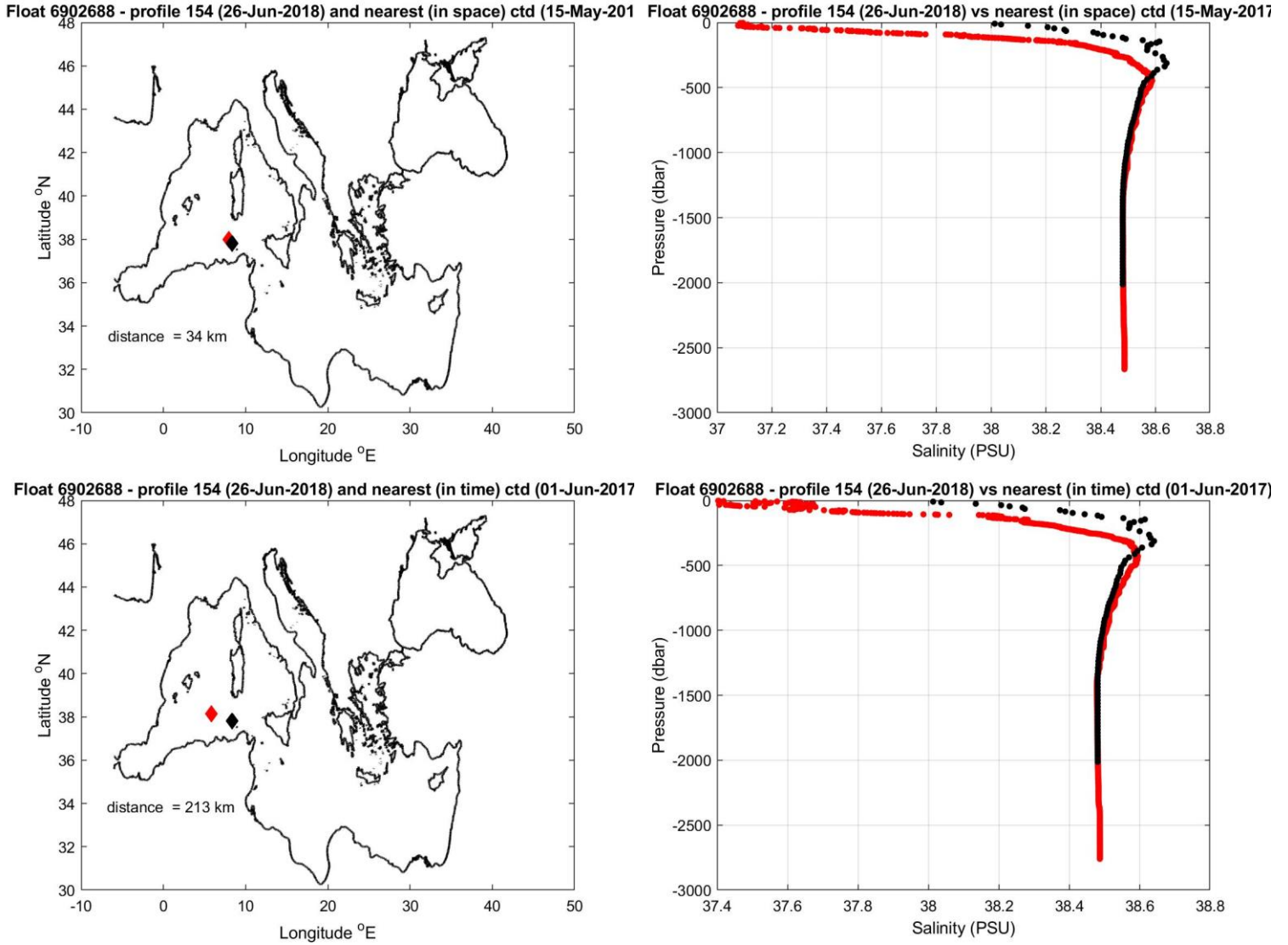
Figure 11: Float 6902688. The salinity float profile number 154 (black dots) are compared to the nearest in space (top) and in time (bottom) reference profile (red dots). The locations of the two profiles and their distance is given in the left panel.
