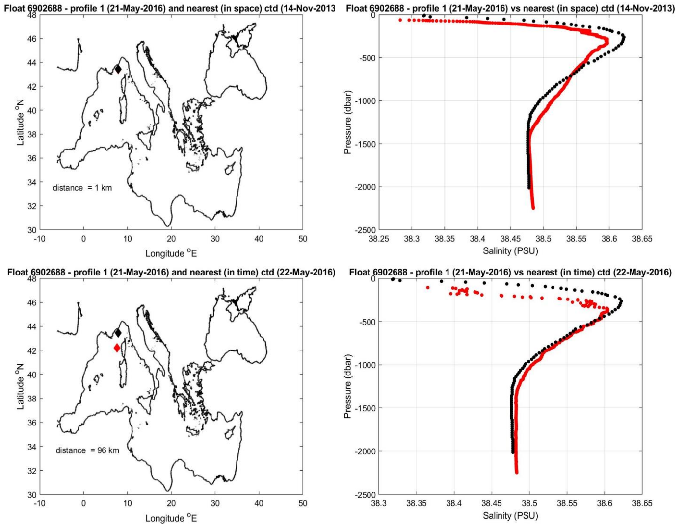
Figure 9: Float 6902688. The salinity float profile number 1 (black dots) are compared to the nearest in space (top) and in time (bottom) reference profile (red dots). The locations of the two profiles and their distance is given in the left panel.
