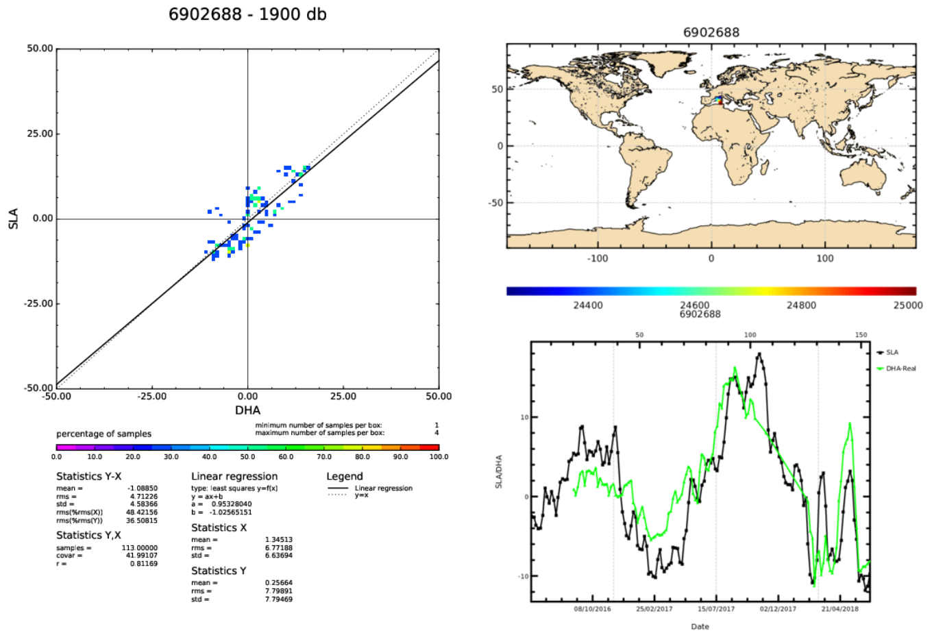
Figure 1: Float 6902688. The comparison between the sea surface height (SSH) from the satellite altimetry and dynamic height anomaly (DHA) extracted from the Argo float temperature and salinity. The figure is created by the CLS/Coriolis and distributed by Ifremer ( ftp://ftp.ifremer.fr/ifremer/argo/etc/argo-ast9-item13-AltimeterComparison/figures/ ).
