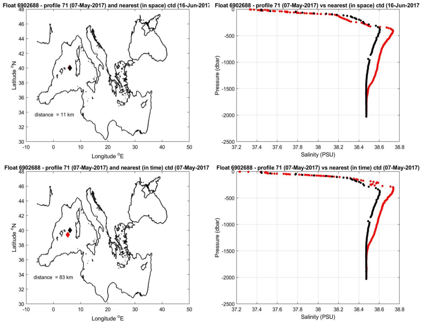
Figure 10: Float 6902688. The salinity float profile number 71 (black dots) are compared to the nearest in space (top) and in time (bottom) reference profile (red dots). The locations of the two profiles and their distance is given in the left panel.
