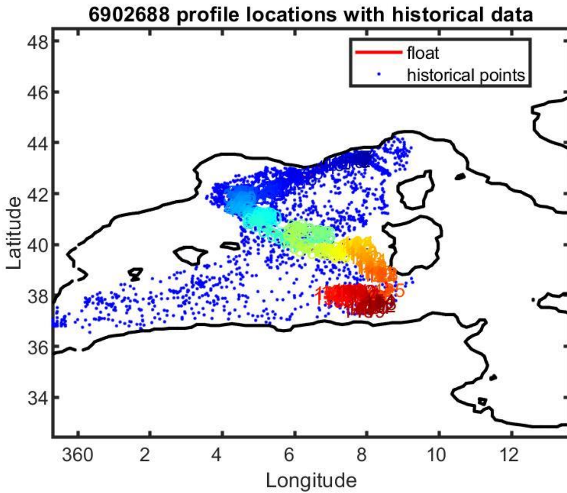
Figure 13: Float 6902688. Location of the float profiles (red line with colored numbers) and the reference data selected for mapping (blue dots).
