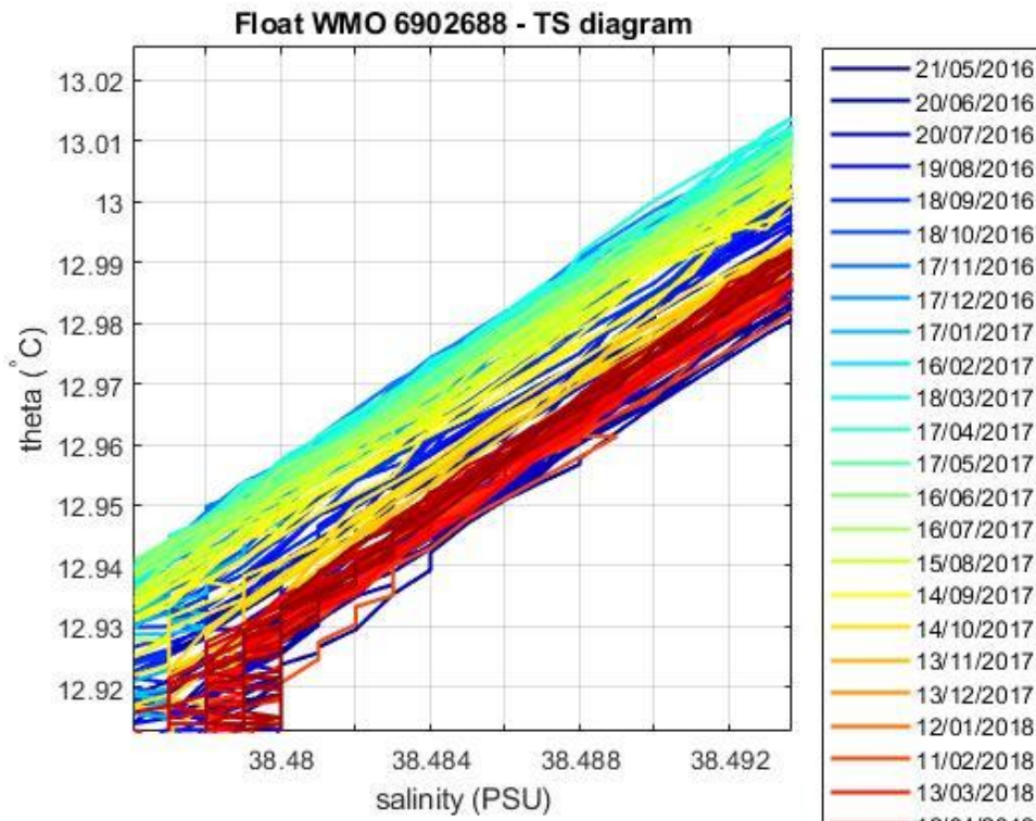
Figure 5: Float 6902688. Area of the \theta -S diagram (color-coded per cycle number) where the \theta -S relationship is more uniform.
