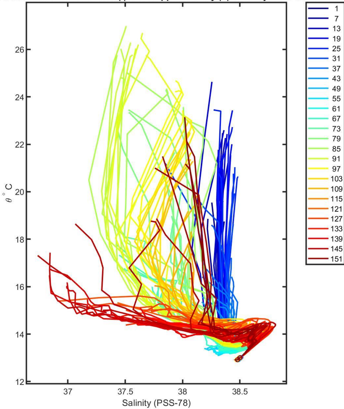
6902688 calibrated float data (-) and mapped salinity (o) with objective errors
