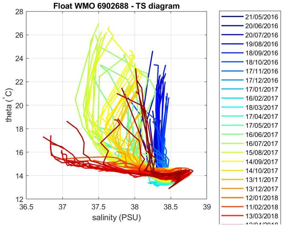
Figure 4: Float 6902688. \theta -S diagram color-coded per cycle number.
