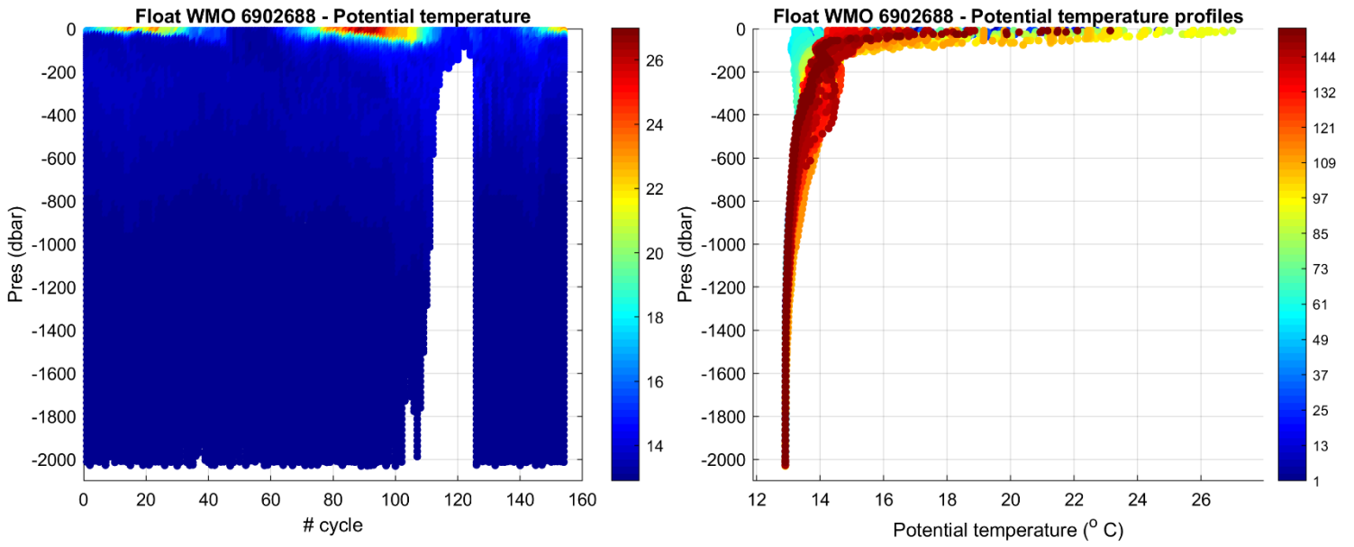
Figure 2: Float 6902688. Time series of Argo float potential temperature ( ^{\circ}\text{C} ) on the left, and potential temperature profiles color-coded per cycle number on the right.
