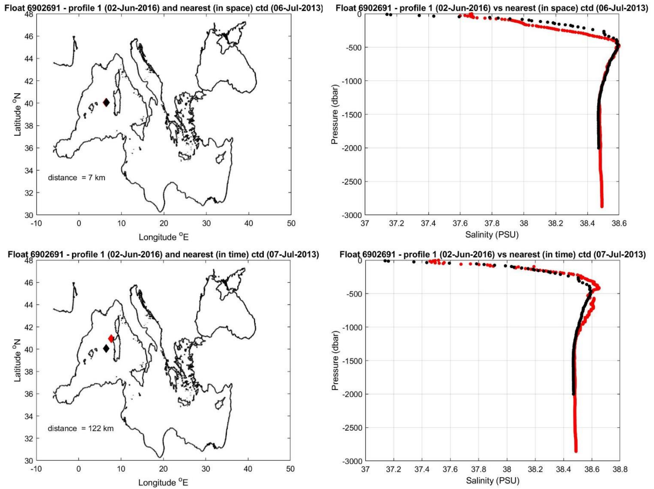
Figure 9: Float 6902691. The salinity float profile number 1 (black dots) are compared to the nearest in space (top) and in time (bottom) reference profile (red dots). The locations of the two profiles and their distance is given in the left panel.
