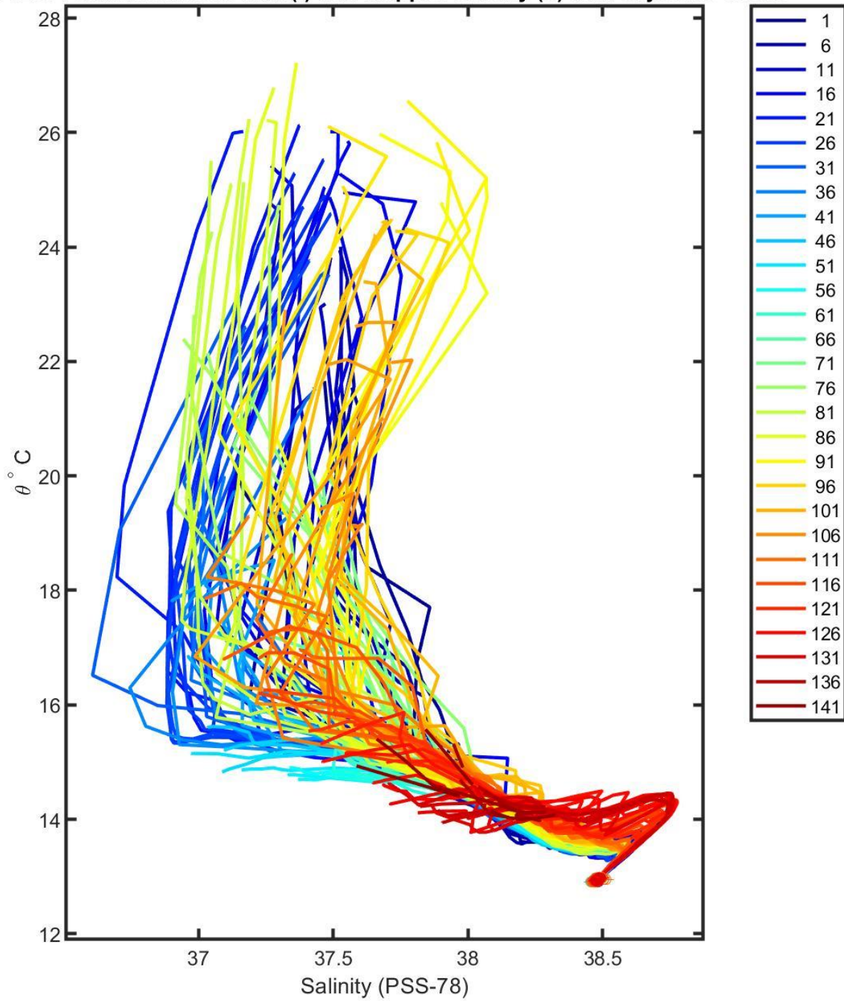
6902691 calibrated float data (-) and mapped salinity (o) with objective errors
