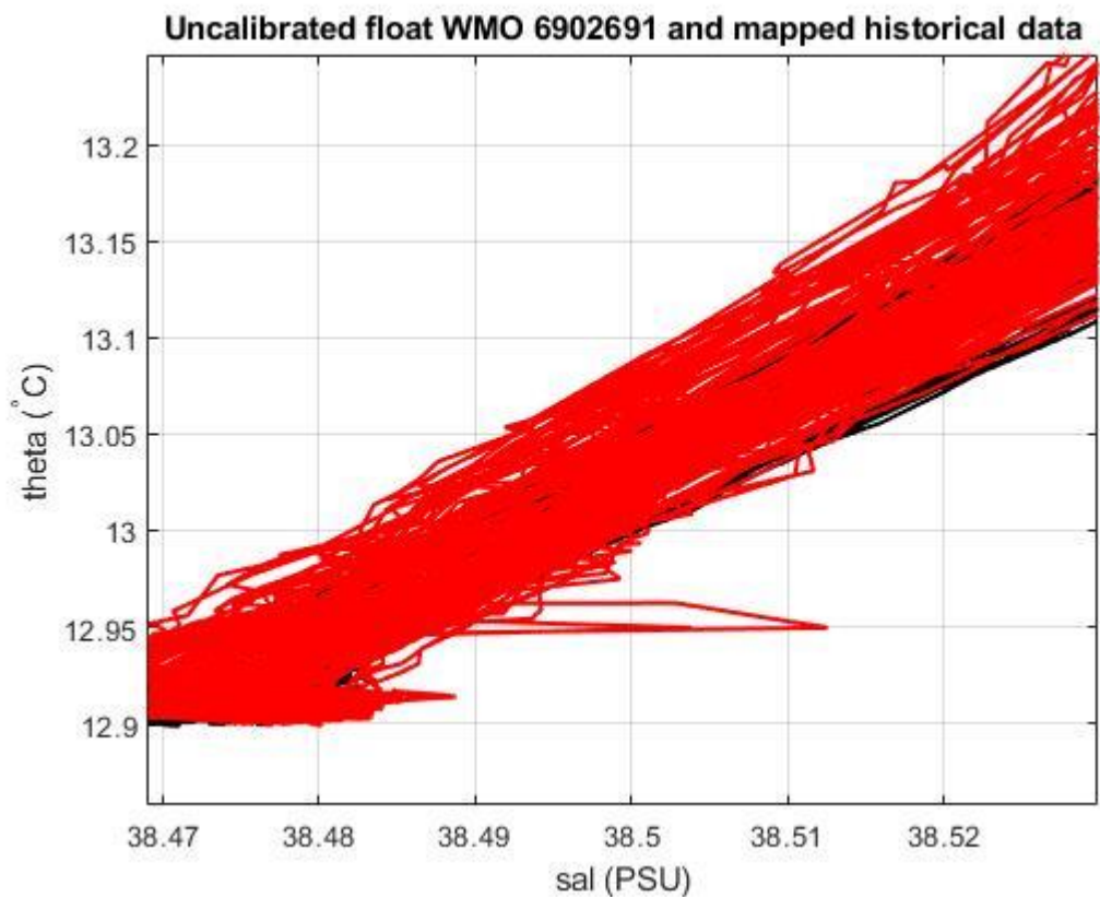
Figure 19: Float 6902691. Uncalibrated float salinity profile (black lines) and mapped historical data (red lines) in the most uniform part of the \theta -S curve.
