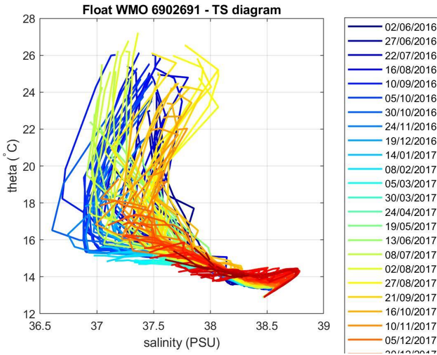
Figure 4: Float 6902691. \theta -S diagram color-coded per cycle number.
