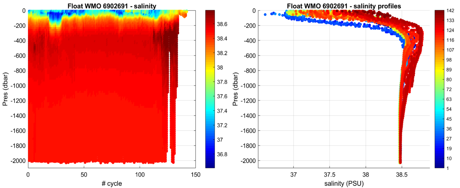
Figure 3: Float 6902691. Time series of Argo float potential salinity (PSS-78) on the left, and salinity profiles color-coded per cycle number on the right.
