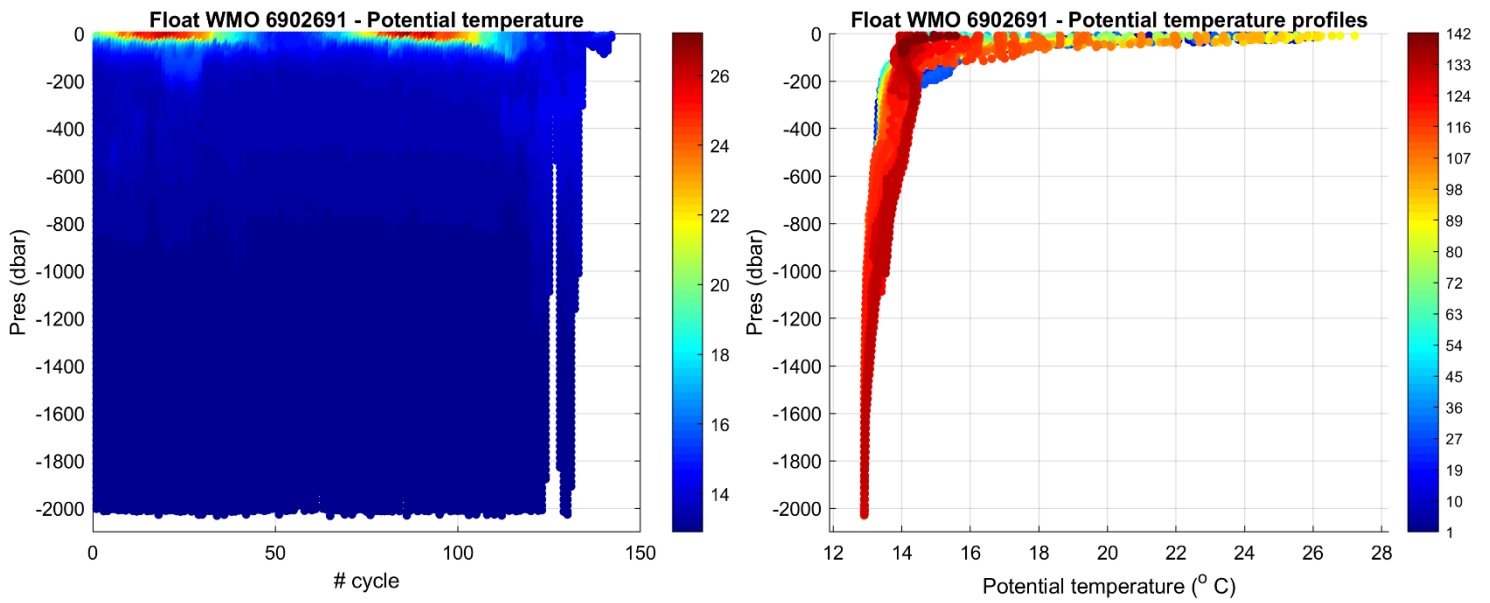
Figure 2: Float 6902691. Time series of Argo float potential temperature ( ^{\circ}\text{C} ) on the left, and potential temperature profiles color-coded per cycle number on the right.
