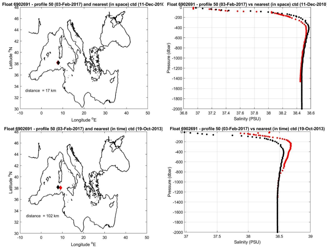
Figure 10: Float 6902691. The salinity float profile number 50 (black dots) are compared to the nearest in space (top) and in time (bottom) reference profile (red dots). The locations of the two profiles and their distance is given in the left panel.
