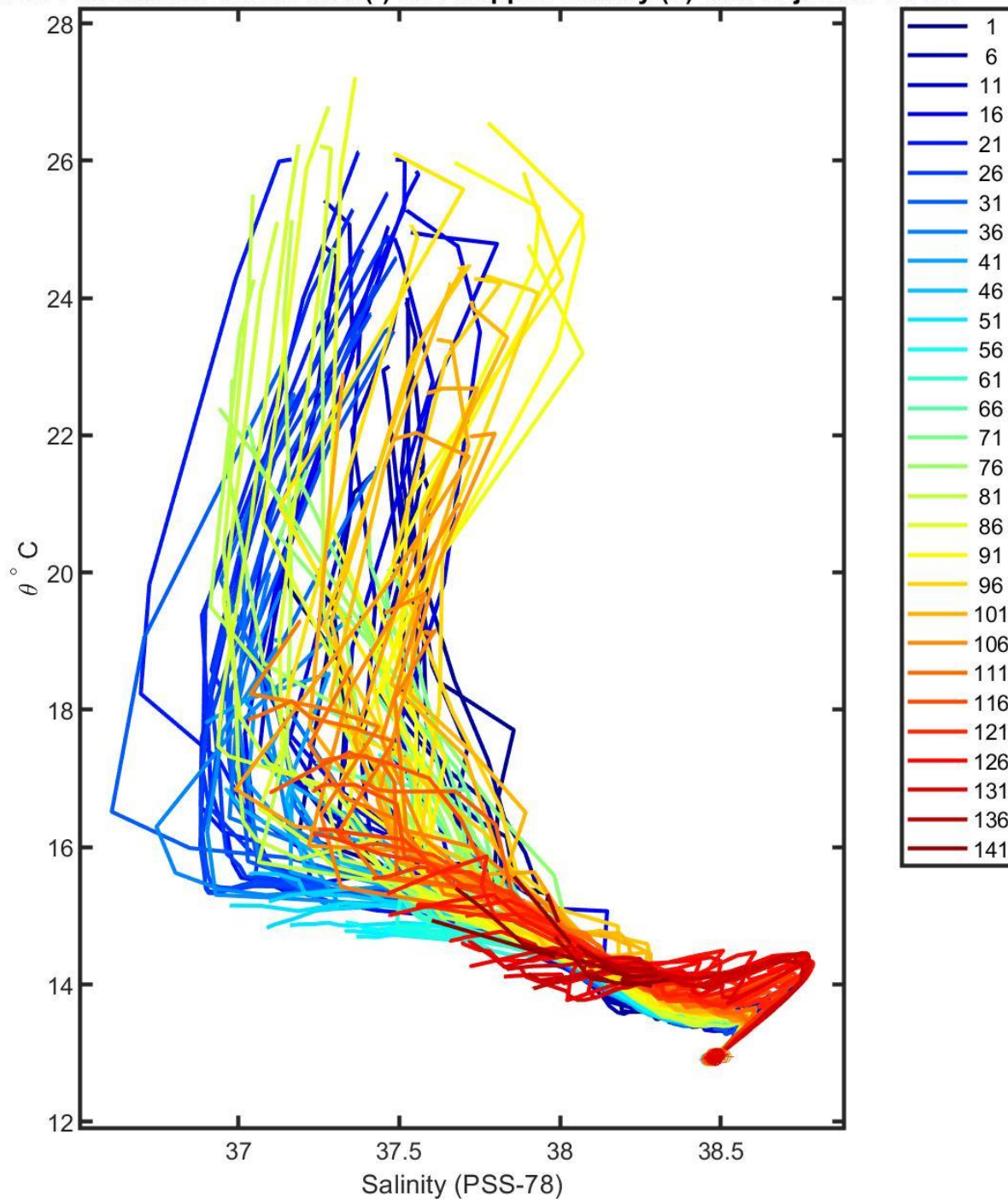
6902691 uncalibrated float data (-) and mapped salinity (o) with objective errors
