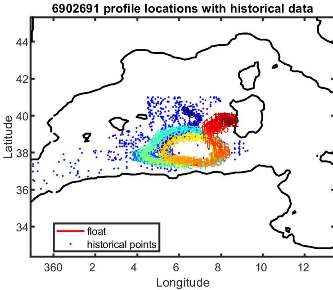
Figure 13: Float 6902691. Location of the float profiles (red line with colored numbers) and the reference data selected for mapping (blue dots).
