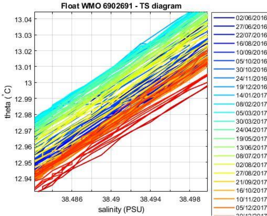
Figure 5: Float 6902691. Area of the \theta -S diagram (color-coded per cycle number) where the \theta -S relationship is more uniform.
