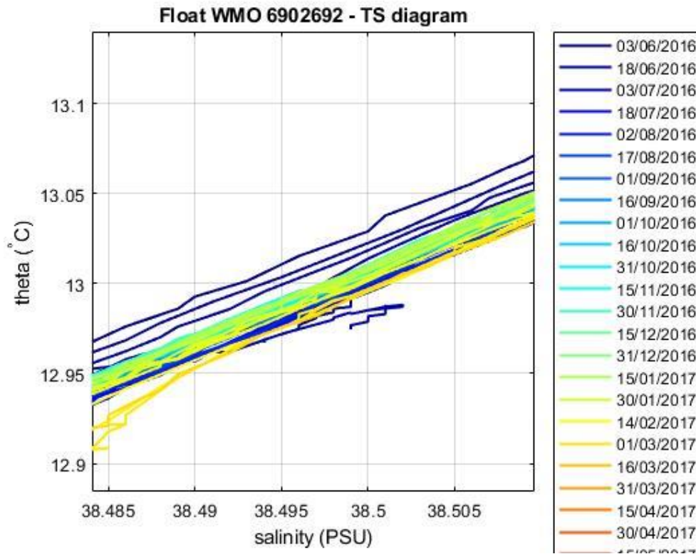
Figure 5: Float 6902692. Area of the \theta -S diagram (color-coded per cycle number) where the \theta -S relationship is more uniform.
