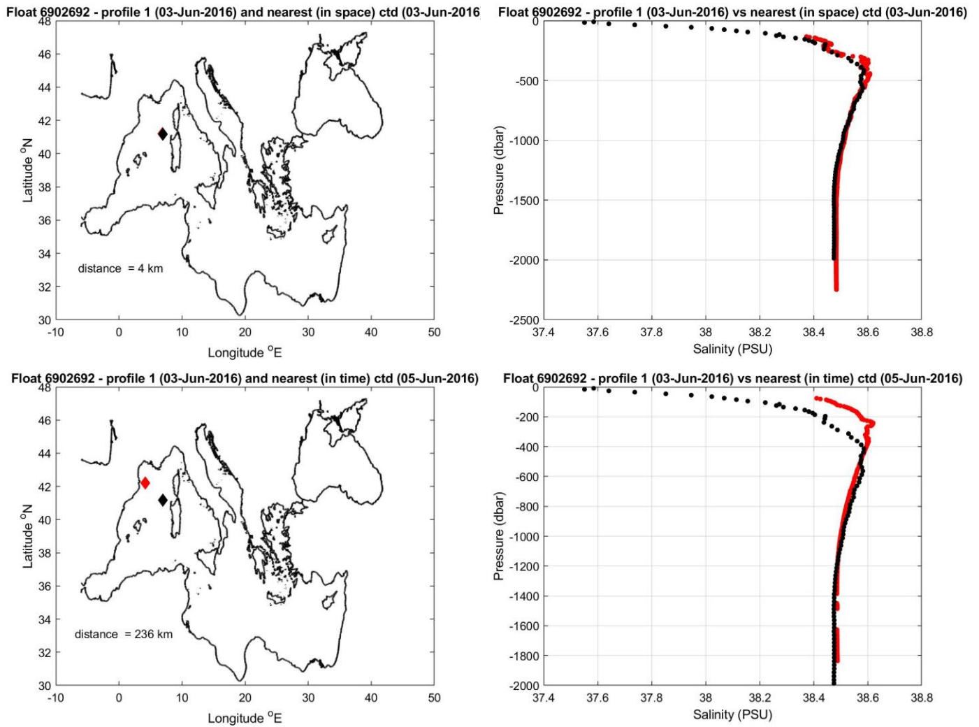
Figure 9: Float 6902692. The salinity float profile number 1 (black dots) are compared to the nearest in space (top) and in time (bottom) reference profile (red dots). The locations of the two profiles and their distance is given in the left panel.
