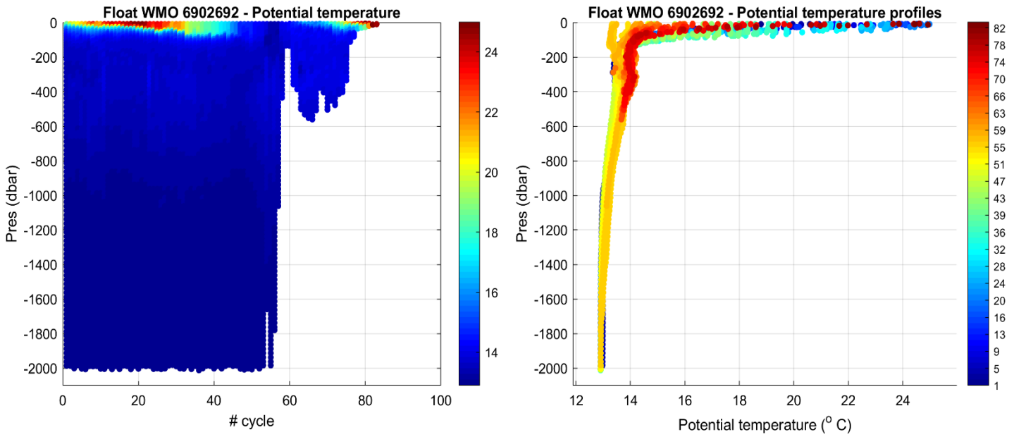
Figure 2: Float 6902692. Time series of Argo float potential temperature ( ^{\circ}\text{C} ) on the left, and potential temperature profiles color-coded per cycle number on the right.
