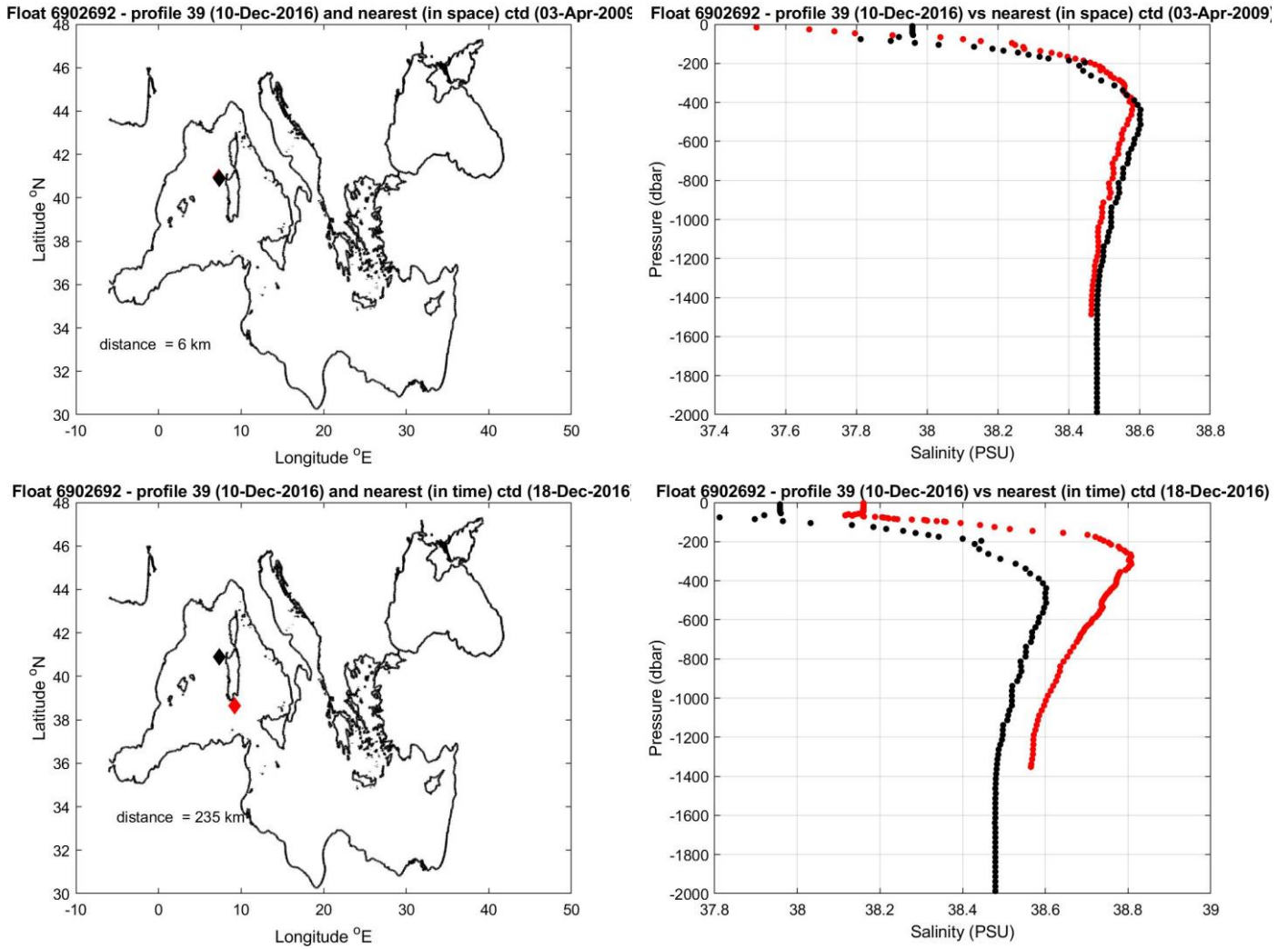
Figure 10: Float 6902692. The salinity float profile number 39 (black dots) are compared to the nearest in space (top) and in time (bottom) reference profile (red dots). The locations of the two profiles and their distance is given in the left panel.
