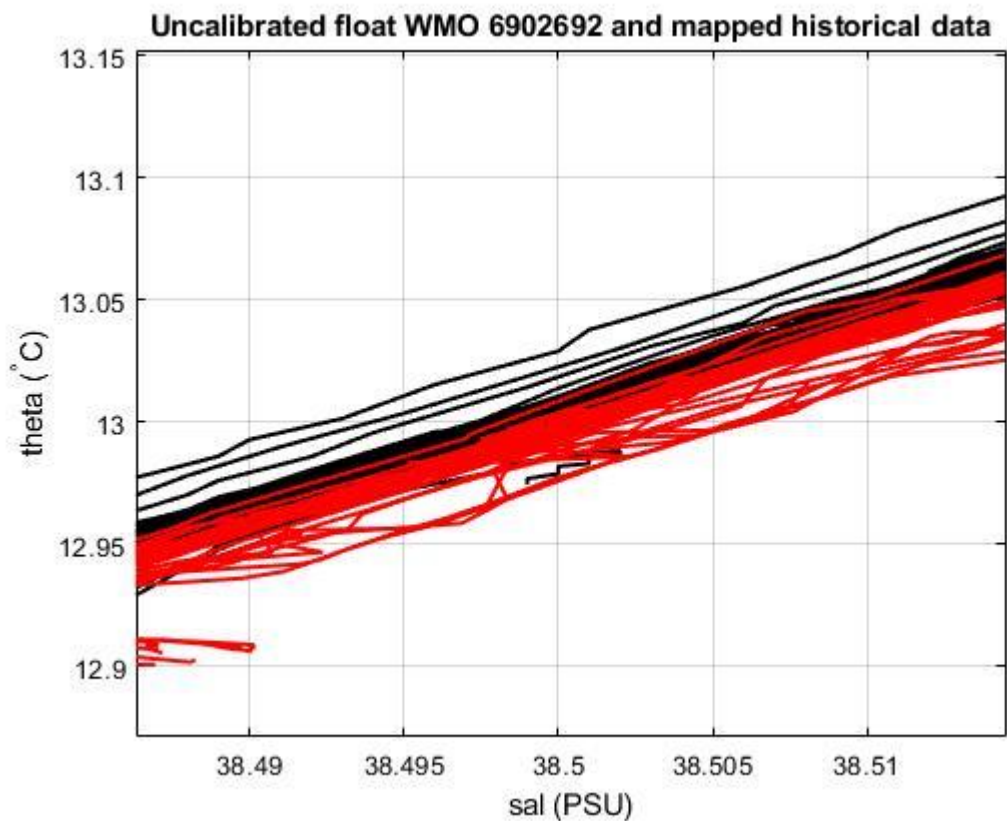
Figure 19: Float 6902692. Uncalibrated float salinity profile (black lines) and mapped historical data (red lines) in the most uniform part of the \theta -S curve.
