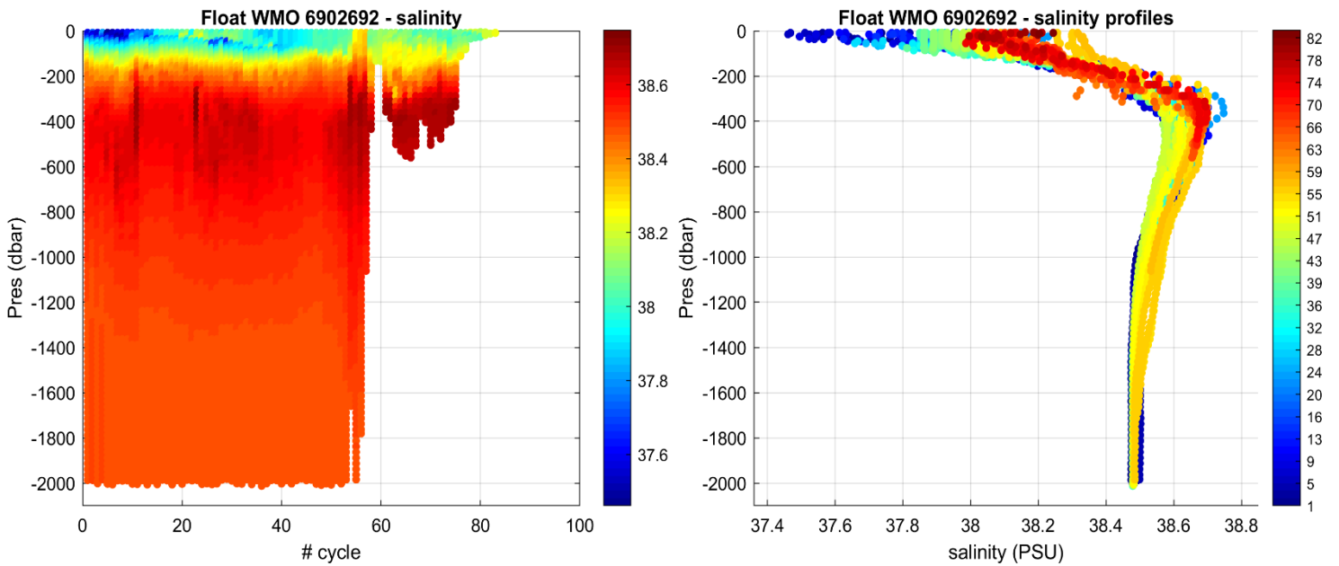
Figure 3: Float 6902692. Time series of Argo float potential salinity (PSS-78) on the left, and salinity profiles color-coded per cycle number on the right.
