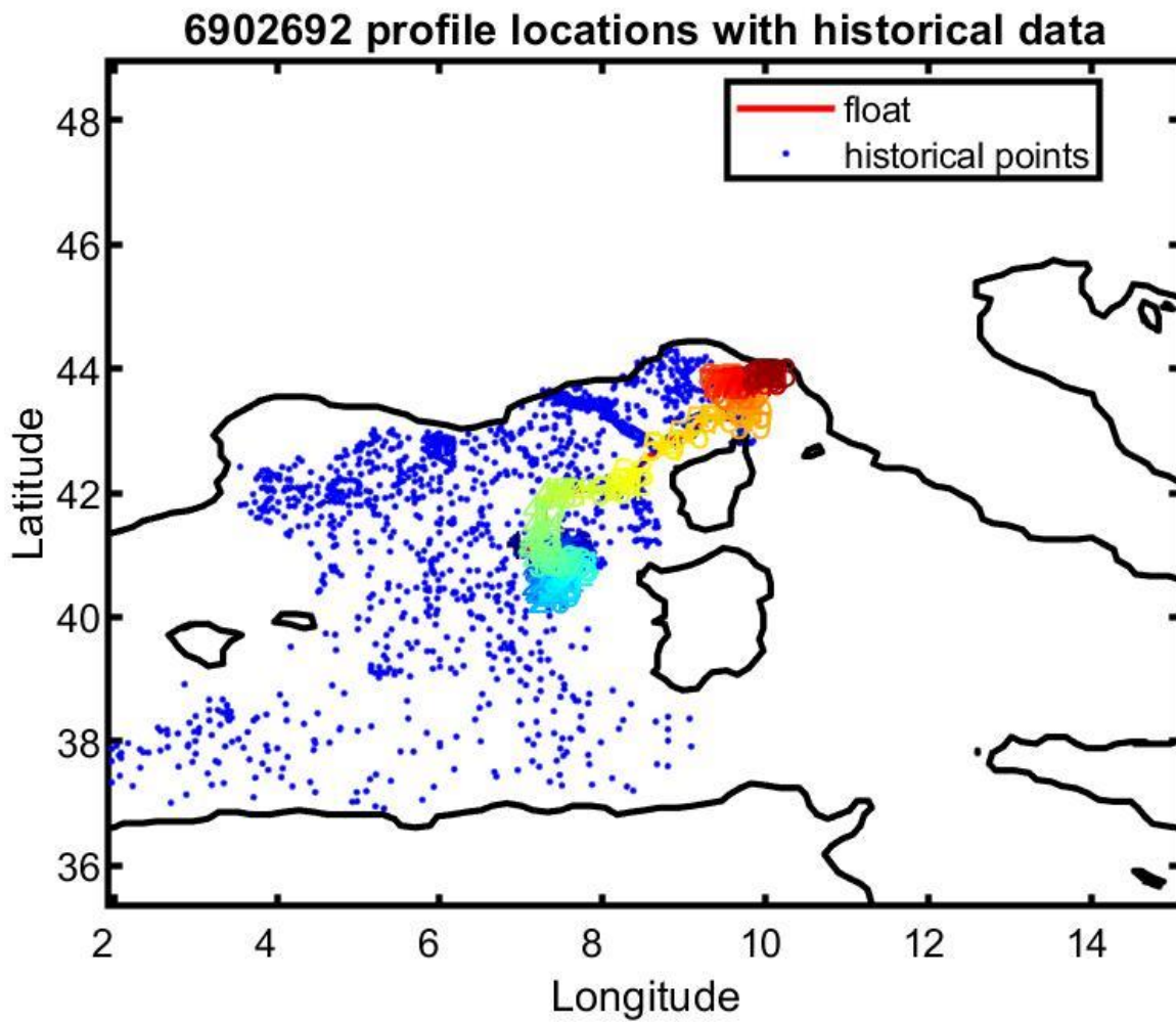
Figure 13: Float 6902692. Location of the float profiles (red line with colored numbers) and the reference data selected for mapping (blue dots).
