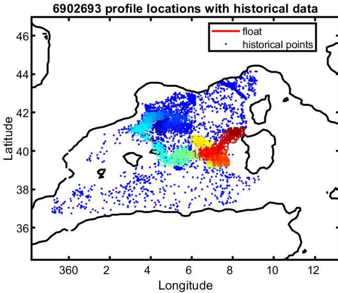
Figure 13: Float 6902693. Location of the float profiles (red line with colored numbers) and the reference data selected for mapping (blue dots).
