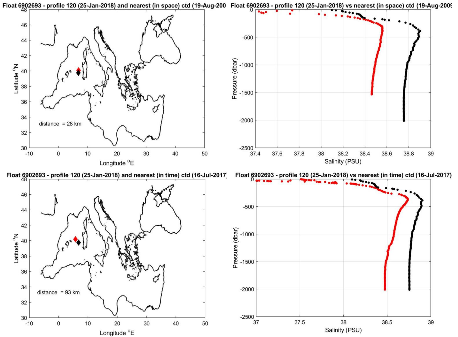
Figure 11: Float 6902693. The salinity float profile number 120 (black dots) are compared to the nearest in space (top) and in time (bottom) reference profile (red dots). The locations of the two profiles and their distance is given in the left panel.
