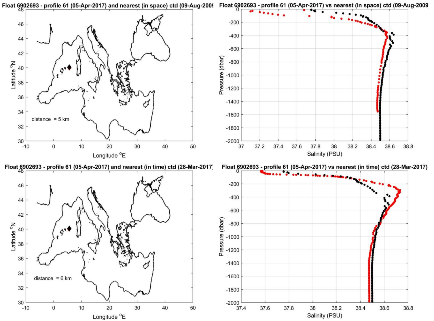
Figure 10: Float 6902693. The salinity float profile number 61 (black dots) are compared to the nearest in space (top) and in time (bottom) reference profile (red dots). The locations of the two profiles and their distance is given in the left panel.
