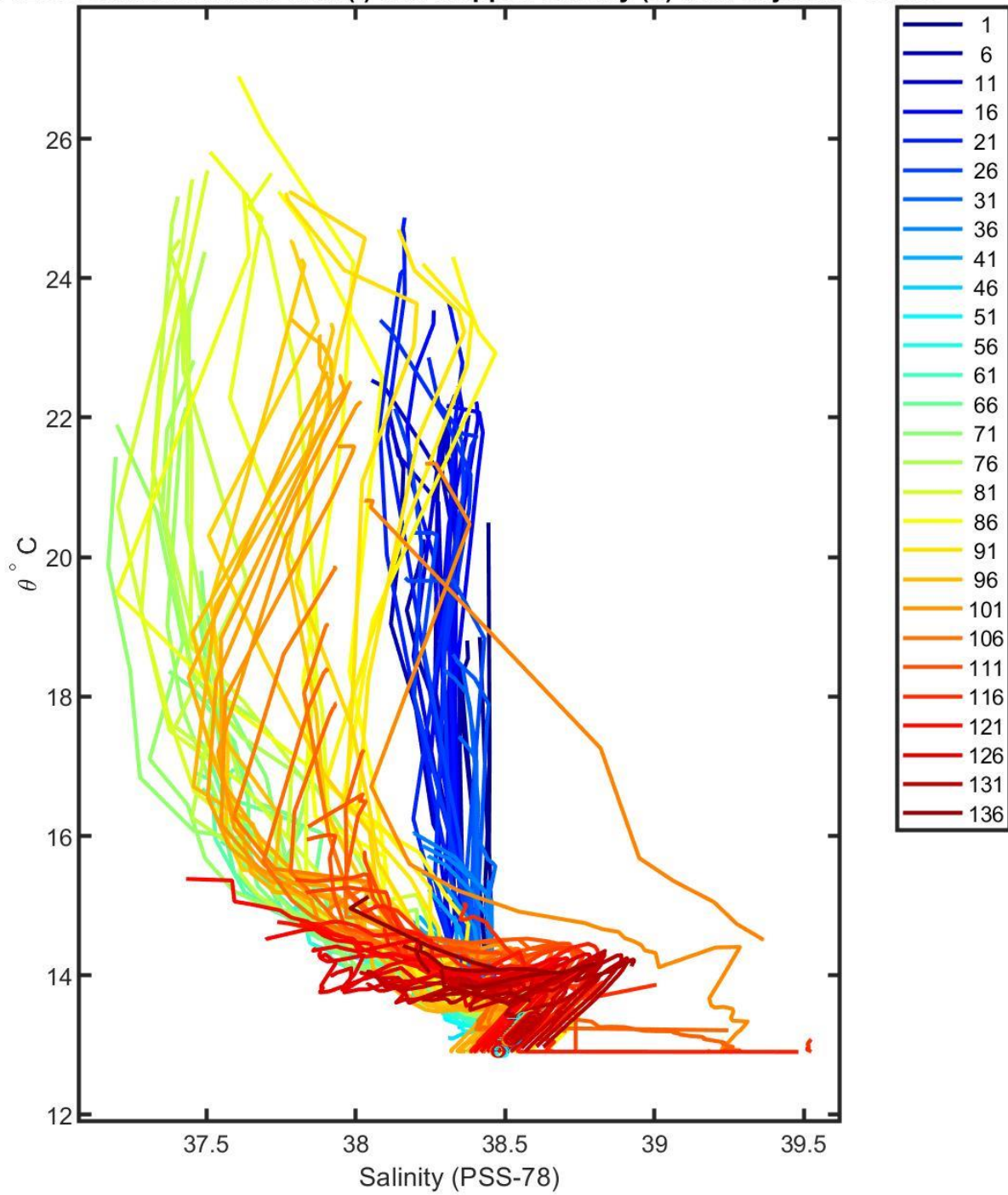
6902693 calibrated float data (-) and mapped salinity (o) with objective errors
