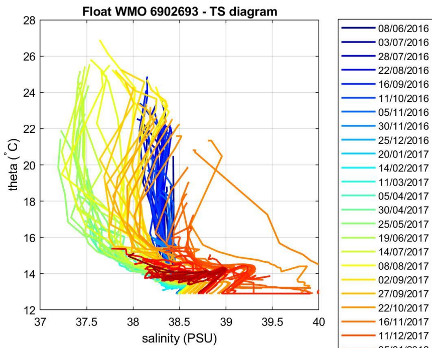
Figure 4: Float 6902693. \theta -S diagram color-coded per cycle number.
