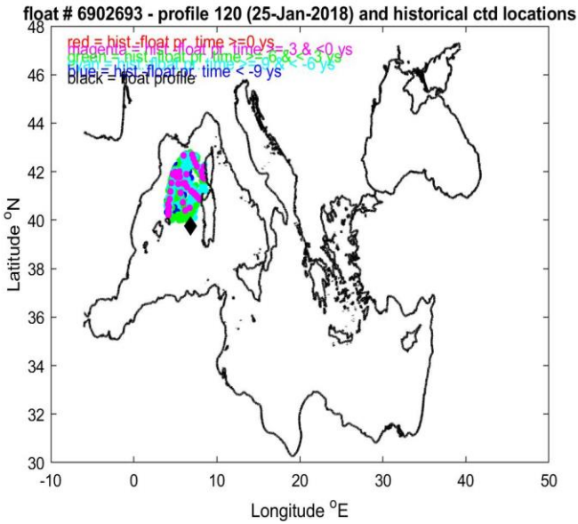
Figure 8: Float 6902693. Locations of the salinity float profile number 120 and historical CTD data (right panel) and the respective salinity profiles (left panel).
