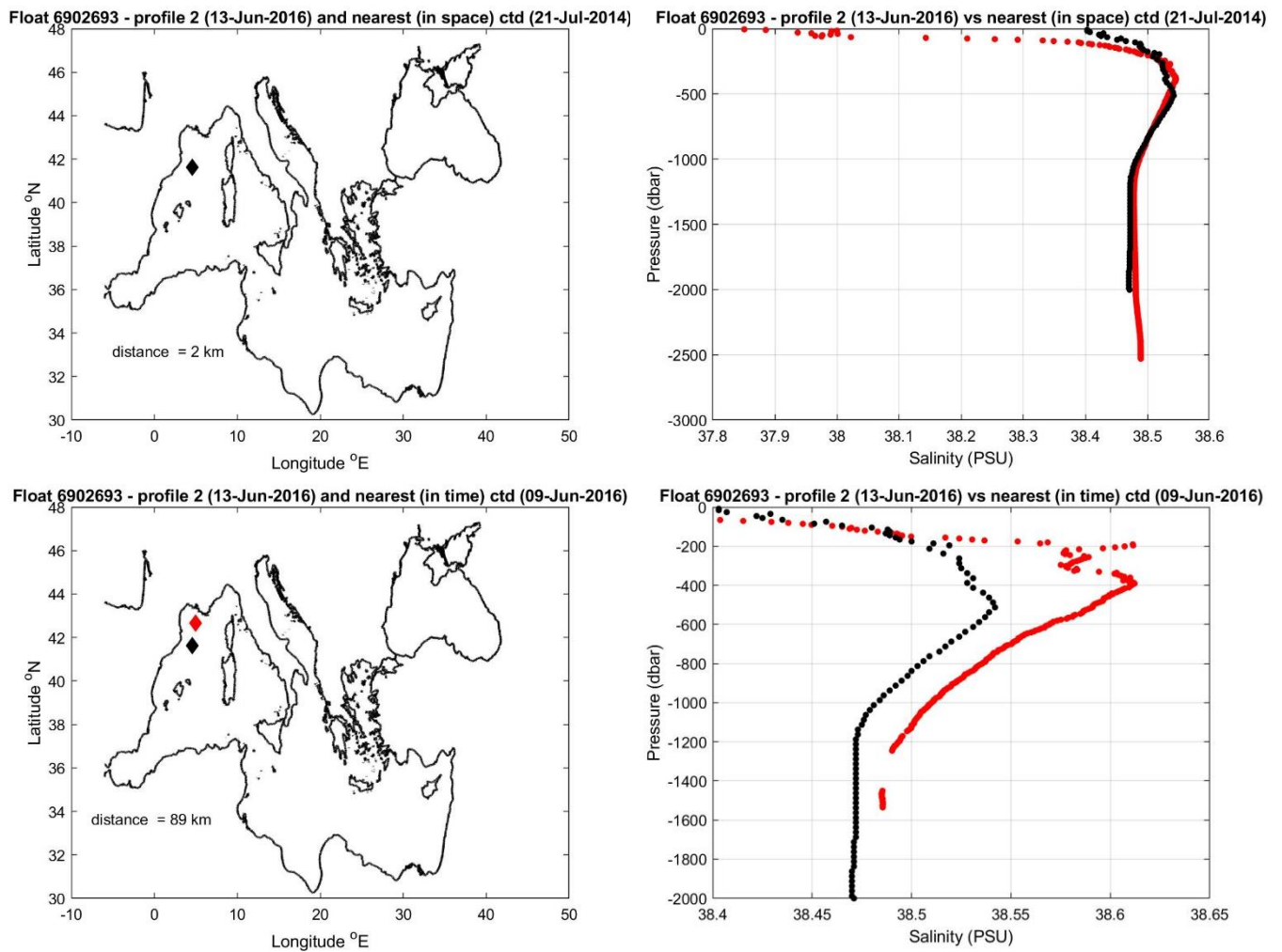
Figure 9: Float 6902693. The salinity float profile number 2 (black dots) are compared to the nearest in space (top) and in time (bottom) reference profile (red dots). The locations of the two profiles and their distance is given in the left panel.
