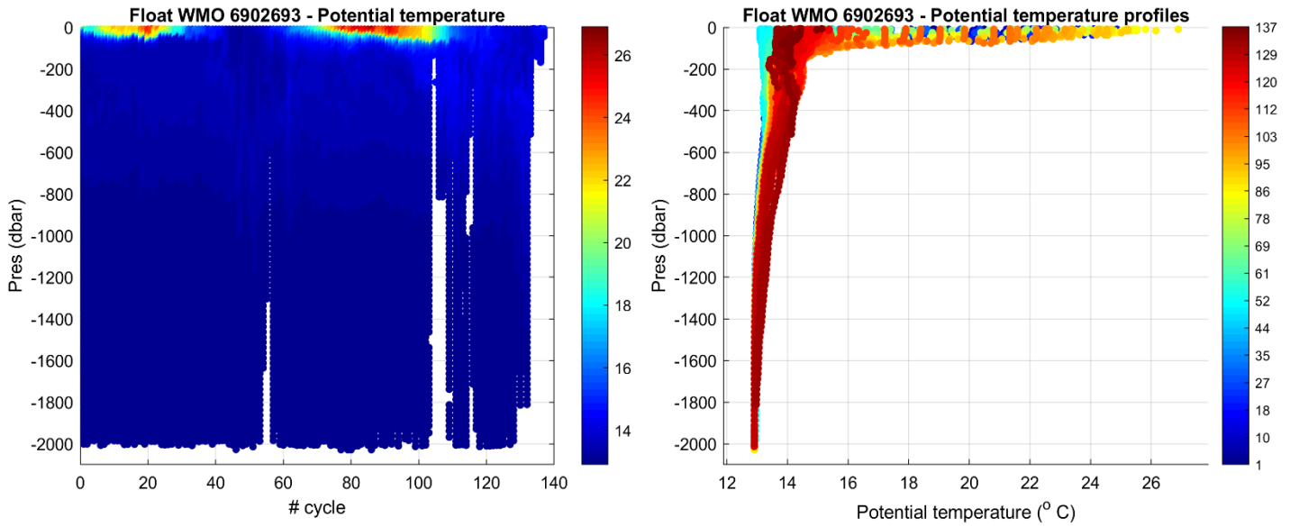
Figure 2: Float 6902693. Time series of Argo float potential temperature ( ^{\circ}\text{C} ) on the left, and potential temperature profiles color-coded per cycle number on the right.
