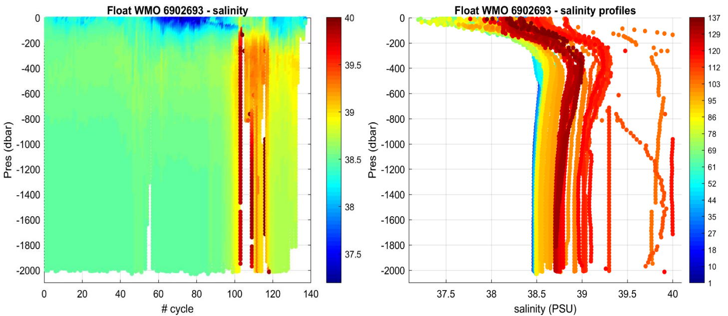
Figure 3: Float 6902693. Time series of Argo float potential salinity (PSS-78) on the left, and salinity profiles color-coded per cycle number on the right.
