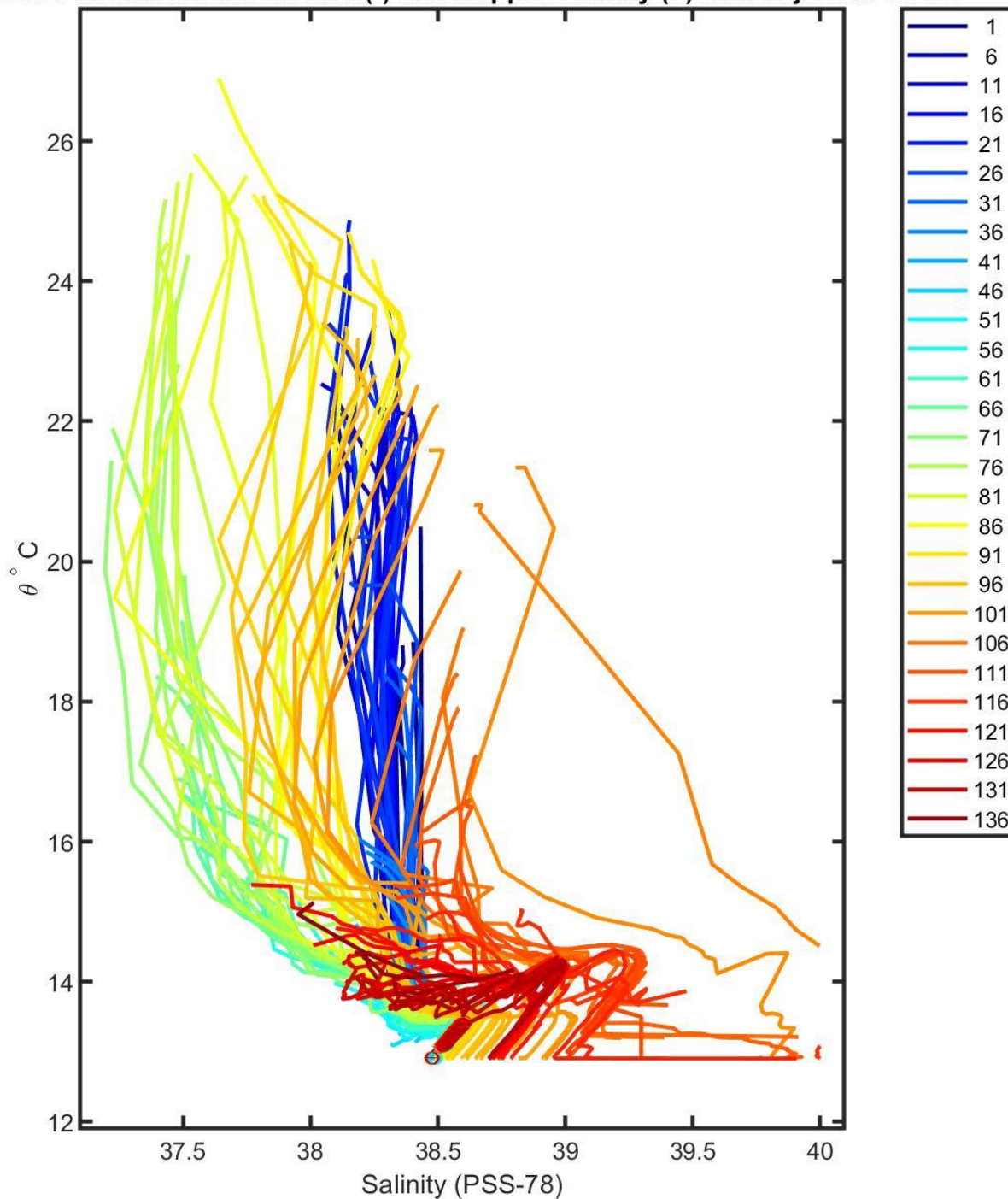
6902693 uncalibrated float data (-) and mapped salinity (o) with objective errors
