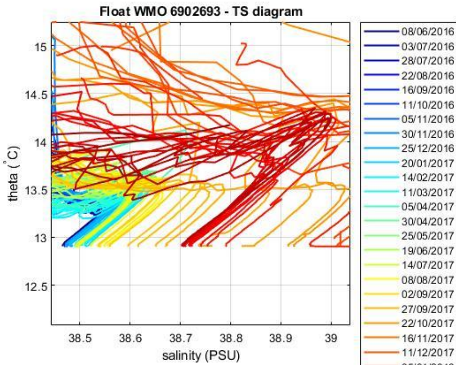
Figure 5: Float 6902693. Area of the \theta -S diagram (color-coded per cycle number) where the \theta -S relationship is more uniform.
