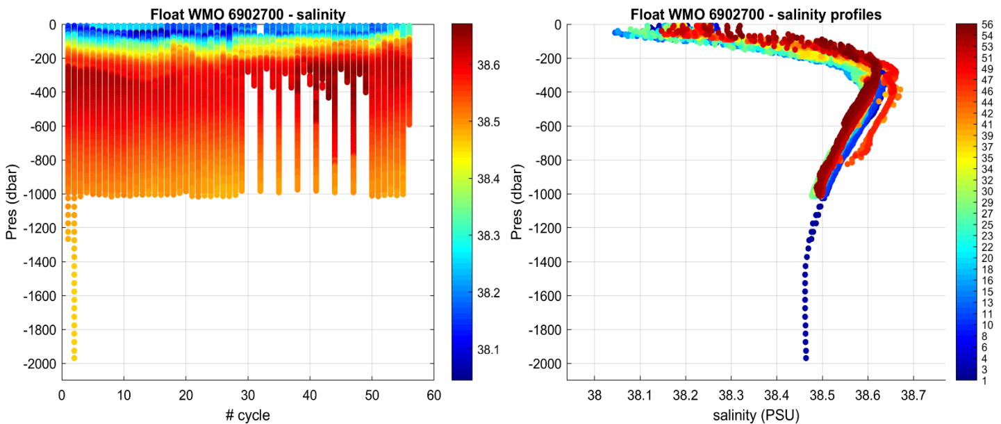
Figure 3: Float 6902700. Time series of Argo float potential salinity (PSS-78) on the left, and salinity profiles color-coded per cycle number on the right.
