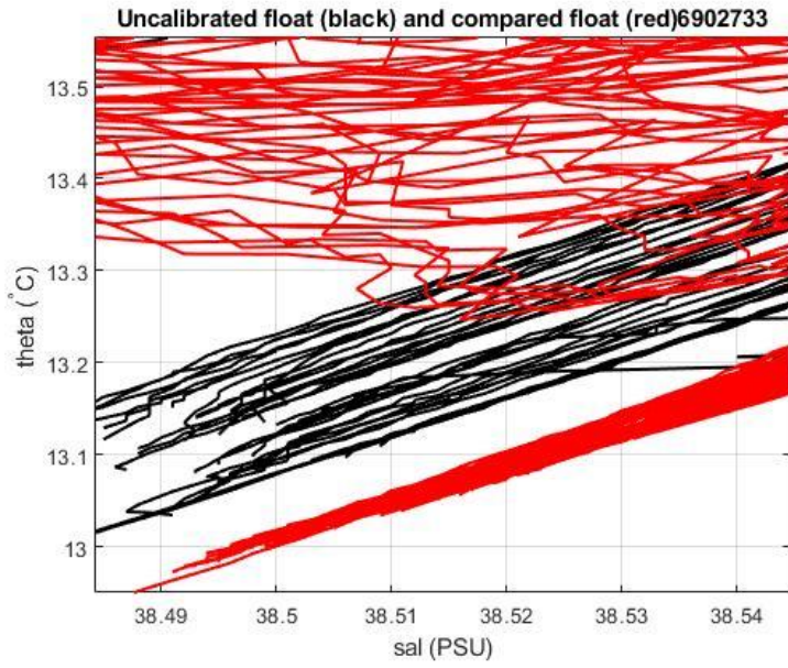
Figure 21: Float 6902700. Comparison between float 6902700 (black line) and float 6902733 on the left and float 3901849 on the right (red line), in the most uniform part of the \theta -S curve.
