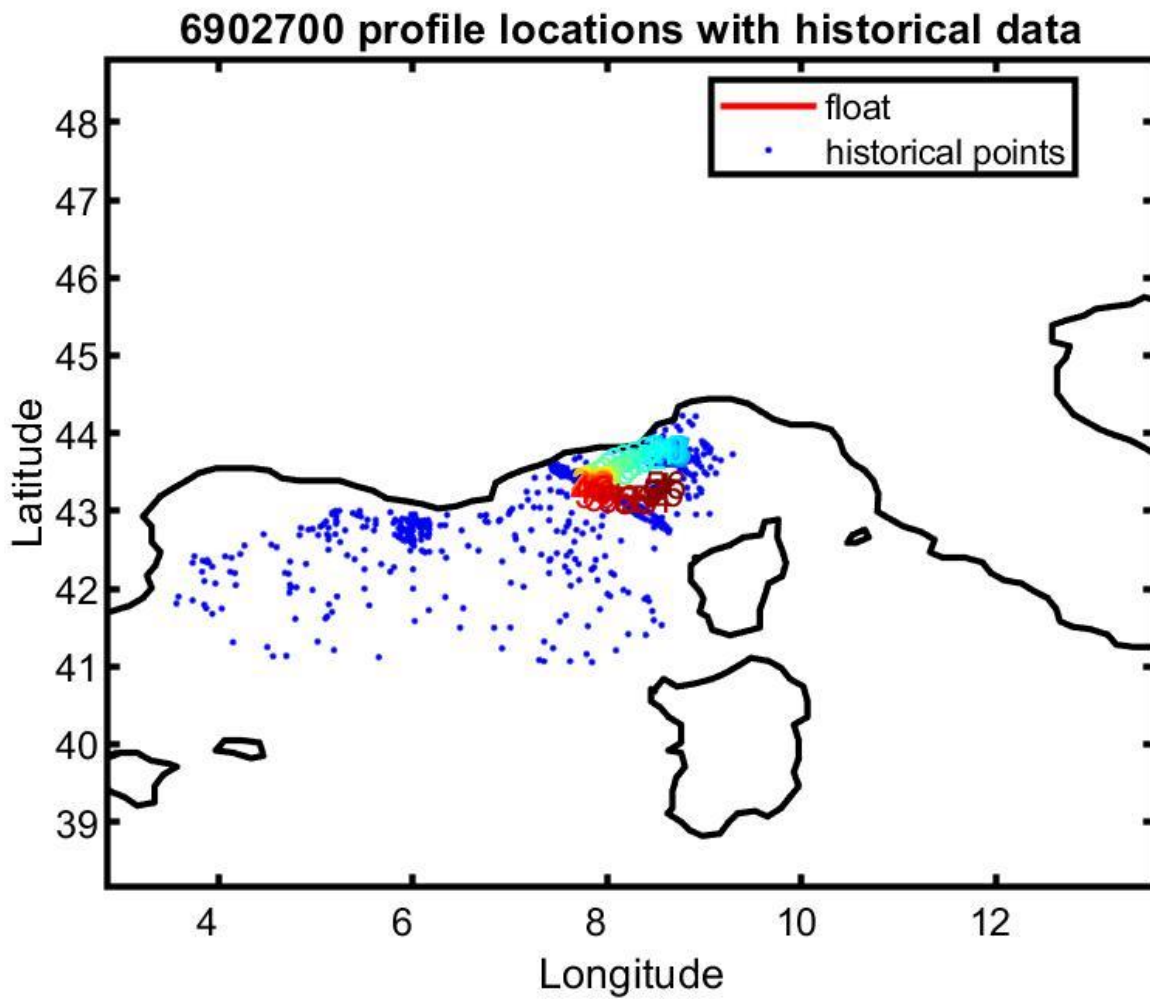
Figure 13: Float 6902700 Location of the float profiles (red line with colored numbers) and the reference data selected for mapping (blue dots).
