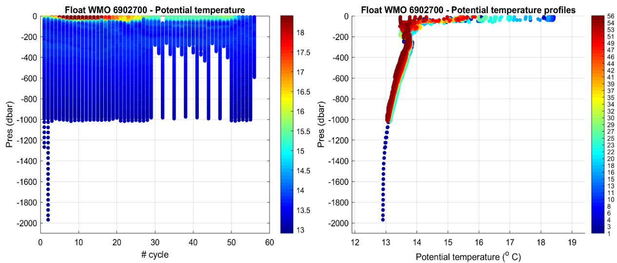
Figure 2: Float 6902700. Time series of Argo float potential temperature ( ^{\circ}\text{C} ) on the left, and potential temperature profiles color-coded per cycle number on the right.
