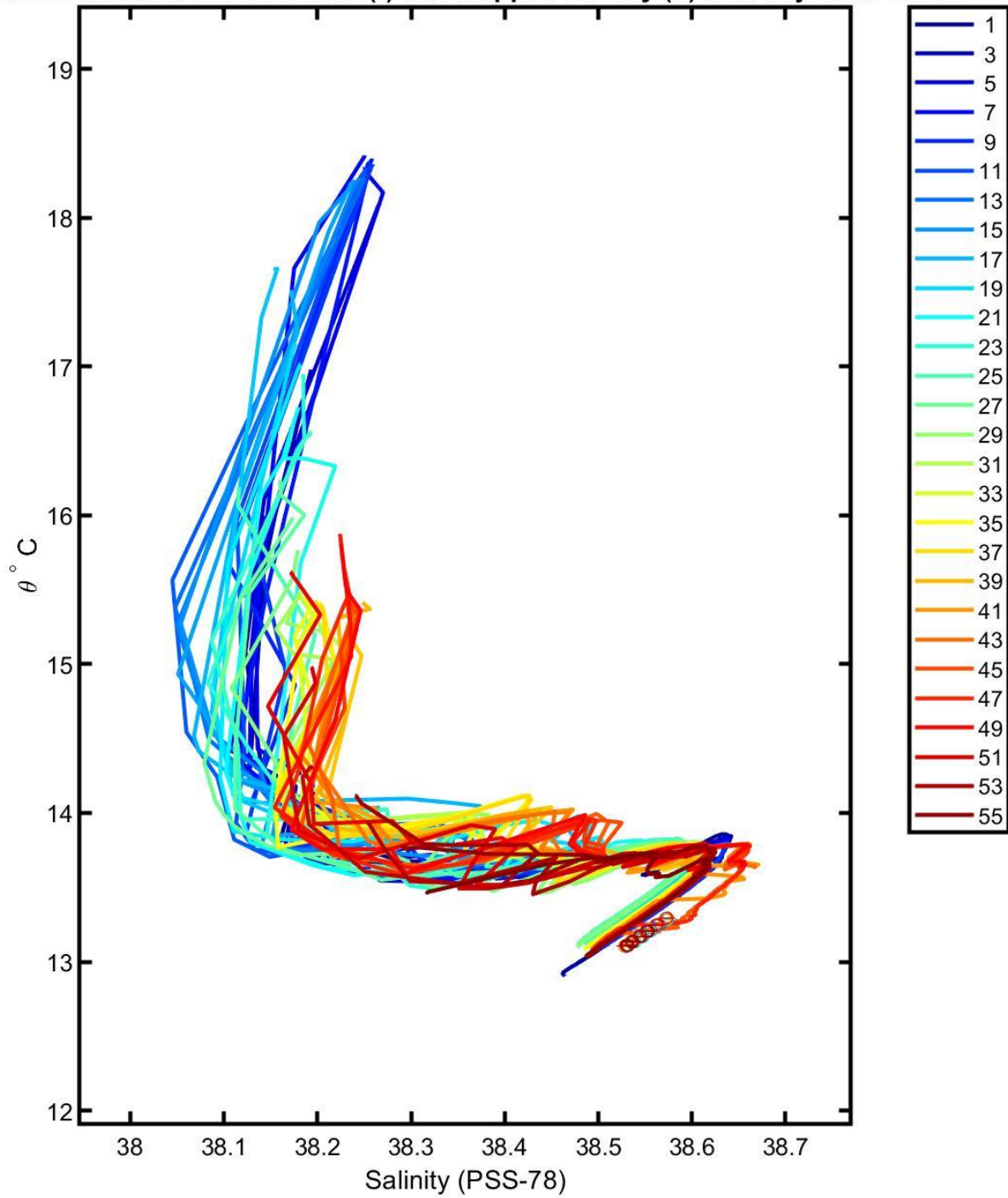
6902700 uncalibrated float data (-) and mapped salinity (o) with objective errors
