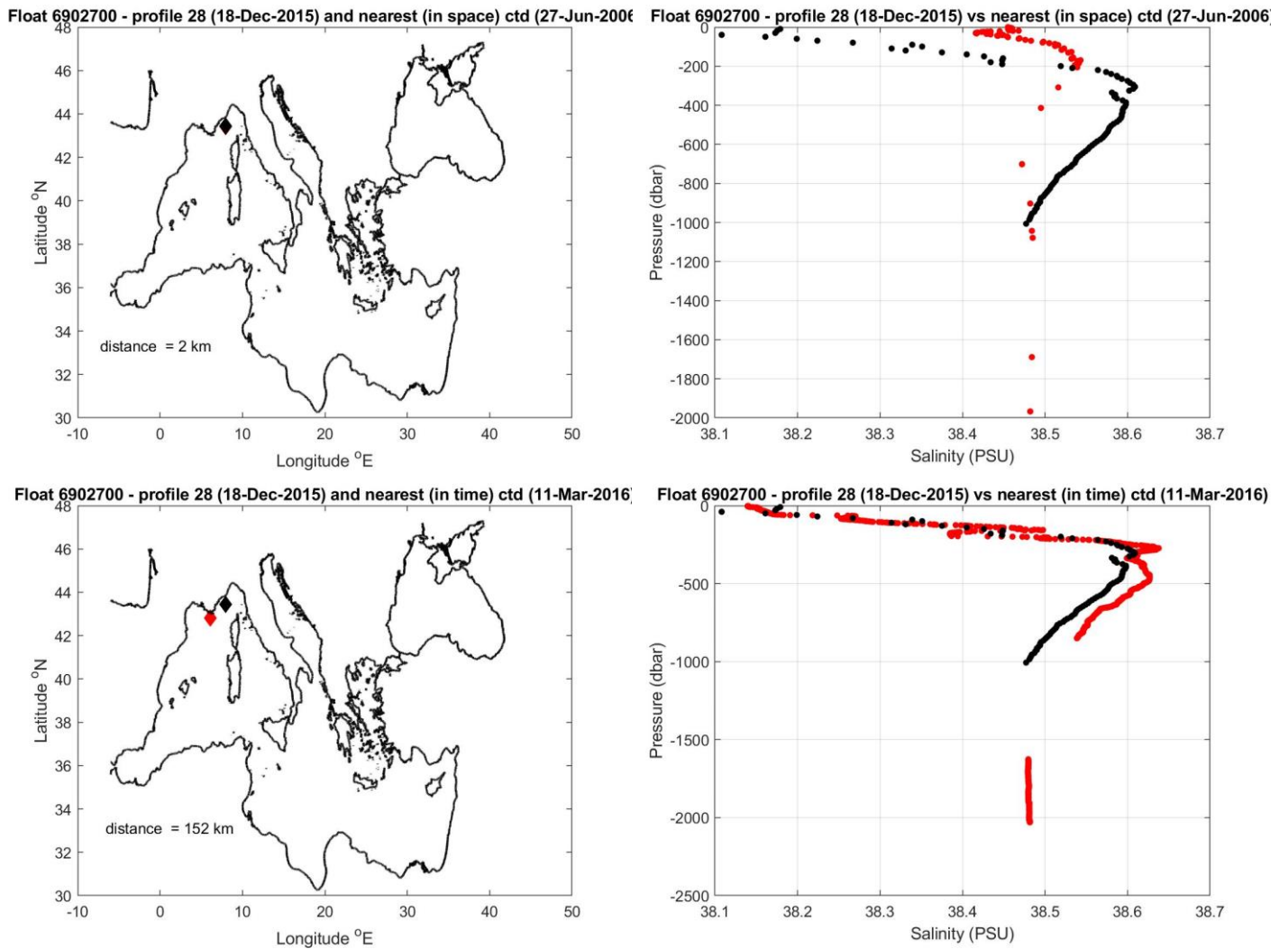
Figure 10: Float 6902700. The salinity float profile number 28 (black dots) are compared to the nearest in space (top) and in time (bottom) reference profile (red dots). The locations of the two profiles and their distance is given in the left panel.
