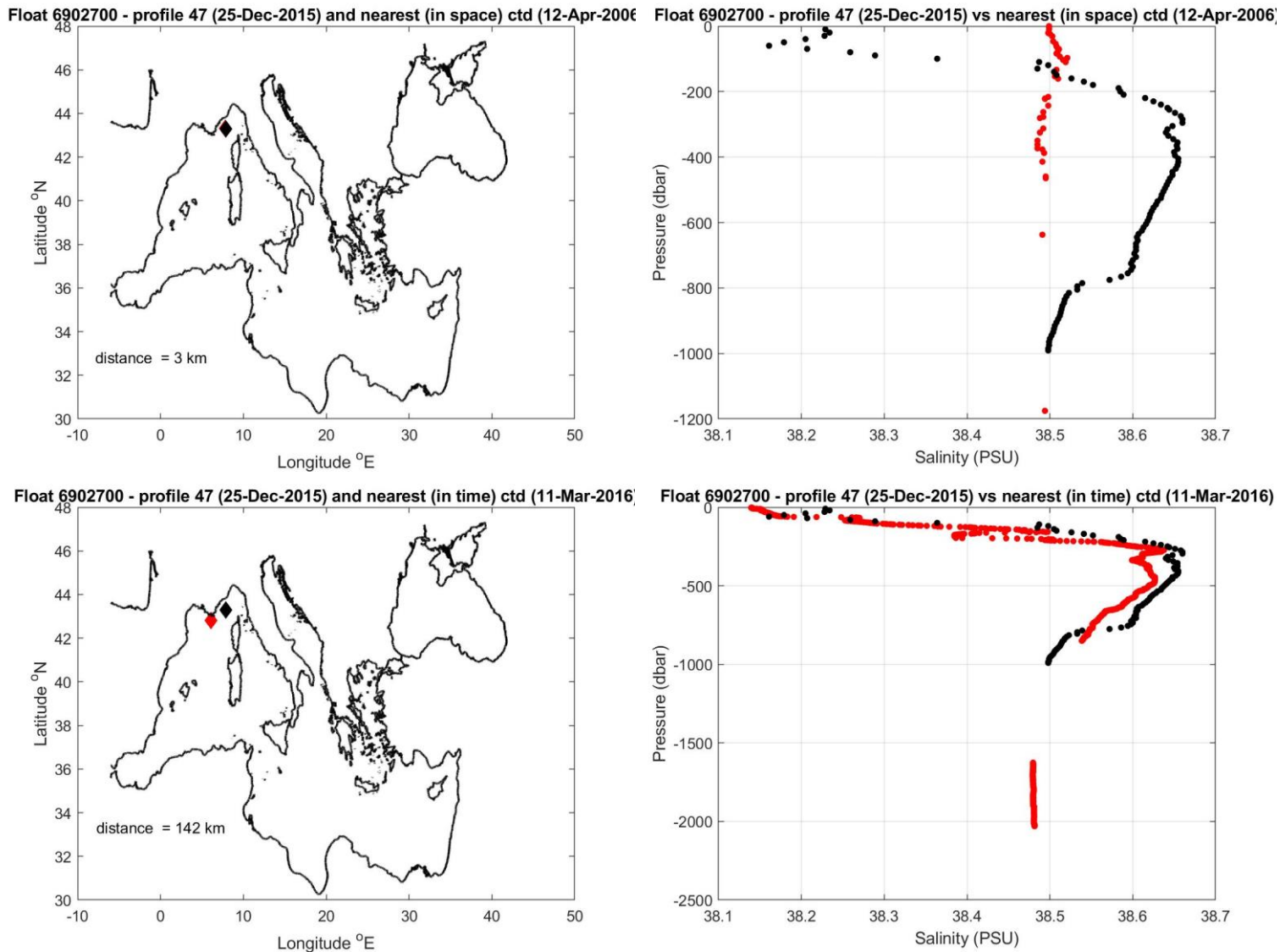
Figure 11: Float 6902700. The salinity float profile number 47 (black dots) are compared to the nearest in space (top) and in time (bottom) reference profile (red dots). The locations of the two profiles and their distance is given in the left panel.
