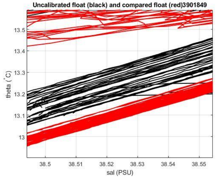
Figure 21: Float 6902700. Comparison between float 6902700 (black line) and float 6902733 on the left and float 3901849 on the right (red line), in the most uniform part of the \theta -S curve.
