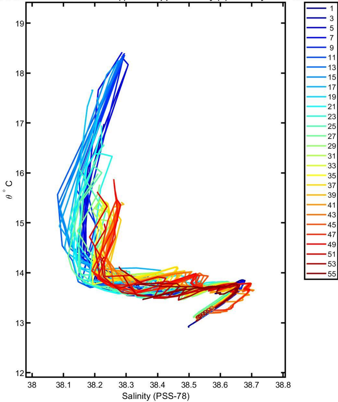
6902700 calibrated float data (-) and mapped salinity (o) with objective errors
