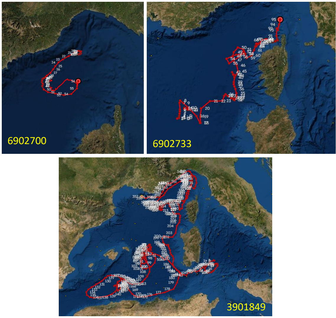
Figure 20: Float 6902700. Trajectory of the floats used for the comparison.
