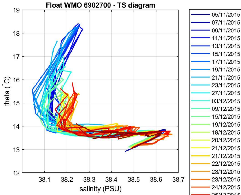
Figure 4: Float 6902700. \theta -S diagram color-coded per cycle number.
