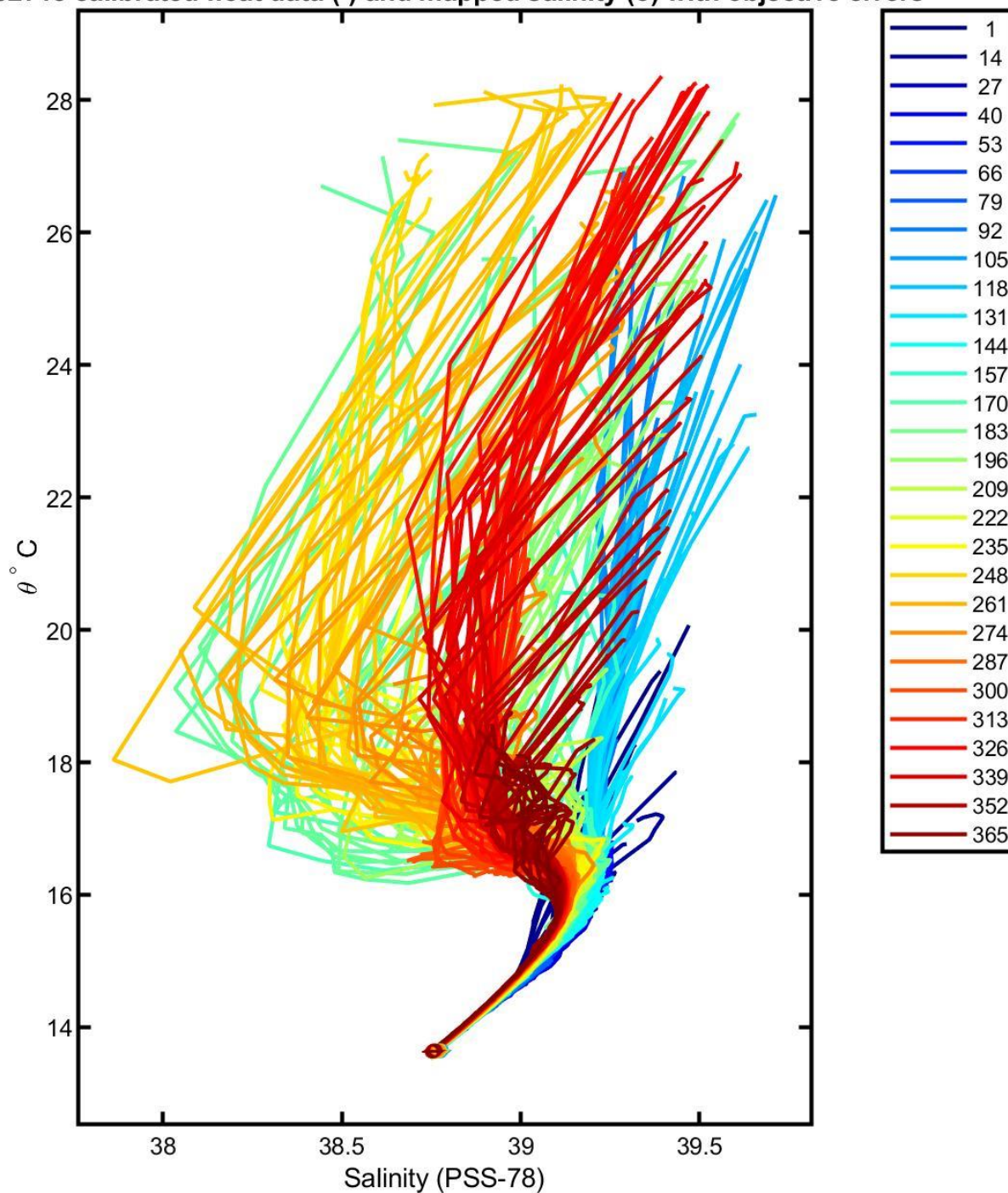
6902718 calibrated float data (-) and mapped salinity (o) with objective errors
