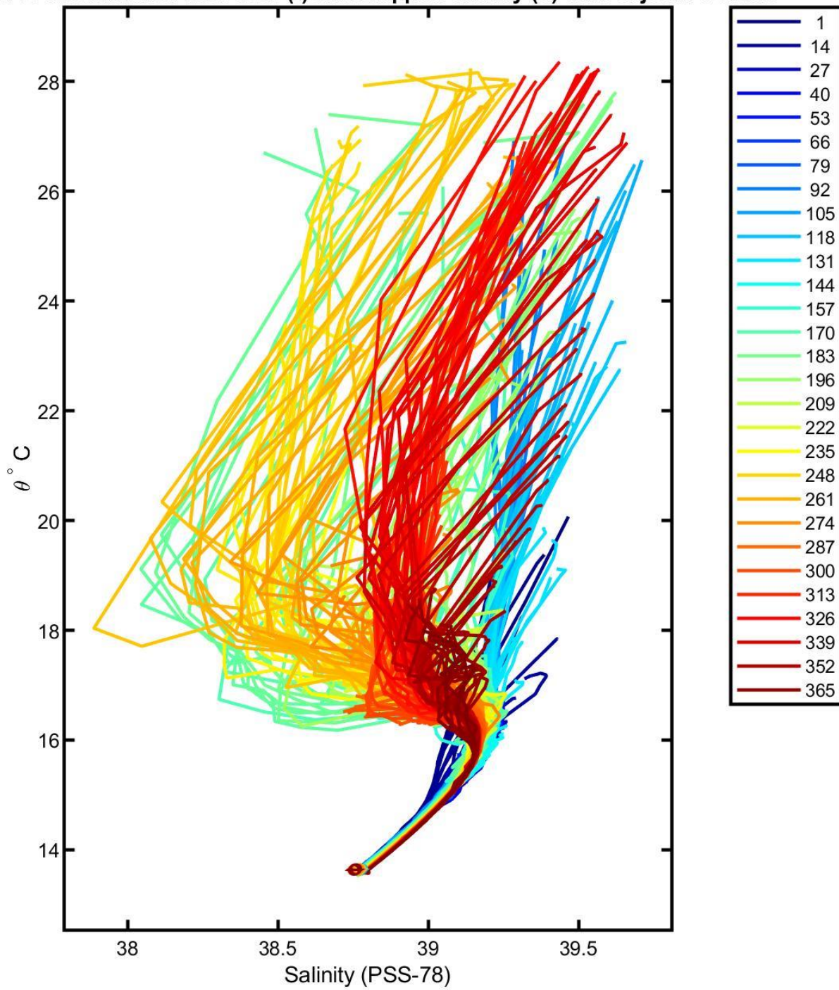
3902718 uncalibrated float data (-) and mapped salinity (o) with objective errors
