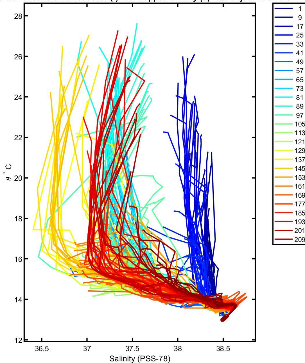
6902732 uncalibrated float data (-) and mapped salinity (o) with objective errors
