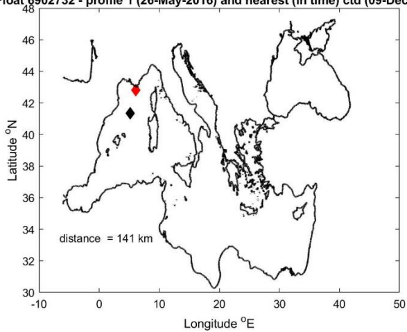
Float 6902732 - profile 1 (26-May-2016) and nearest (in time) ctd (09-Dec-2013)
