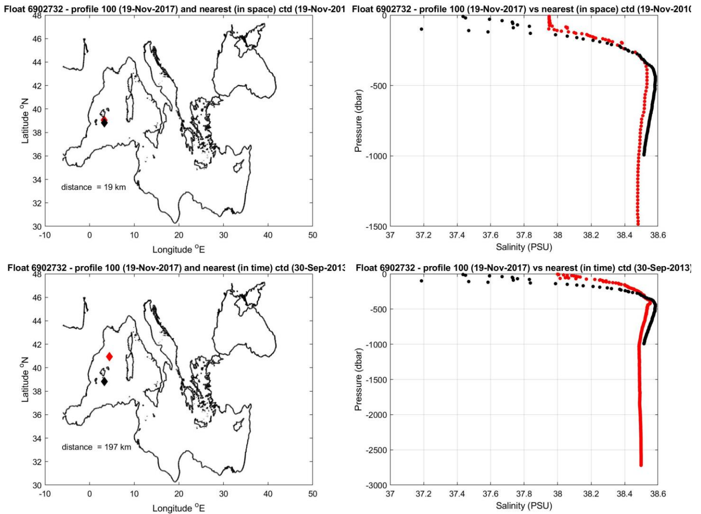
Figure 10: Float 6902732. The salinity float profile number 100 (black dots) are compared to the nearest in space (top) and in time (bottom) reference profile (red dots). The locations of the two profiles and their distance is given in the left panel.
