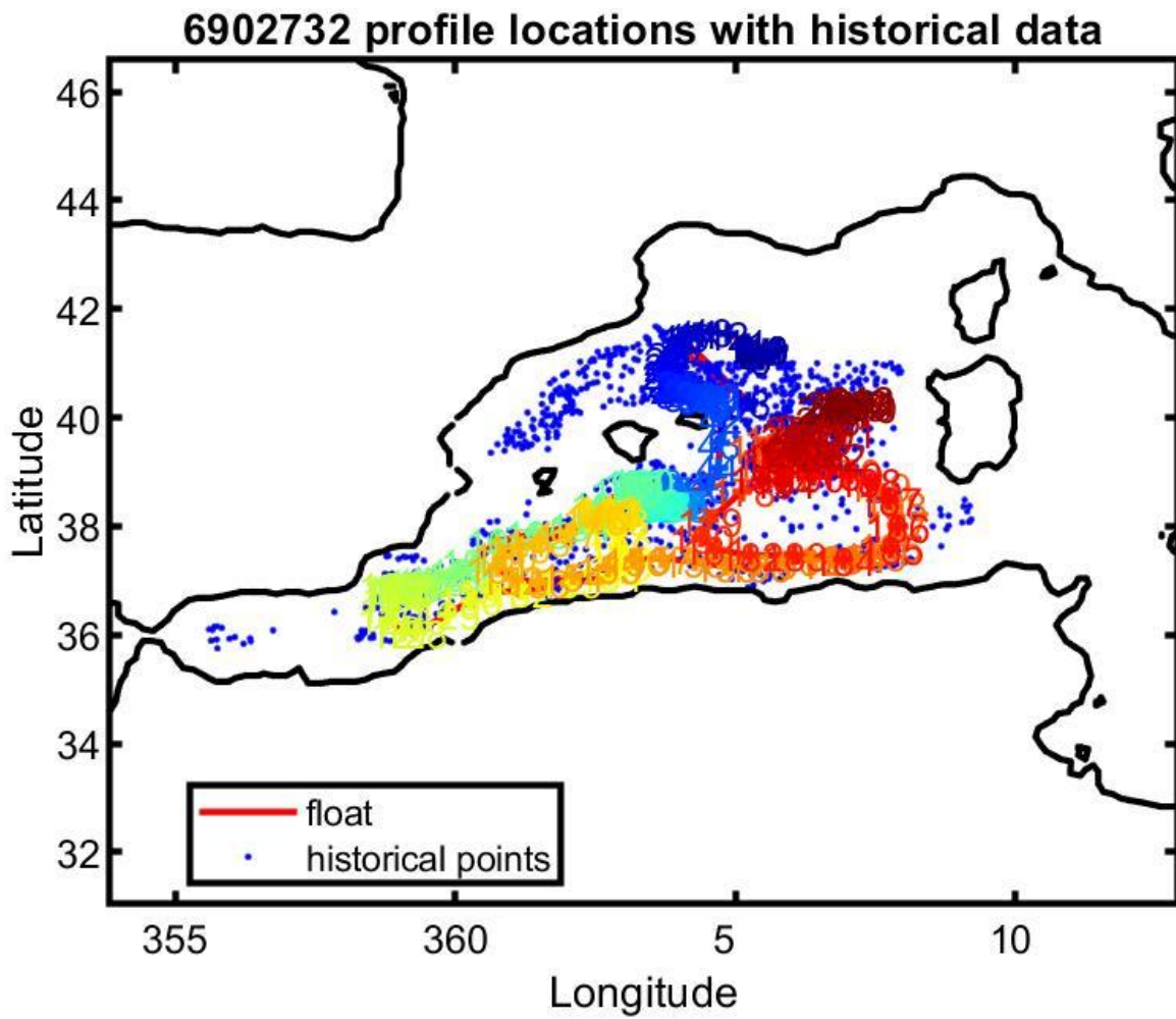
Figure 13: Float 6902732. Location of the float profiles (red line with colored numbers) and the reference data selected for mapping (blue dots).
