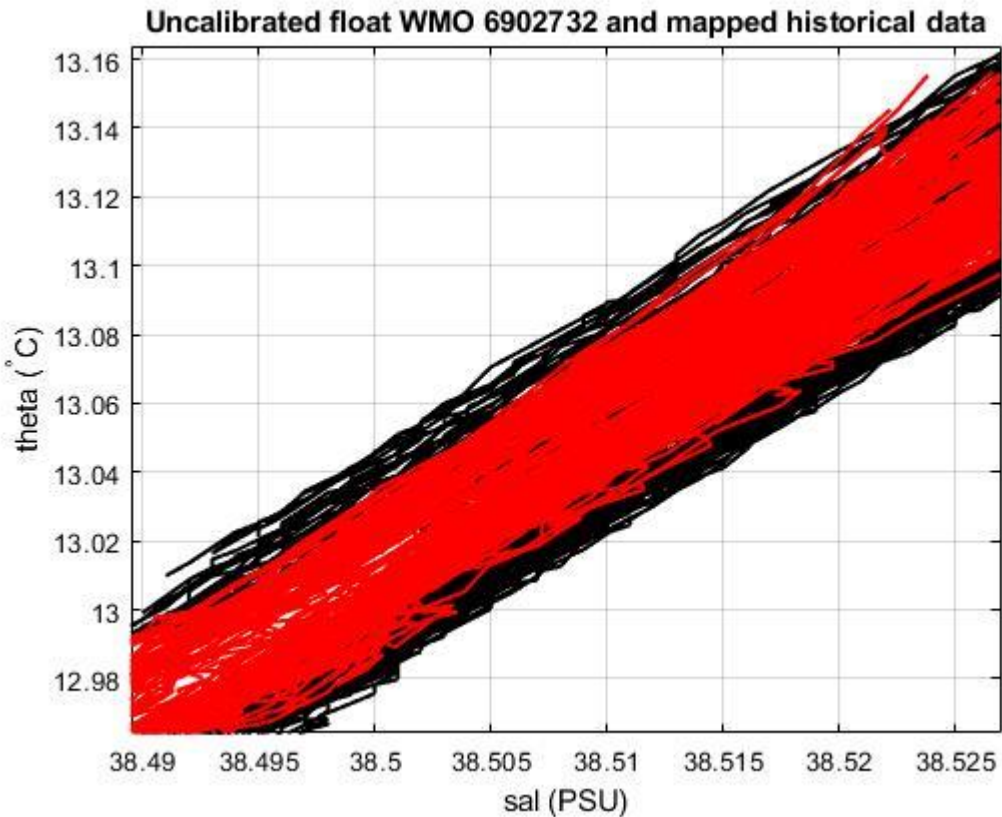
Figure 19: Float 6902732. Uncalibrated float salinity profile (black lines) and mapped historical data (red lines) in the most uniform part of the \theta -S curve.
