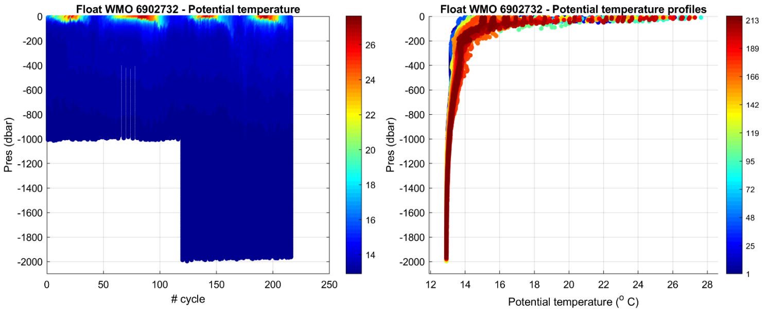
Figure 2: Float 6902732. Time series of Argo float potential temperature ( ^{\circ}\text{C} ) on the left, and potential temperature profiles color-coded per cycle number on the right.
