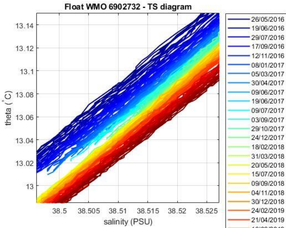
Figure 5: Float 6902732. Area of the \theta -S diagram (color-coded per cycle number) where the \theta -S relationship is more uniform.
