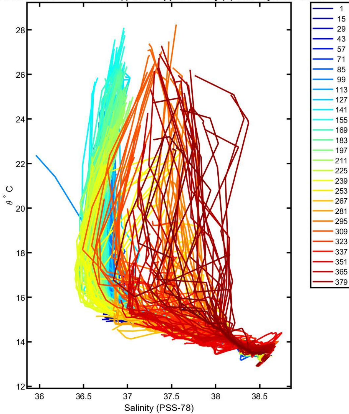
6902764 calibrated float data (-) and mapped salinity (o) with objective errors
