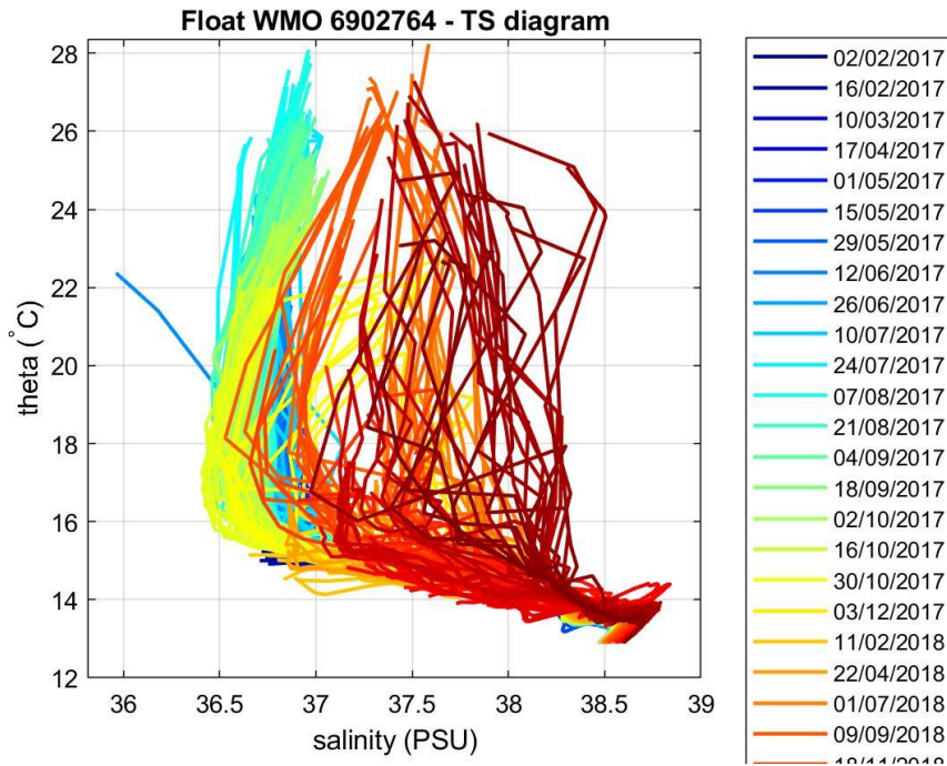
Figure 4: Float 6902764. \theta -S diagram color-coded per cycle number.
