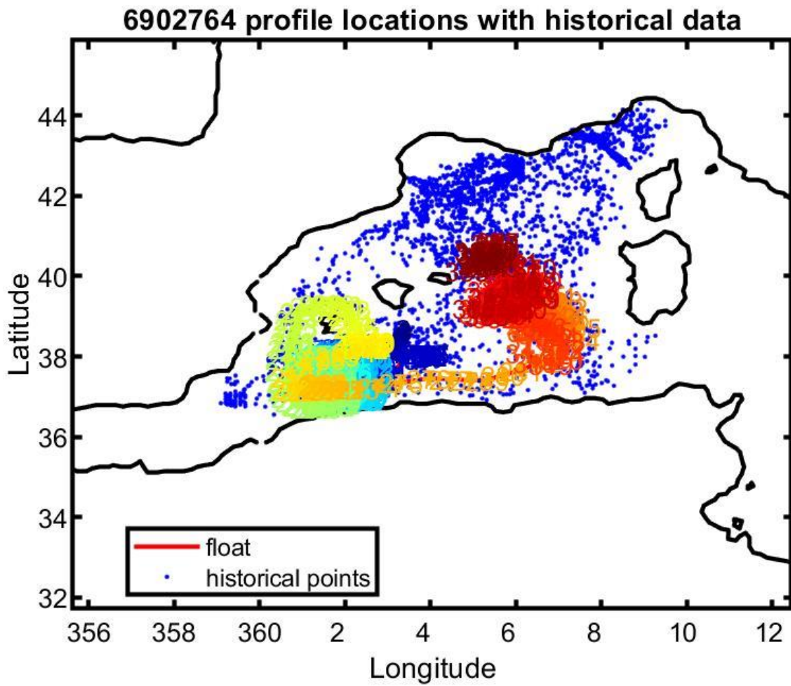
Figure 13: Float 6902764. Location of the float profiles (red line with colored numbers) and the reference data selected for mapping (blue dots).
