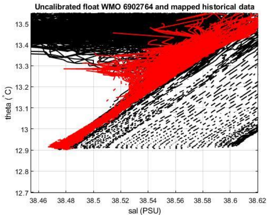
Figure 19: Float 6902764. Uncalibrated float salinity profile (black lines) and mapped historical data (red lines) in the most uniform part of the \theta -S curve.
