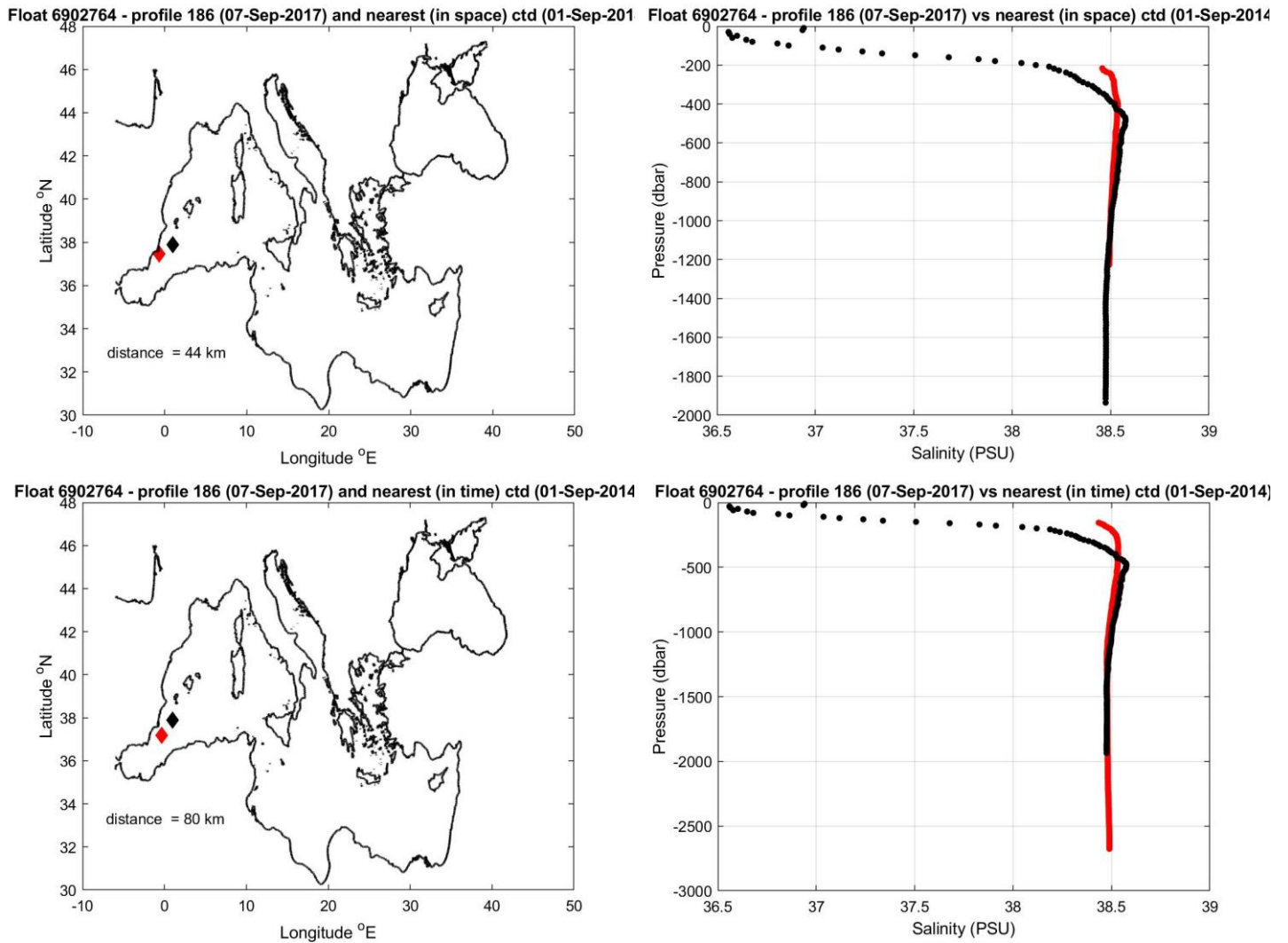
Figure 10: Float 6902764. The salinity float profile number 186 (black dots) are compared to the nearest in space (top) and in time (bottom) reference profile (red dots). The locations of the two profiles and their distance is given in the left panel.
