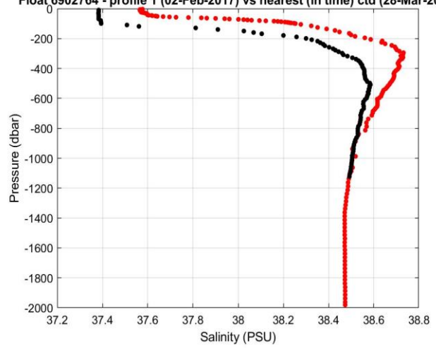
Float 6902764 - profile 1 (02-Feb-2017) vs nearest (in time) ctd (28-Mar-2017)
