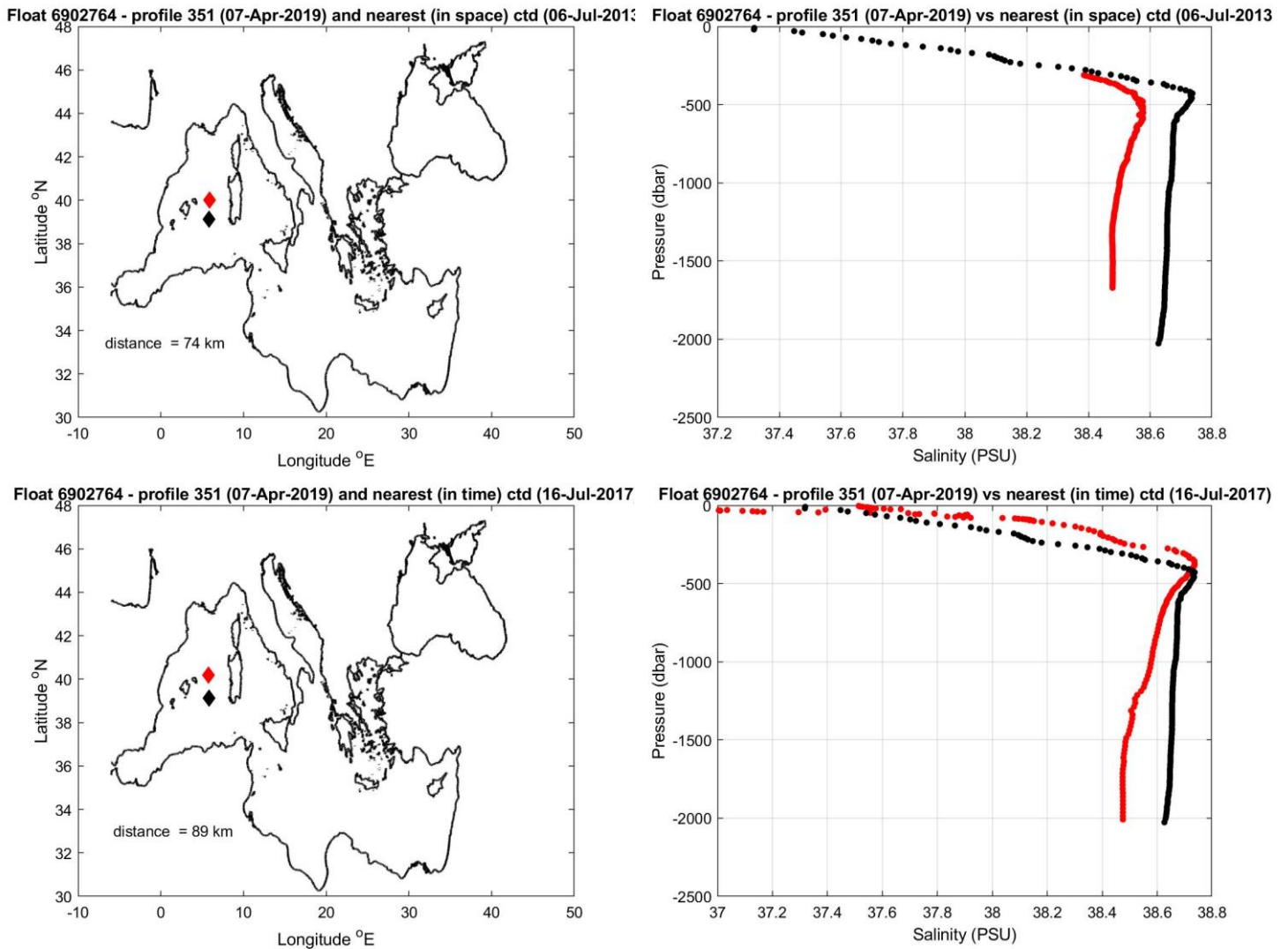
Figure 11: Float 6902764. The salinity float profile number 351 (black dots) are compared to the nearest in space (top) and in time (bottom) reference profile (red dots). The locations of the two profiles and their distance is given in the left panel.
