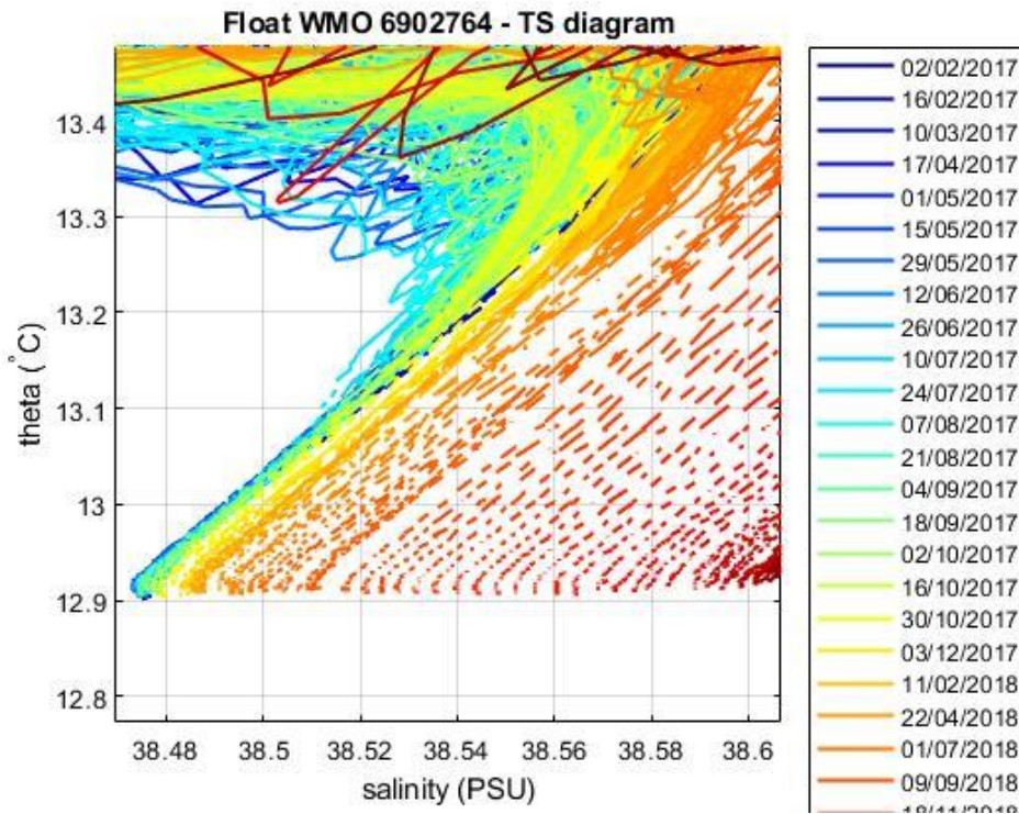
Figure 5: Float 6902764. Area of the \theta -S diagram (color-coded per cycle number) where the \theta -S relationship is more uniform.
