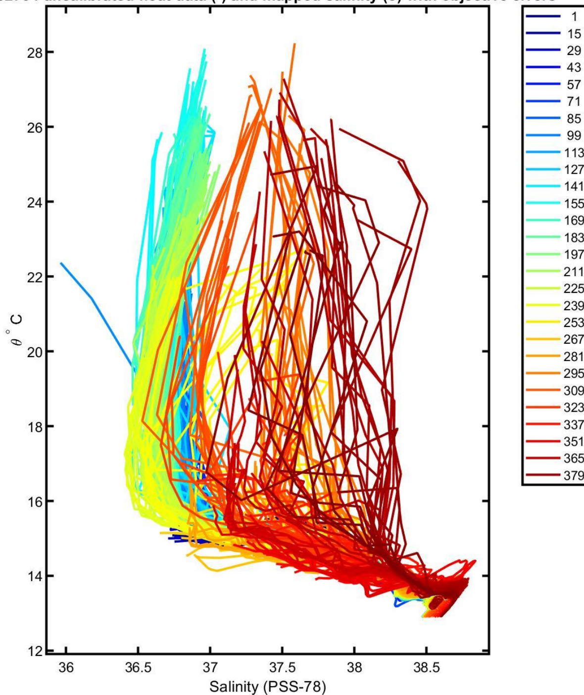
6902764 uncalibrated float data (-) and mapped salinity (o) with objective errors
