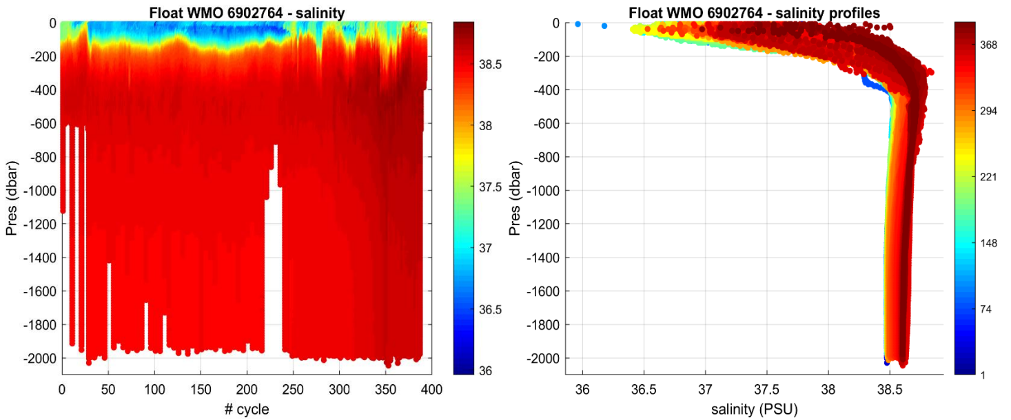
Figure 3: Float 6902764. Time series of Argo float potential salinity (PSS-78) on the left, and salinity profiles color-coded per cycle number on the right.
