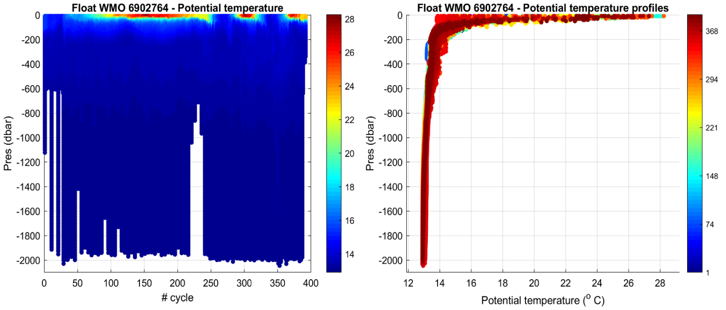
Figure 2: Float 6902764. Time series of Argo float potential temperature ( ^{\circ}\text{C} ) on the left, and potential temperature profiles color-coded per cycle number on the right.
