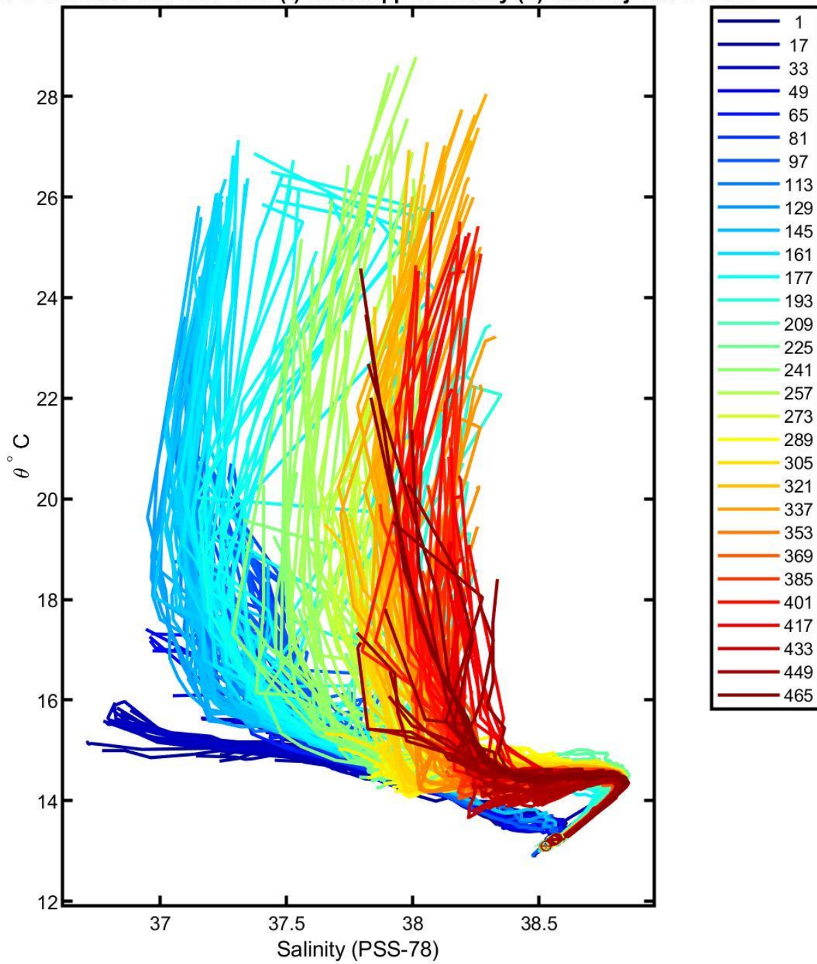
3902767 uncalibrated float data (-) and mapped salinity (o) with objective errors
