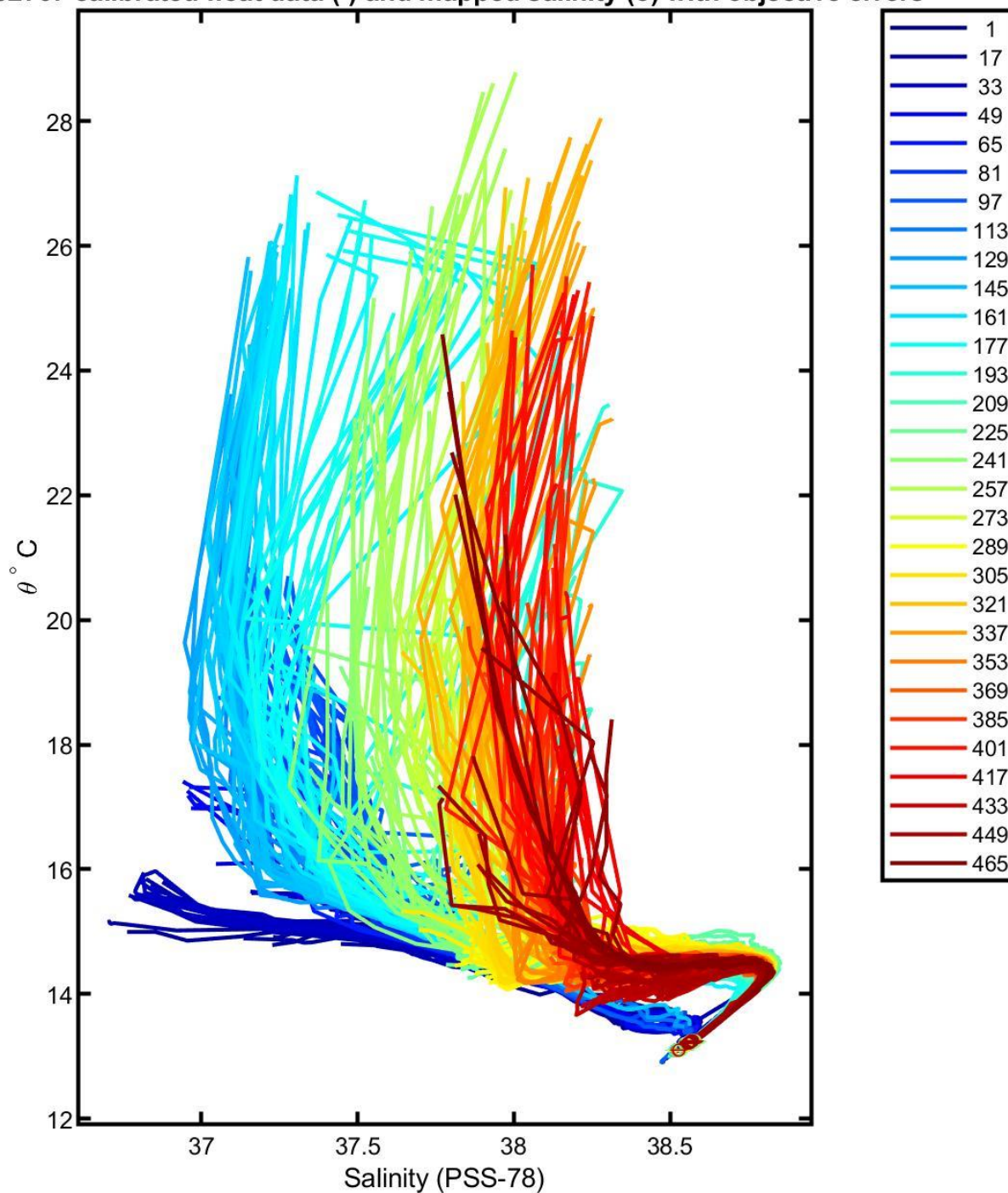
6902767 calibrated float data (-) and mapped salinity (o) with objective errors
