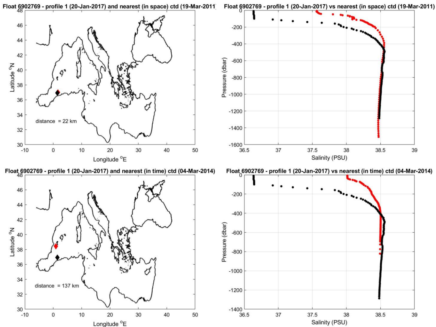
Figure 9: Float 6902769. The salinity float profile number 1 (black dots) are compared to the nearest in space (top) and in time (bottom) reference profile (red dots). The locations of the two profiles and their distance is given in the left panel.
