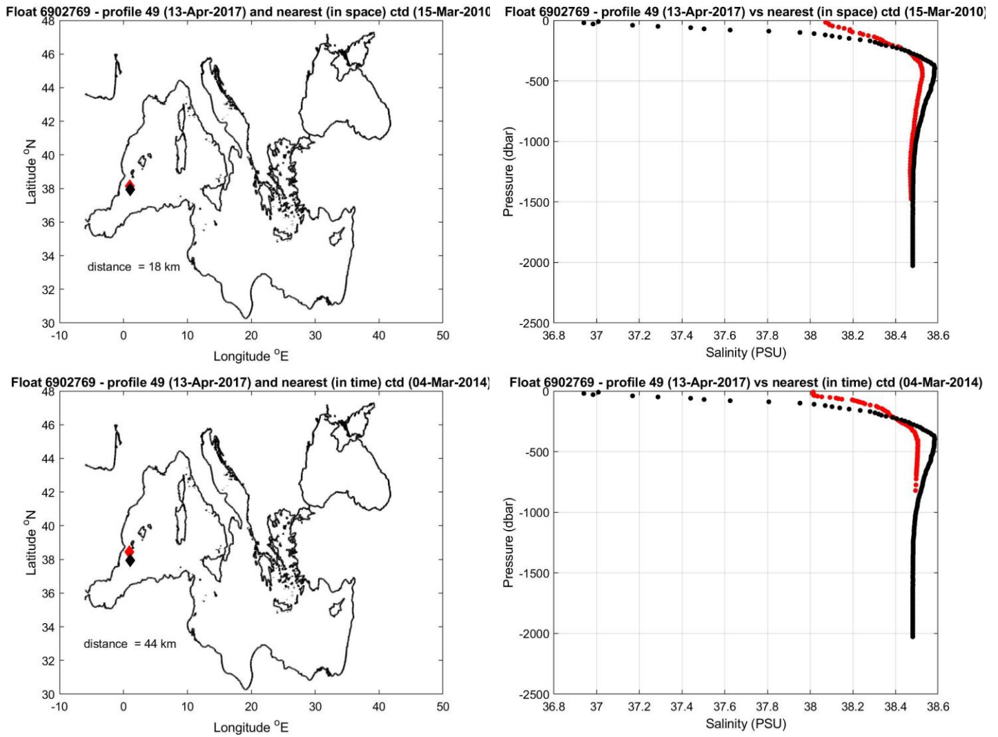
Figure 10: Float 6902769. The salinity float profile number 49 (black dots) are compared to the nearest in space (top) and in time (bottom) reference profile (red dots). The locations of the two profiles and their distance is given in the left panel.
