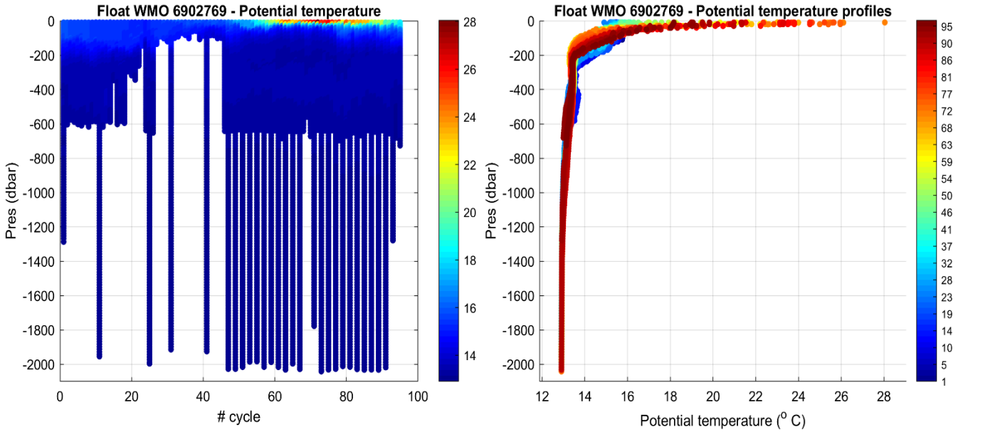
Figure 2: Float 6902769. Time series of Argo float potential temperature ( ^{\circ}\text{C} ) on the left, and potential temperature profiles color-coded per cycle number on the right.
