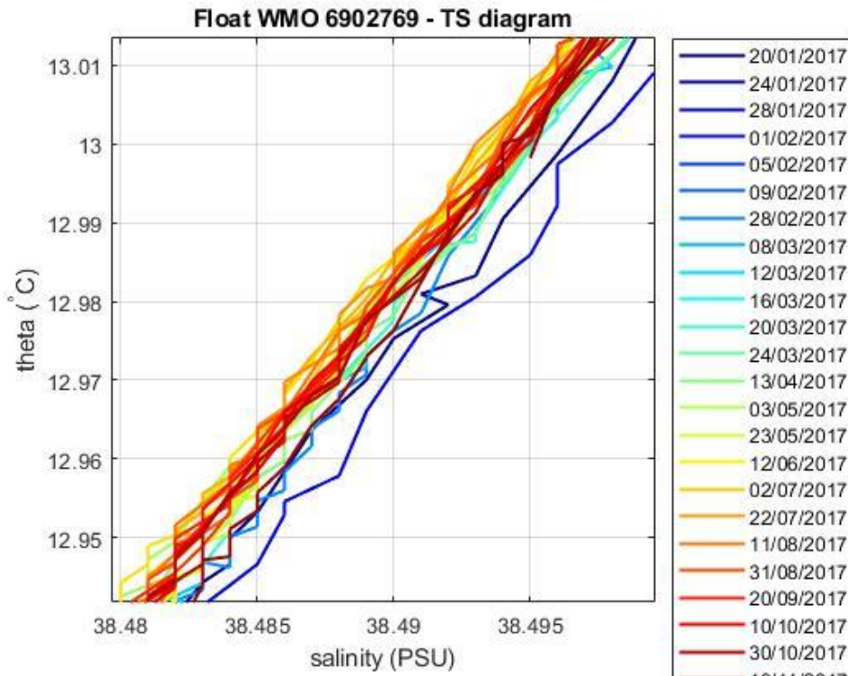
Figure 5: Float 6902769. Area of the \theta -S diagram (color-coded per cycle number) where the \theta -S relationship is more uniform.
