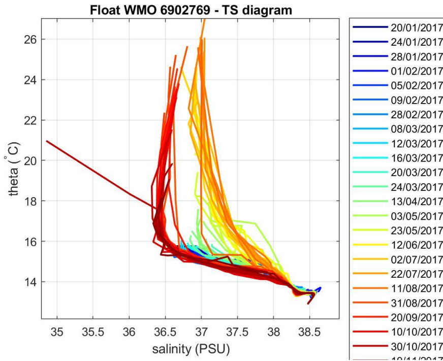
Figure 4: Float 6902769. \theta -S diagram color-coded per cycle number.
