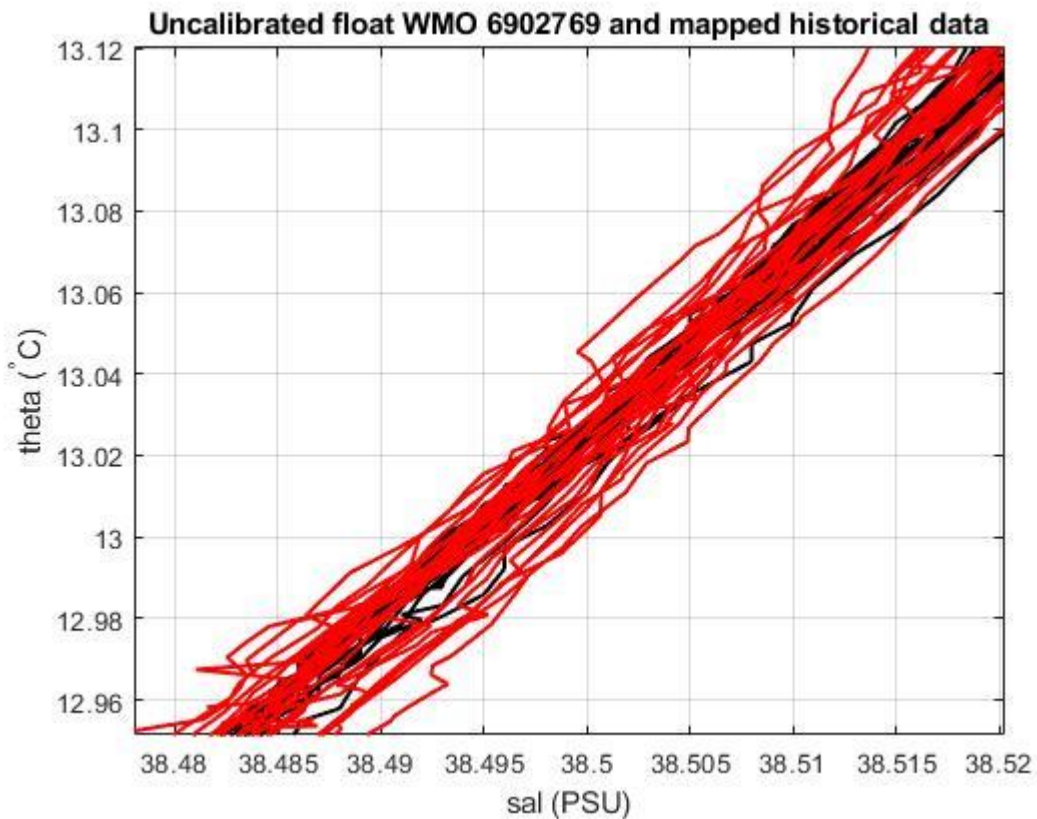
Figure 19: Float 6902769. Uncalibrated float salinity profile (black lines) and mapped historical data (red lines) in the most uniform part of the \theta -S curve.
