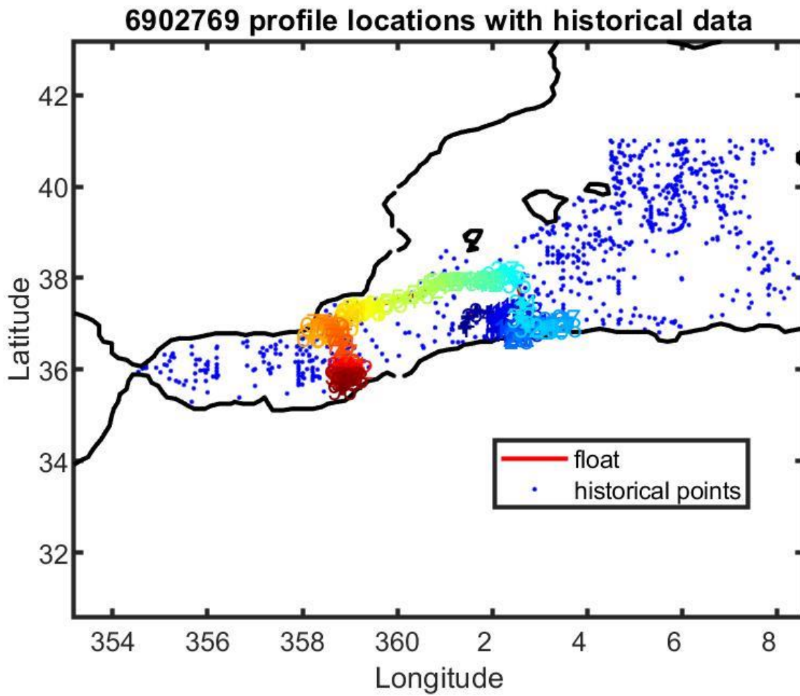
Figure 13: Float 6902769. Location of the float profiles (red line with colored numbers) and the reference data selected for mapping (blue dots).
